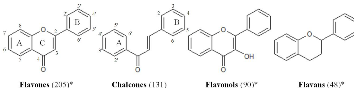
Figure 1. The most important flavonoid classes represented in the flavonoids chemical library. The amount of compounds per class present in the library is indicated between parentheses. Flavanones, isoflavonoids, neoflavonoids and dihydroflavonols are also included. * The numbering of the chemical structure of the flavonols and flavans is similar to the flavones, and it follows the criteria of [15].
