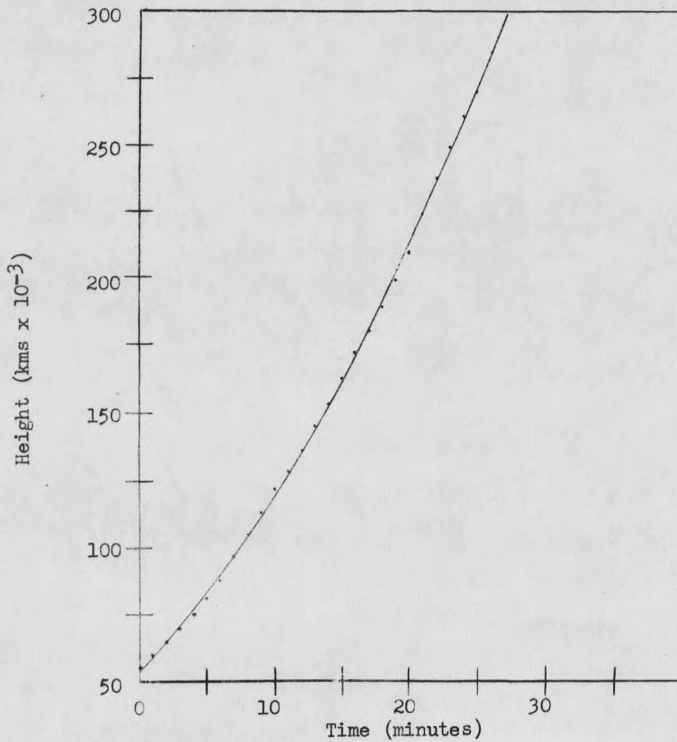
Figure 10. Illustrating the fit of the curve y = 5.80 \times 10^4 + 3.75 \times 10^3 t + 167 t^2 to the observed points plotted from a measure of the height (y) vs. the time along the ordinate x = 40 for the lower envelope of the prominence.
