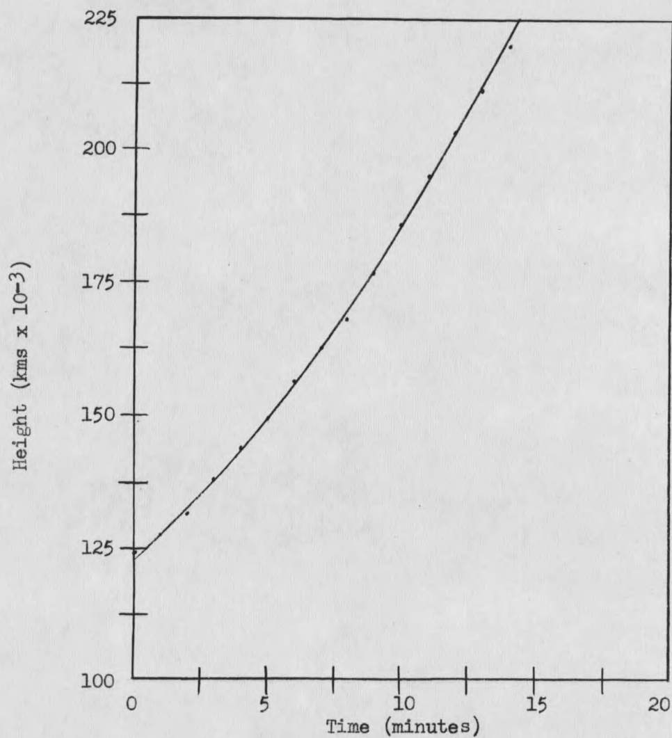
Figure 13. Illustrating the fit of the curve y = 1.24 \times 10^5 + 4.31 \times 10^3 t + 183 t^2 to the observed points plotted from a measure of the height (y) vs. the time along the ordinate x = -30 for the upper envelope of the prominence.
