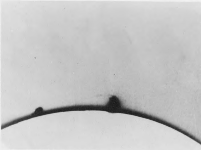
Figure 5. The prominence at 19 h 00 m U.T. The material visible at the top of figure 4 has risen out of the scope of the camera. The two mounds of material shown here remained this way for more than an hour.
