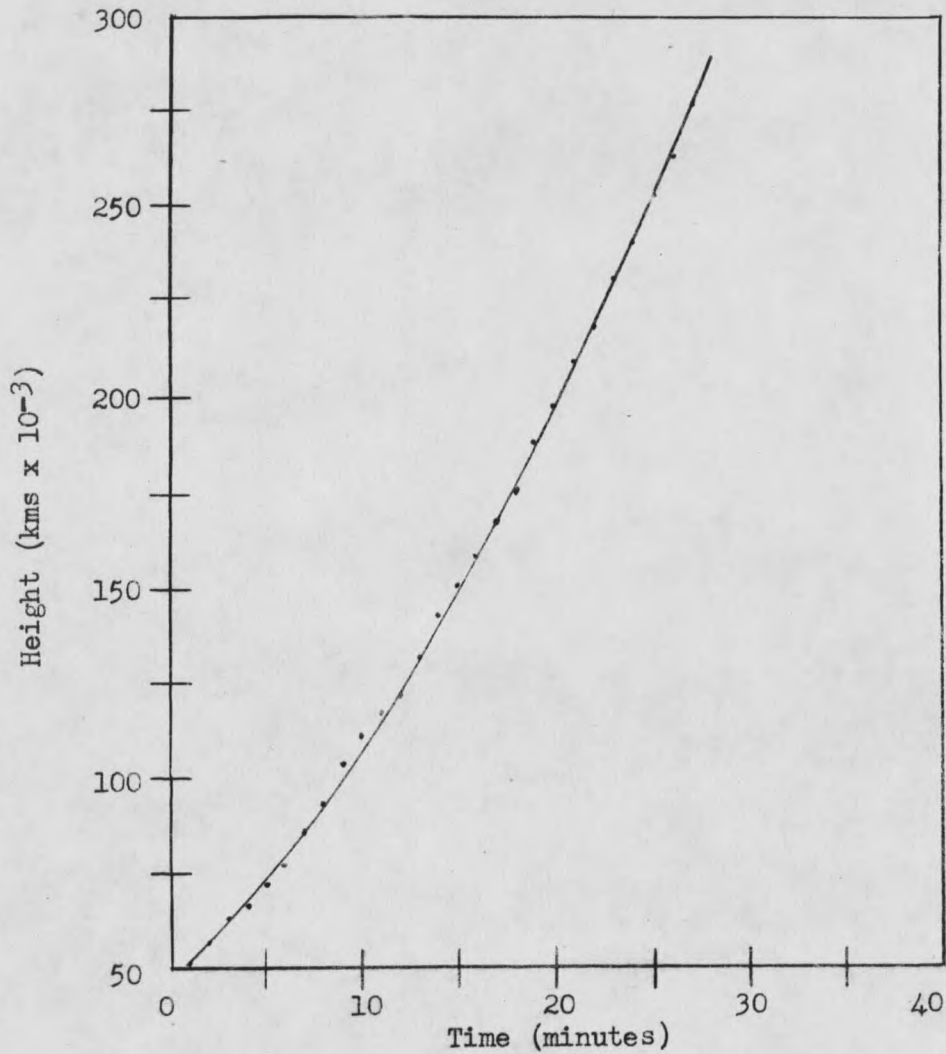
Figure 9. Illustrating the fit of the curve y = 4.80 \times 10^4 + 3.62 \times 10^3 t + 129t^2 to the observed points plotted from a measure of the height (y) vs. the time along the ordinate x = -20 for the lower envelope of the prominence.
