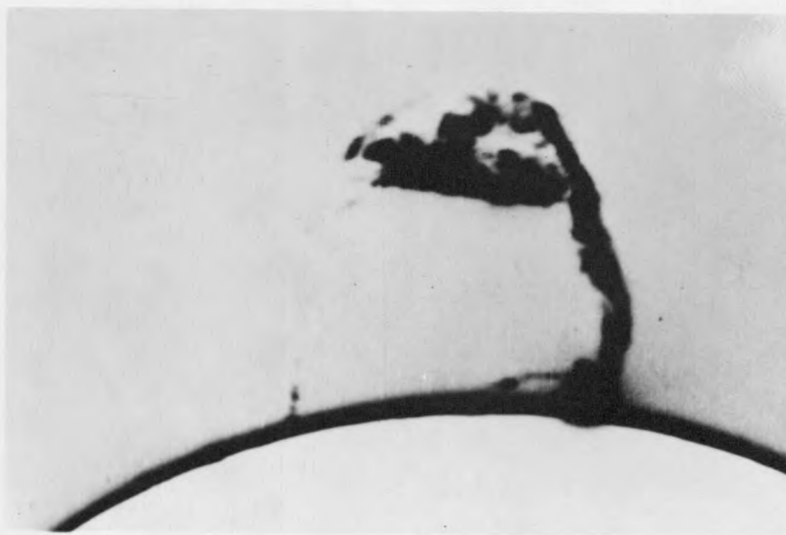
Figure 3. The prominence at 18 h 00 m U.T. Note the gradual formation of the looplike arch.
