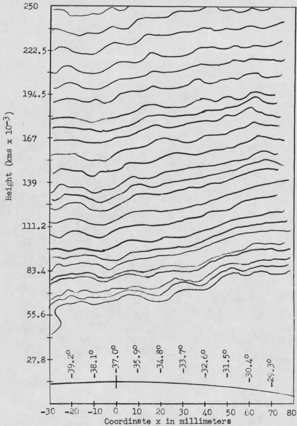
Figure 6. Showing the lower envelopes of the prominence as they were traced. The region shown is that lying between the parallel lines of figures 3 and 4. Time between any two curves is one minute.
