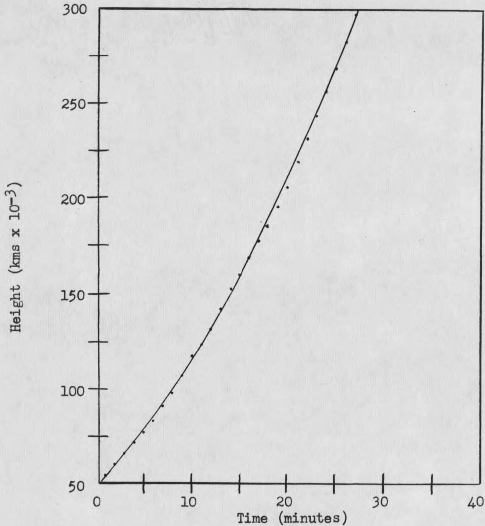
Figure 11. Illustrating the fit of the curve y = 5.00 \times 10^4 + 4.10 \times 10^3 t + 190 t^2 to the observed points plotted from a measure of the height (y) vs. the time along the ordinate x = 20 for the lower envelope of the prominence.
