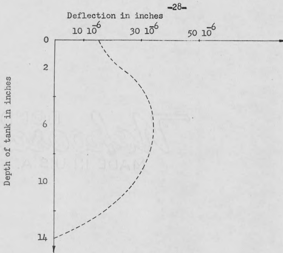
Fig. 7. Deflection diagram along center lines AG and BF (see Fig. 1a.)
