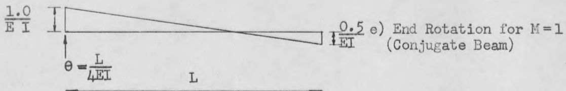
Fig. 2. Study of Relative Stiffness - Prismatic Beams.
