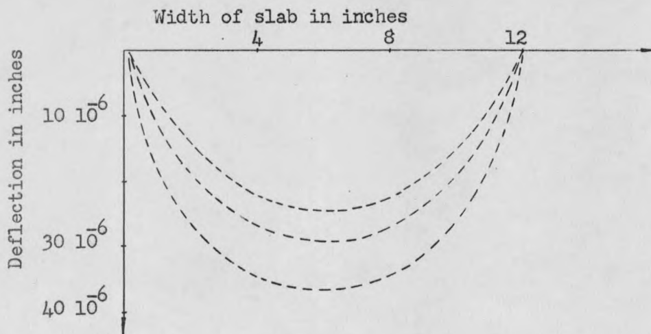
Fig. 8. Deflection diagrams along center lines JC ,ID and HE (see Fig. 1a.)
