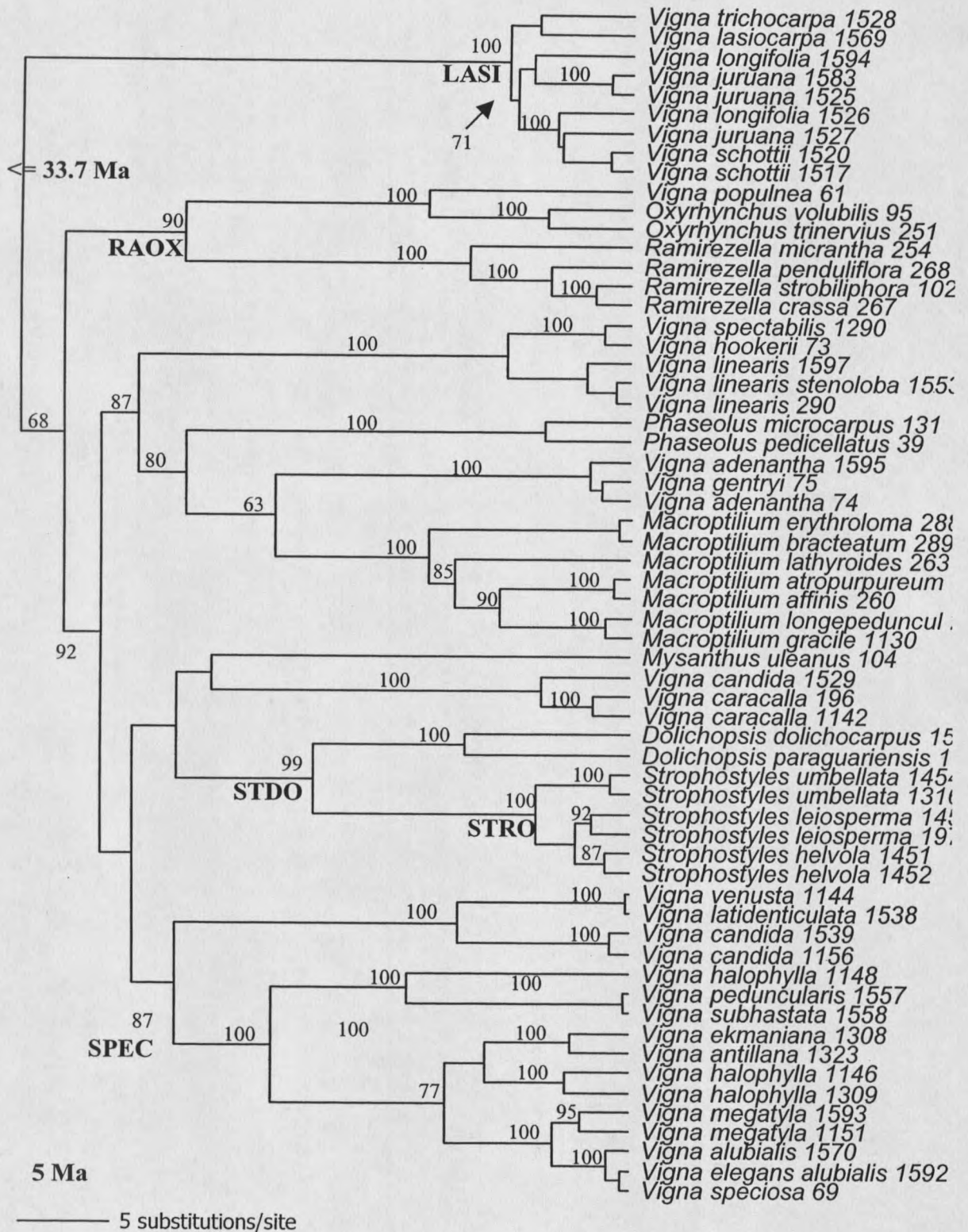
Fig. 9 Chronogram for New World Phaseolinae derived from penalized likelihood rate smoothing of a Bayesian likelihood tree, which was estimated with sequences from the ITS region.
