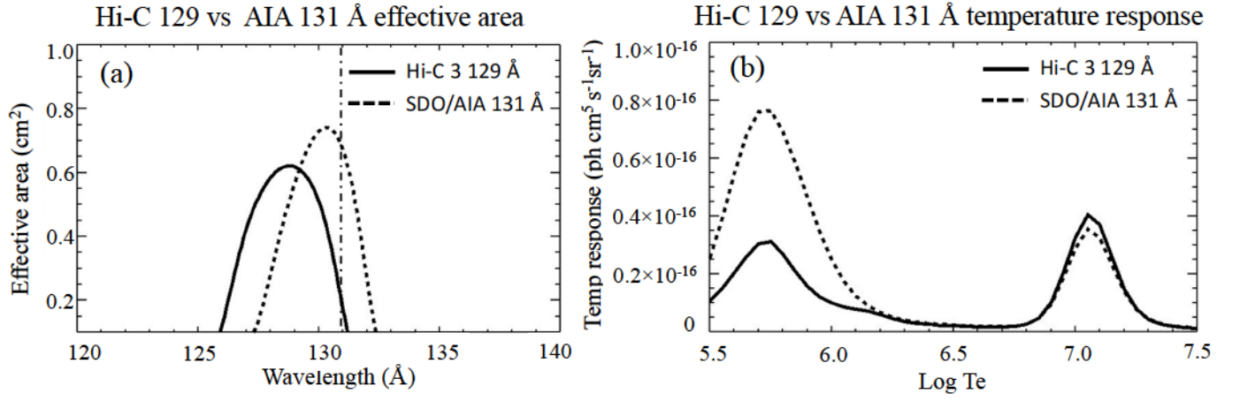
Figure 3. Comparison of Hi-C 129 and AIA 131 channel characteristics. Panel (a): the effective area of the Hi-C 3 129 Å passband (solid) and AIA 131 Å channel (dashed). A vertical dashed-dotted line marks the wavelength location of Fe VIII ( \lambda = 131 Å). Panel (b): the temperature response of Hi-C 129 Å (solid) and AIA 131 Å (dashed). At the cooler temperature peak ( \log T_e = 5.7 ), AIA is about 2.5 times more sensitive than Hi-C, whereas both are nearly equally sensitive to hotter plasma at the peak of \log T_e = 7.05 .
