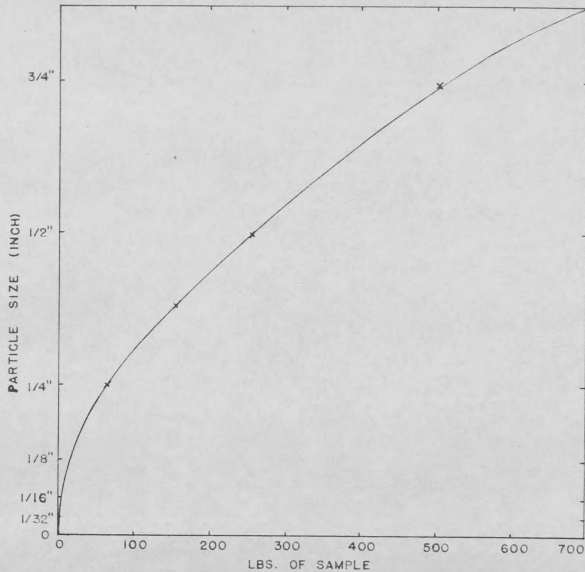
Fig. 4 Sample Size to be Used for Analysis
