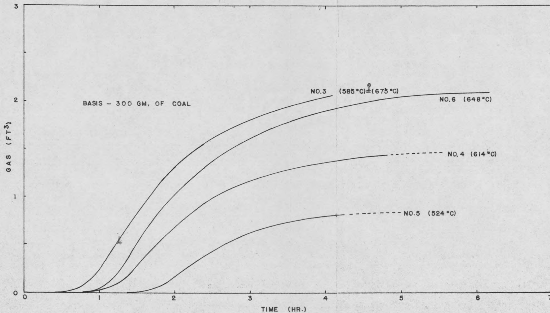
Fig. 24 Cumulative Gas Amount vs. Carbonization Time for Brophy Coal
