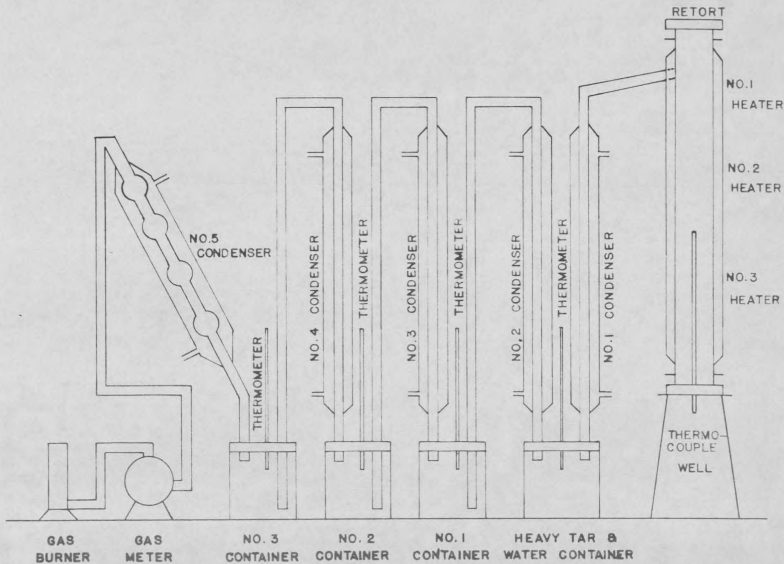
Fig. 2 Schematic Diagram of New Small Retort
