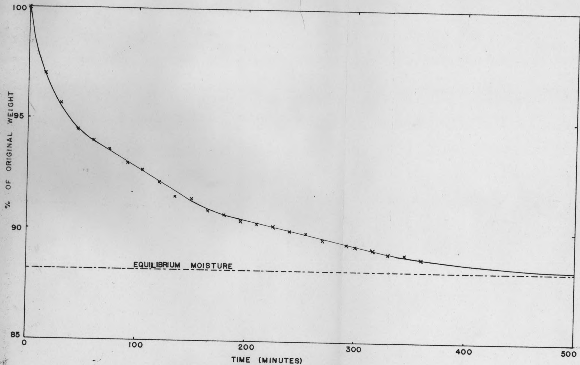
Fig. 5 Drying Test of Coal Ground by a Jaw Crusher
