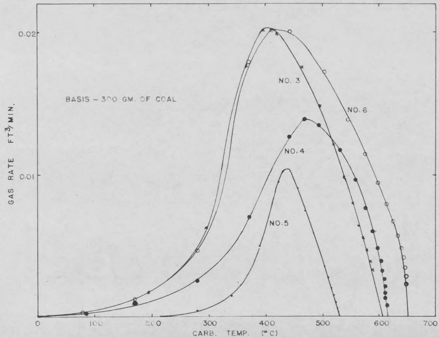
Fig. 26 Gas Rate vs. Carbonization Temperature for Brophy Coal
