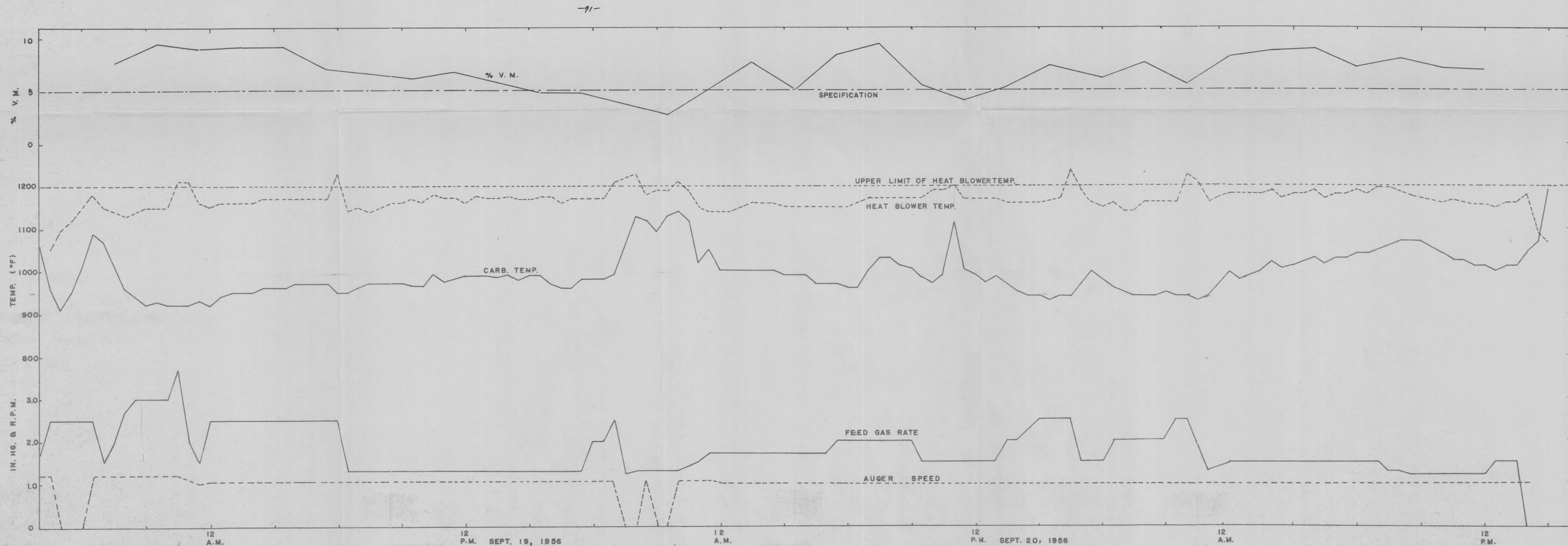
Fig. 10 Data Chart for Pilot Plant Run No. 4 (Brophy Coal)
