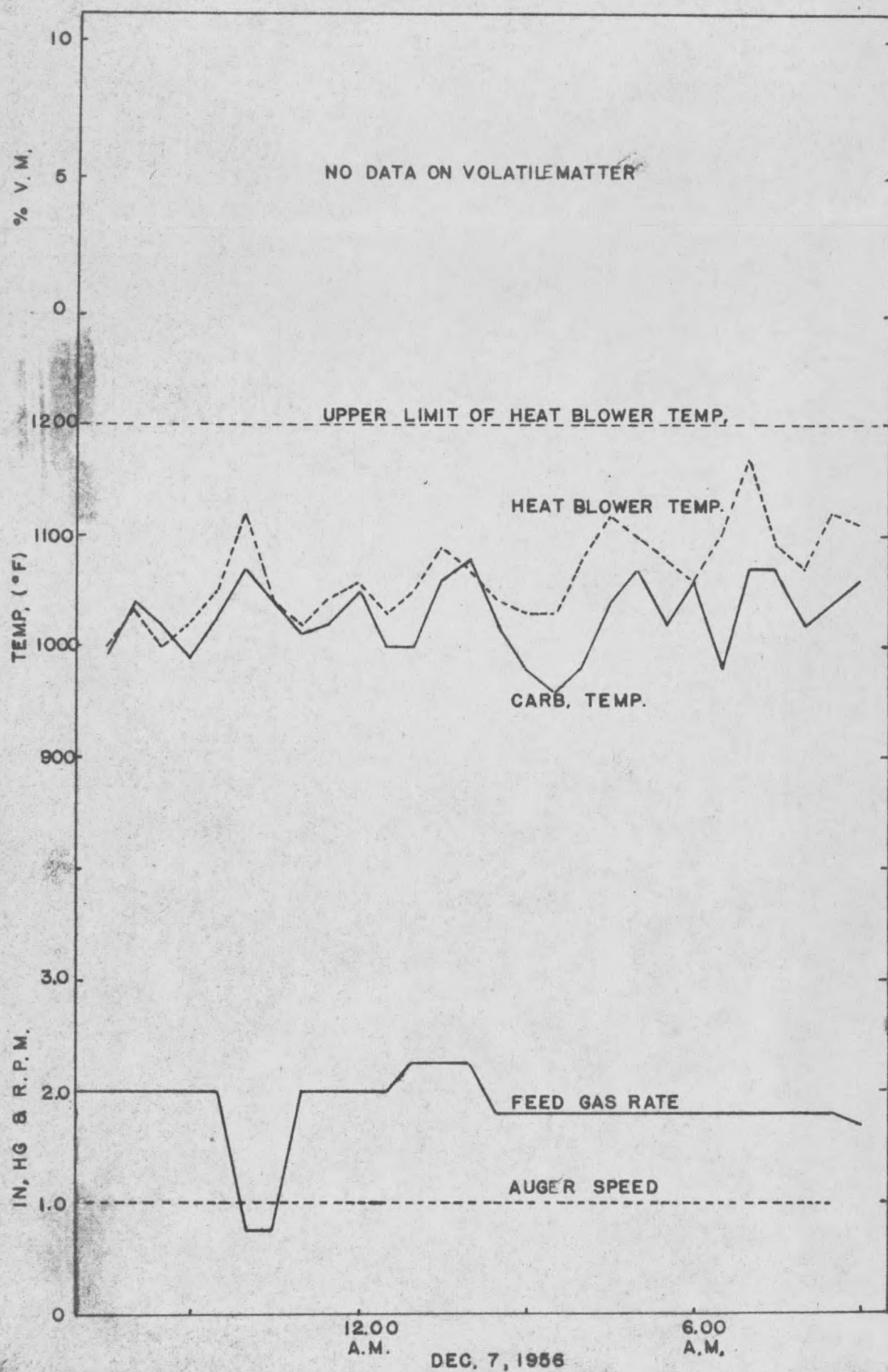
Fig. 12 Data Chart for Pilot Plant Run No. 7 (Brophy Coal)
