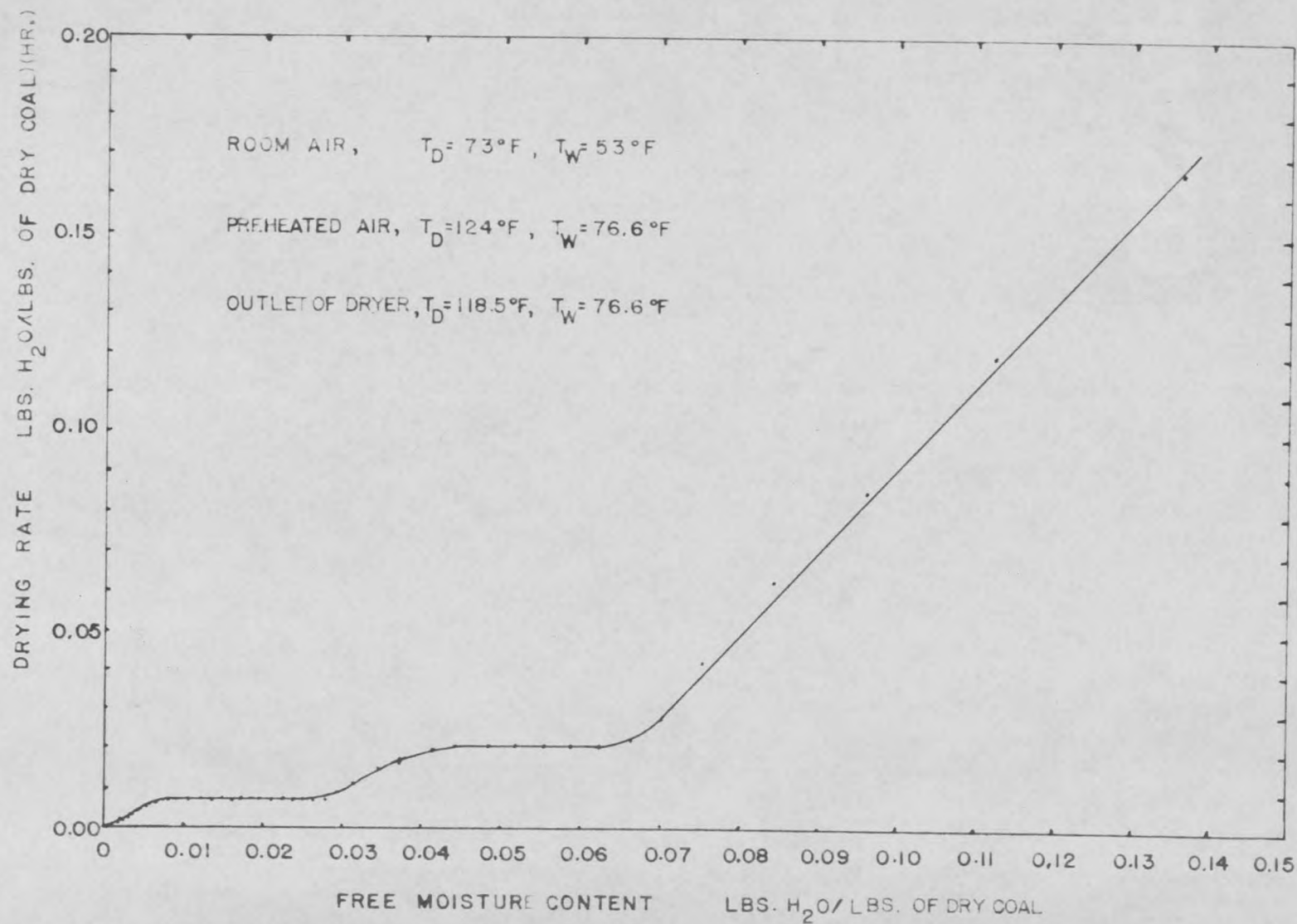
Fig. 6 Drying Rate of Brophy Regular Coal vs. Free Moisture Content
