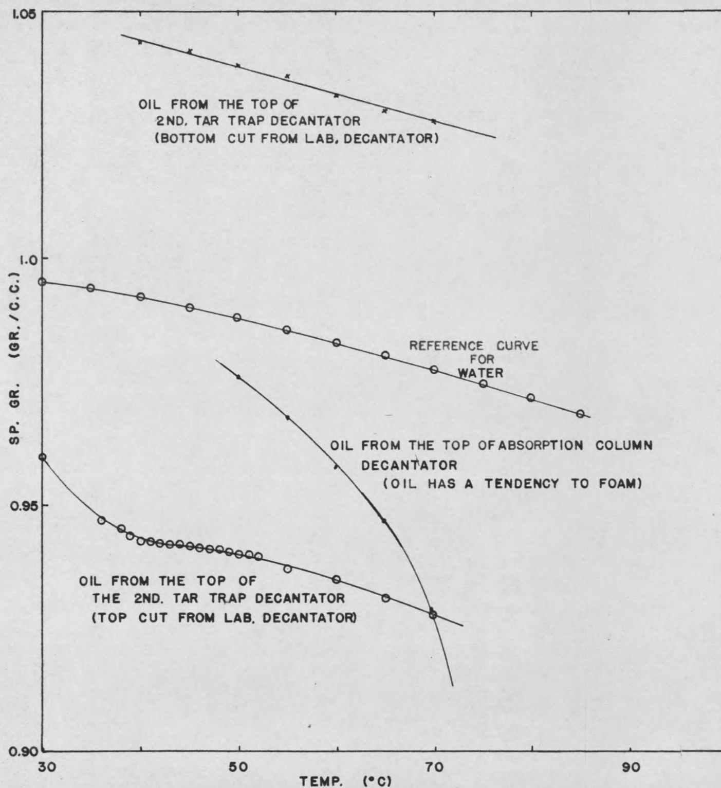
Fig. 30 Specific Gravity of Pilot Plant Coal Tar vs. Temperature
