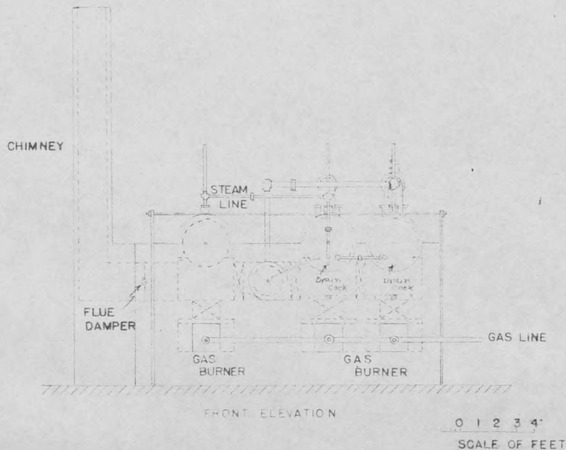
Fig. 36 Front Elevation of Crude Tar Still for Red Lodge Plant
