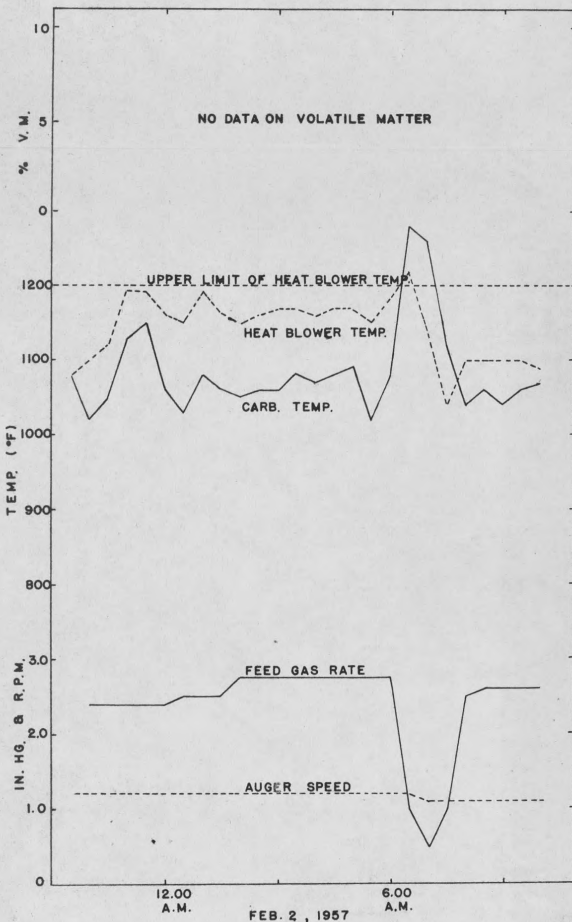
Fig. 14 Data Chart for Pilot Plant Run No. 9 (Brophy Coal)
