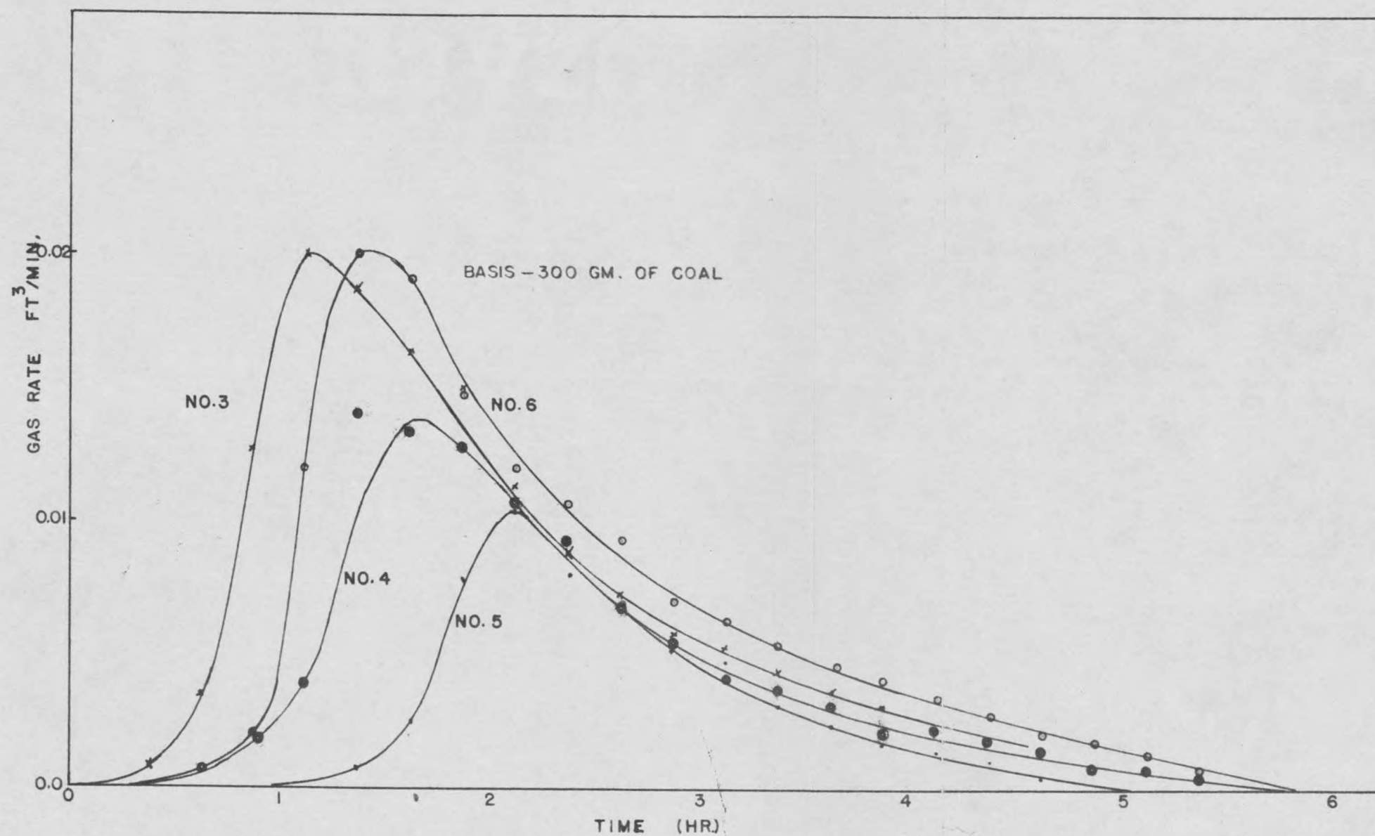
Fig. 25 Gas Rate vs. Time for Brophy Coal
