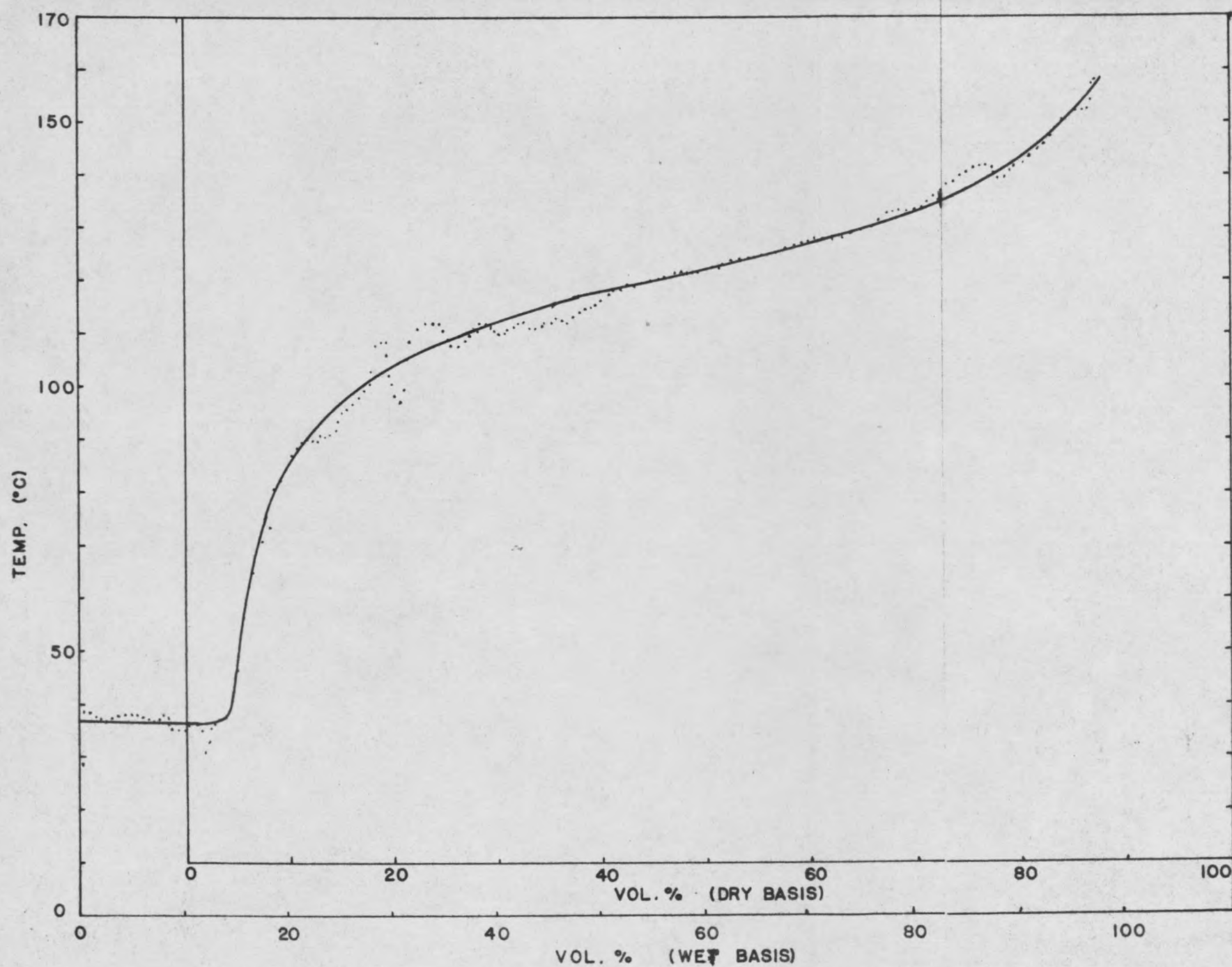
Fig. 32 Light Oil Distillation Curve (60 mmHg)
