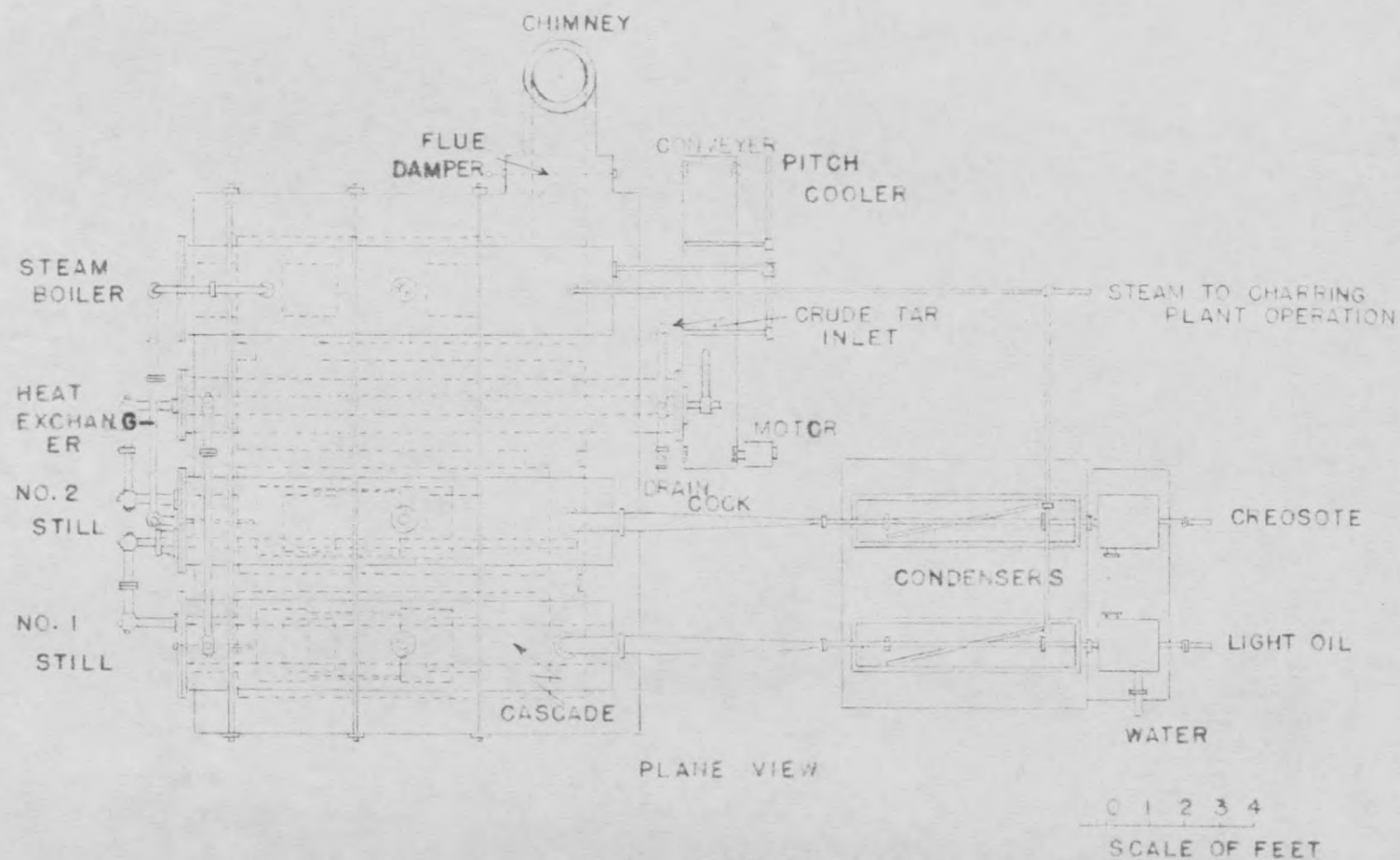
Fig. 35 Plane View of Crude Tar Still for Red Lodge Plant
