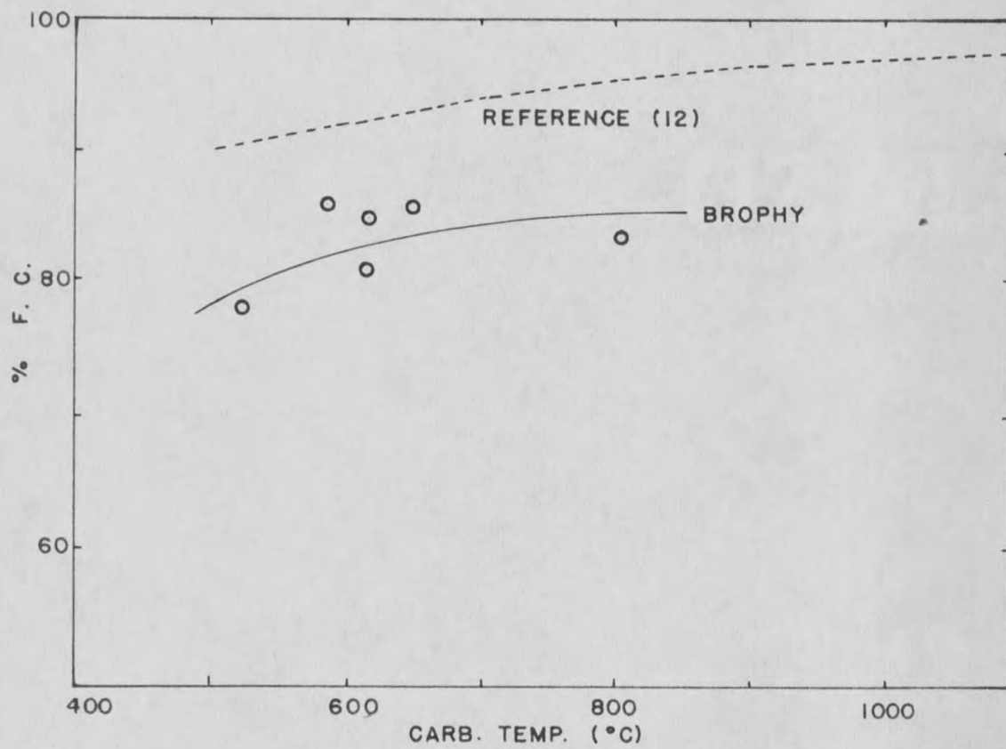
Fig. 19 Fixed Carbon Content in Coke vs. Carbonization Temperature
