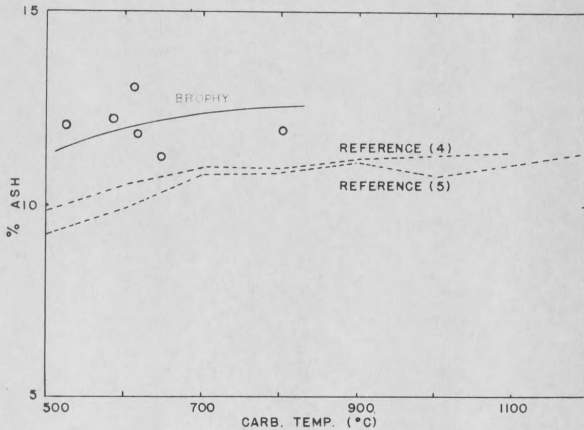
Fig. 20 Ash Content in Coke vs. Carbonization Temperature
