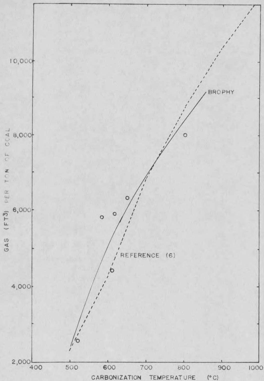
Fig. 22 Gas Amount vs. Carbonization Temperature
