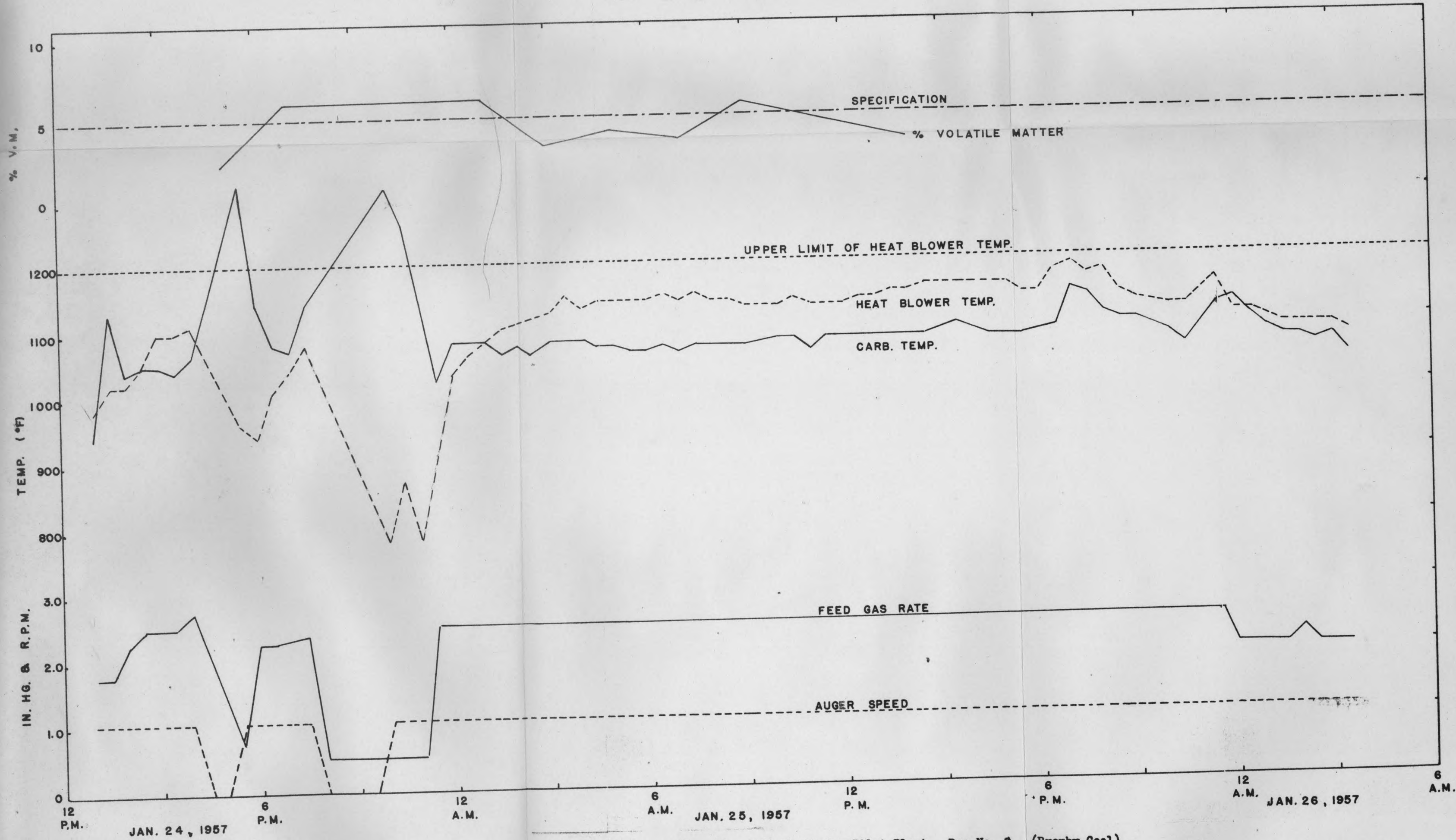
Fig. 13 Data Chart for Pilot Plant Run No. 8 (Brophy Coal)
