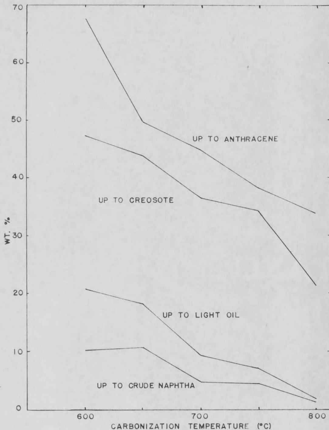
Fig. 29 Cumulative Weight Percentages of Each Fraction in Coal Tar
