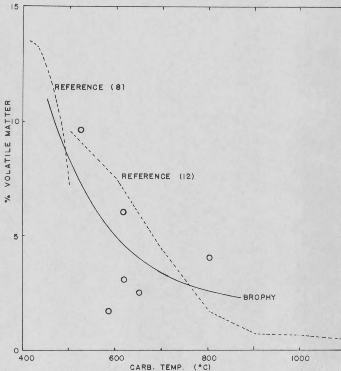
Fig. 18 Volatile Matter Content in Coke vs. Carbonization Temperature
