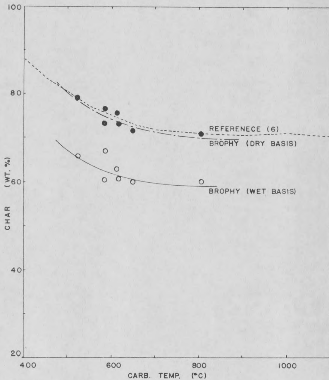
Fig. 17 Coke Percentage vs. Carbonization Temperature
