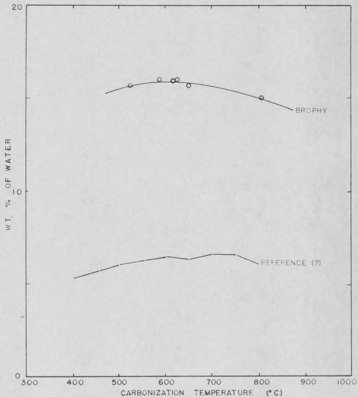
Fig. 21 Wt. % of Aqueous Distillate vs. Carbonization Temperature
