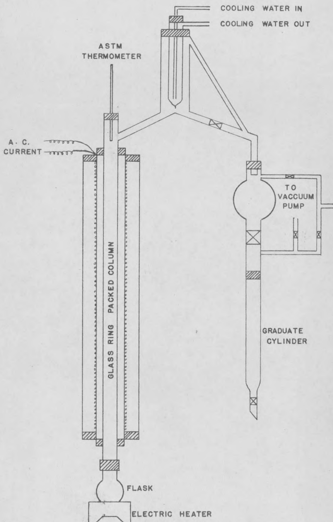
Fig. 31 Fractional Distillation Apparatus
