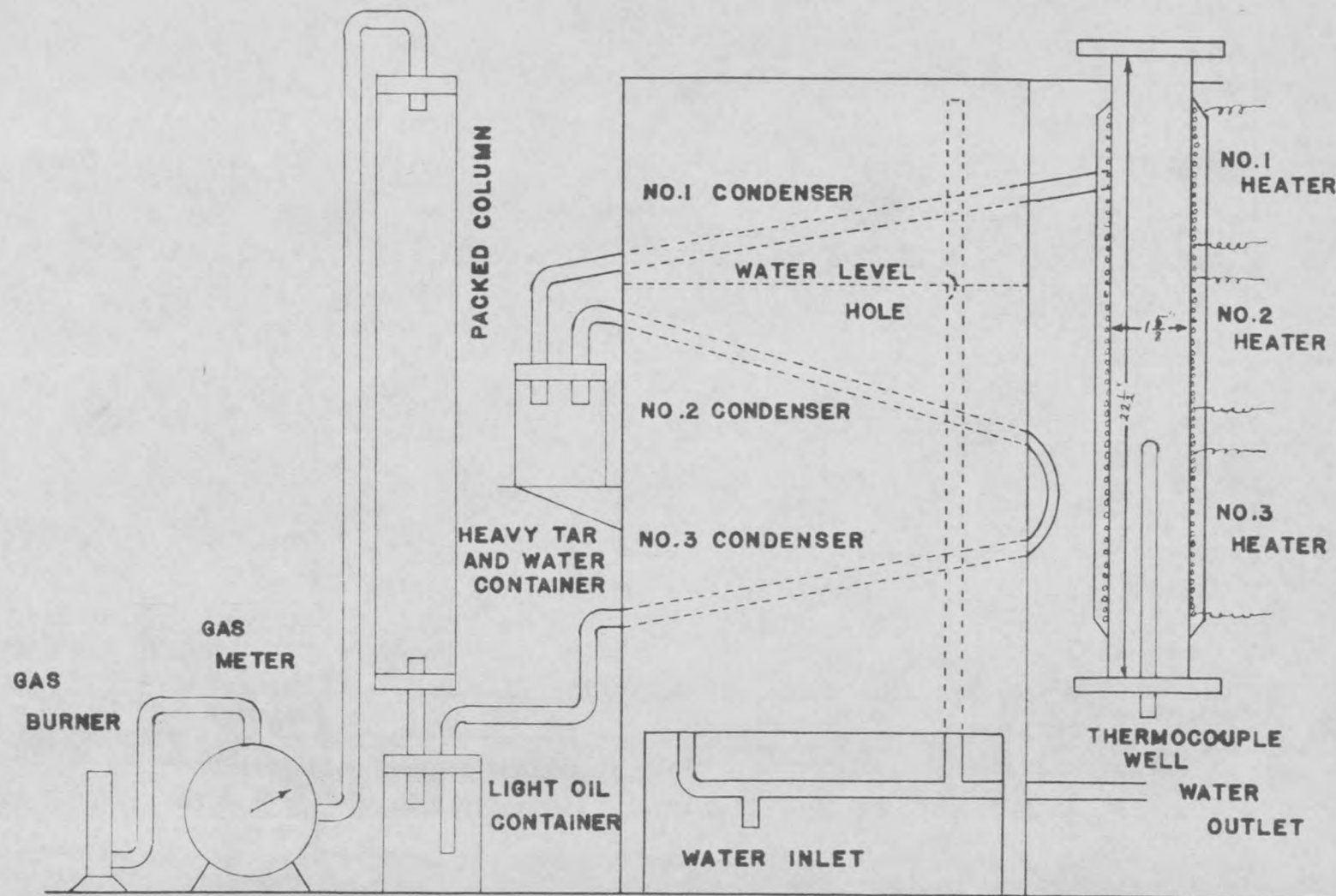
Fig. 1 Schematic Diagram of Old Small Retort
