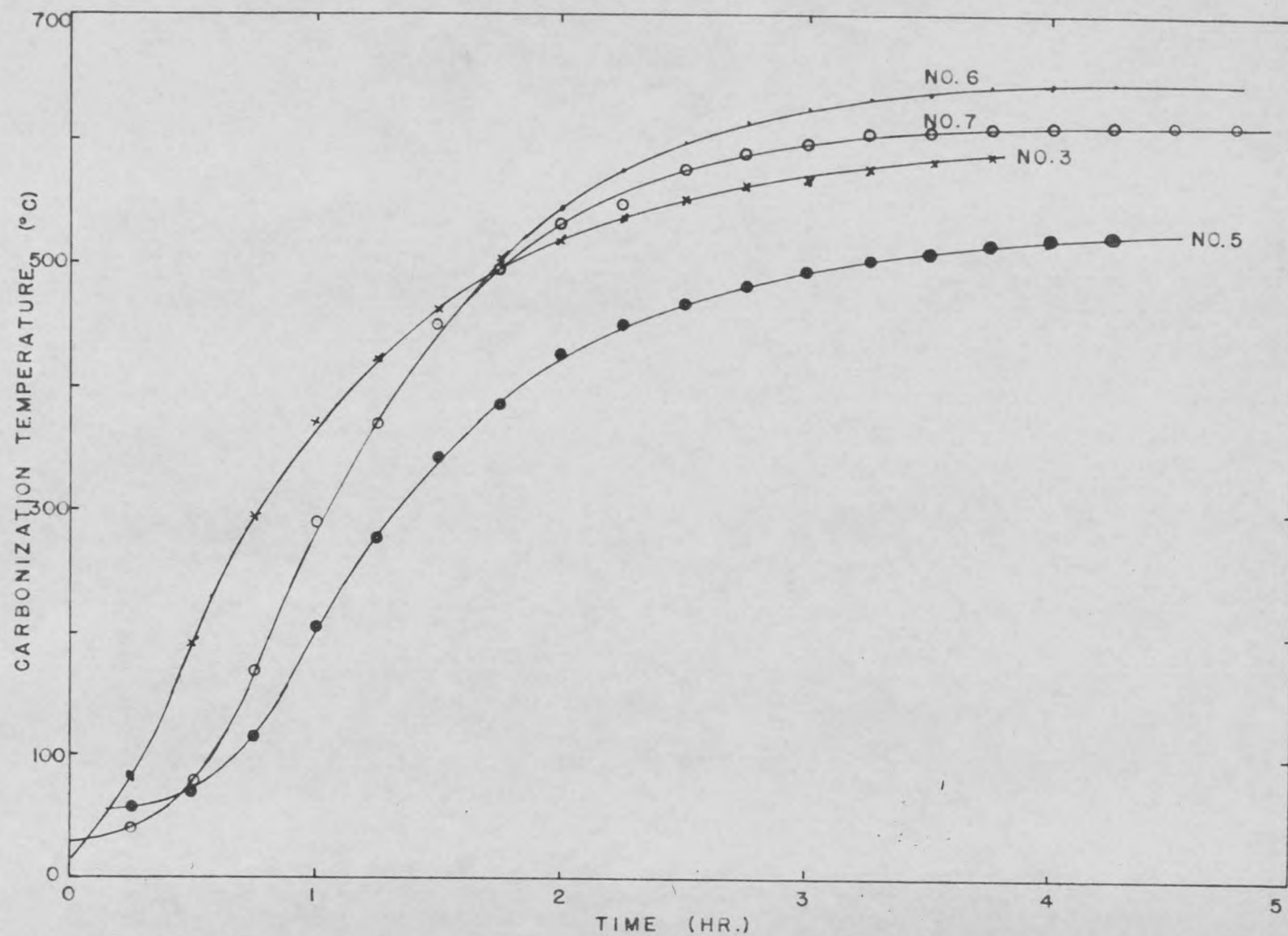
Fig. 27 Carbonization Temperature vs. Time for Brophy Coal
