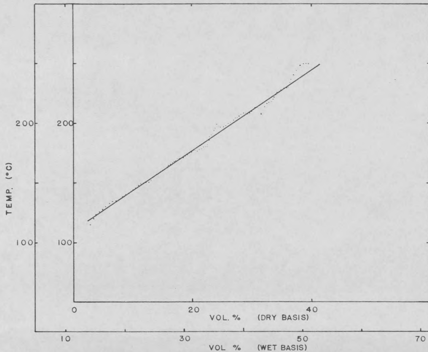
Fig. 33 Tar Distillation Curve (60 mmHg)
