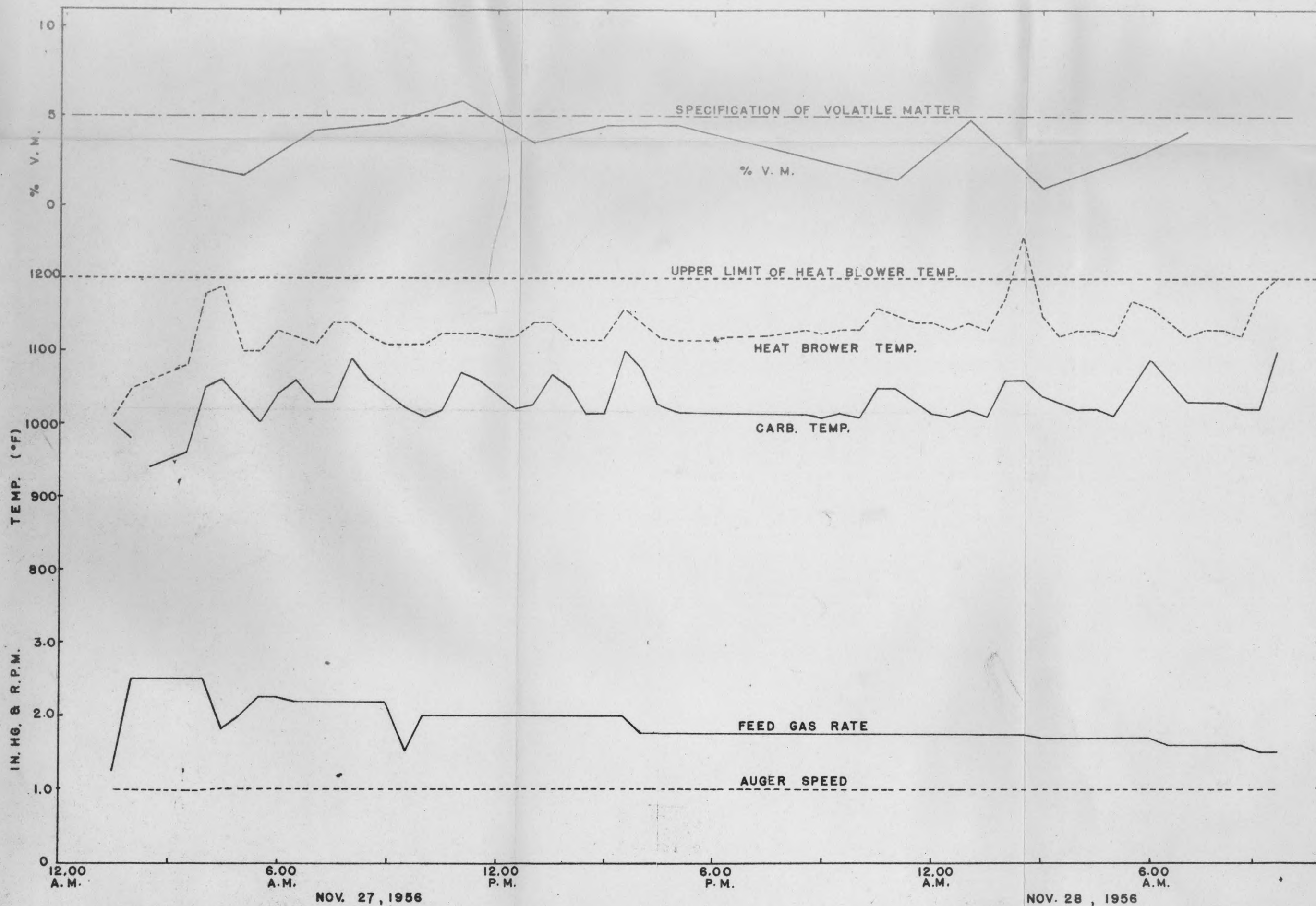
Fig. 11 Data Chart for Pilot Plant Run No. 6 (Brophy Coal)
