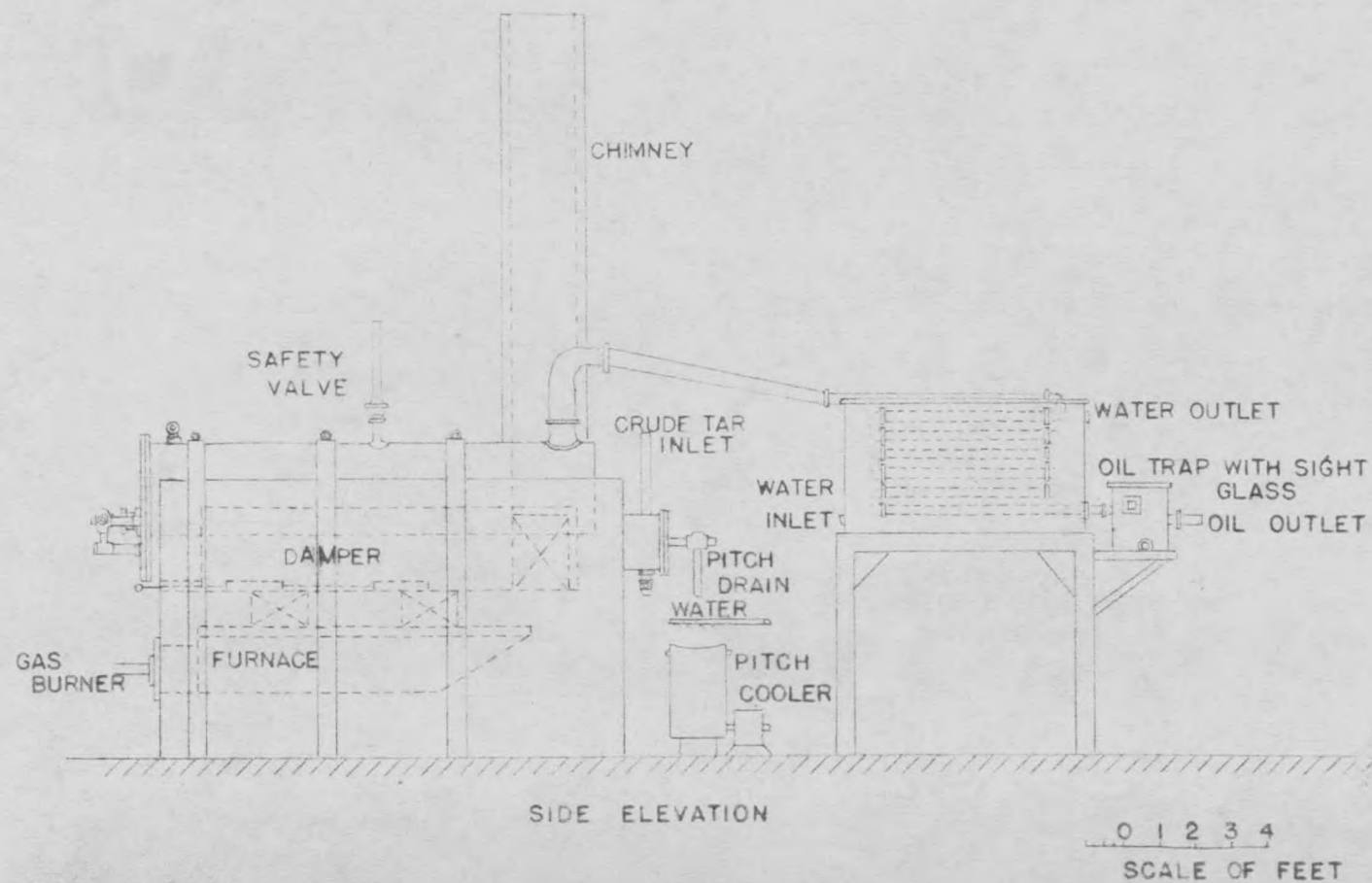
Fig. 34 Side Elevation of Crude Tar Still for Red Lodge Plant
