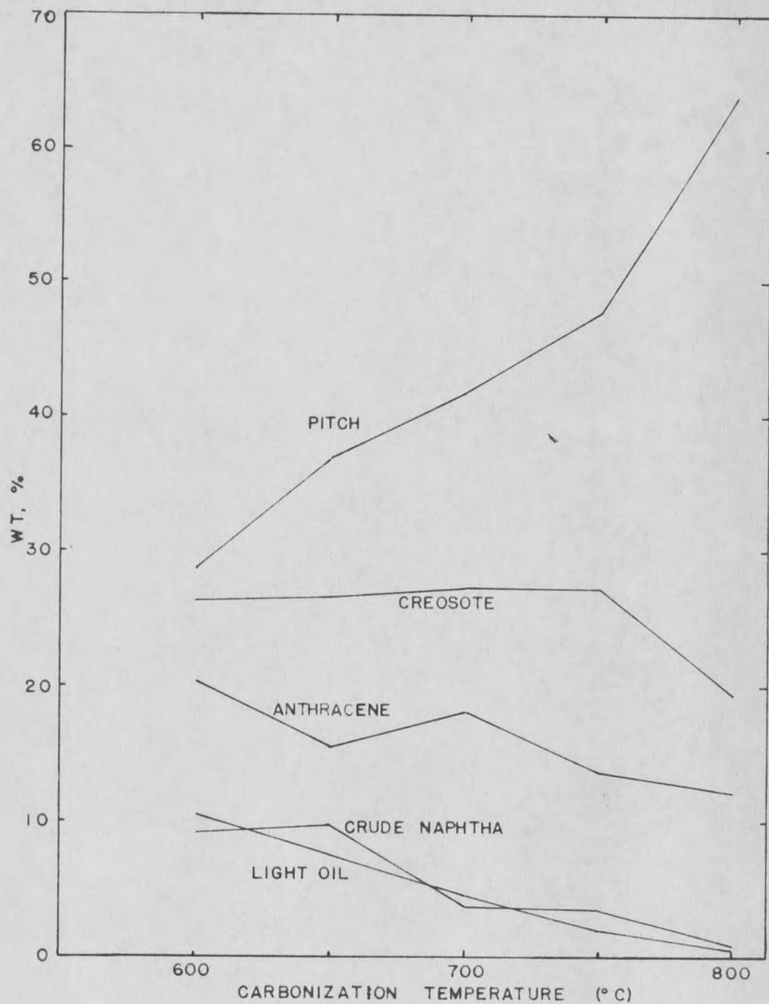
Fig. 28 Effect of Carbonization Temperature on Composition of Coal Tar
