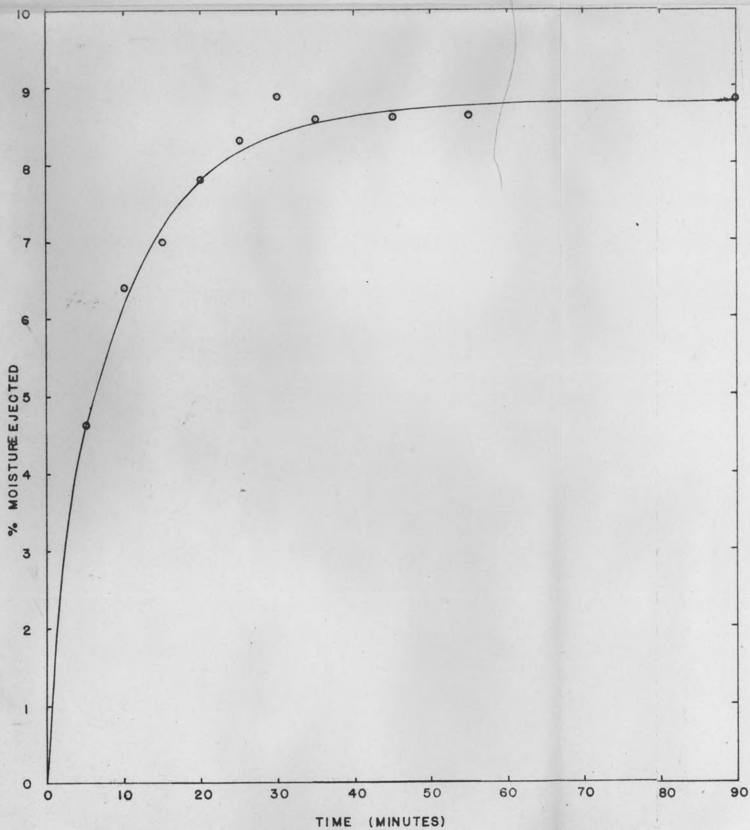
Fig. 7 Determination of Required Period for Moisture Analysis
