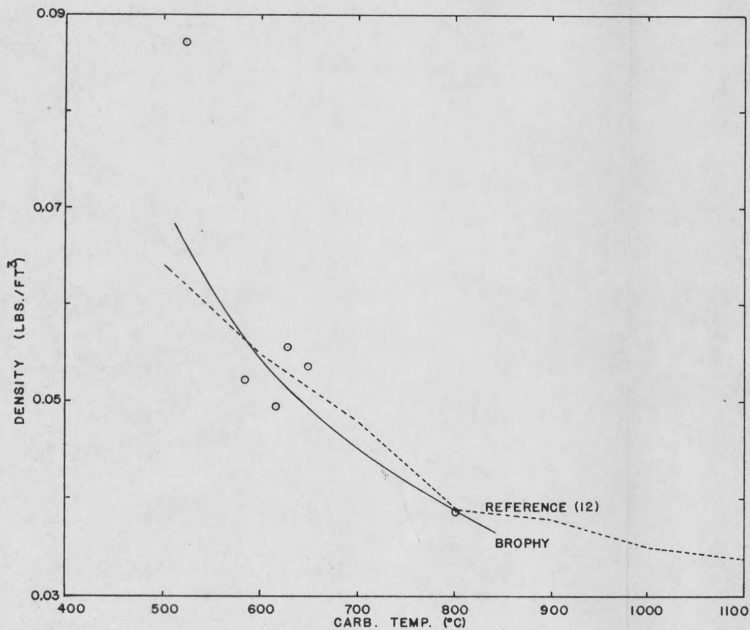
Fig. 23 Approximate Density of Coal Gas vs. Carbonization Temperature
