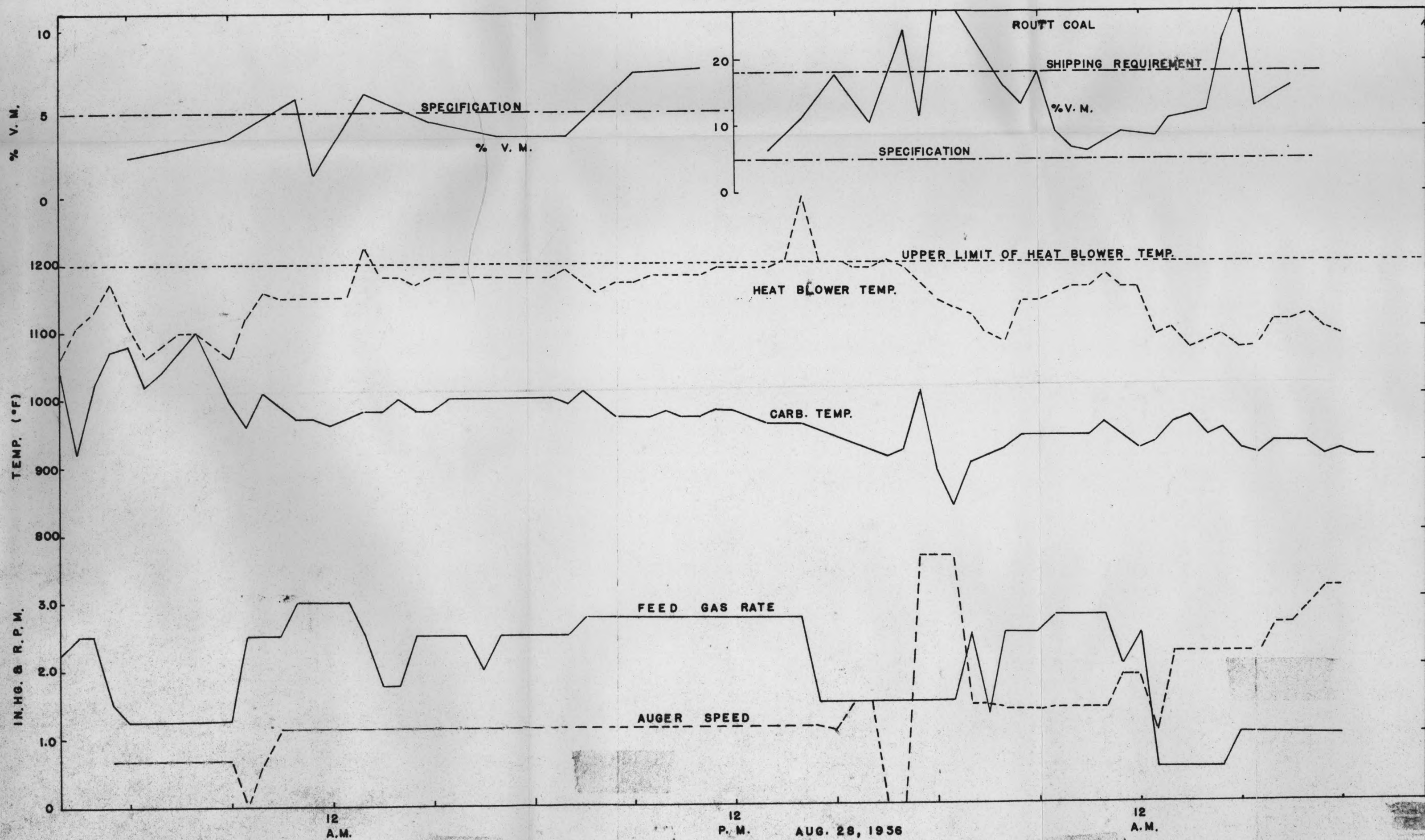
Fig. 9 Data Chart for Pilot Plant Run No. 3
