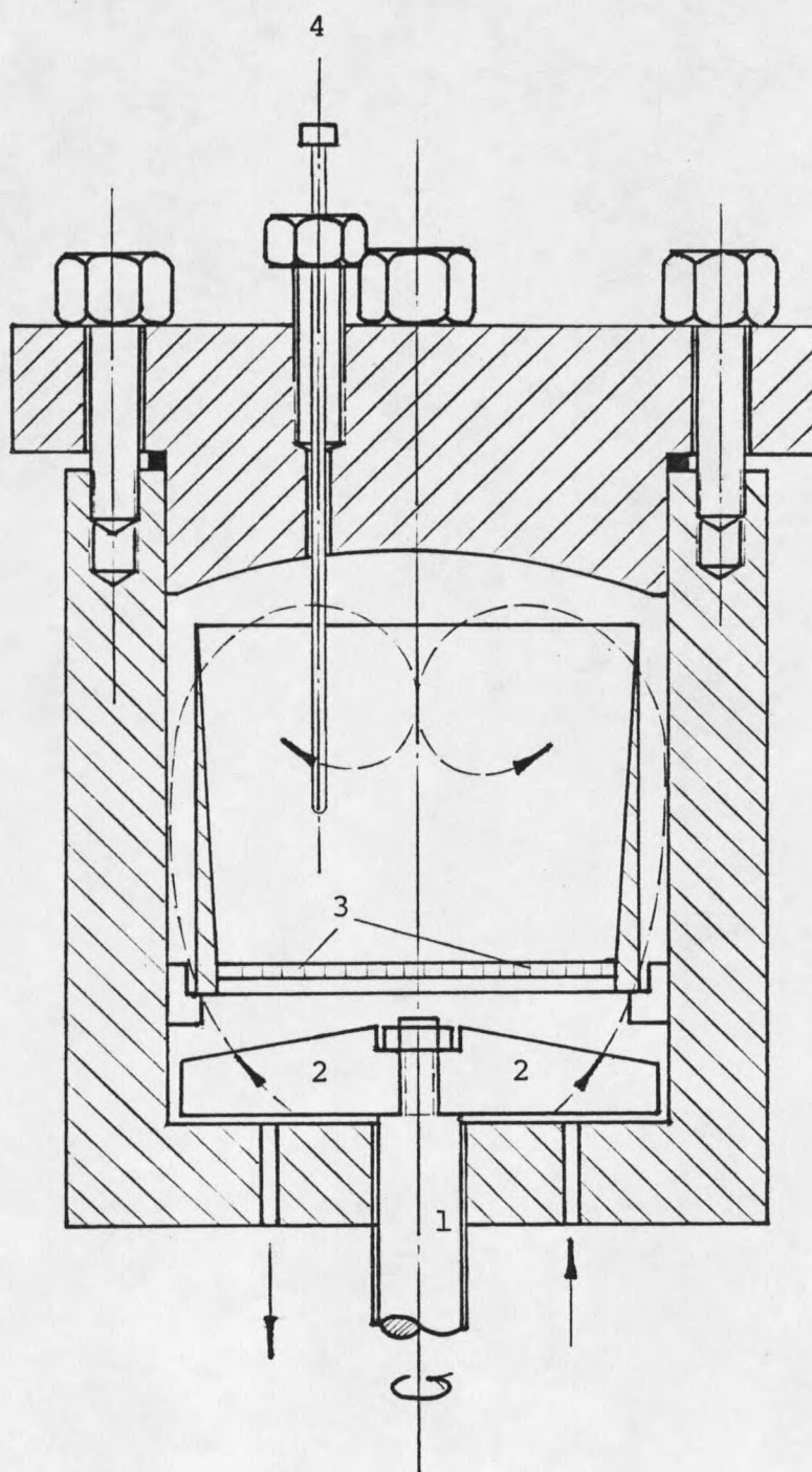
Figure 11. Schematic diagram of Berté reactor. 1. magnetic drive. 2. impeller. 3. catalyst bed. 4. thermocouple.
