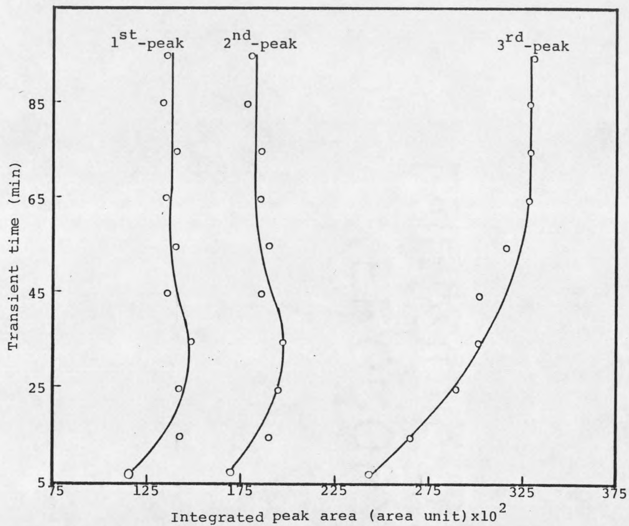
Figure 34. Experimental data for sample A-26 in p-cymene cracking reaction at 315°C.
