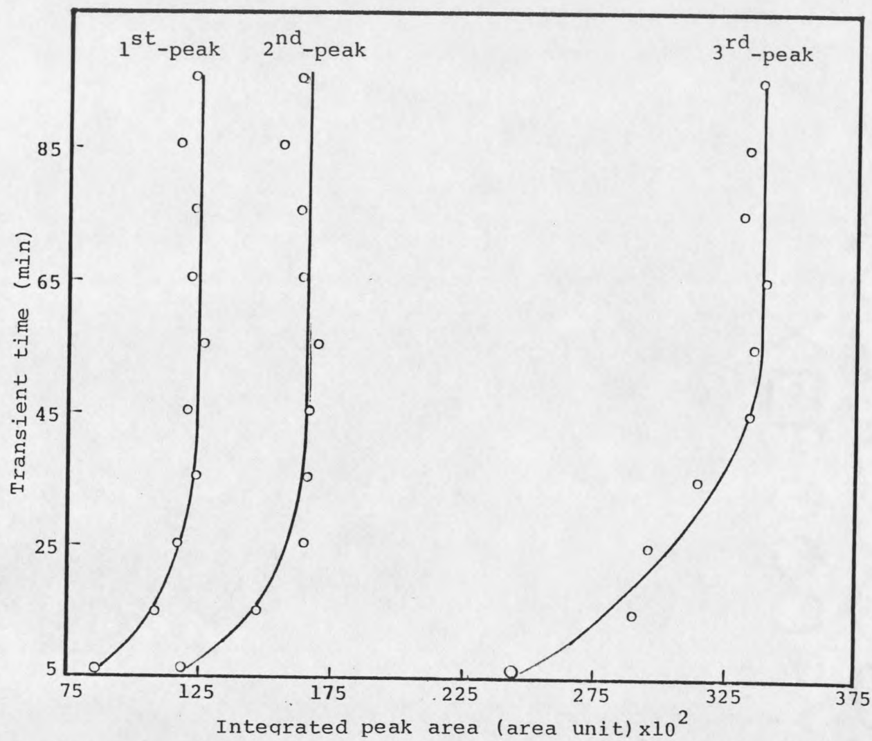
Figure 35. Experimental data for sample A-44 in p-cymene cracking reaction at 315°C
