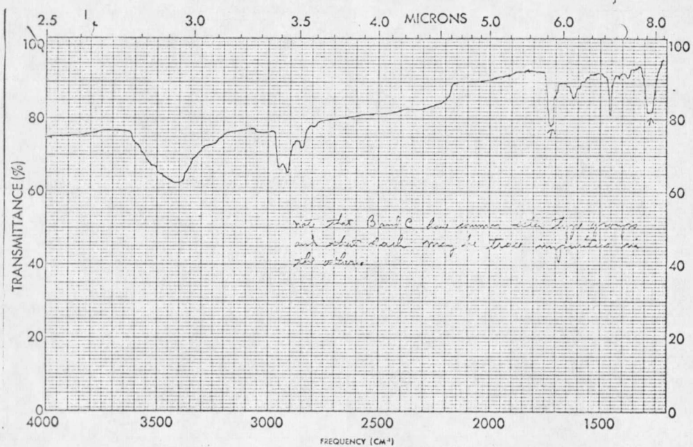
Figure 13. Infrared Spectrum of Compound IV.
