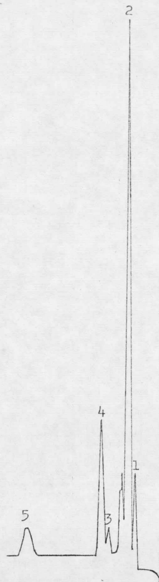
Figure 7. Chromatogram of Gaseous Products.
