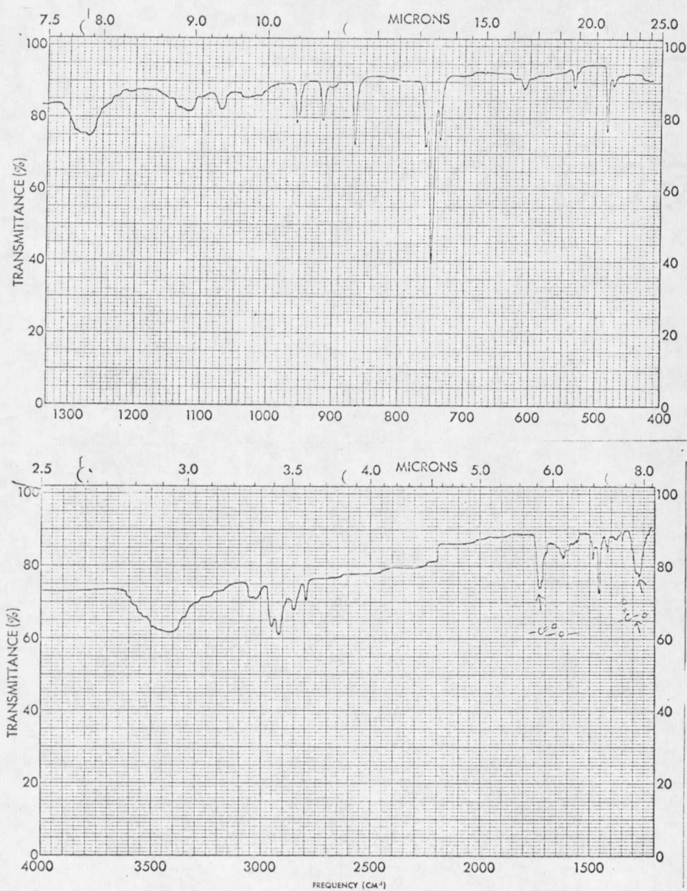
Figure 12. Infrared Spectrum of Compound III.
