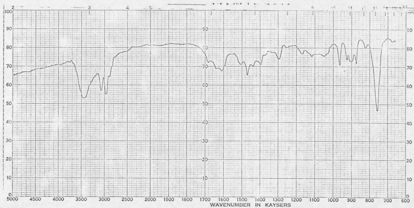
Figure 10. Infrared Spectrum of Compound I.
