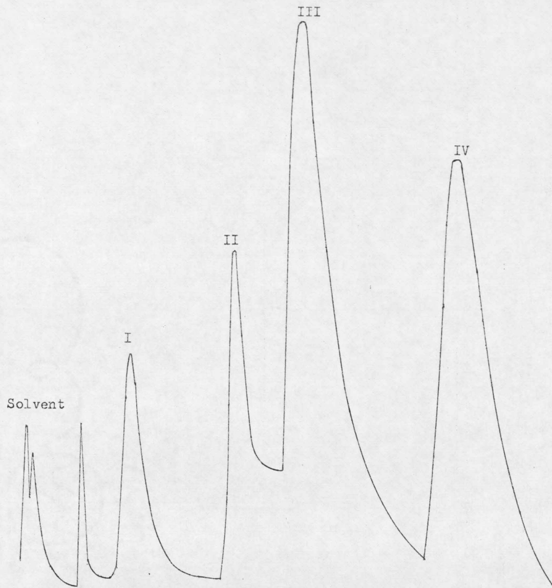
Figure 8. Condensate Chromatogram.
