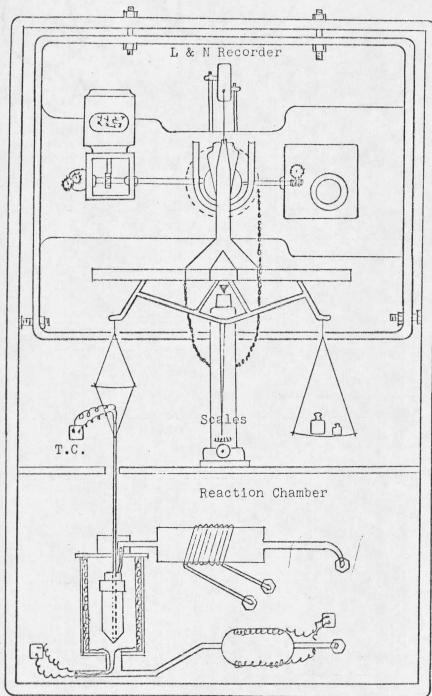
Figure 1. Thermogravimetric Analysis Apparatus
