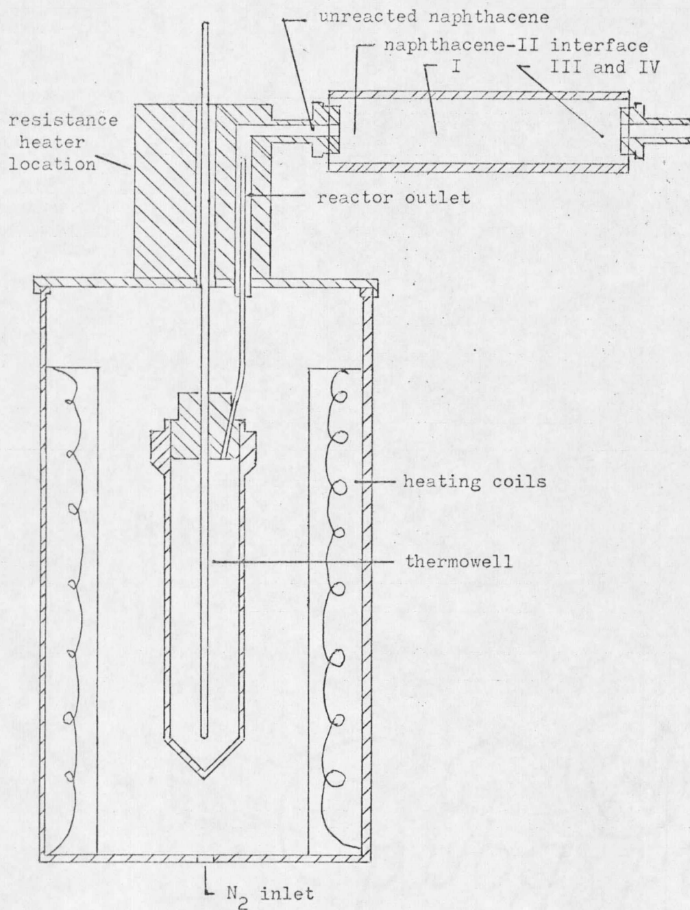
Figure 2. Equipment Modifications and Product Locations
