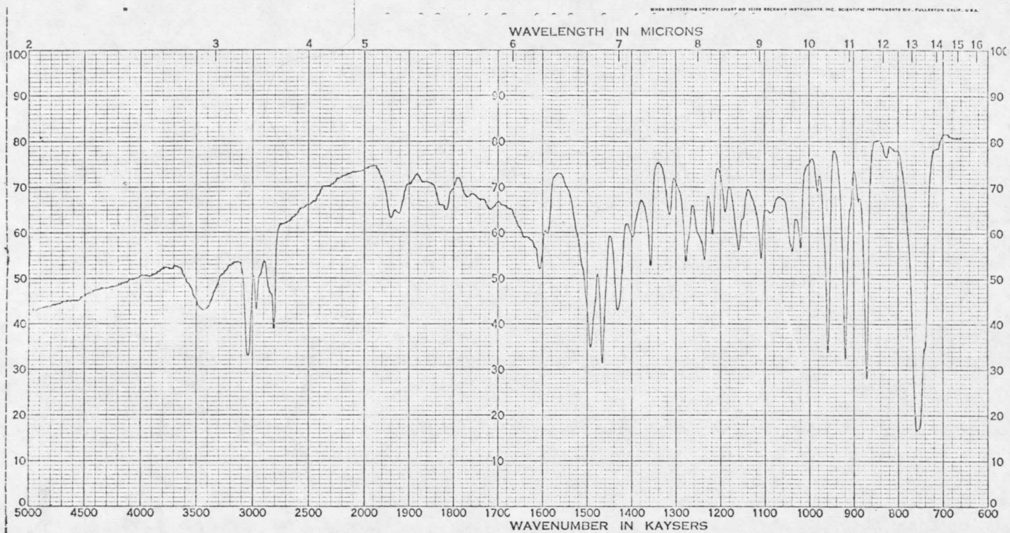
Figure 9. Infrared Spectrum of Compound II.
