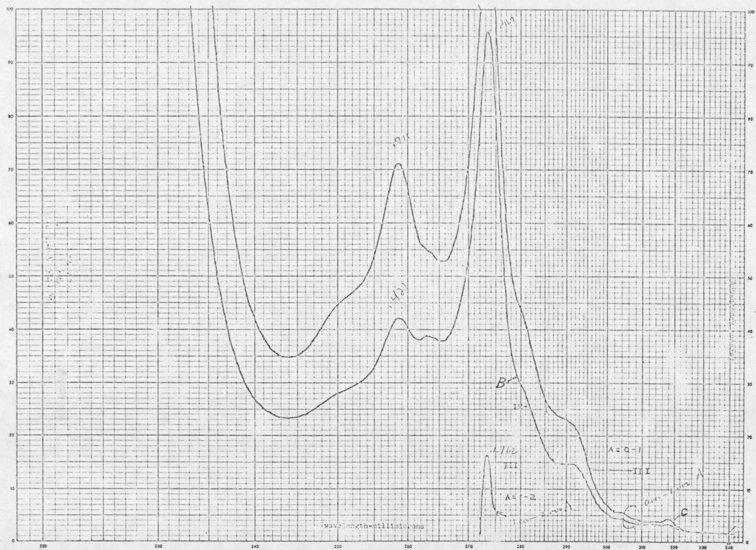
Figure 14. Ultraviolet Spectra of Compounds III and IV in Ethanol.
