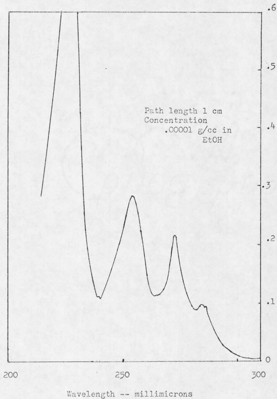
Figure 11. Ultraviolet Spectrum of Compound I.
