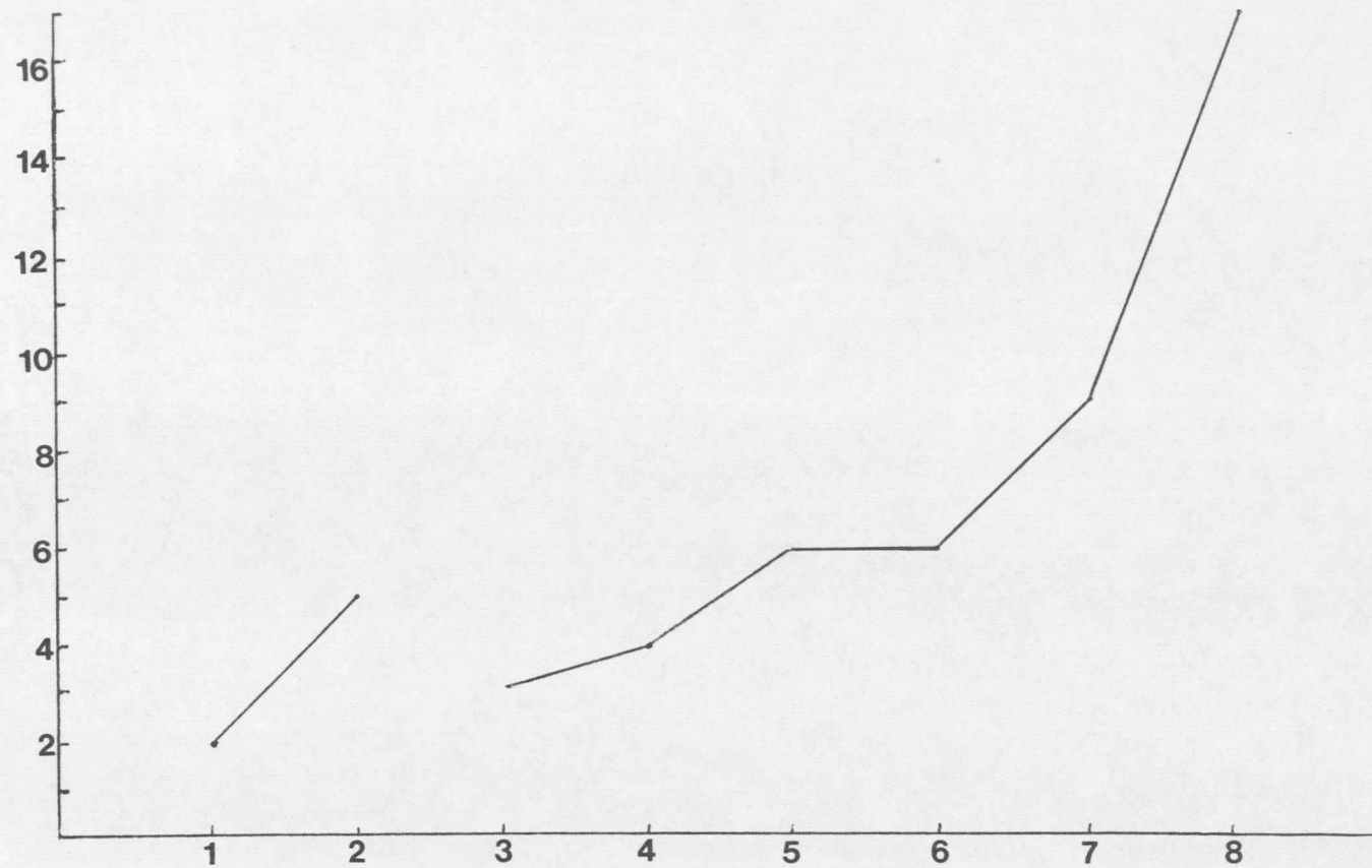
Figure 7. Number of fish species collected in the eight study sections of Sarpy Creek during 1975 - 1976.
