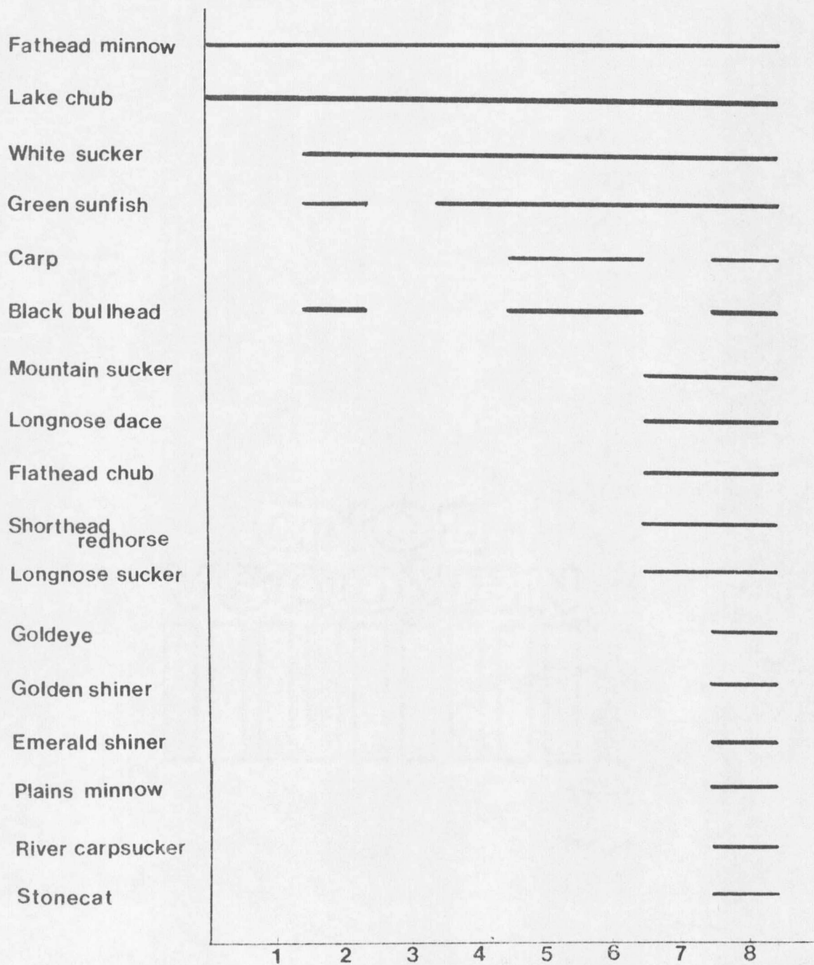
Figure 6. Distribution of fish species in the eight study sections of Sarpy Creek.
