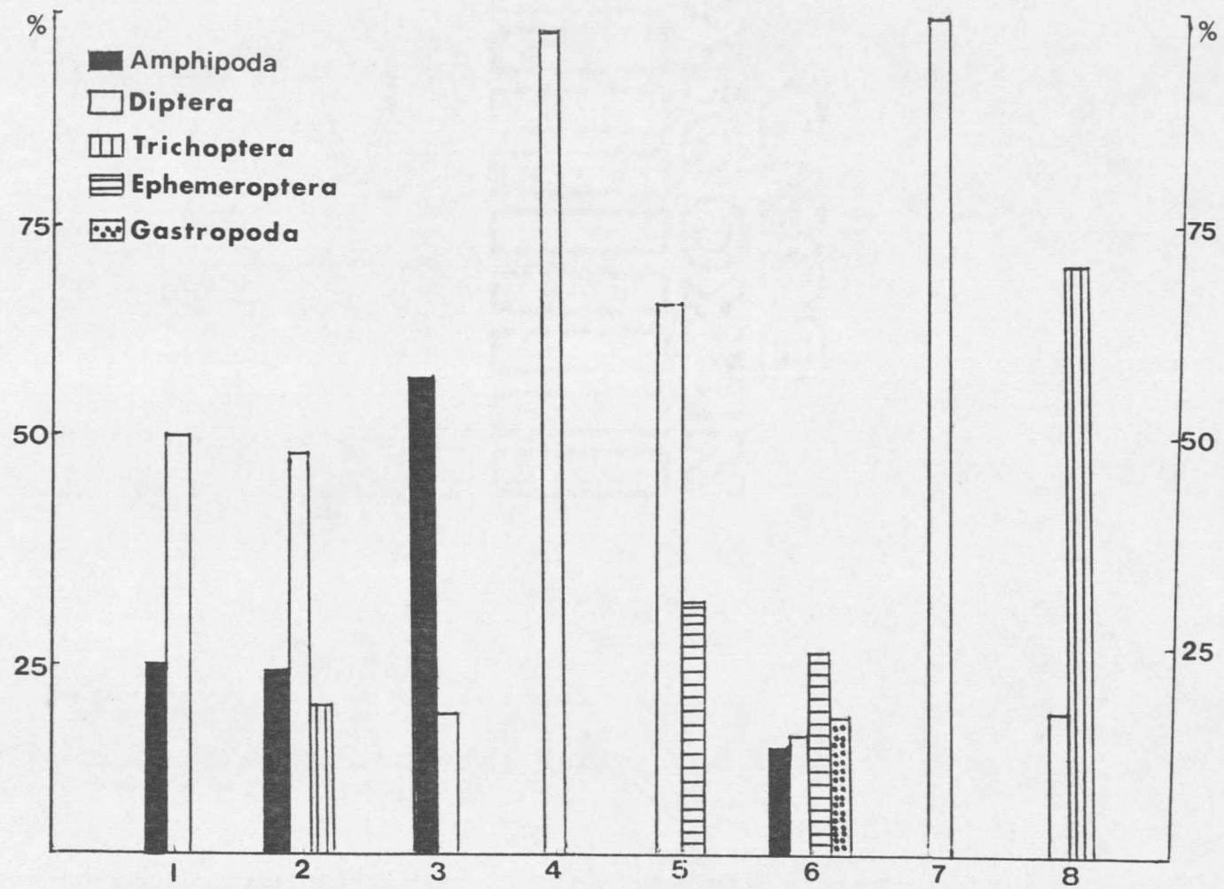
Figure 3. Relative abundance of dominant invertebrates as collected on basket samplers.
