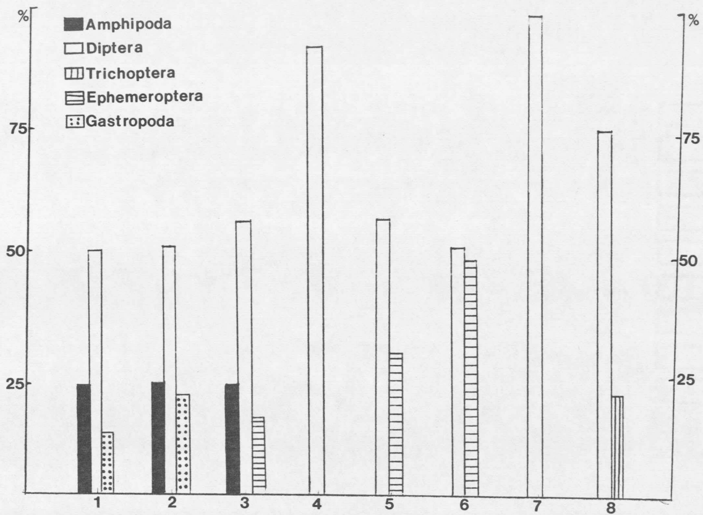
Figure 5. Relative abundance of dominant invertebrates collected on basket samplers from March 28 - May 14, 1976.
