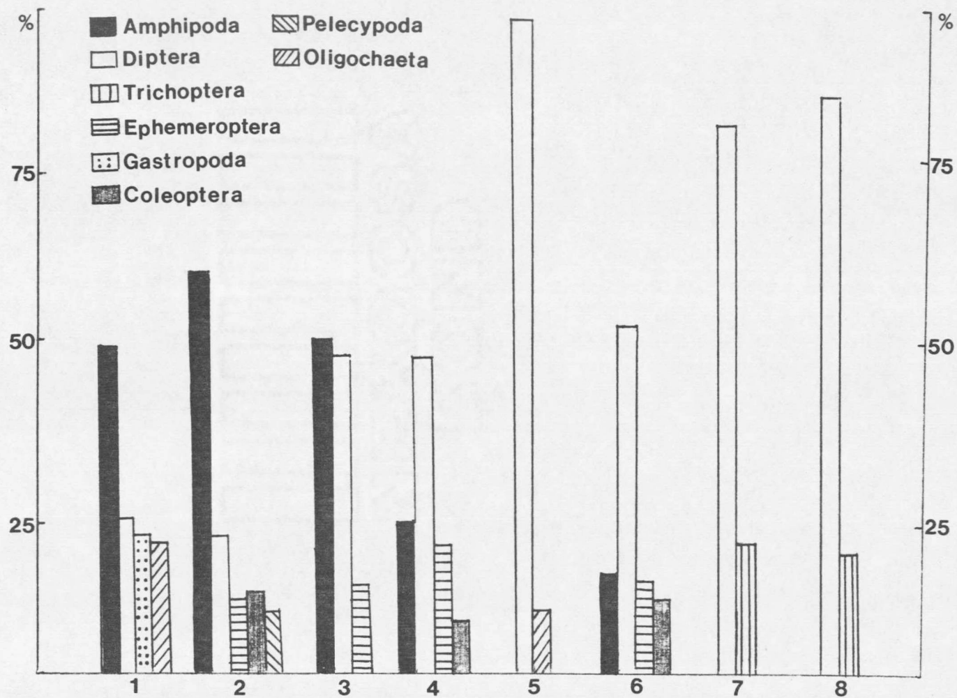
Figure 4. Relative abundance of dominant invertebrates collected in substrate samplers.
