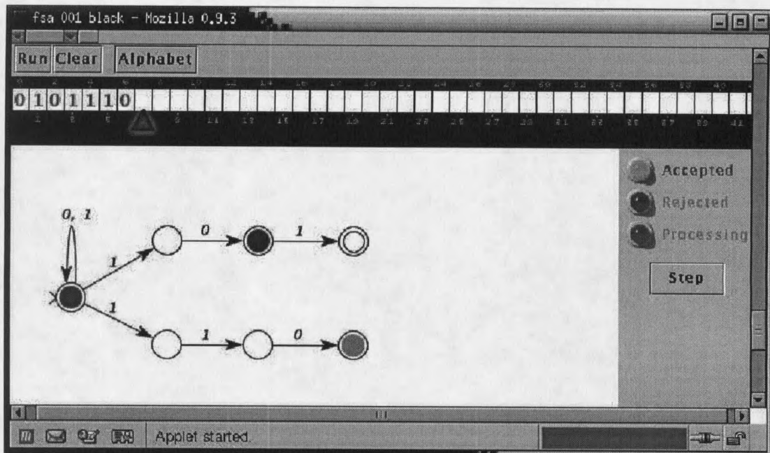
Figure 4.3: A nondeterministic FSA in Version 2 of the FSA Simulator
