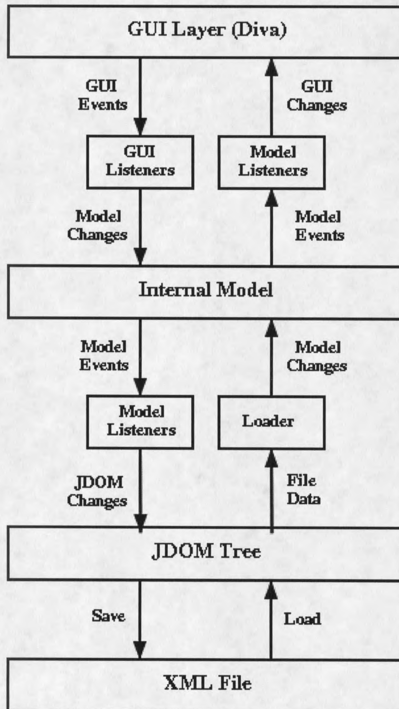
Figure 4.2: The Architecture of Version 2.
