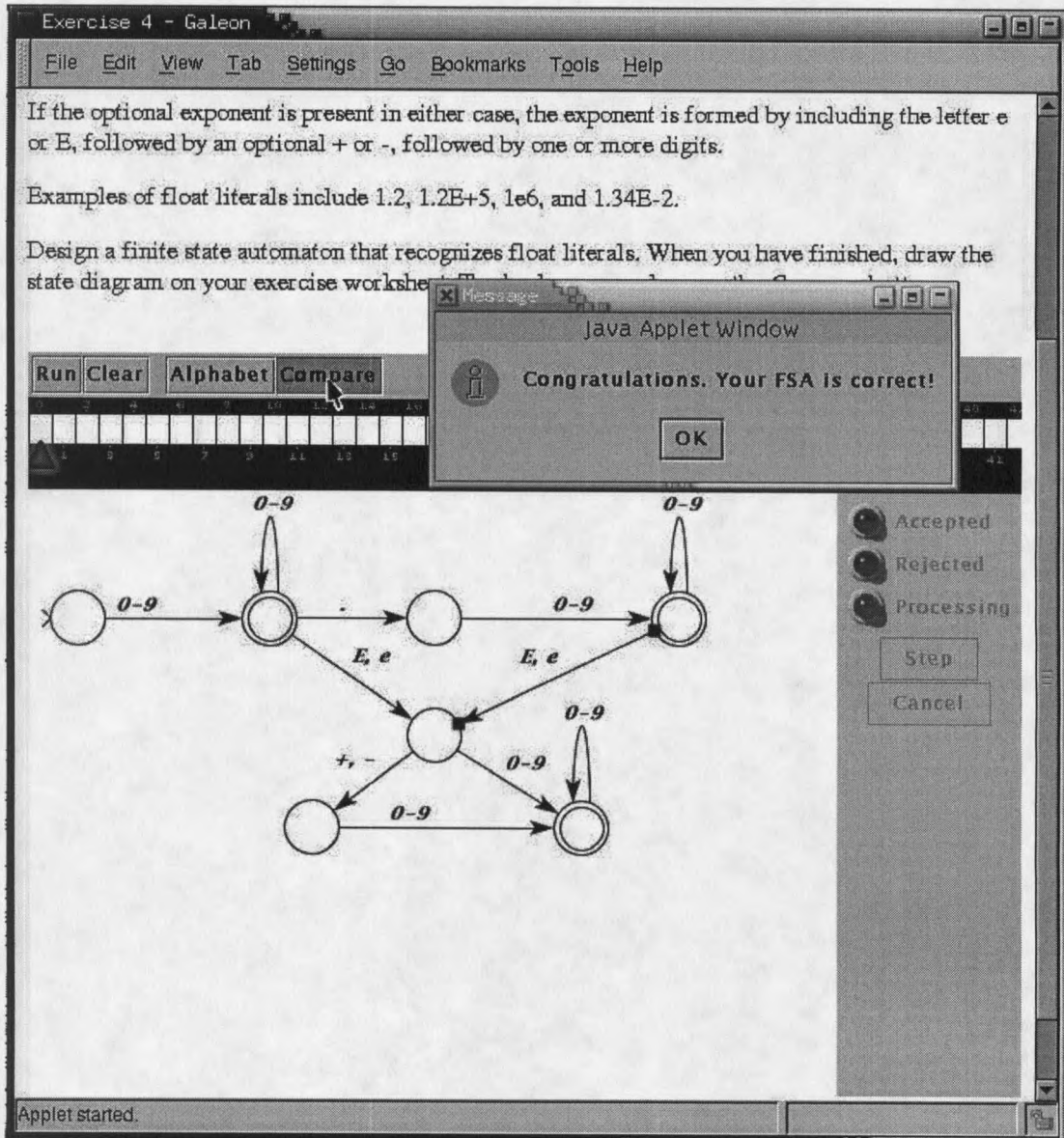
Figure 3.12: FSA comparison message when the student's FSA correctly recognizes the target language
