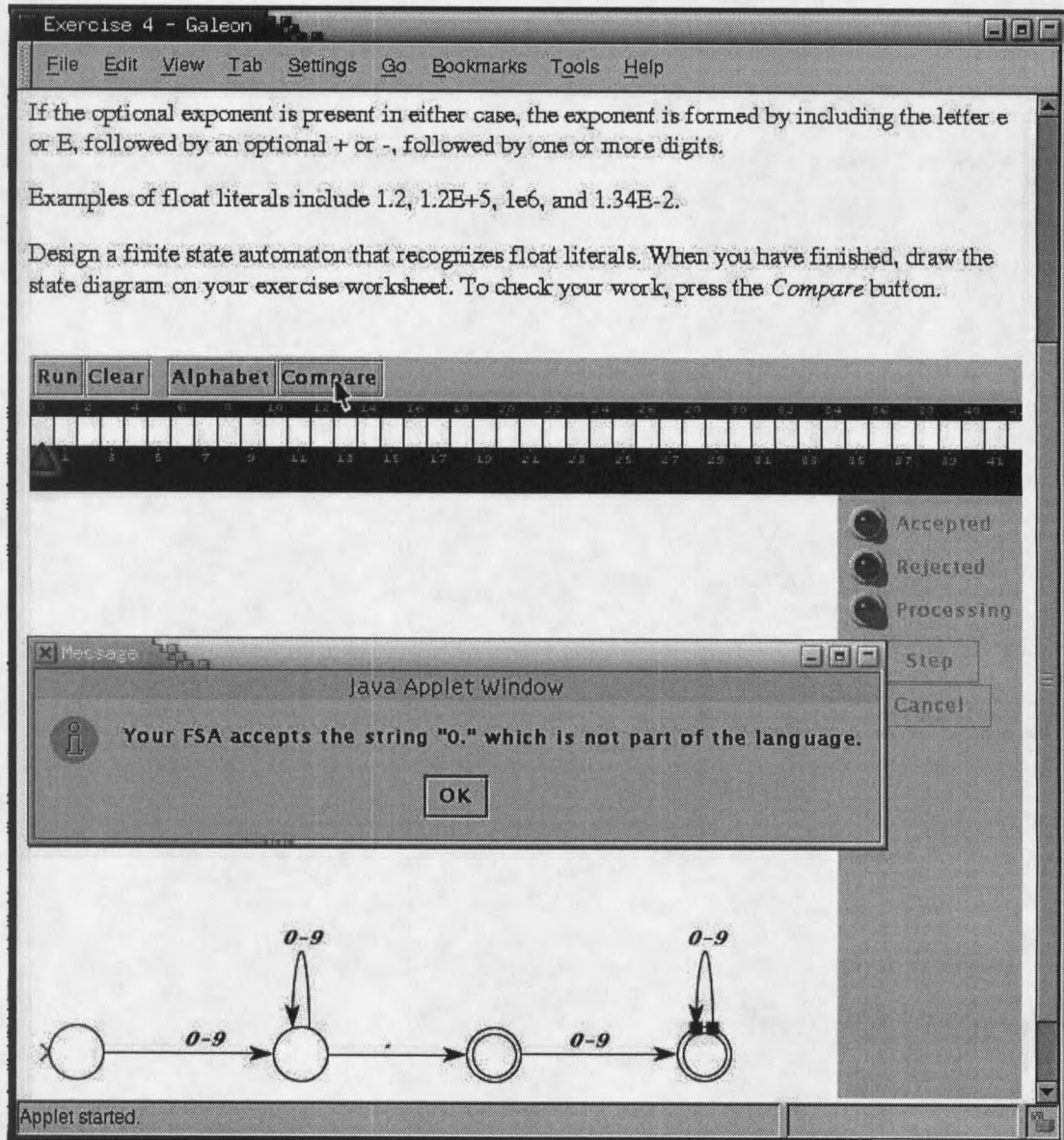
Figure 3.10: FSA comparison message when the student's FSA accepts a string not in the target language
