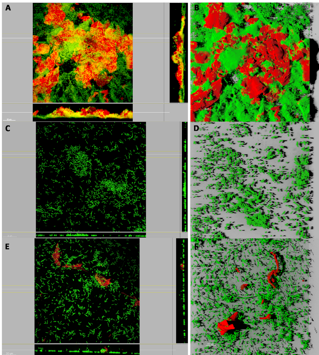
Figure 2. Representative projection analysis (column on the left) and 3-D-reconstructed CLSM images (column on the right) of E. coli biofilm grown on non-functionalized LDPE, LDPE-OH, LDPE-COOH surfaces (A, B), LDPE-CA (C, D) and LDPE-SA (E, F) functionalized surfaces ( \lambda_{\text{ex}} at 488 nm, and \lambda_{\text{em}} < 530 nm, 60 \times , 0.9 NA water immersion objective). Live cells were stained green with SYBR green I, whereas the polysaccharide matrix was stained red with Texas Red-labeled concanavalin A. Scale bar = 20 \mu\text{m} .
