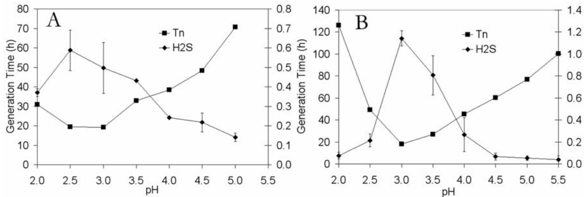
Figure 3.3 Influence of pH on generation time (Tn) and total sulfide production for isolate 18U65 (A) and 18D70 (B).
