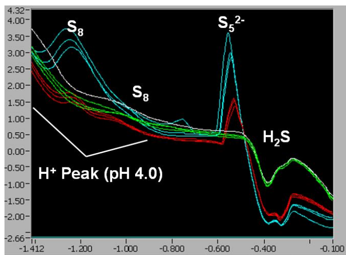
Figure 5.1. Differential pulse voltamogram of A. sulfurireducens (isolate 18D70) grown in the presence of S^{\circ} . Green line, 12 hrs; red line, 24 hrs; white line, 36 hrs; blue line, 72 hrs. X-axis is volts (mV), y-axis is amperage (μA)
