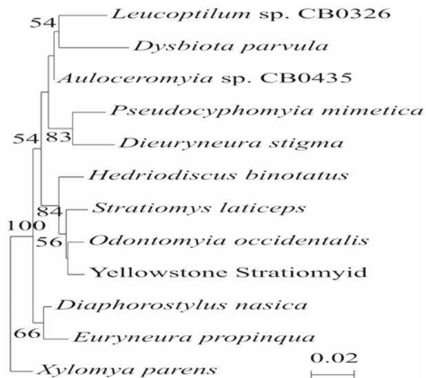
Figure 4.3. Taxonomic affiliation 28S rRNA genes of unclassified Yellowstone stratiomyid larvae and selected members of the Stratiomyidae calculated by the neighbor-joining method using Jukes and Cantor correction. The bar represents 0.02% nucleotide substitution. Bootstrap values of >50% are shown.
