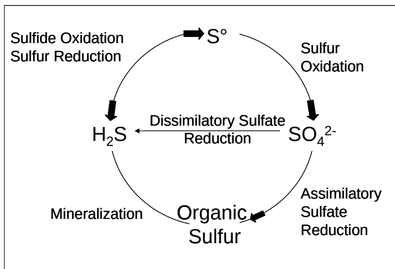
Figure 2.2. Key reactions in the sulfur cycle. Modified from Kleinjan et al (84).
