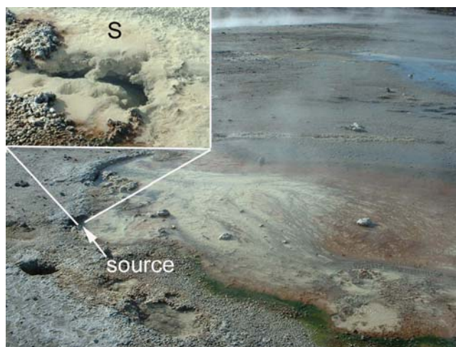
Figure 3.1. Dragon Spring source with abundant \text{S}^{\circ} flocs (labeled S in picture inset)
