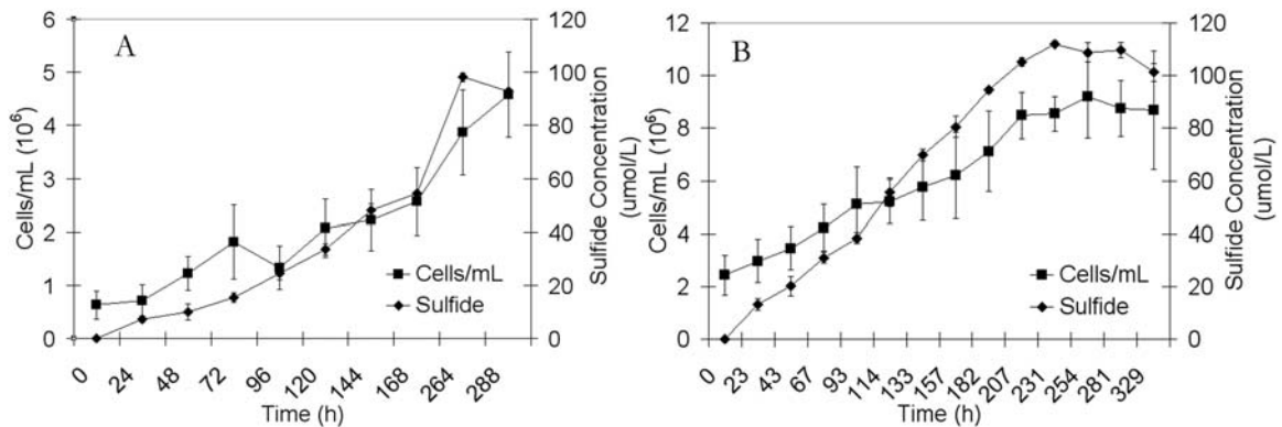
Figure 3.4. Growth curve of isolates 18U65 (A) and 18D70 (B) grown at optimal temperature and pH.
