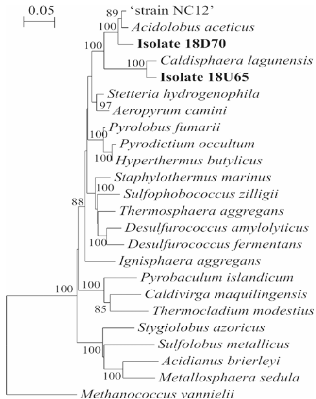
Figure 3.5 Phylogenetic relationship of isolate 18U65 and 18D70 and members of the Crenarchaeota based on comparison of 16S rRNA gene calculated using the neighbor-joining method. Bootstrap values (100 re-samplings) are shown at branch points; values greater than 80 are reported. Bar represents 5 nucleotide substitutions per 100 nucleotides. Methanococcus vanniellii used as the outgroup.
