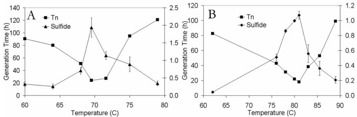
Figure 3.2. Influence of temperature on generation time (Tn) and total sulfide production for isolate 18U65 (A) and 18D70 (B).
