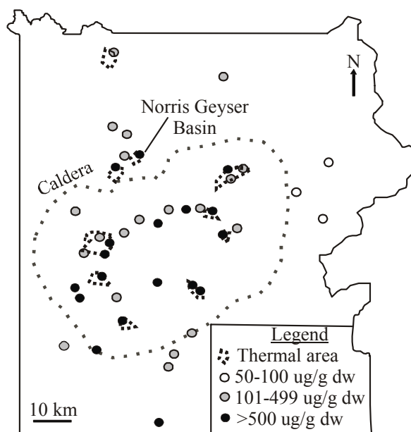
Figure 4.2. Soil mercury concentrations in Yellowstone National Park, Wyoming. Only the major thermal areas are identified. Figure adapted from Phelps and Busick (1980)
