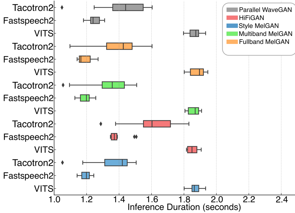
Figure 4.6: Inference time required for each TTS model and vocoder combinations.
