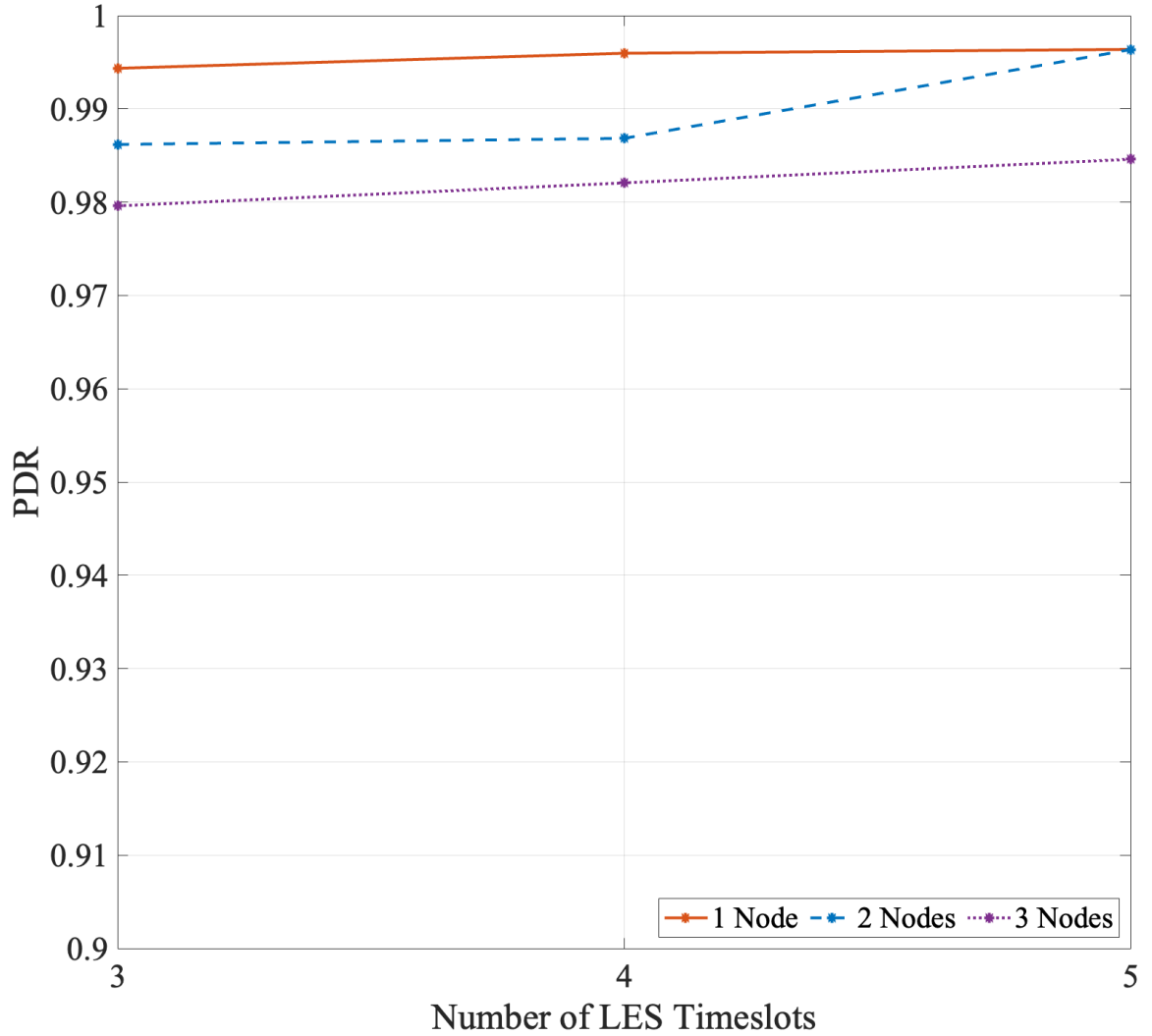
Figure 2.7: PDR versus Number of Control Timeslots.
