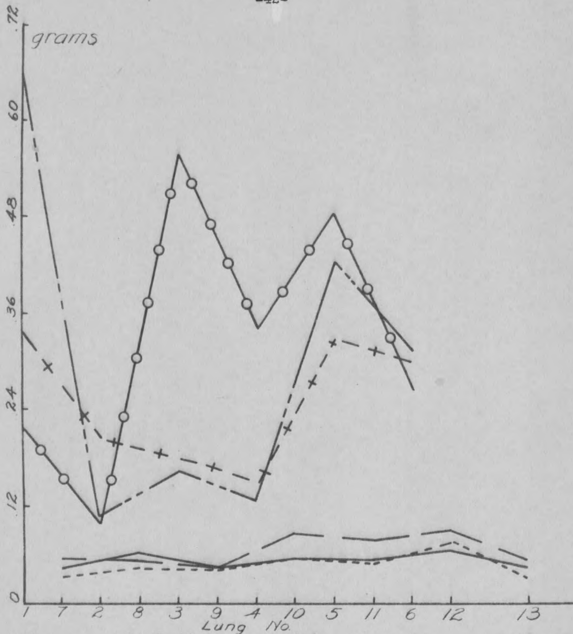
Grams of Calcium, Magnesium, and Iron per Lung in Normal and "Lunger" Sheep (Lungs Arranged According to Increase in Silica Content)
