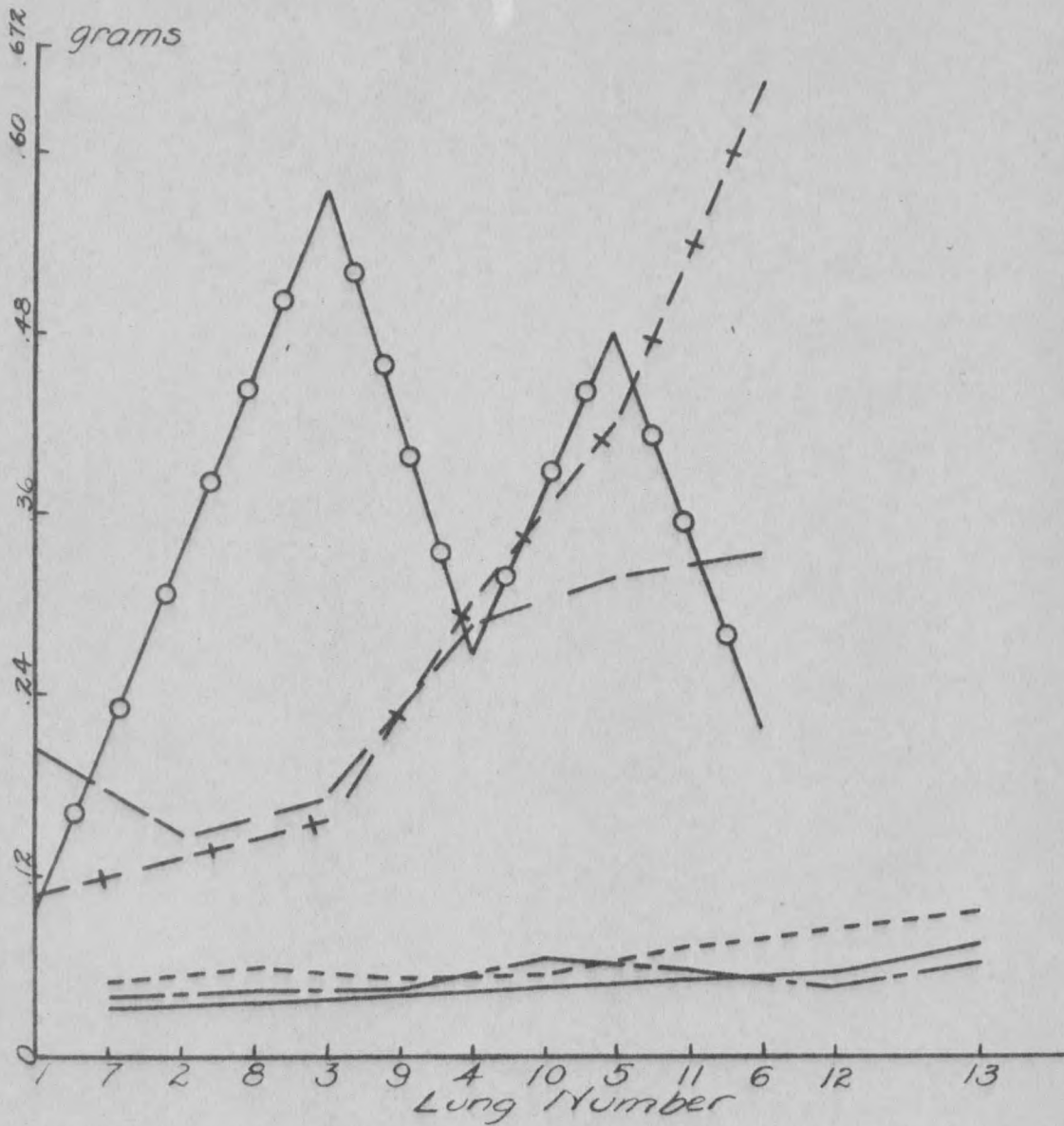
Grams of Calcium, Magnesium and Iron per Lung in Normal and "Lunger" Sheep (Lungs Arranged According to Increase in Calcium Content)
