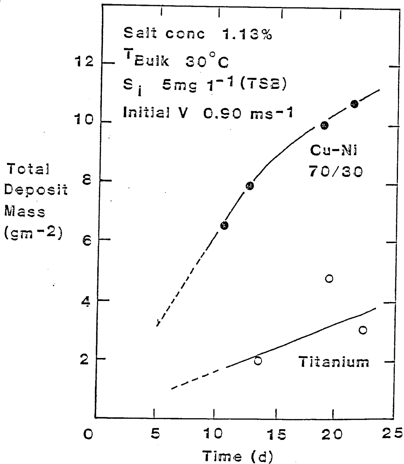
Fig. 15.- Accumulation of fouling deposit on two alloys 19 .
