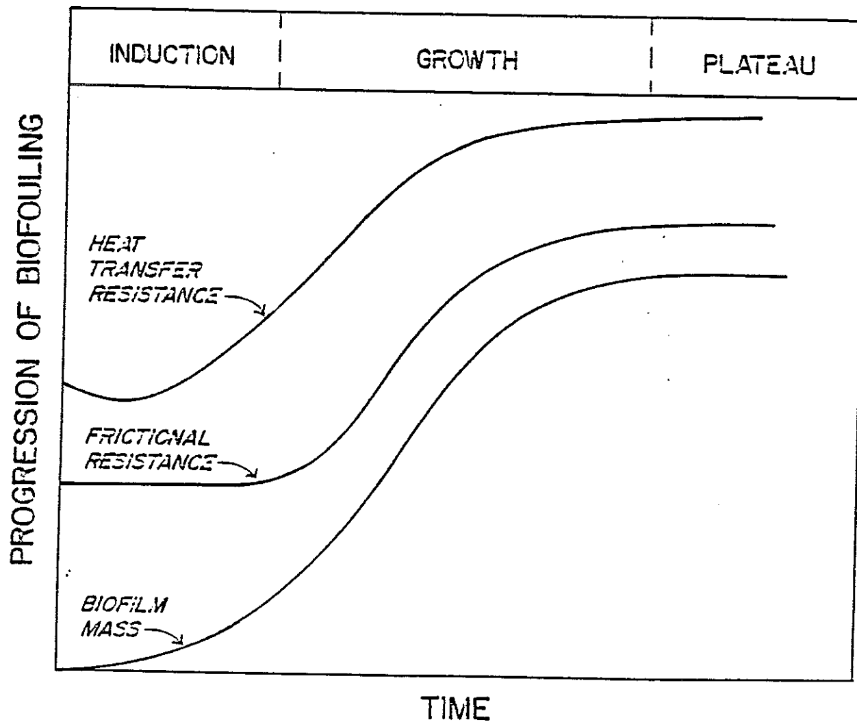
Fig. 6.- A schematic representation of the progression of fouling deposition.
