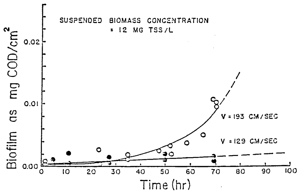
Fig. 13.- Influence of fluid shear stress on biofilm development 29 .
