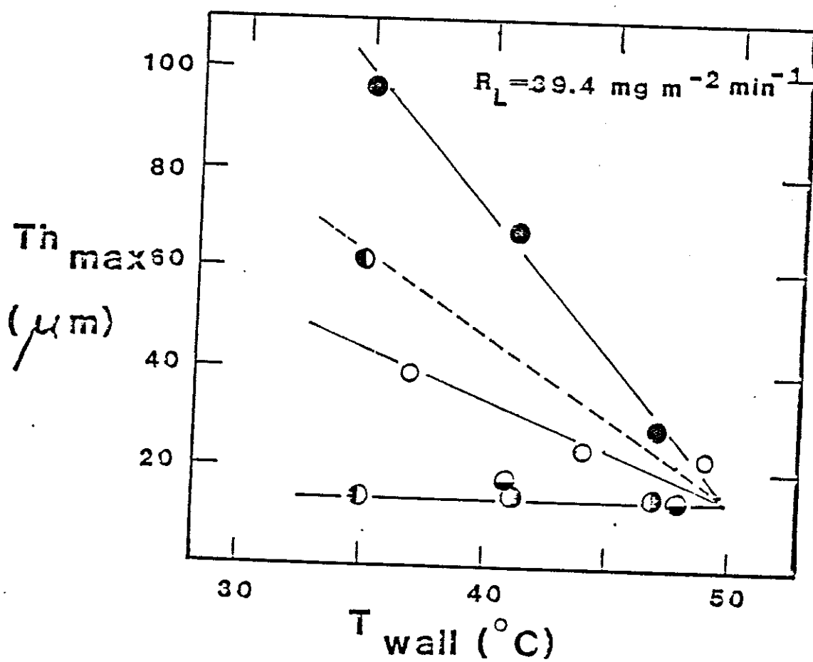
Fig. 12.- The influence of wall temperature and nutrient loading rate on maximum biofouling deposit thickness in a laboratory system 23 .
