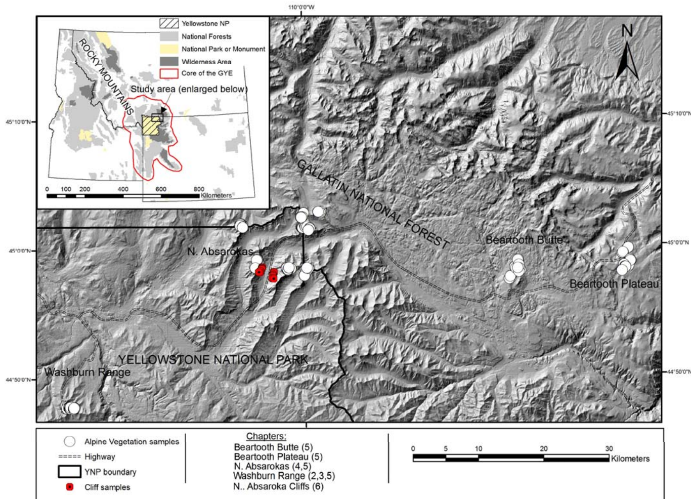
Figure 1.1. Study area locations dealt with in Chapters 2 through 6. The GYE consists of protected federal lands directly adjoining and including Yellowstone National Park (cf. Reese 1991). The North-Central Rocky Mountains encompass a similar region, i.e. regions in the Rockies bounded by the Windriver Range to the south and the Big Belt and Crazy Mountains to the north (Howard and Williams 1972).
