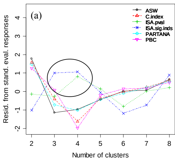
Figure C.1.2. Talus. (a) Individual evaluator responses. (b) Average evaluator response. Four classes chosen as optimum. Note ISA evaluators are being favored over other strategies.
