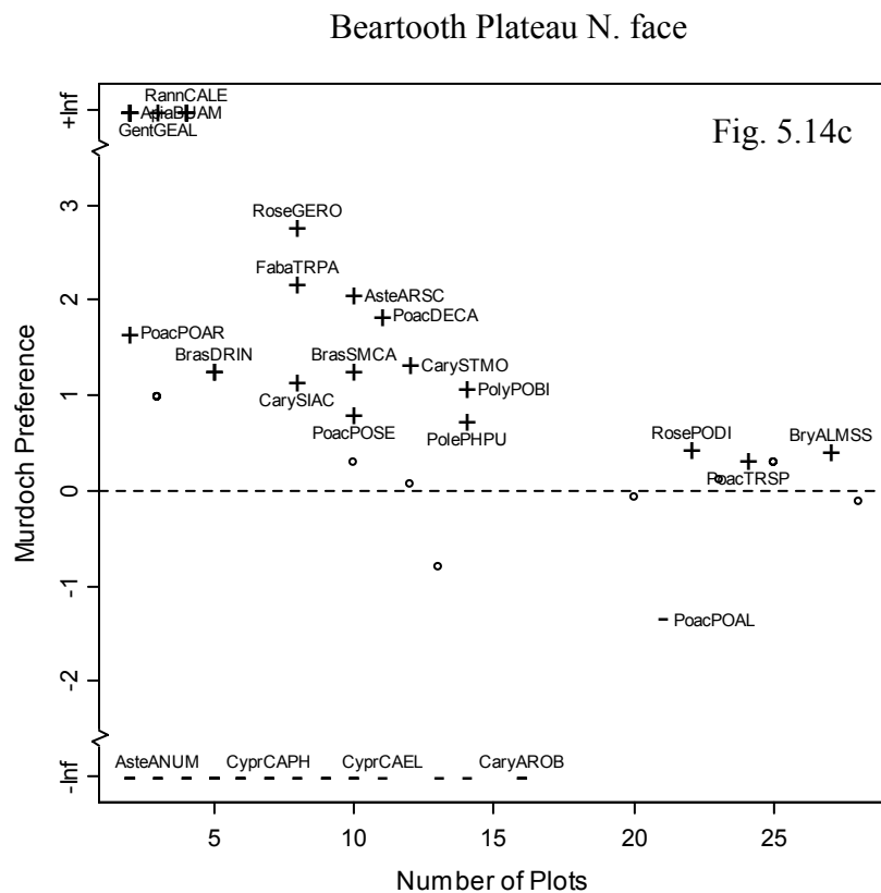
Figure 5.14. Murdoch analysis results for north-facing sites across alpine regions: (a) Washburn Range, (b) N. Absarokas, (c) Beartooth Plateau, (d) Beartooth Butte. Ninety-five species which occurred in at least 5% of the 38 north-facing plots across in the 4 alpine regions were analyzed. Significant positive and negative species are identified where space on the graph allows, “+” indicates a positively significant Murdoch species, “-” indicates a negatively significant Murdoch species, “0” indicates neither significantly positive nor negative. Due to overlaying species not all species can be identified in graphs. For species codes see Appendix D.1. For complete summary of Murdoch analysis for north facing areas see Appendix D.2, Table D.2.6.
