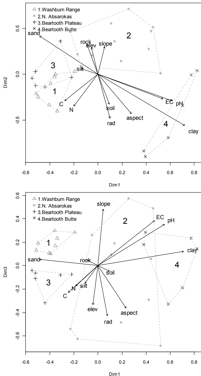
Figure 5.15. Three dimensional NMDS solution for snowbank plots, stress =10.76. Environmental vectors are overlaid, and the four alpine areas are separated by symbols and dashed lines. For exact relationship of vectors to configurations see Table 5.1. For explanations of vector annotations see Fig. 5.3.
