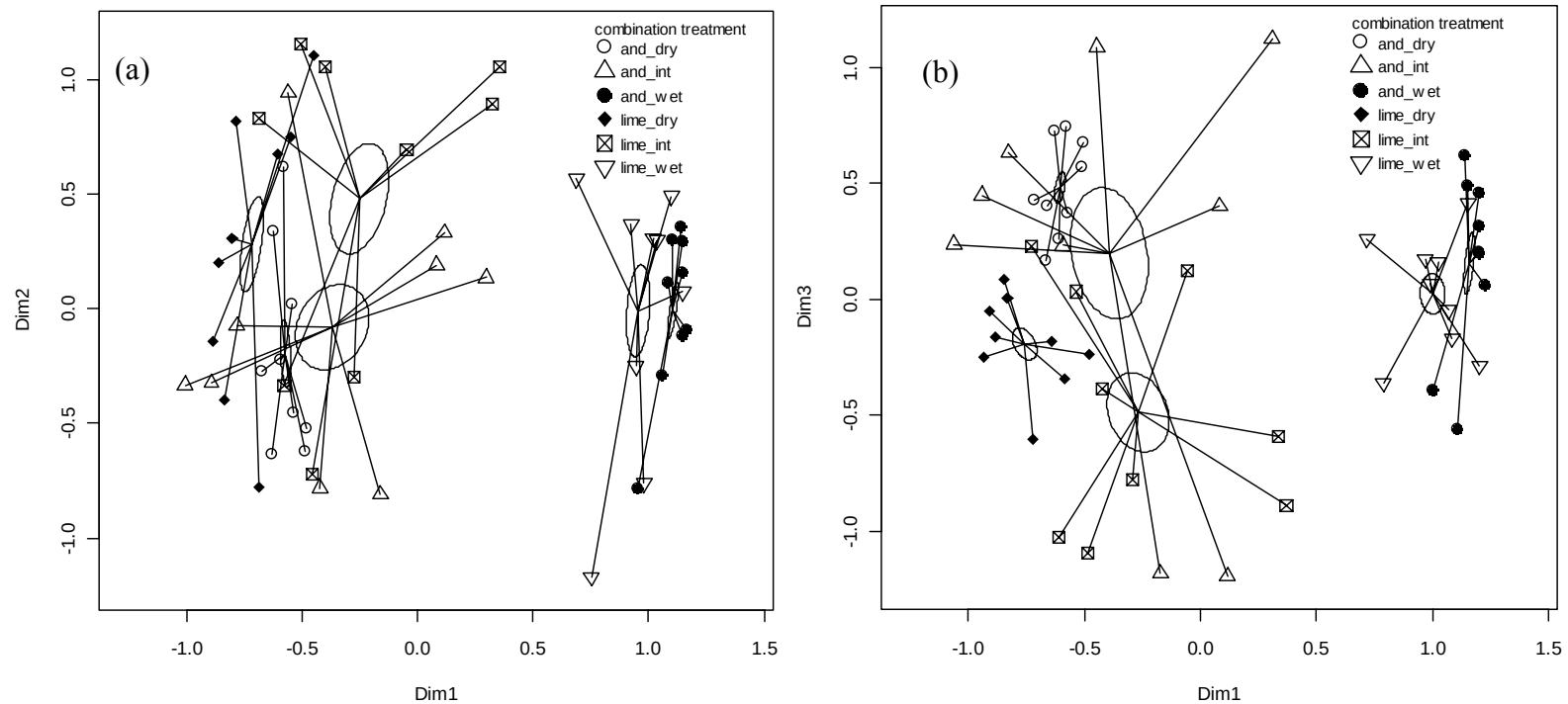
Figure 6.5. Ordination with six water/substrate combination treatments indicated. Spiders connect replicates with the same treatment. Ellipses indicate 95% confidence intervals around treatment centroids.
