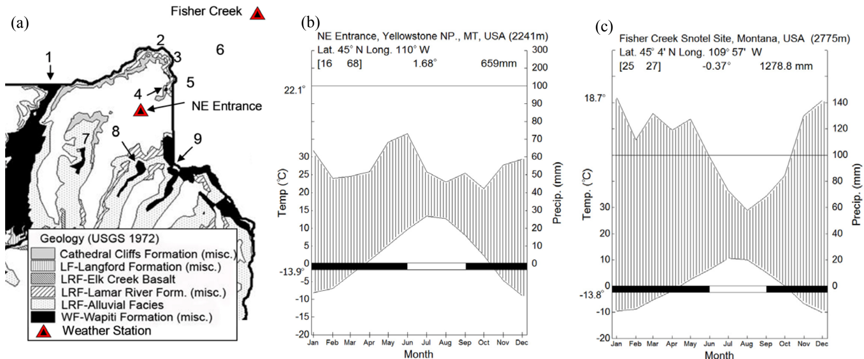
Figure 4.2. Volcanic geology and climatic description of the study area. (a) Locations of Absaroka Volcanic supergroup formations. LF = Langford formation, LRF = Lamar River formation, WF = Wapiti formation, and locations of surveyed peaks: 1. Cutoff, 2. Wolverine, 3. Sunset, 4. Meridian, 5. Mineral, 6. Miller, 7. Barronette, 8. Abiathar, and 9. Amphitheatre. (b, c) Climate diagrams (Walter and Leith 1967) for the Northeast Entrance weather station and the Fisher Creek Snotel site directly adjacent to study area. The upper plotted line indicates average monthly precipitation. The lower plotted line is average mean monthly temperature. The hatched area between the plotted lines indicates the months (in this case all 12 months) that precipitation exceeds evaporation. Text at the top of the figure gives general information about the site, the number of years of temperature and precipitation data were used to create the figure (in brackets), and the overall mean temperature and average yearly precipitation. Along the temperature axis, average daily maximum temperature of the warmest month and average daily minimum temperature of the coldest month are also indicated. The blackened area of the rectangle at the bottom of the figure indicates the frost period (the months where average minimum temperature was below zero degrees). Raw climate data was provided by the Western Regional Climate Center (WRCC 2006).
