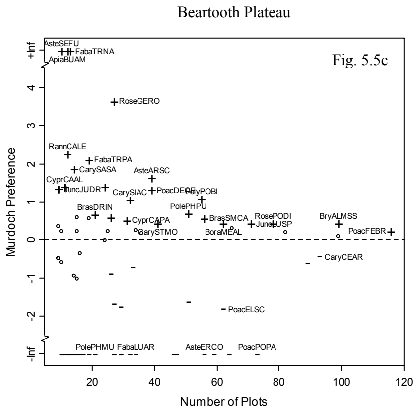
Figure 5.5. Murdoch analysis results for alpine areas: (a) Washburn Range, (b) N. Absarokas, (c) Beartooth Plateau, (d) Beartooth Butte. The eighty-six species which occurred in at least 5% of the 178 plots across the 4 alpine areas were analyzed. Significant positive and negative species are identified where space on the graph allows, “+” indicates a positively significant Murdoch species, “-” indicates a negatively significant Murdoch species, “0” indicates neither significantly positive nor negative. Due to overlaying species not all species can be identified in graphs. For species codes see Appendix D.1. For complete summary of Murdoch analyses for alpine areas see Appendix D.2, Table D.2.2.
