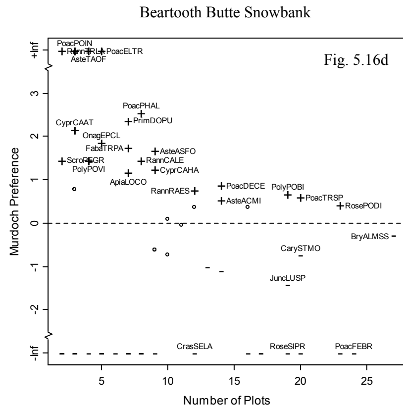
Figure 5.16. Murdoch analysis results for snowbank across alpine regions: (a) Washburn Range, (b) N. Absarokas, (c) Beartooth Plateau, (d) Beartooth Butte. Seven-nine species which occurred in at least 5% of the 32 late-melt plots across in the 4 alpine regions were analyzed. Significant positive and negative species are identified where space on the graph allows, “+” indicates a positively significant Murdoch species, “-” indicates a negatively significant Murdoch species, “0” indicates neither significantly positive nor negative. Due to overlaying species not all species can be identified in graphs. For species codes see Appendix D.1. For complete summary of Murdoch analysis for late melt areas see Appendix D.2, Table D.2.7.
