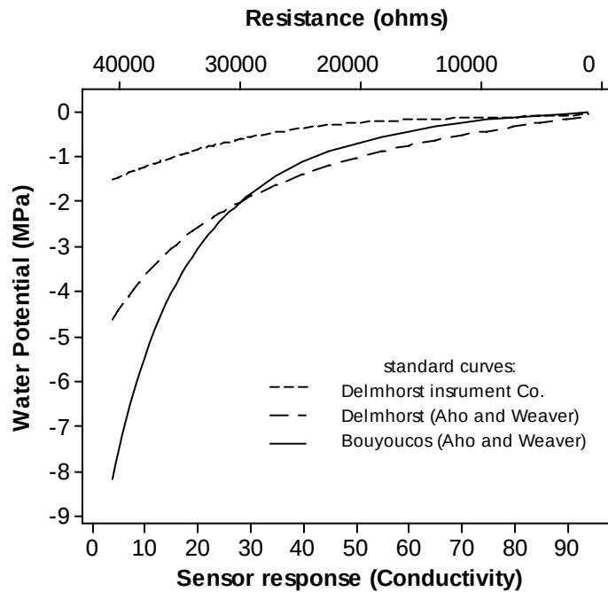
Figure 9.2. Relationship of soil water potential to meter reading and approximate electrical resistance (ohms) for Bouyoucos and Delmhorst sensors (Eqs. 9.1-9.2). A calibration curve provided by Delmhorst Inst Co. for use with their meter and blocks is also shown (see Eq. 9.3).
