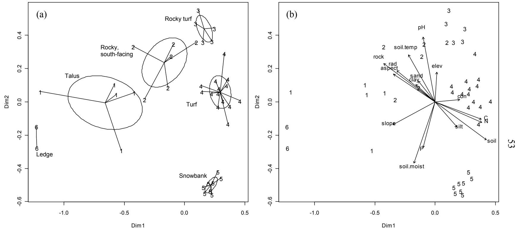
Figure. 3.3. NMDS ordination and vector analysis of Washburn data. (a) Communities indicated with spider diagrams. Ellipses indicate 95% confidence intervals around cluster centroids. Community 1 = Elymus scribneri talus (ELSC), community 2 = Senecio canus - Astragalus kentrophyta (SECA-ASKE), community 3 = Erigeron rydbergii - Oxytropis lagopus (ERRY-OXLA), community 4 = Carex elynoides - Astragalus alpina (CAEL-ASAL), community 5 = Carex paysonis - Artemisia scopulorum (CAPA-ARSC), community 6 = Arnica rydbergii (ARRY). (b) Vector analysis. Environmental variables are: P = Phosphorous ( \text{mg kg}^{-1} ), C = % soil carbon, N = % soil nitrogen, elev = elevation (m), slope = slope(degrees), aspect = degrees from N, rad = solar radiation ( \text{MJ} \cdot \text{cm}^2/\text{yr.} ), soil = % cover of surface soil, con = soil conductivity ( \text{mmhos cm}^{-1} ), sand = % sand content of soil, clay = % clay content of soil, silt = % silt content of soil, soil.temp. = soil temp (number of summer days > 10^\circ\text{C} ), soil moist = soil moisture (number of summer days wetter than -0.12\text{Mpa} ). Note that (b) is an identical ordination to (a) . Final stress for 2D NMDS solution = 12.9.
