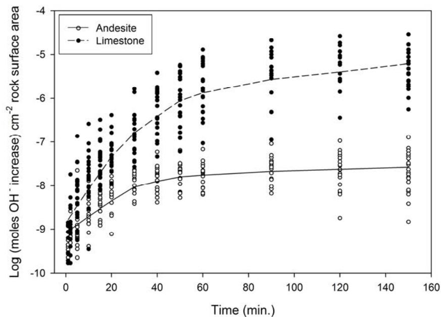
Figure 8.4. Equilibration of pH for samples in KCl solution [ \log(\Delta \text{moles OH}^- \text{ ions}) \text{ cm}^{-2} \text{ min}^{-1} ]. Differences between substrates were statistically significant after 15 minutes. Lines are lowess smoothers.
