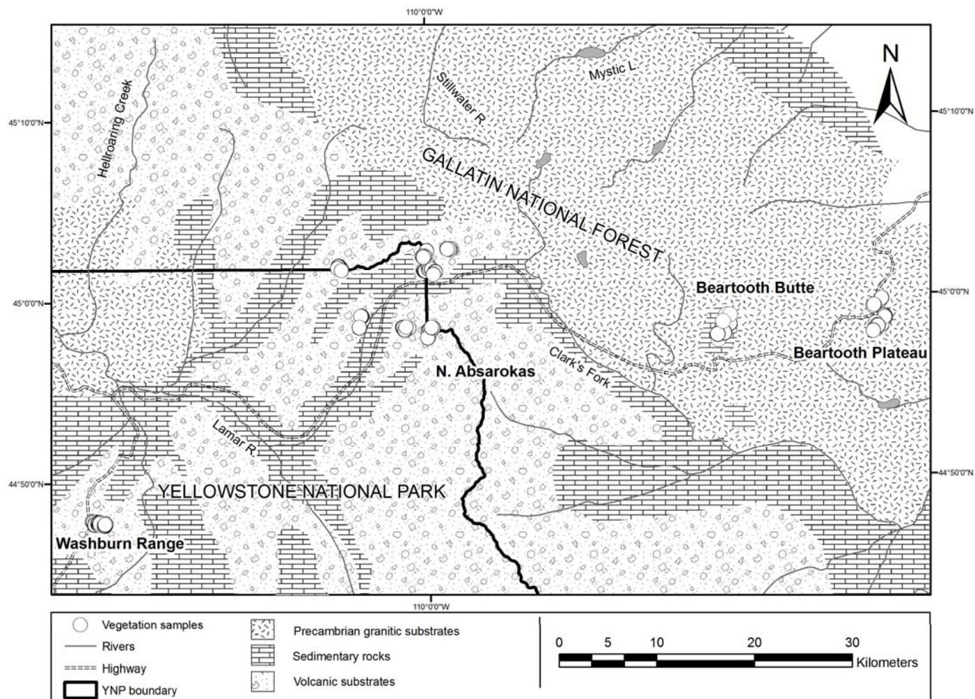
Figure 5.1b. General geology of study area. Map follows Anderson (1984).
