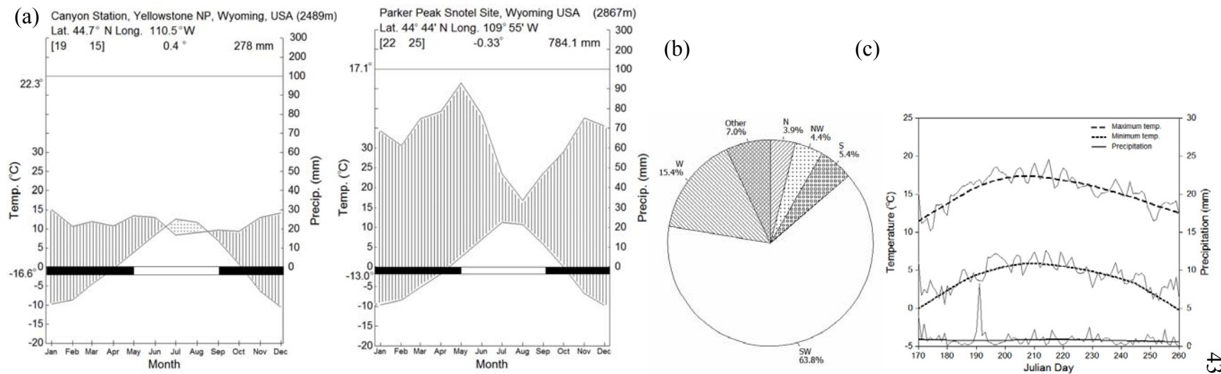
Figure 3.2. Climate of Mount Washburn. (a) Climate diagram (cf. Walter and Leith 1967) for the Canyon Village weather station adjacent to ( < 11 km), and 600m below the Washburn summit and the Parker Peak snotel station, near alpine elevation (2867m) and 50 km to the east (see Fig. 3.1). Raw climate data was provided by the Western Regional Climate Center (WRCC 2006). The upper plotted line indicates average monthly precipitation; the lower humped line indicates average mean monthly temperature. The vertically hatched area indicates the months that precipitation exceeds evaporation. The dotted area (Fig. 3.2a only) indicates months when evaporation exceeds precipitation. Text at the top of the climate diagrams gives general information about the site: the length of records in years for temperature and precipitation data respectively (in brackets), the latitude and longitude, the name of the station, the elevation, and the average yearly precipitation and overall mean temperature. Average daily maximum temperature of the warmest month and average daily minimum temperature of the coldest month are also indicated on the temperature axis. The blackened area of the long rectangle near the bottom of the figure indicates the frost period (i.e. the months when average minimum temperature was < 0^{\circ}\text{C} ). (b) Wind direction, at the Washburn summit, for 1965-1997 and 2001-2004 (N = north, S = south, W = west). (c) Summer weather data at the Washburn summit (1965-2004) showing mean maximum temperature, mean minimum temperature, and mean precipitation. Localized weighted scatterplot smoother (LOWESS) lines are superimposed. Washburn summit weather data was provided by the National Park Service. For additional regional climate information see Figs. 4.2, 5.1c, and 5.2.
