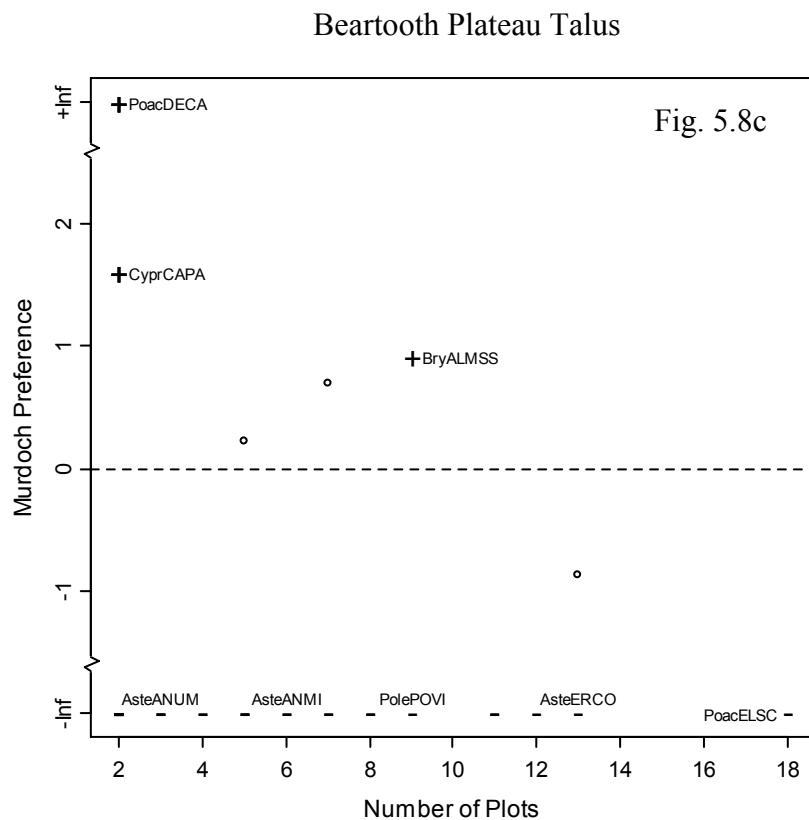
Figure 5.8. Murdoch analysis results for talus sites across alpine regions: (a) Washburn Range, (b) N. Absarokas, (c) Beartooth Plateau, (d) Beartooth Butte. Forty-five species (those which occurred in at least 5% of the 36 talus plots sampled in the 4 alpine regions) were analyzed. Significant positive and negative species are identified where space on the graph allows, “+” indicates a positively significant Murdoch species, “-” indicates a negatively significant Murdoch species, “0” indicates neither significantly positive nor negative. Due to overlapping species not all species can be identified in graphs. For species codes see Appendix D.1. For complete summary of Murdoch analysis for talus areas see Appendix D.2, Table D.2.3.
