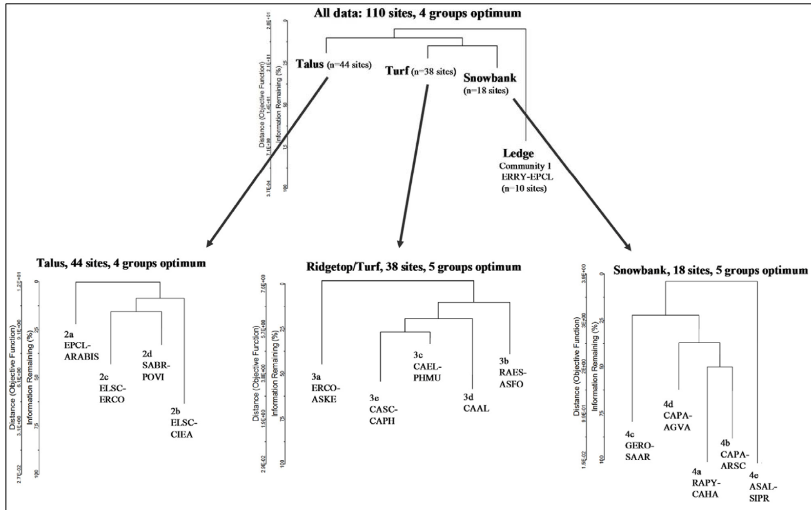
Figure 4.3. Dendrograms showing the division of the entire data set into four super-types ( ledge, talus, turf, and snowbank) and subdivision of those types into fifteen communities. Flexible- \beta agglomerative classification was used to identify types.
