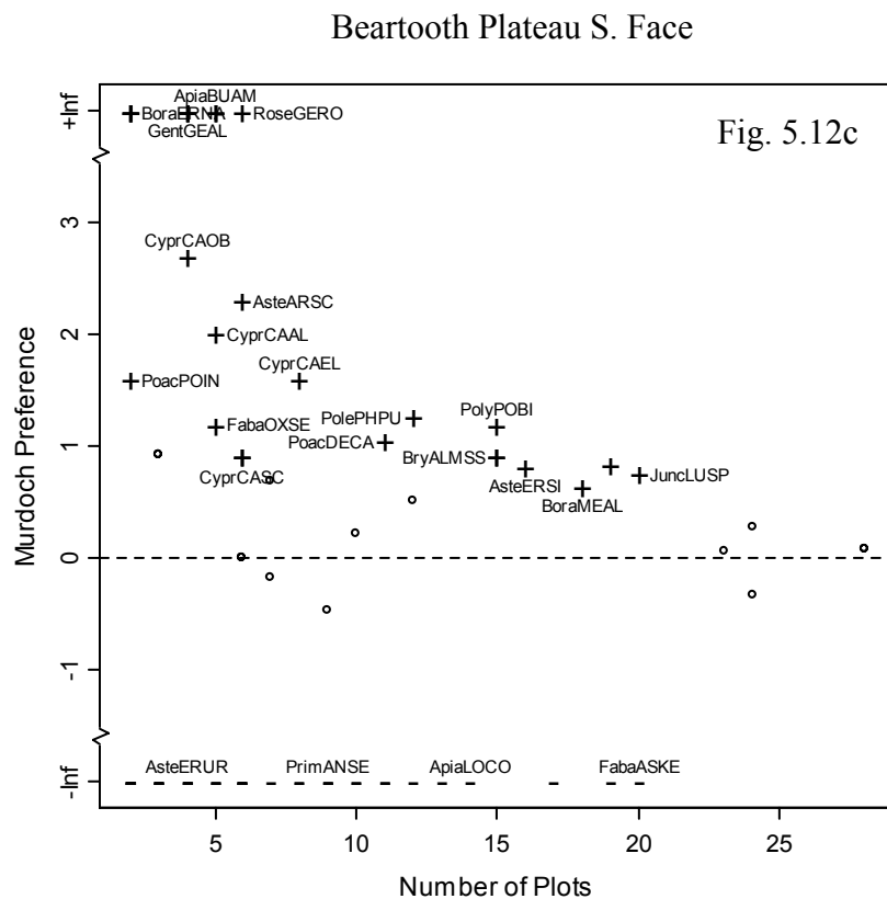
Figure 5.12. Murdoch analysis results for south-facing sites across alpine regions: (a) Washburn Range, (b) N. Absarokas, (c) Beartooth Plateau, (d) Beartooth Butte. Eighty-five species which occurred in at least 5% of the 36 south-facing plots across in the 4 alpine regions were analyzed. Significant positive and negative species are identified where space on the graph allows, “+” indicates a positively significant Murdoch species, “-” indicates a negatively significant Murdoch species, “0” indicates neither significantly positive nor negative. Due to overlaying species not all species can be identified in graphs. For species codes see Appendix D.1 for complete summary of Murdoch analysis for south facing areas see Appendix D.2, Table D.2.5.
