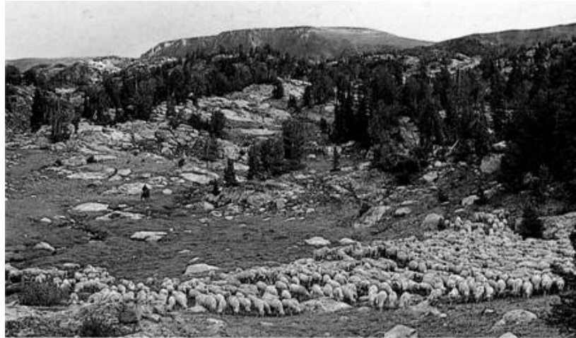
Figure 5.6. Domestic sheep grazing on the Beartooth Plateau (Anderson 1984). Domestic grazing may account for particularly high levels of unpalatable G. rossi on the Beartooth Plateau.
