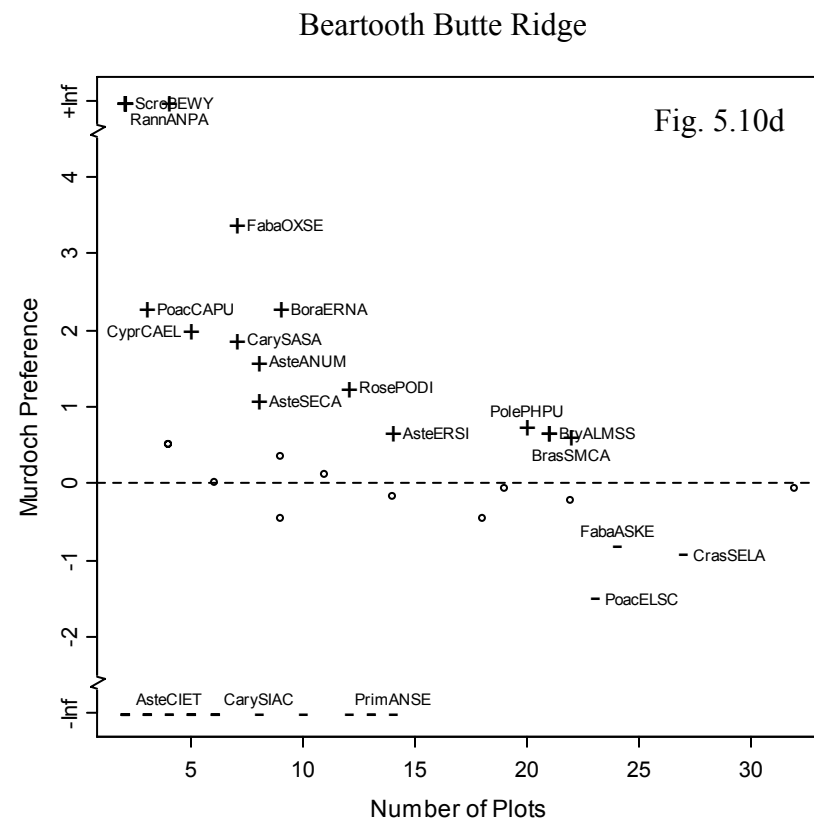
Figure 5.10. Murdoch analysis results for ridgetop sites across alpine regions: (a) Washburn Range, (b) N. Absarokas, (c) Beartooth Plateau, (d) Beartooth Butte. Sixty-seven species (those which occurred in at least 5% of the 36 ridge plots sampled in the 4 alpine regions) were analyzed. Significant positive and negative species are identified where space on the graph allows, “+” indicates a positively significant Murdoch species, “-” indicates a negatively significant Murdoch species, “0” indicates neither significantly positive nor negative. Due to overlapping species not all species can be identified in graphs. For species codes see Appendix D.1. For complete summary of Murdoch analysis for ridge areas see Appendix D.2.4.
