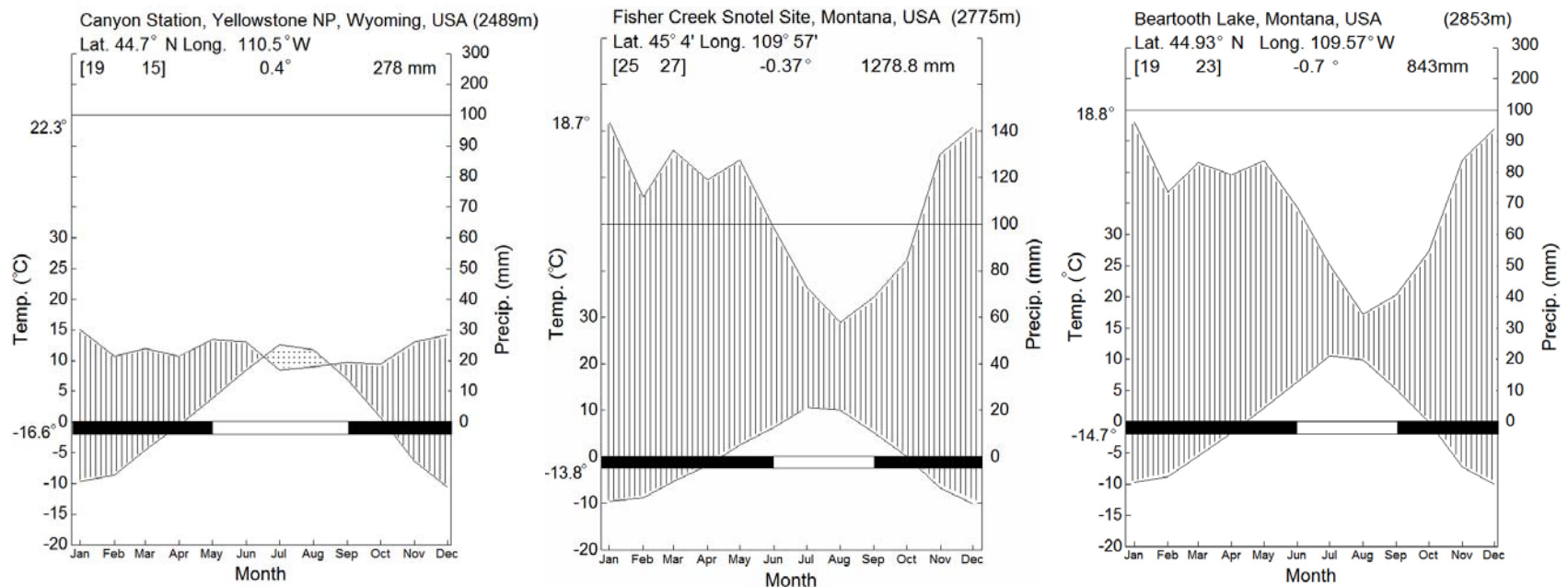
Figure 5.2. Climatic diagrams (cf. Walter and Lieth 1967) for weather stations adjacent to study sites. The Canyon Village weather station is adjacent to Mt. Washburn (for additional climate data on Washburn see Fig. 3.2). The Fisher Creek Station is close to Northern Absaroka sites. The Beartooth Lake station is close to Beartooth Plateau and Beartooth Butte sites (see Fig. 5.1c). The upper plotted line indicates average monthly precipitation; the lower humped line indicates average mean monthly temperature. The vertically hatched area indicates the months that precipitation exceeds evaporation. The dotted area on the Canyon Station diagram indicates months when evaporation exceeds precipitation. Text at the top of the figure gives general information about the site: the length of records in years for temperature and precipitation data respectively (in brackets), the latitude and longitude, the name of the station, the elevation, and the average yearly precipitation and overall mean temperature. Average daily maximum temperature of the warmest month and average daily minimum temperature of the coldest month are also indicated on the temperature axis. The blackened area of the long rectangle near the bottom of the figure indicates the frost period (i.e. the months when average minimum temperature was < 0^{\circ}\text{C} ). Raw climate data was provided by the Western Regional Climate Center (WRCC 2006).
