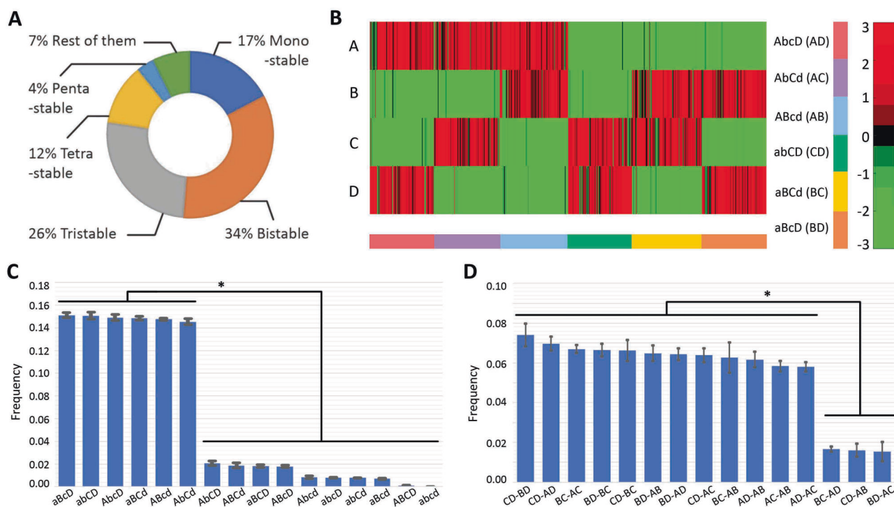
Fig. 2 | Characterization of phenotypes enabled by a toggle tetrahedron.
