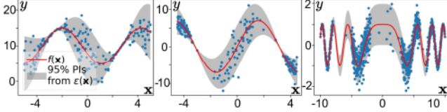
Figure 3: Initial cos , hetero , and cosqr datasets and the ideal 95% PIs calculated from \varepsilon_a(x) across the domain.
