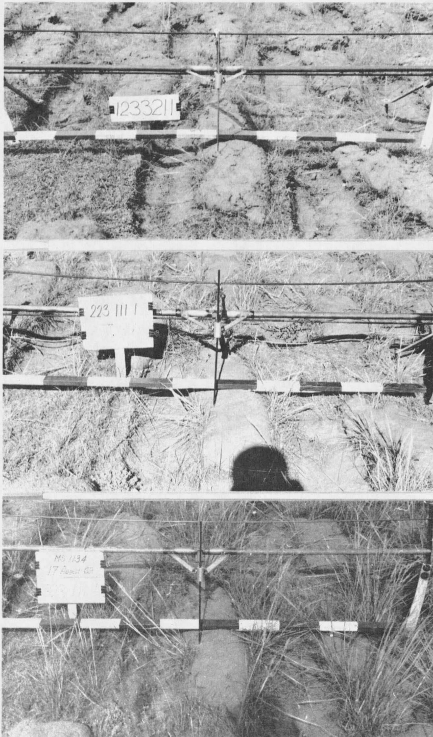
Figure 13. Pitted, unfertilized range: A. 1960; B. 1961; C. 1962. The higher amount of available moisture is reflected in grass vigor.
