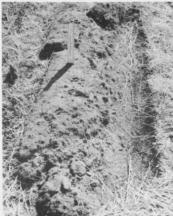
Figure 4. Freshly made pit. Overturned sod oriented by hand.
