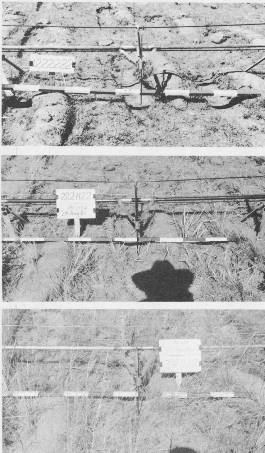
Figure 14. Pitted range which received nitrogen at the rate of 50 pounds per acre in 1959 only. Views taken A. 1960; B. 1961; C. 1962.
