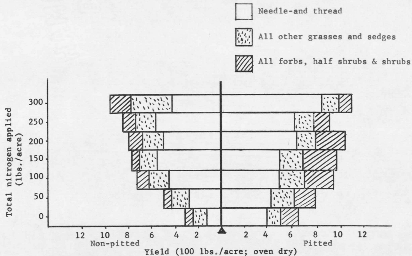
Figure 11. Total yields of pitted and non-pitted range as affected by total amounts of nitrogen fertilizers applied over a three-year period (1959-61). (Oven dry weights).
