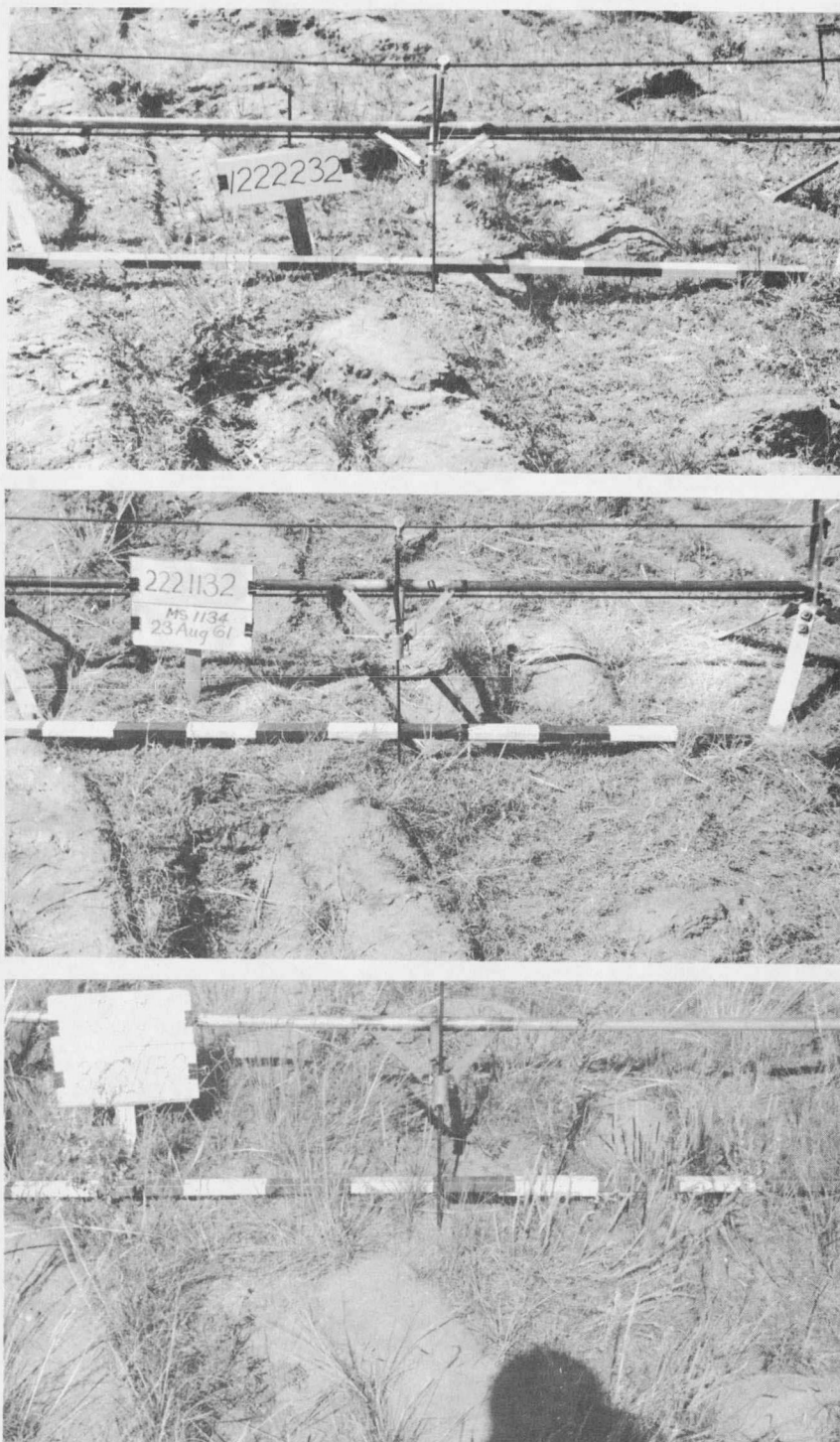
Figure 15. Pitted range which received nitrogen at the rate of 100 pounds per acre in 1959 only. Views taken A. 1960; B. 1961; C. 1962.
