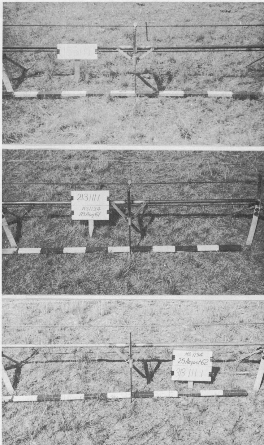
Figure 12. Non-pitted, unfertilized plot: A. 1960; B. 1961; C. 1962. Note relatively small amount of change although seasonal precipitations varied greatly.
