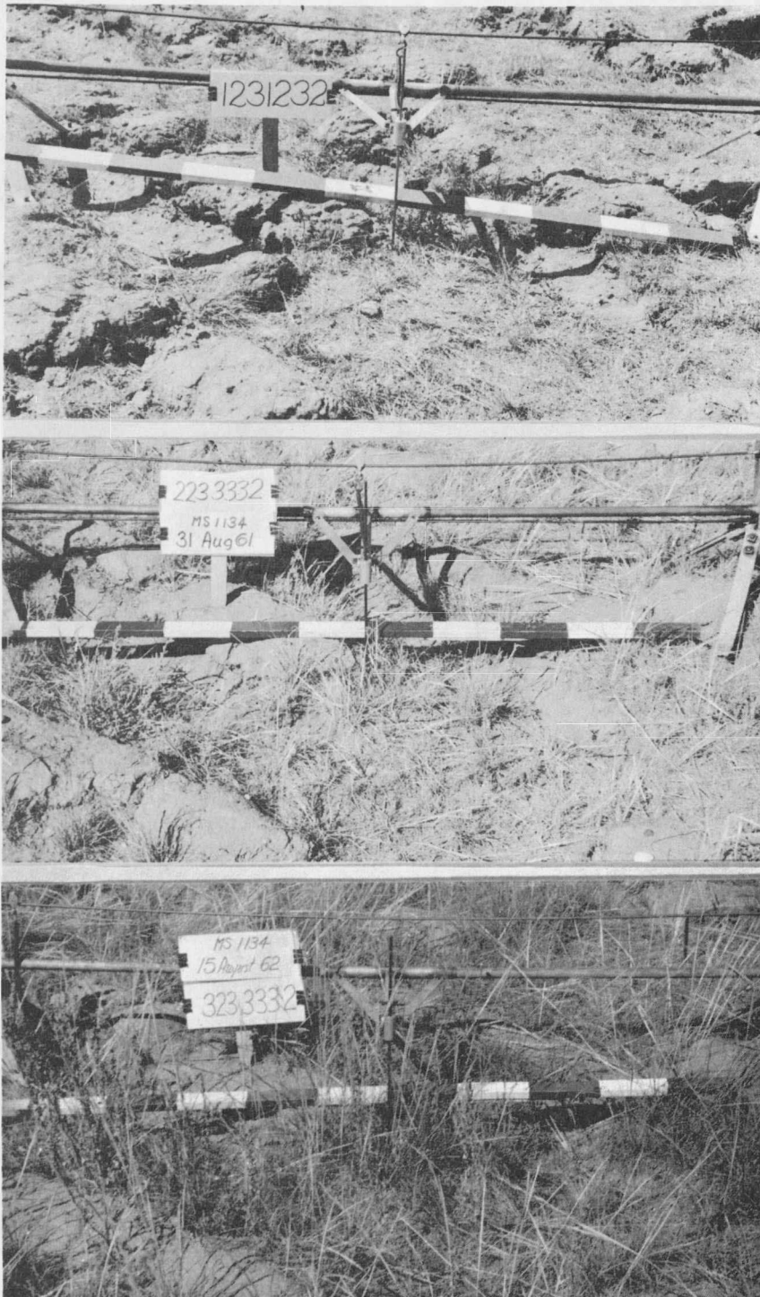
Figure 16. Pitted range which received nitrogen at the rate of 100 pounds per acre during 1959, 1960, and 1961. Views taken A. 1960; B. 1961; C. 1962.
