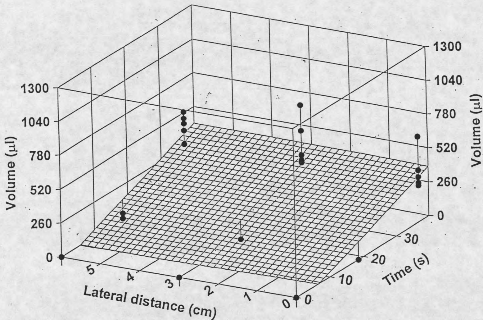
Figure 3. Spray pattern of water and neem kernel extract. Plane described by the equation: Volume of NKE = -74 + 11.3(\text{time}) + 1.8(\text{lateral distance})
