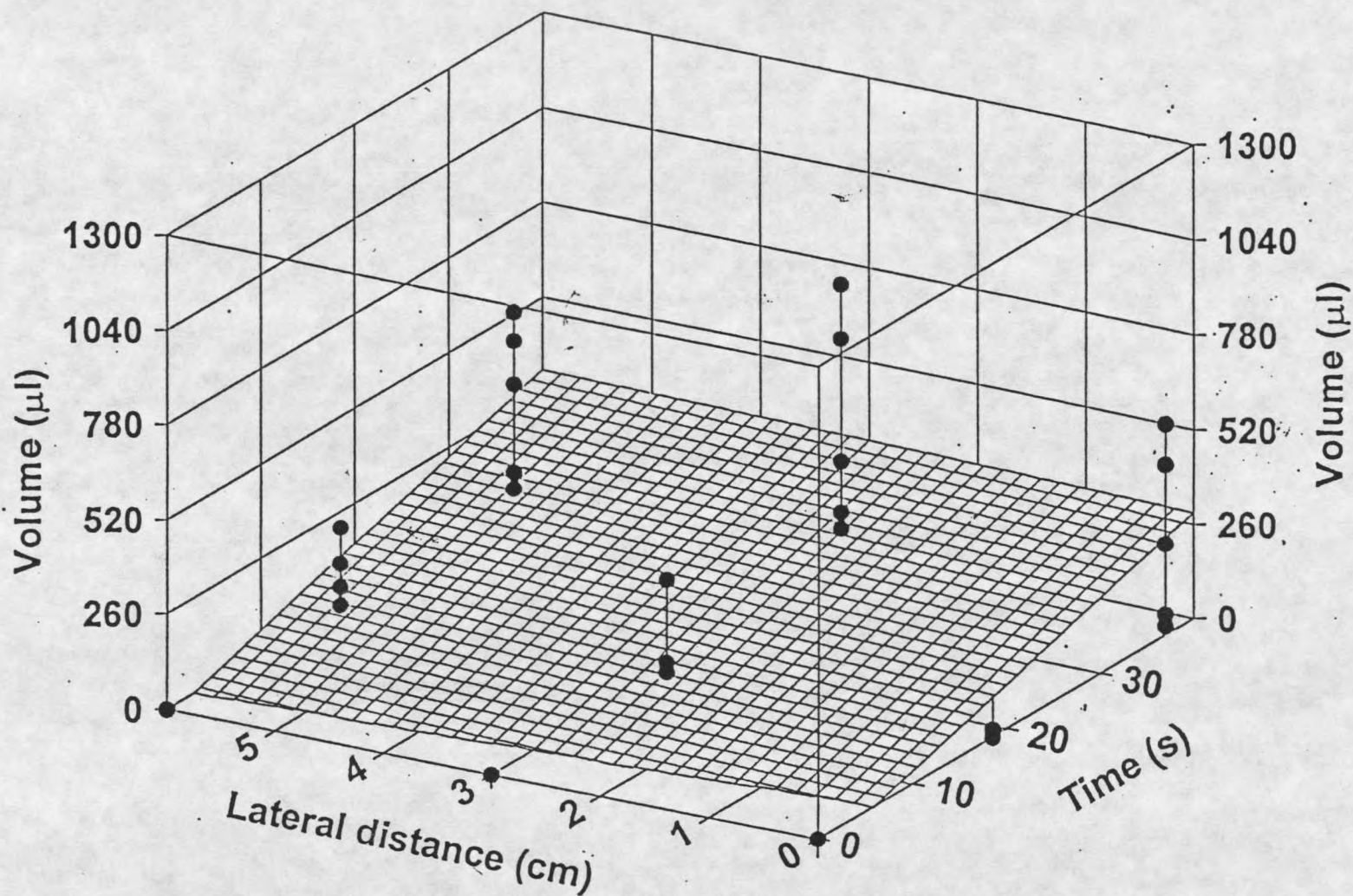
Figure 4. Spray pattern of water and neem kernel extract with 3.5 g of village prepared soap. Plane described by the equation: Volume of NKE = -51 + 8.6(\text{time}) + 4.4(\text{lateral distance})
