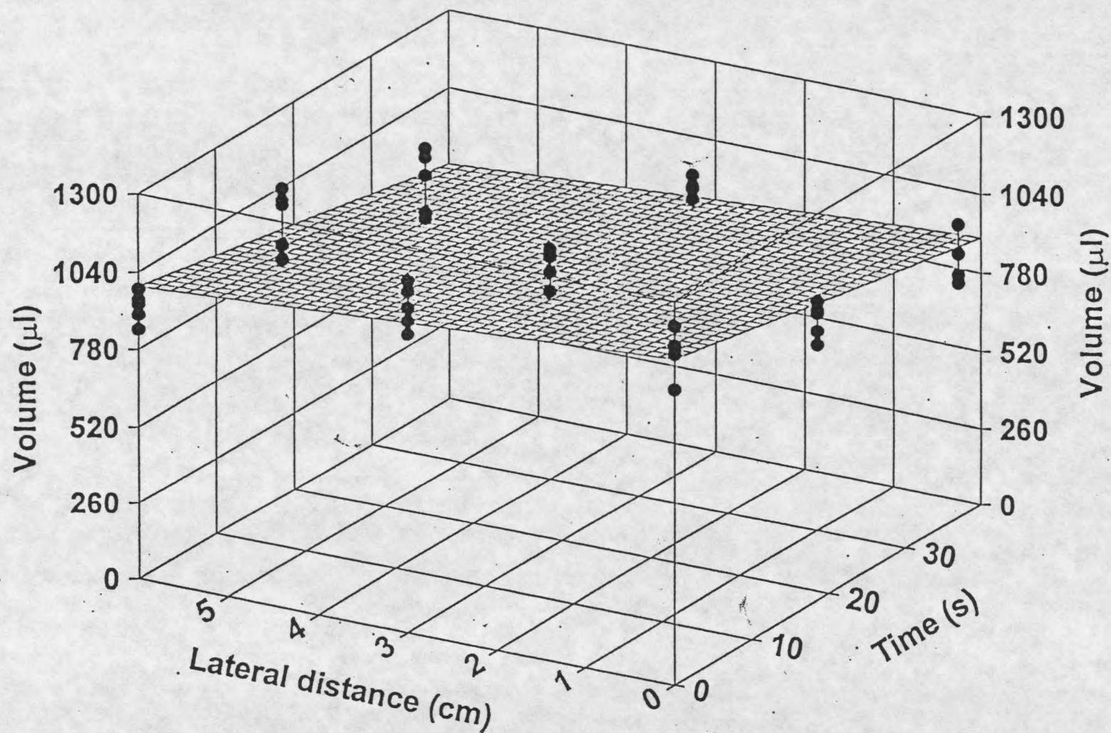
Figure 2. Spray pattern of water alone. Plane described by the equation: Volume of water = 1103 - 5.2(\text{time}) - 18.2(\text{lateral distance})
