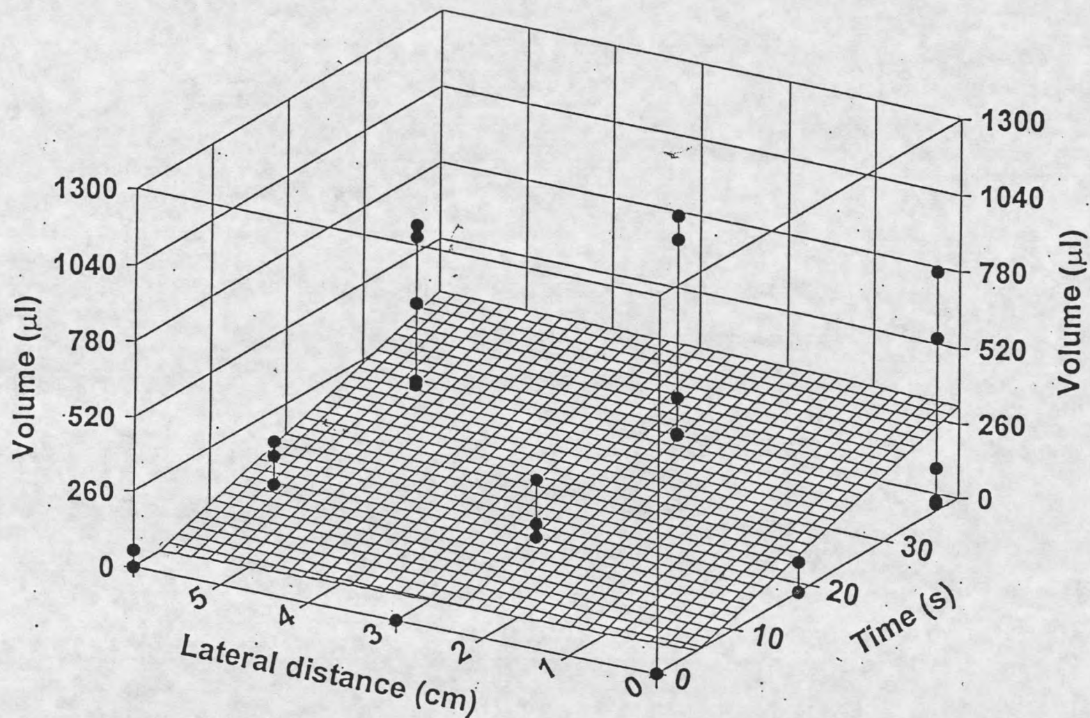
Figure 5. Spray pattern of water (0.25% X-77 surfactant) and neem kernel extract. Plane described by the equation: Volume of NKE = -50 + 9.3(\text{time}) + 2.7(\text{lateral distance})
