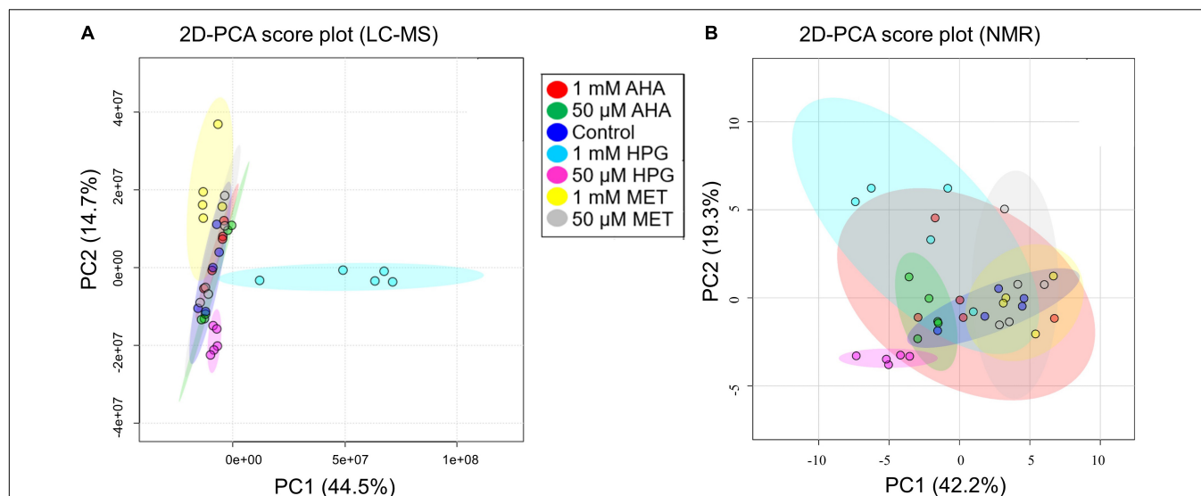
FIGURE 1 | 2D-PCA plots of all experimental conditions from E. coli NCAA experiment. (A) MS data and (B) NMR data are shown. (A) The PCA plot of the MS data shows that only cultures grown with 1 mM HPG separate from the other experiment conditions. (B) The NMR data show significant overlap and a lack of differentiation between experimental groups, the only exception being the group with 50 \mu M HPG.
