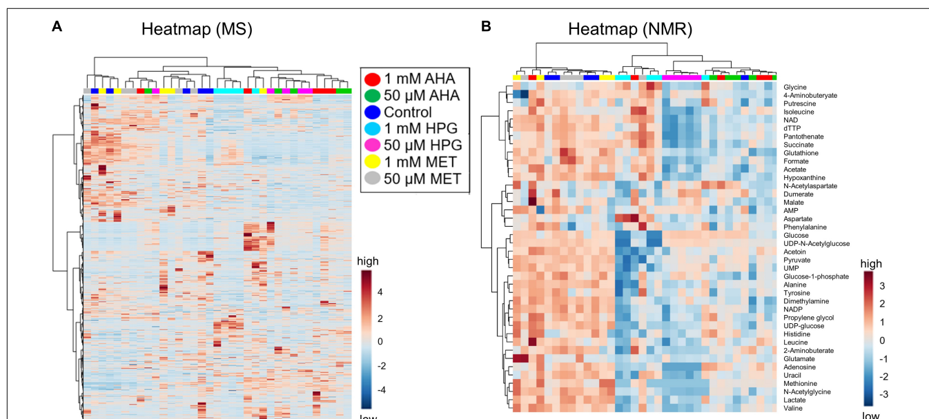
FIGURE 2 | Heatmaps of treatment groups clustered on metabolite intensity from E. coli NCAA experiment. (A) MS data and (B) NMR data are shown. The scale of the heat map indicates blue as lowest and red as highest in abundance as calculated across sample groups after normalization using fold change. (A) The heatmap with HCA of 4,036 features as detected by MS is shown. The lack of clustering of the different experimental groups and no significant patterns of up- or down-regulated features for the different groups are indicative of a lack of differentiation between sample types. (B) The NMR data (40 metabolites) also shows a lack of group clustering, the only exception being the group with 50 \mu M HPG. For enlarged images with metabolite names and sample identifications see Supplementary Figure S5 .
