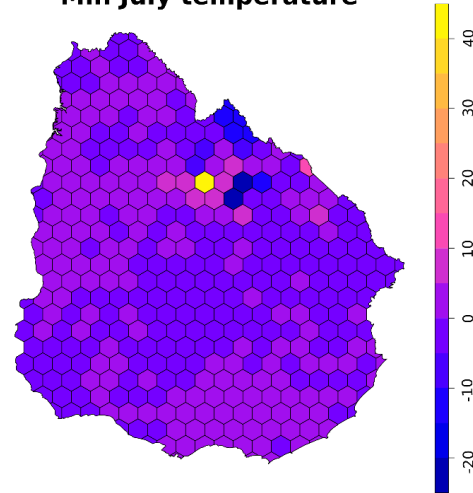
D Min July temperature
