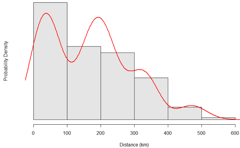
Supplementary Figure 8. Distribution of pairwise distances among colonies used for the metapopulation model simulations. A right-skewed bimodal distribution is observed, where the first density peak corresponds to the intra-cluster distances and the second peak account for inter-cluster distances.
