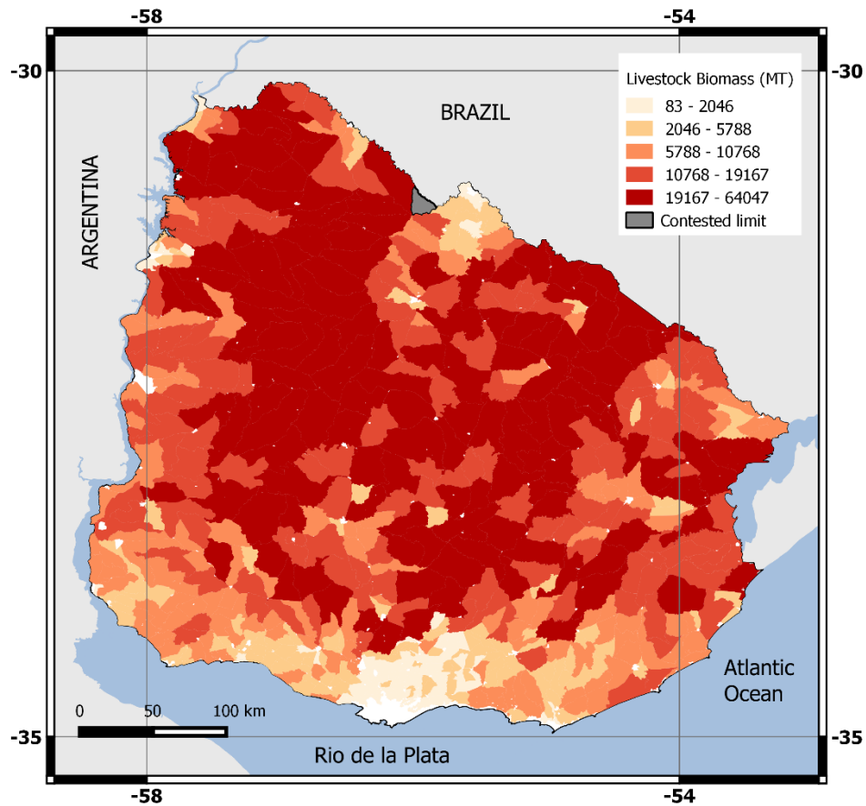
Supplementary Figure S2. Livestock biomass (in metric tons) according to the Uruguay 2011 agricultural census. To obtain the total livestock biomass we multiplied the main total abundance of three livestock prey for vampire bats (cattle, sheep and horses) obtained from the census data, by the average weight for each species, obtained from PanTHERIA database (Jones et al. 2009). Mean weight for the three species is 618, 39 and 403 kg for cattle, sheep and horses respectively. Cattle biomass is currently the best proxy for vampire bat abundance, as there is no direct estimation of population sizes nor a complete inventory of shelters.
