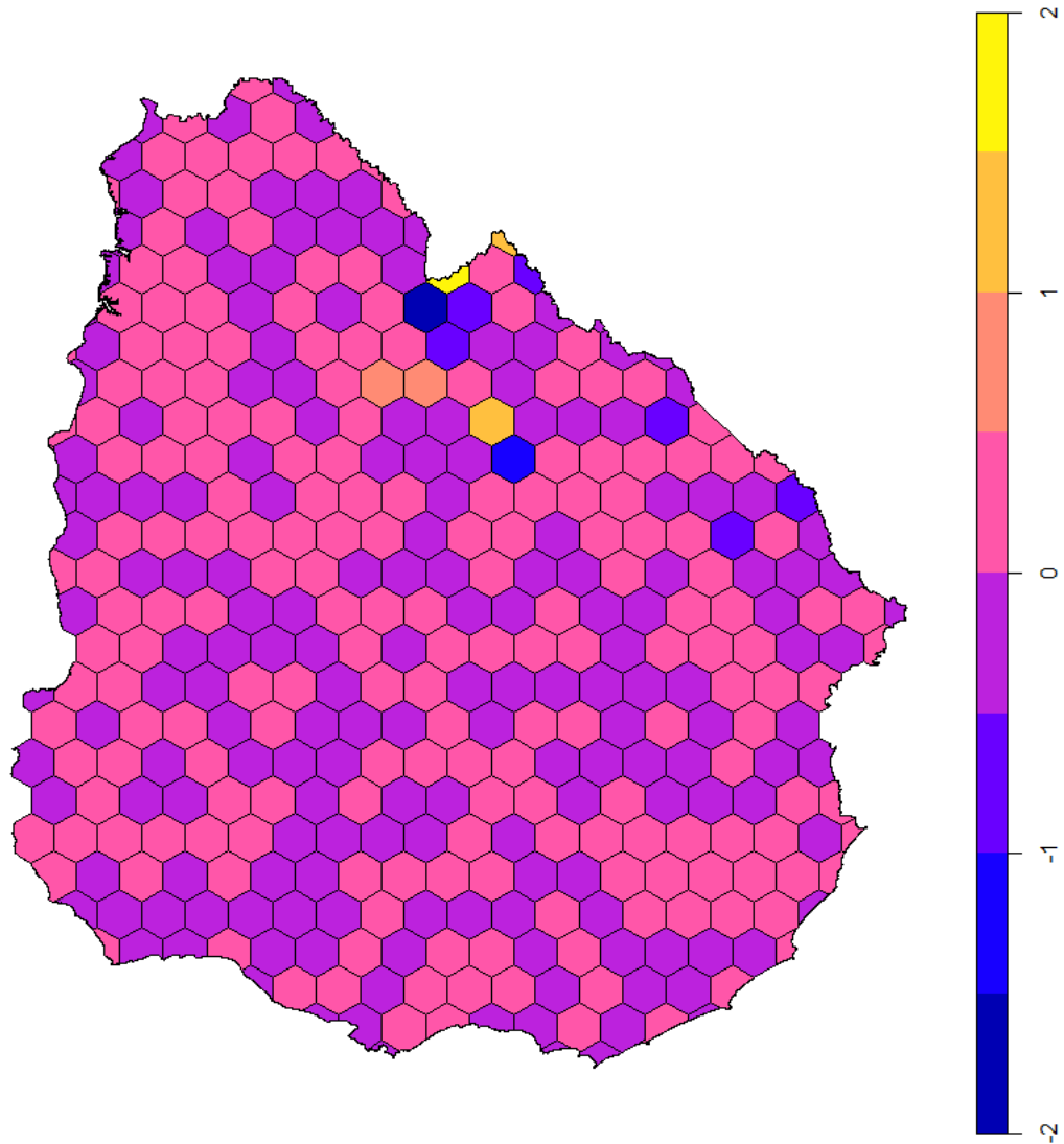
Supplementary Figure S11. Distribution of the residuals from the final Geographically Weighted Regression (GWR): \text{detrended\_residuals} \sim pc.frag1 + c.fnp + c.fpl + temp\_jul . Residuals from the final model showed no significant spatial autocorrelation (Geary's C=1.13 , p\text{-value}=0.99 ).
