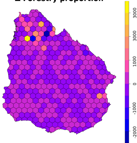
C \Delta Forestry proportion
