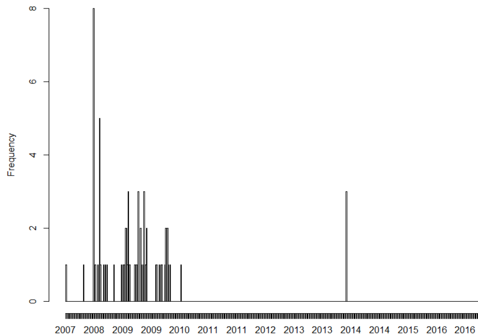
Supplementary Figure S1. Temporal distribution of rabies outbreaks as number of new quarantined ranches per week from 2007 to 2017.
