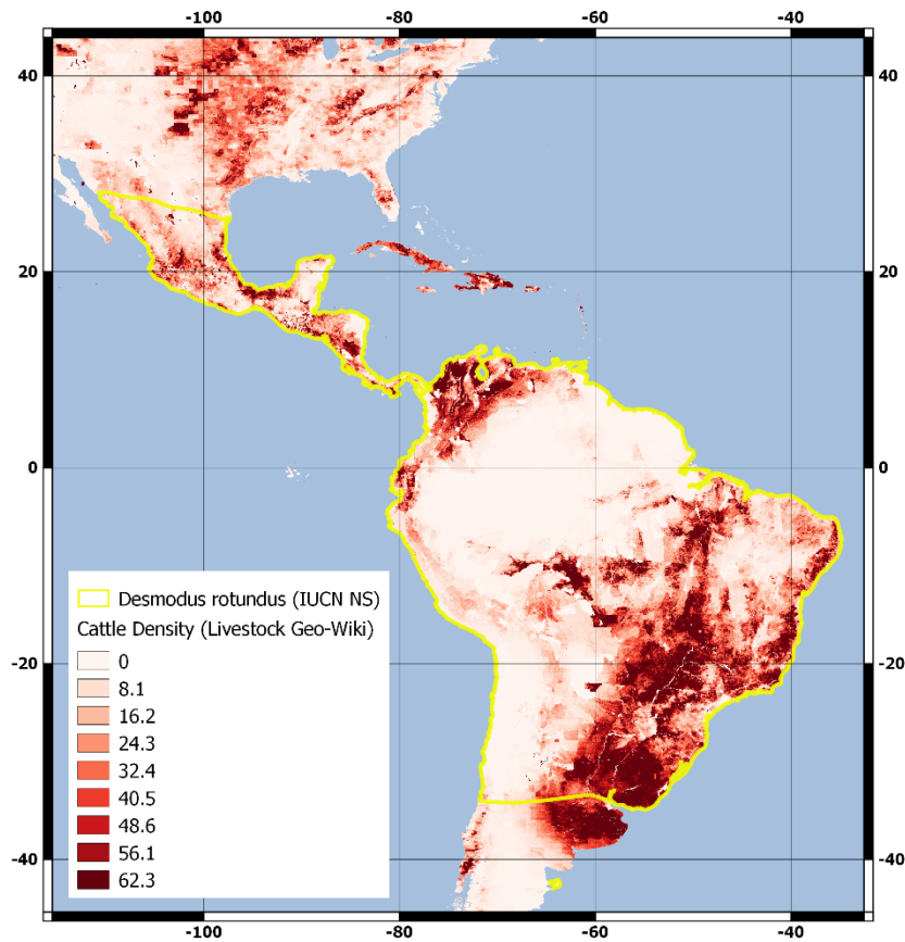
Supplementary Figure S1. Distribution of the common vampire bat ( Desmodus rotundus ) in relation to cattle density. The distribution of D. rotundus is not limited by the absence of food sources. Both in the southern and northern limits, there are areas of high density of cattle outside the area of presence of D. rotundus . The distribution of D. rotundus was obtained from IUCN – Nature Server (Barquez et al. 2015) and the estimated densities of cattle for 2005 (heads of cattle per km 2 ) were obtained from Livestock Geo-Wiki (Robinson et al. 2014). The southernmost record for D. rotundus , in Peninsula Valdés (Chubut Province, Argentina: 42°30' S, 63°56' W), corresponds to only one unconfirmed observation of the species (Barquez et al. 1999).
