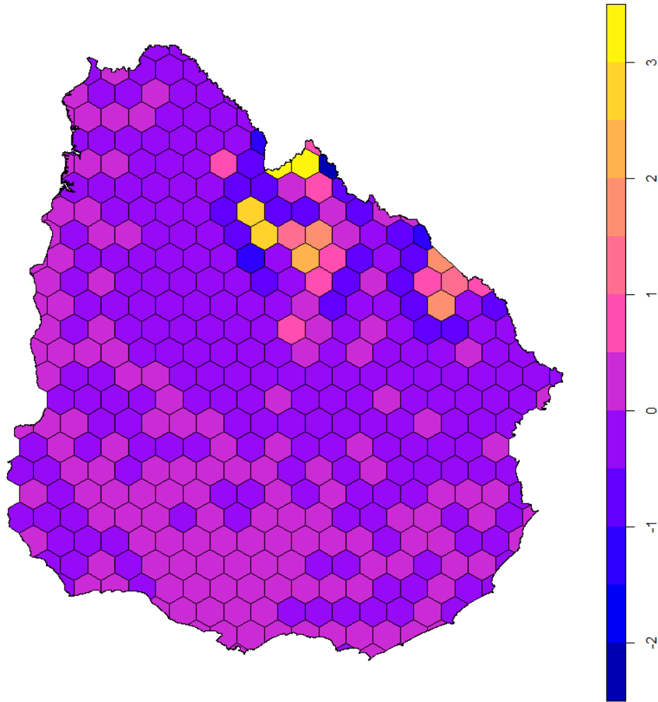
Supplementary Figure S8. Distribution of the residuals from the final Spatial Autoregressive (SAR) Model ( \text{detrended\_residuals} \sim c.fnp * temp\_jul ). The autocorrelation analysis for the residuals, using Geary's C, shows no significant autocorrelation (Geary's C=0.96, p-value=0.15).
