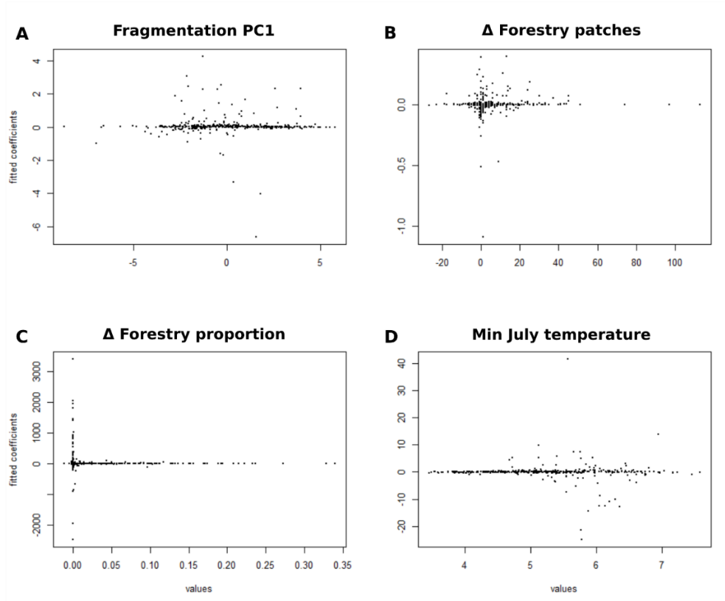
Supplementary Figure S10. Distribution of the fitted coefficient values for the final GWR model ( \text{detrended\_residuals} \sim pc.frag1 + c.fnp + c.fpl + temp\_jul ), in relation to the original values of each variable: A. Fragmentation PC1 ( pc.frag1 ), positive values indicate higher fragmentation of livestock areas B. \Delta forestry patches ( c.fnp ), change in number of exotic forestry patches between 2000 and 2011 C. \Delta forestry proportion ( c.fpl ), change in proportion of landscape covered by exotic forestry between 2000 and 2011 D. Minimum Jul temperature ( temp\_jul ), average minimum temperature of the coldest month.
