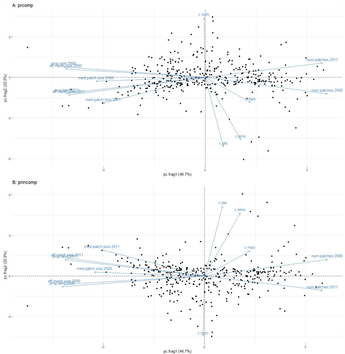
Supplementary Figure S4. Comparison of the results from the Principal Component Analyses using spectral decomposition (function prcomp , panel A) and singular decomposition (function princomp , panel B). Both methods gave similar results, with only inverted loadings on the second principal component.
