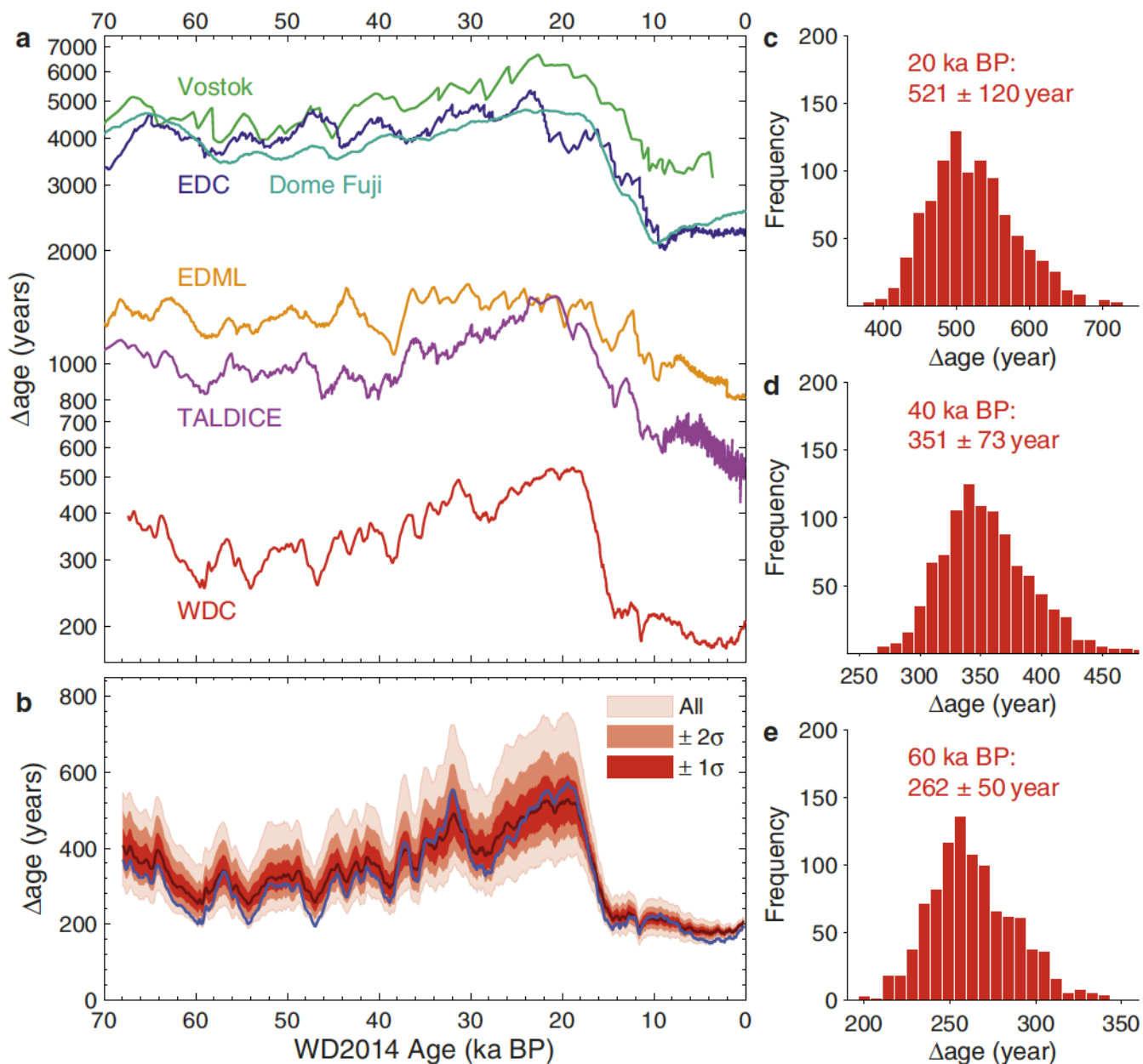
Extended Data Figure 1 | Difference between gas age and ice age ( \Delta age) at WAIS Divide. a, Comparison of WDC \Delta age with other Antarctic cores. Ice core abbreviations: EDC, EPICA Dome Concordia; EDML, EPICA Dronning Maud Land; TALDICE, Talos Dome; WDC, WAIS Divide. \Delta age values are taken from refs 23, 63–65. The vertical axis is on a logarithmic scale. b, \Delta age uncertainty bounds obtained from an ensemble of 1,000 alternative \Delta age
