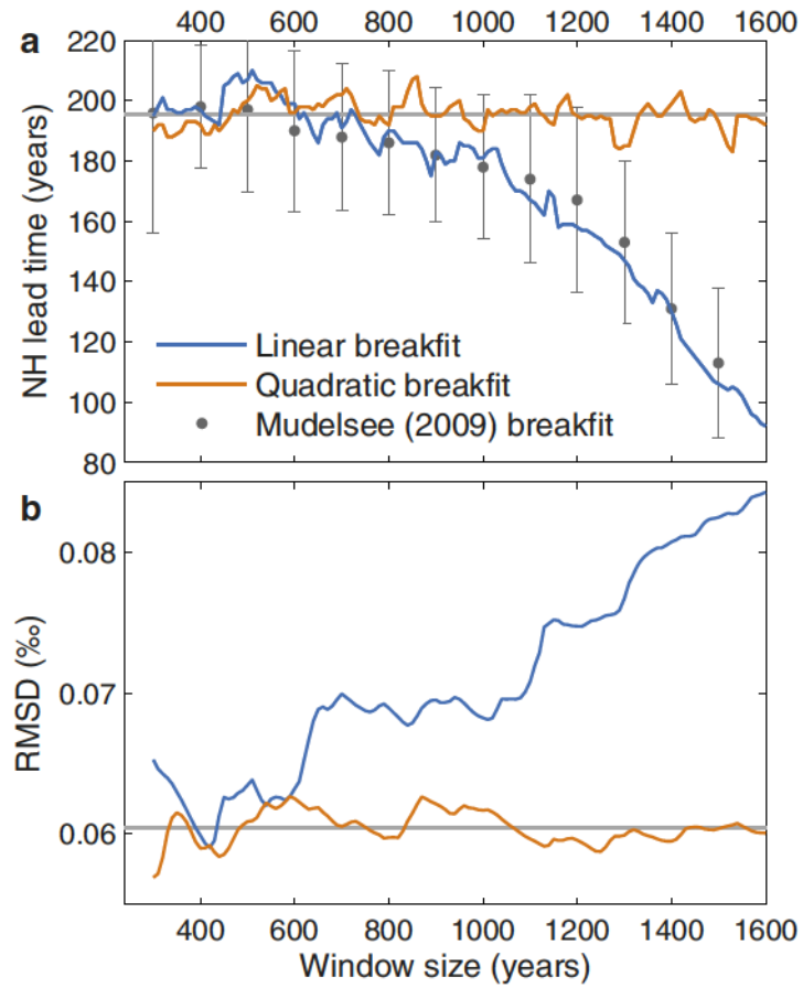
Extended Data Figure 5 | Evaluating the performance of the breakpoint detection algorithm. a, Breakpoint detection as a function of data window size using both linear (blue) and quadratic (orange) functions, compared with the BREAKFIT algorithm 48 (grey dots with 1\sigma error bars). The data window is
