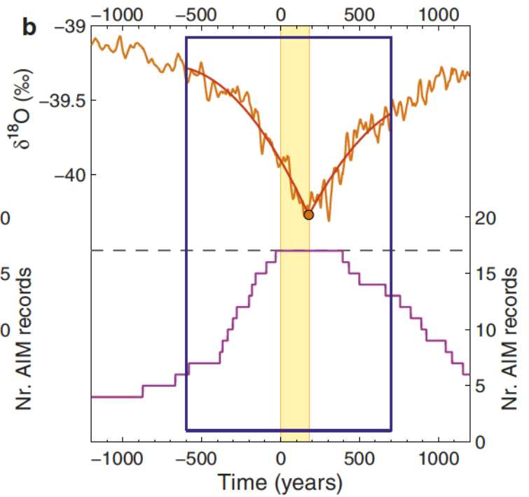
termination) (b). Blue rectangles indicate the time window over which the fitting procedure evaluates the fit to the data (-600 to +700 years); shaded vertical yellow bars show NH lead time.
