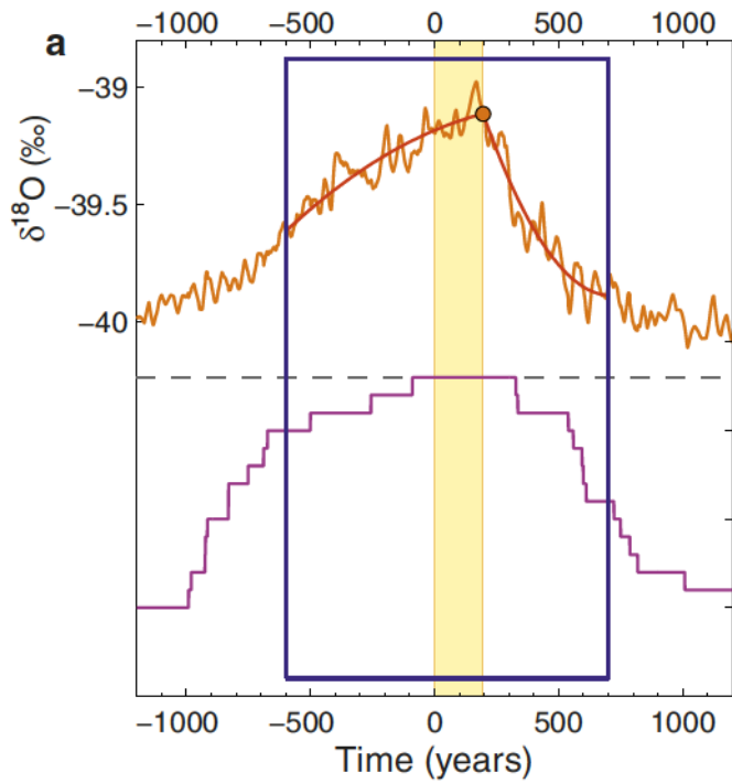
Extended Data Figure 4 | Number of records and fitting procedure. Number of contributory records to the WDC \delta^{18}\text{O} stacks for abrupt NH warming (interstadial onset) (a) and for abrupt NH cooling (interstadial
