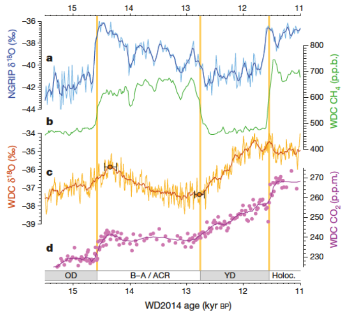
Figure 3 | Timing of the last deglaciation. a, NGRIP \delta^{18}\text{O} on GICC05 chronology 1 . b, WDC \text{CH}_4 . c, WDC \delta^{18}\text{O} with breakpoints as orange dots and error bars showing the 2\sigma uncertainty bounds (Extended Data Table 1). d, WDC \text{CO}_2 data (dots) with spline fit (solid line) 26 . Period abbreviations: OD, Oldest Dryas; B–A, Bølling–Allerød; ACR, Antarctic Cold Reversal; YD, Younger Dryas; Holoc., Holocene. Vertical orange lines correspond to the midpoints of the WDC \text{CH}_4 transitions. NGRIP and WDC chronologies are both based on annual-layer counting, and are fully independent.
