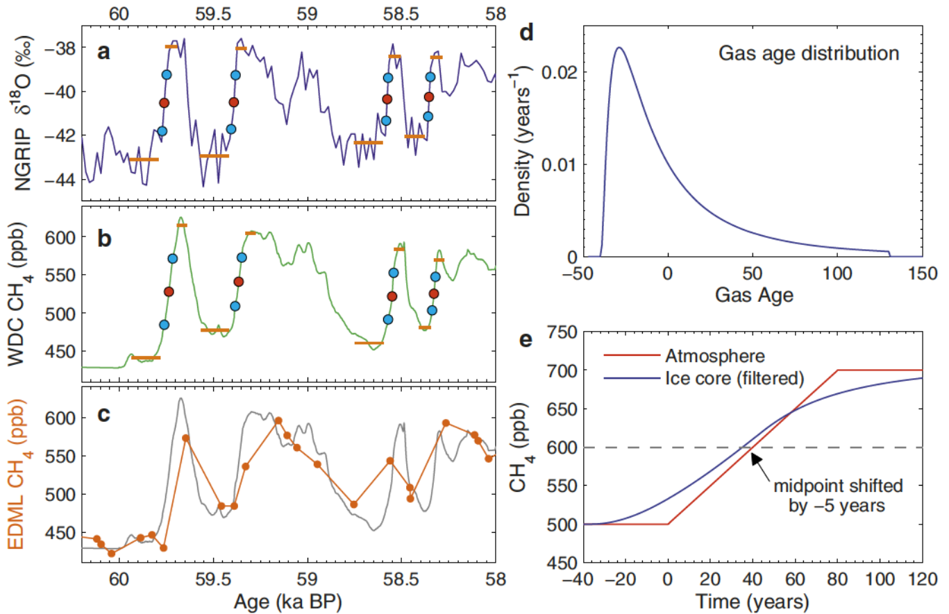
Extended Data Figure 2 | Determining the timing of the abrupt DO transitions. a, b, DO 17.2, 17.1, 16.2 and 16.1 (from oldest to youngest 41 ) as recorded in NGRIP \delta^{18}\text{O} (a) and WDC \text{CH}_4 (b). Horizontal orange bars denote pre-transition and post-transition levels; the transition midpoint (50% of signal amplitude) is indicated by a red dot; the 25% and 75% signal amplitude markers
