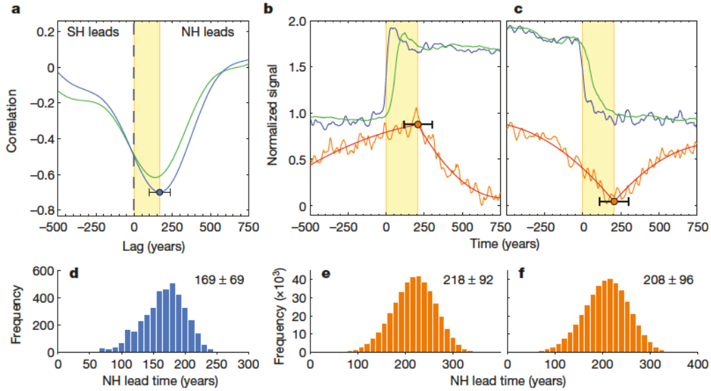
Figure 2 | Interhemispheric phasing of the bipolar seesaw. a, Lagged correlation between NGRIP \delta^{18}\text{O} and WDC d(\delta^{18}\text{O})/dt (blue), and between WDC \text{CH}_4 and d(\delta^{18}\text{O})/dt (green). Millennial-scale variability is isolated by using a fourth-order Butterworth bandpass filter (500–10,000-year window); the \text{CH}_4 -synchronized part of the records is used (31.2–68 kyr). b, DO 3–18 stack of NGRIP \delta^{18}\text{O} (blue), WDC \text{CH}_4 (green) and WDC \delta^{18}\text{O} (orange with curve fit), aligned at the midpoint of the DO warming signal. Events are averaged with their original amplitudes and normalized after stacking for
