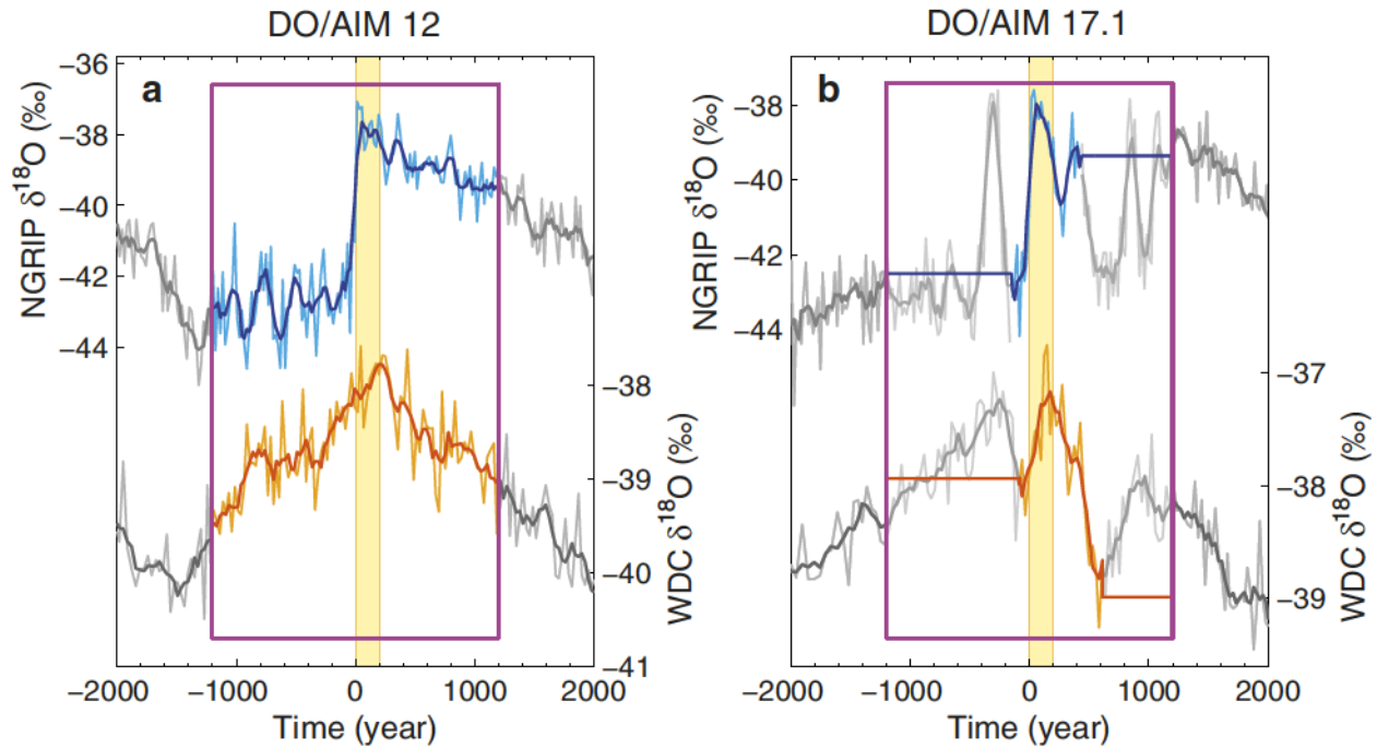
Extended Data Figure 3 | Cropping of individual records in the stack to prevent overlap of events. a , DO/AIM12, where no cropping is needed. b , DO/AIM17.1, where the most cropping is needed. Full time series with five-point running average are plotted in grey, and the contributory records are
