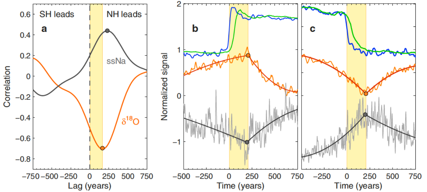
Extended Data Figure 7 | Timing of sea-salt sodium. a, Lagged correlation between NGRIP \delta^{18}\text{O} and the time derivative of WDC \delta^{18}\text{O} (orange), and between NGRIP \delta^{18}\text{O} and the time derivative of WDC ssNa (grey). The dots indicate the maximum (anti-)correlation at 167-year and 229-year NH lead for WDC \delta^{18}\text{O} and ssNa, respectively. A fourth-order Butterworth bandpass filter with a 500–10,000-year window is applied to the time series to isolate the millennial-scale variability. b, DO3–18 stack of NGRIP \delta^{18}\text{O} (blue), WDC \text{CH}_4
