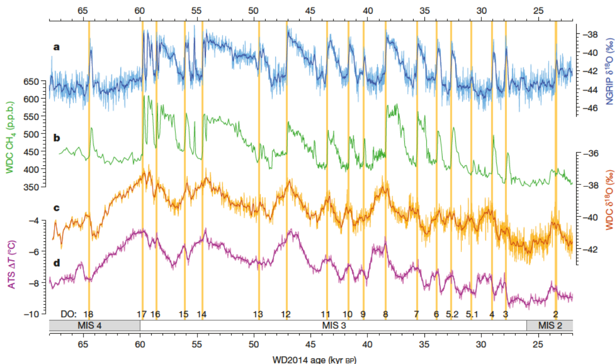
Figure 1 | Records of glacial abrupt millennial-scale climatic variability. a, Greenland NGRIP \delta^{18}\text{O} record 1 on GICC05 \times 1.0063 chronology (Methods). b, WDC discrete \text{CH}_4 record on the WD2014 chronology, which is based on layer counting (0–31.2 kyr) and \text{CH}_4 synchronization to NGRIP
