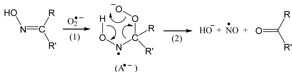
Scheme 2. The proposed mechanism for the oxidative transformation of the \text{C=N-OH} group “outside the active site”.
