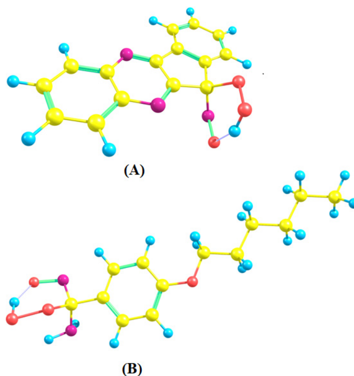
Figure 4. The DFT-optimized geometric structures (gas phase) of the anion–radical adduct A\cdot^- formed from the compounds IQ-1 (Panel A) and AL1 (Panel B) in step (1) (see Scheme 2). The carbon, hydrogen, nitrogen, and oxygen atoms are shown as yellow, light-blue, magenta, and red balls, respectively.
