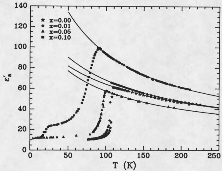
Figure 14. Temperature dependence of the real part of the dielectric constant \epsilon'_a measured along the a axis for various ammonium concentrations x in RADA. Solid line represents a fit to Eq. (5.1); see Table 1 for fitting constants.
