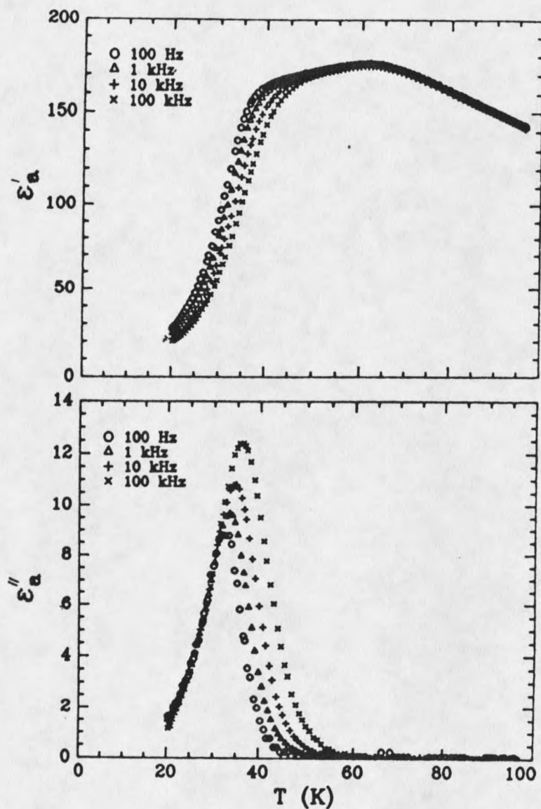
Figure 22. Temperature dependence of the (a) real part \epsilon'_a and (b) imaginary part \epsilon''_a of the dielectric permittivity measured along the a axis in the proton glass regime for x=0.40 RADA.
