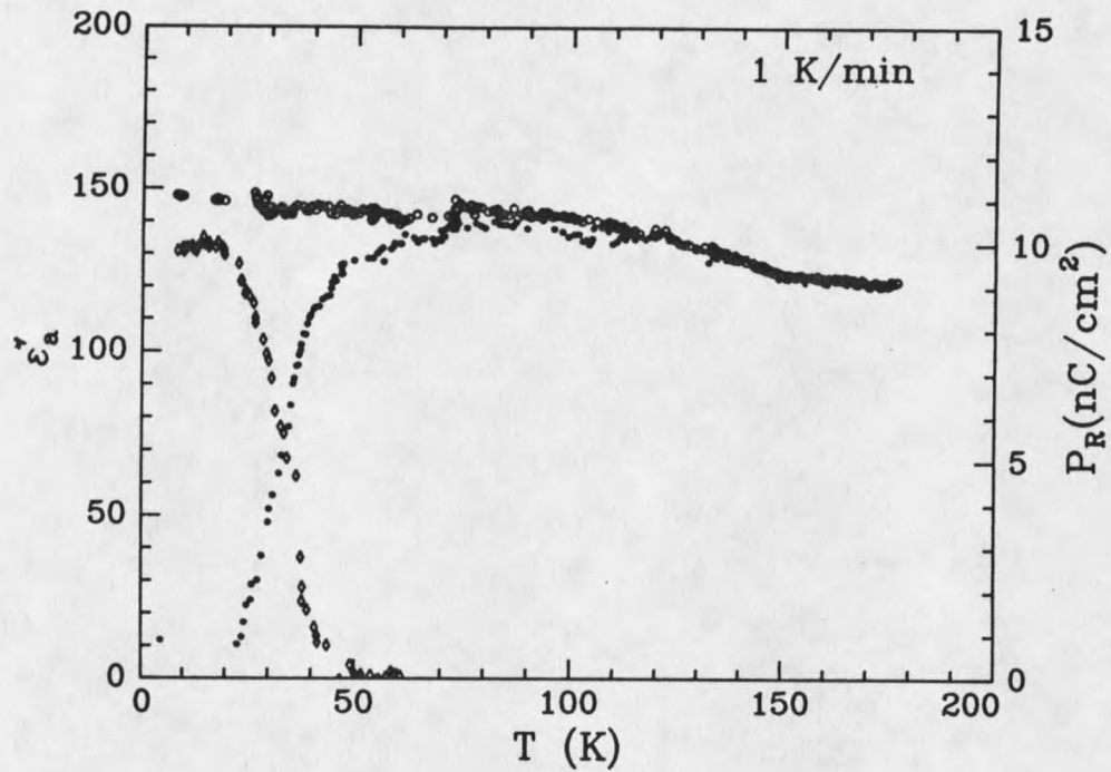
Figure 30. Temperature dependence of the field-cooled ( \circ ) and zero-field-cooled ( \bullet ) static dielectric constant (left scale) of DRADA with x=0.28 measured along the \underline{a} axis. The remanent polarization P_R ( \diamond ) is also shown (right scale). The electric field applied was 500 V/cm and the heating/cooling rate was 1 K/min.
