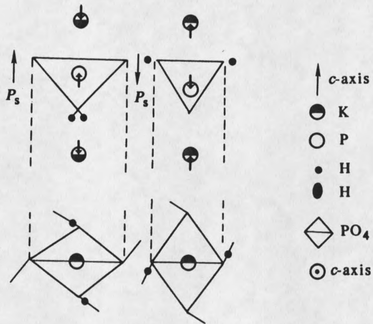
Figure 4. Schematic representation of the dipole moment in KDP. Polarization along the \underline{c} axis. [5]
