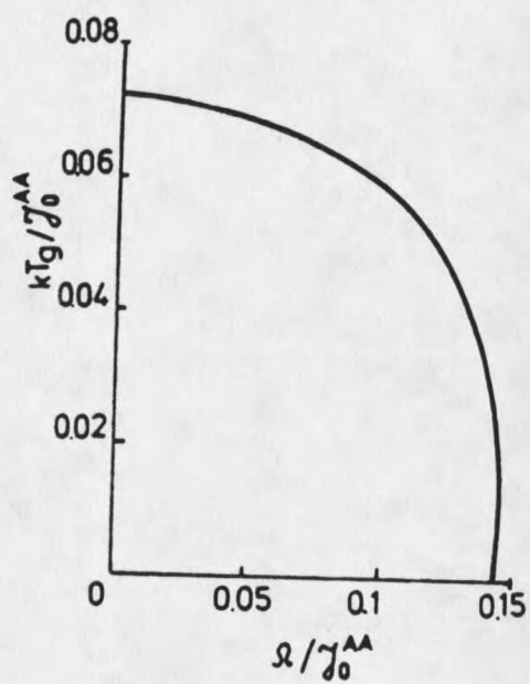
Figure 11. Transition temperature T_g , versus the ratio \Omega/J_0^{AA} for x_A = x_B = 0.5 .
