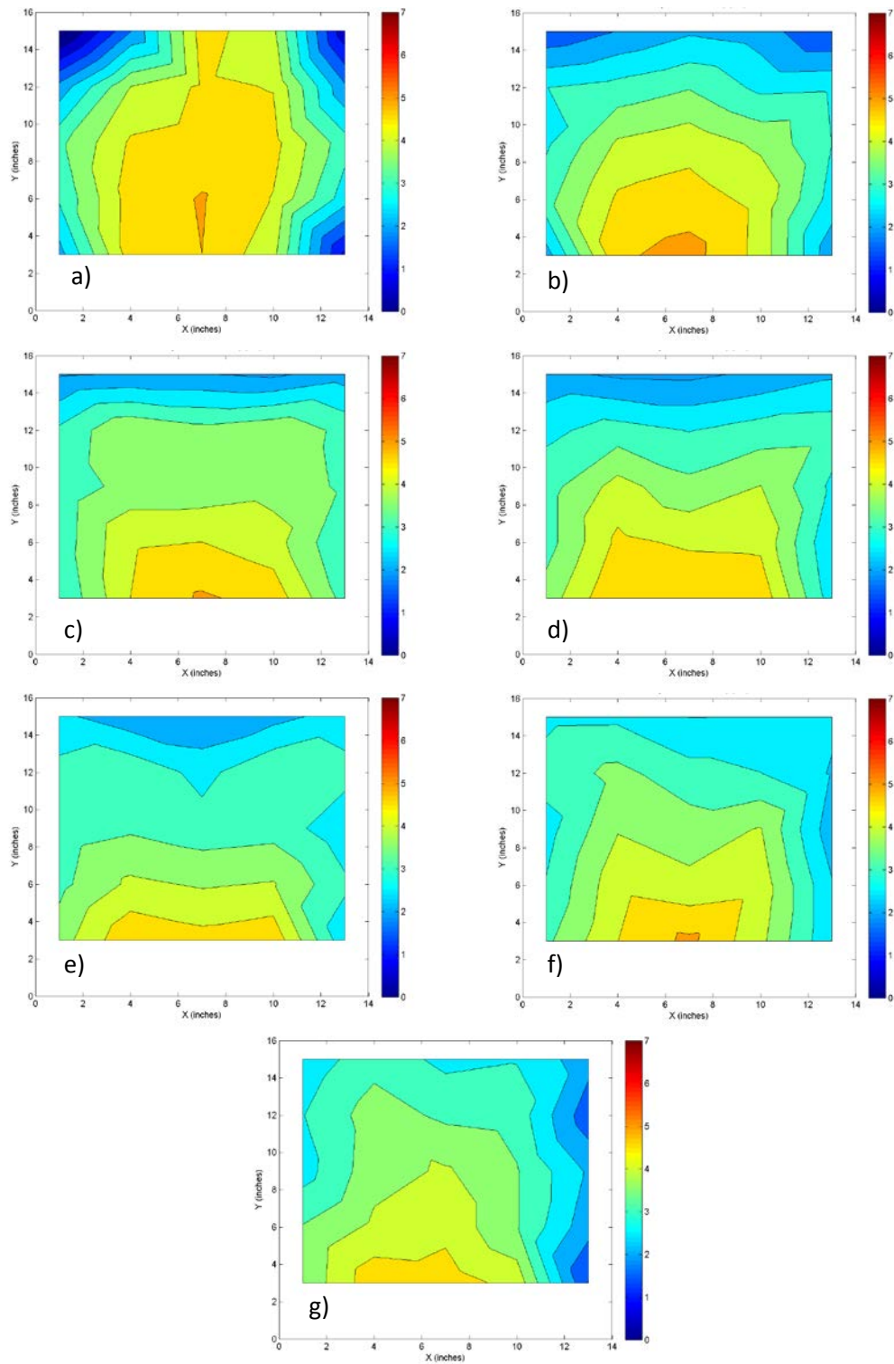
Figure 10: ECM velocity for low head and steep slope at sections a) 23, b) 73, c) 123, d) 163, e) 203, f) 248, and g) 294 inches from the inlet, units are feet per second.
