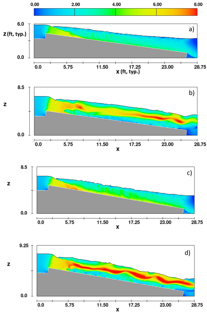
Figure 28: Velocity distribution at longitudinal centerline at 30 seconds of simulation time for a) low head, shallow slope, b) high head, shallow slope, c) low head steep slope, d) high head, steep slope, units are in feet per second.
