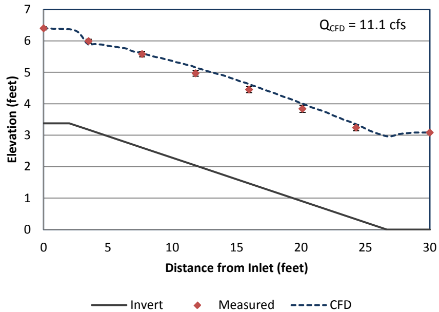
Figure 13: CFD model and observed water surface elevation for the time-averaged water surface profile at the centerline of the fishway for high head and shallow slope. Error bars represent the standard deviation.
