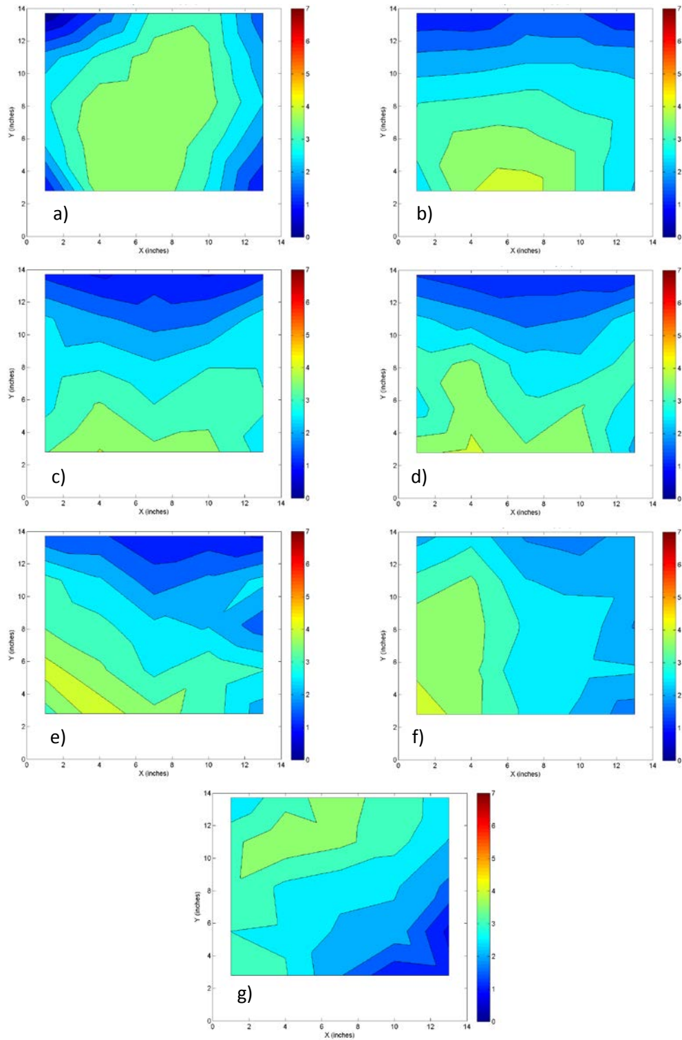
Figure 8: ECM velocity for low head and shallow slope at sections a) 23, b) 73, c) 123, d) 163, e) 203, f) 248, and g) 294 inches from the inlet, units are feet per second.
