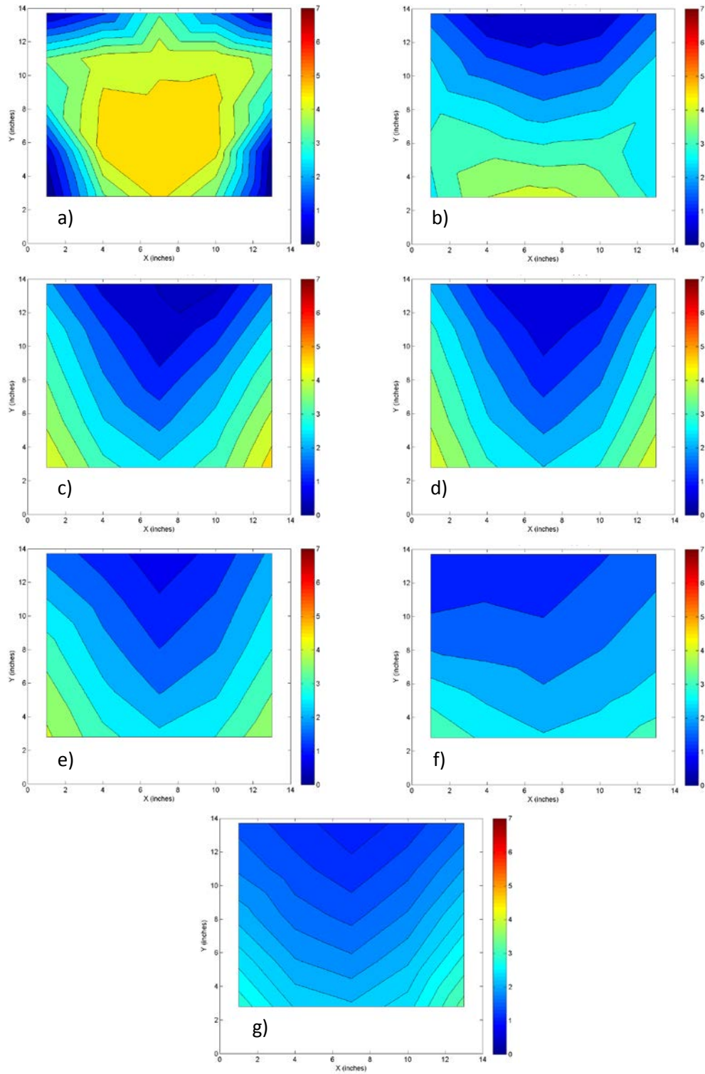
Figure 24: CFD model results for velocity for low head and shallow slope at sections a) 23, b) 73, c) 123, d) 163, e) 203, f) 248, and g) 294 inches from the inlet, units are in feet per second.
