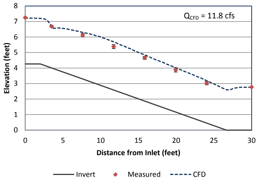
Figure 15: CFD model and observed water surface elevation for the time-averaged water surface profile at the centerline of the fishway for high head and steep slope. Error bars represent the standard deviation.
