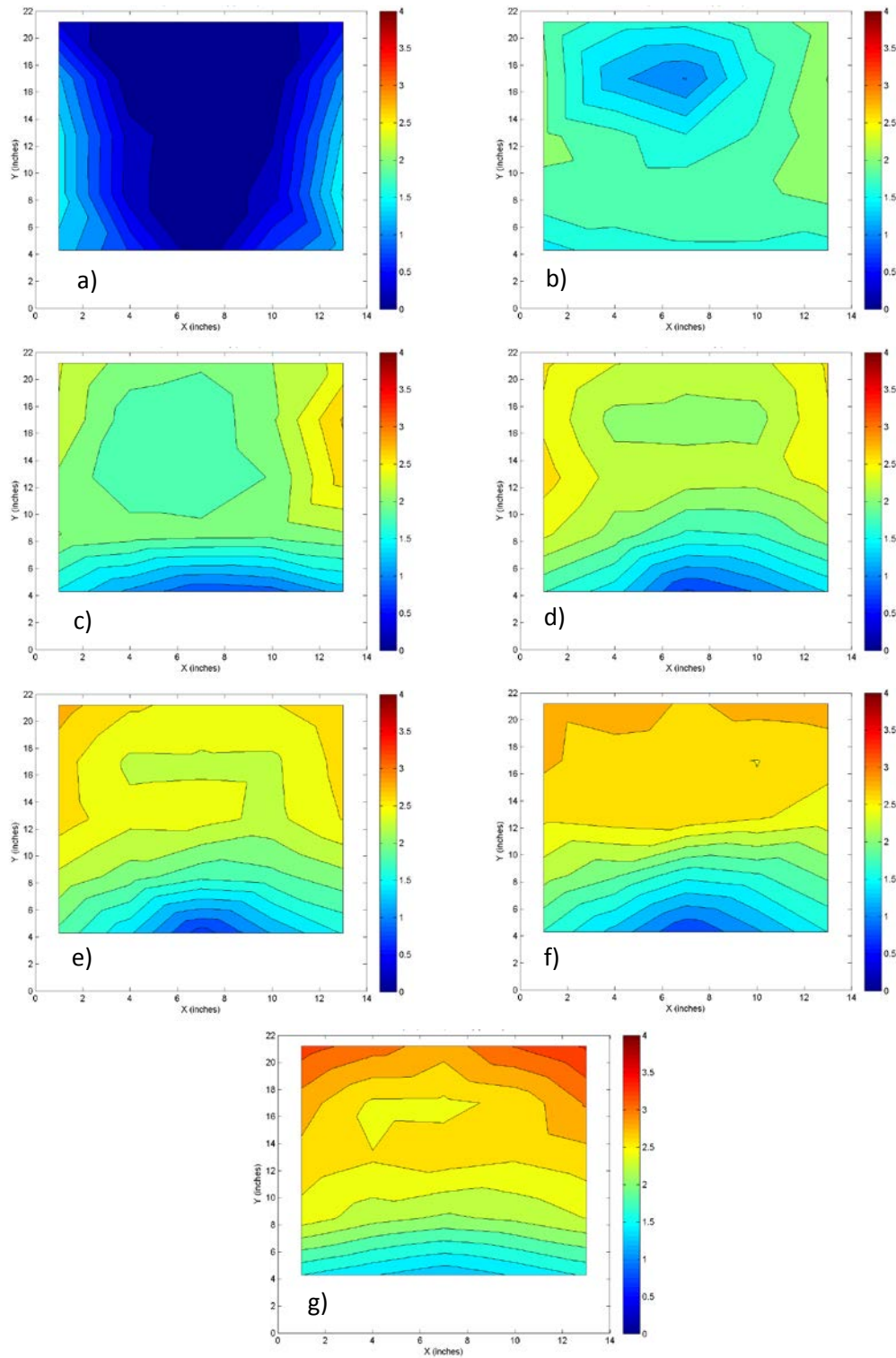
Figure 30: CFD model results for turbulent kinetic energy for high head and shallow slope at sections a) 23, b) 73, c) 123, d) 163, e) 203, f) 248, and g) 294 inches from the inlet, units are in foot pound-force.
