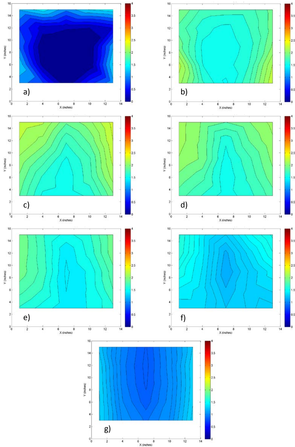
Figure 31: CFD model results for turbulent kinetic energy for low head and steep slope at sections a) 23, b) 73, c) 123, d) 163, e) 203, f) 248, and g) 294 inches from the inlet, units are in foot pound-force.
