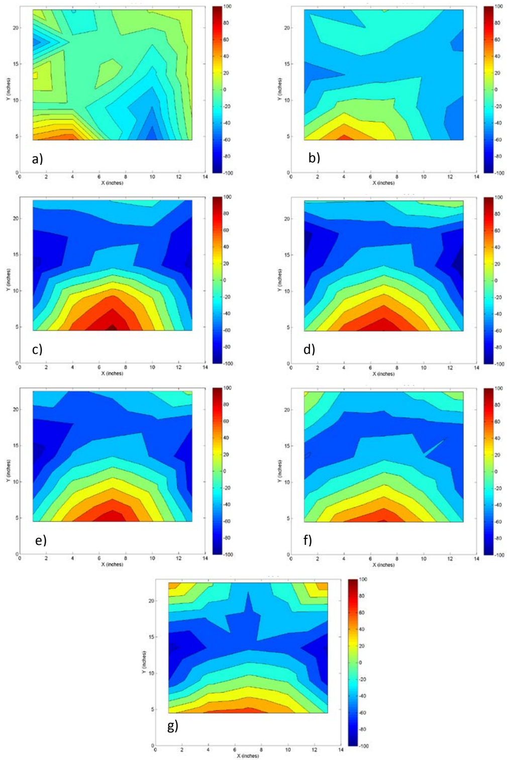
Figure 19: Percentage error between ECM and CFD velocities for high head and steep slope at sections a) 23, b) 73, c) 123, d) 163, e) 203, f) 248, and g) 294 inches from the inlet, units are percent.
