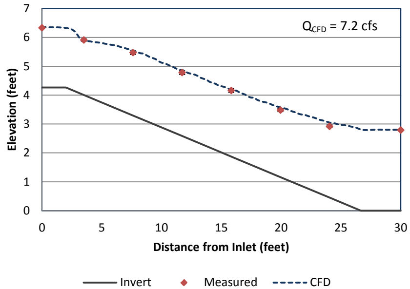
Figure 14: CFD model and observed water surface elevation for the time-averaged water surface profile at the centerline of the fishway for low head and steep slope. Error bars represent the standard deviation.
