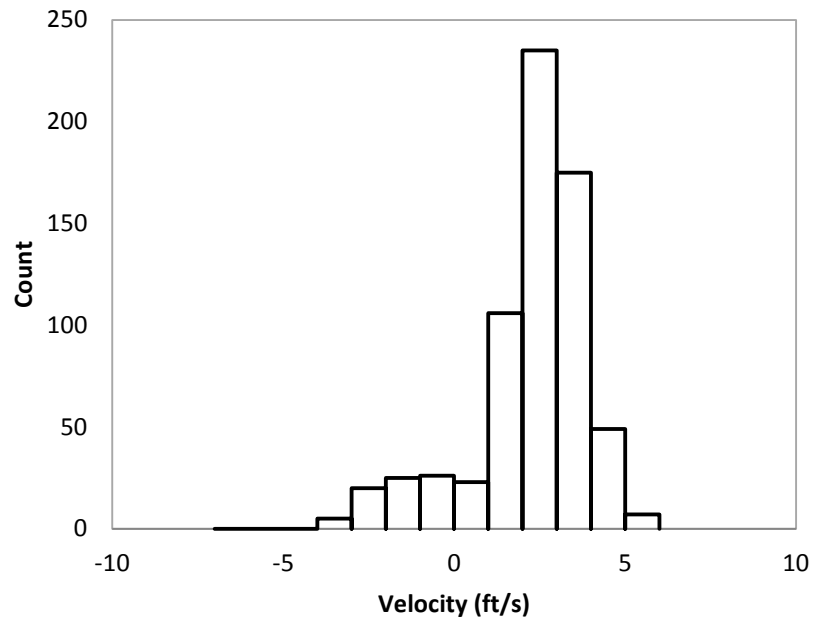
Figure 55: Filtered velocity data distribution at a point in section 73.
