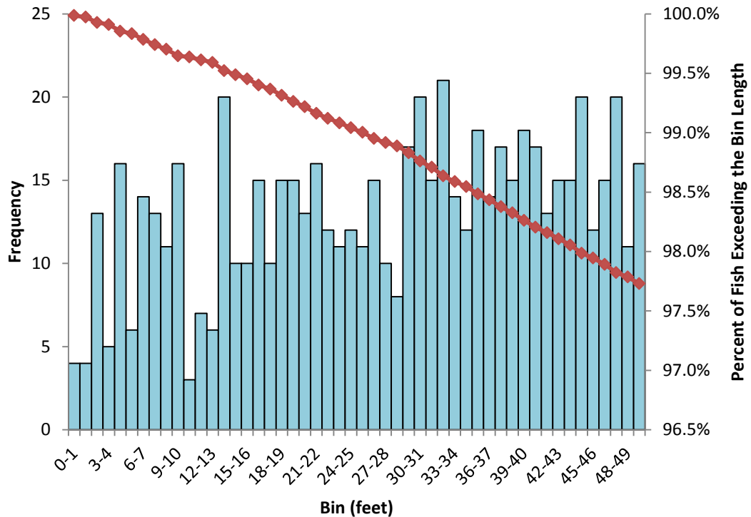
Figure 48: Histogram relating passage success to the length of a conceptual infinitely long steepass fishway using fine bin sizes to examine shorter fishway lengths for the high head, shallow slope hydraulic condition.
