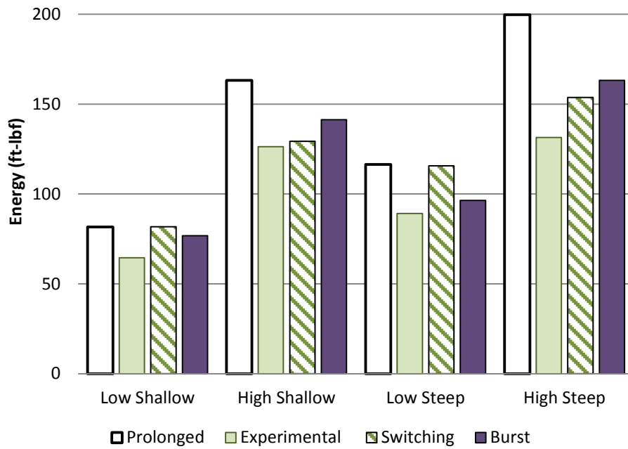
Figure 44: Average energy expenditure (feet pound-force) for all models for the low velocity tendency and high velocity tendency path algorithms.
