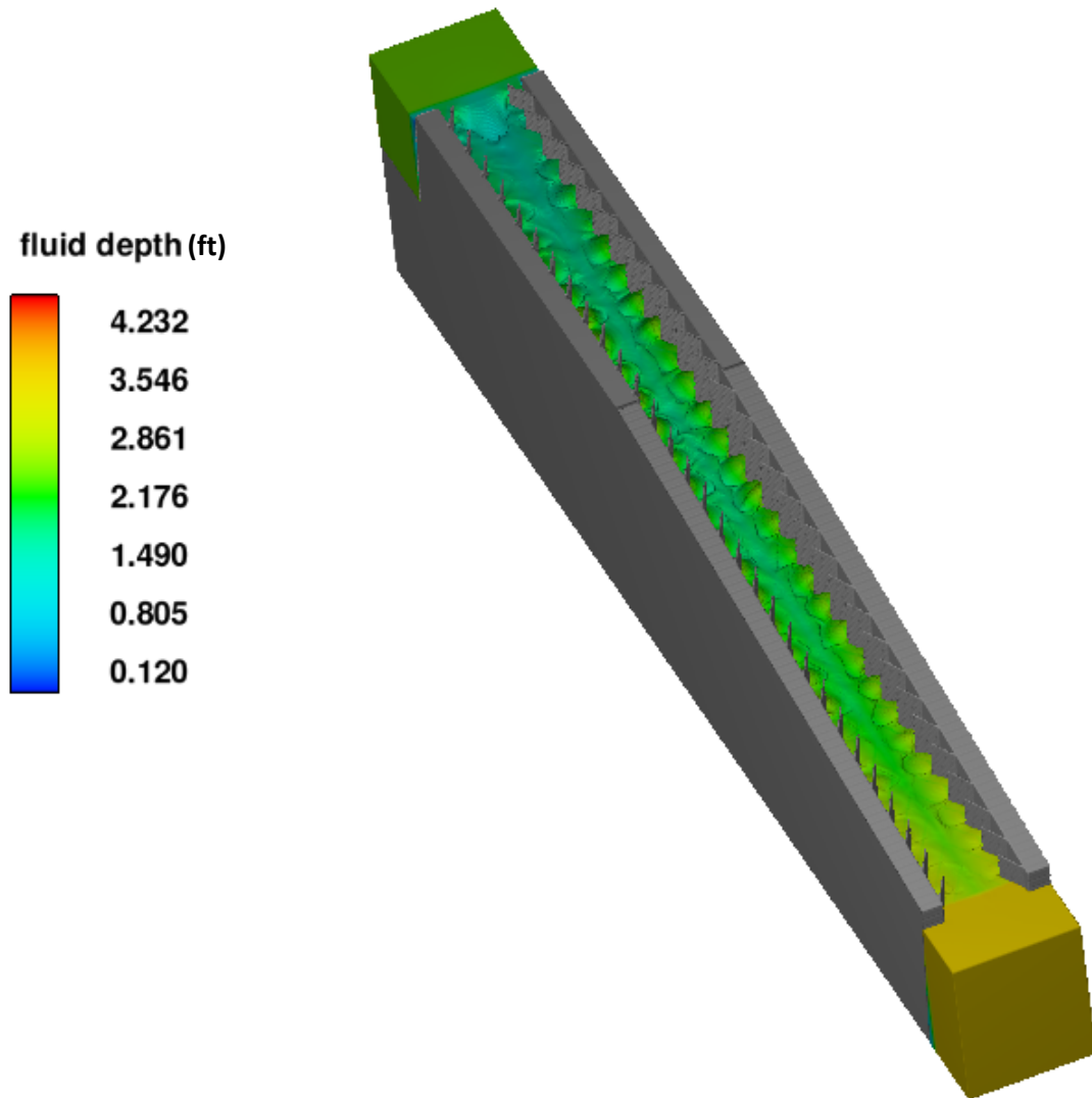
Figure 23: CFD model results for water surface of the fishway for low head and shallow slope at 35 seconds model time, color shading indicates fluid depth in feet.
