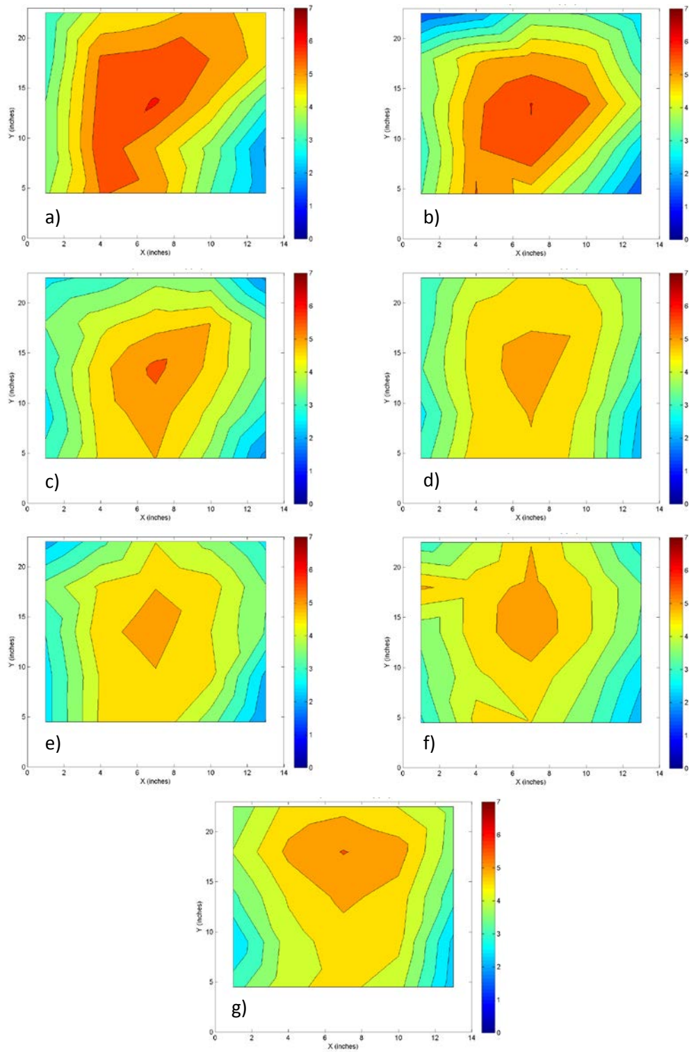
Figure 11: ECM velocity for high head and steep slope at sections a) 23, b) 73, c) 123, d) 163, e) 203, f) 248, and g) 294 inches from the inlet, units are feet per second.
