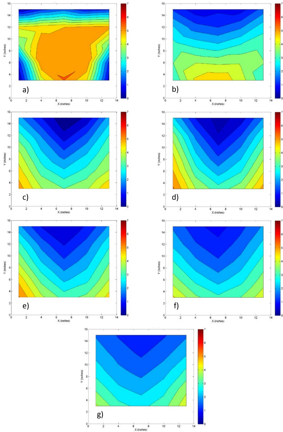
Figure 26: CFD model results for velocity for low head and steep slope at sections a) 23, b) 73, c) 123, d) 163, e) 203, f) 248, and g) 294 inches from the inlet, units are in feet per second.
