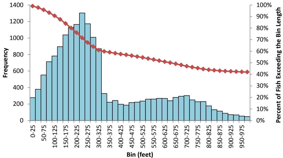
Figure 47: Histogram relating passage success to the length of a conceptual infinitely long steppass fishway using coarse bins for the high head, shallow slope hydraulic condition.
