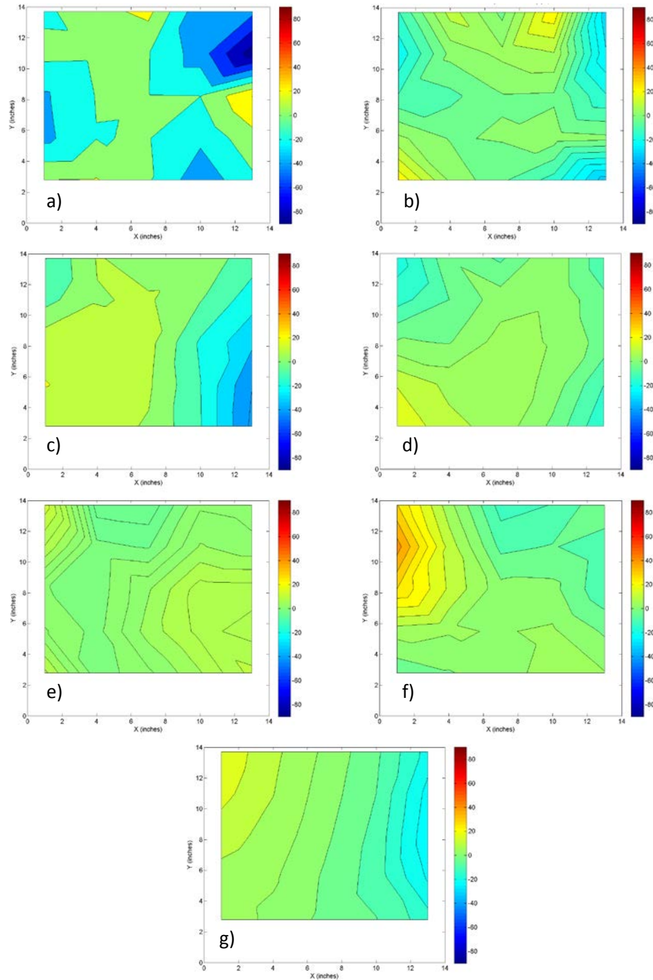
Figure 6: The relative error in the downstream component of the CFD-predicted velocity between models having fine and coarse grids for a low head and shallow sloped fishway at sections a) 23, b) 73, c) 123, d) 163, e) 203, f) 248, and g) 294 inch from the inlet (units are percent).
