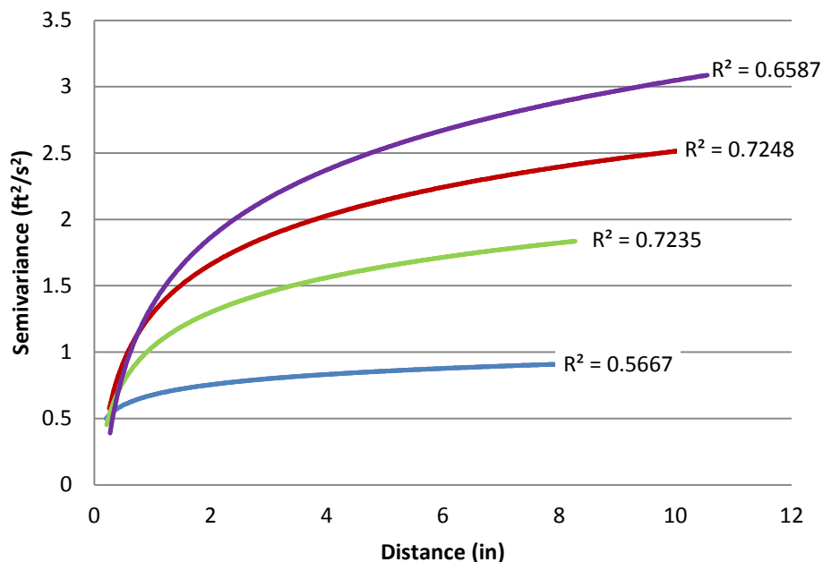
Figure 21: Semivariogram of velocity residuals in the y-z direction for low shallow (blue), low steep (green), high shallow (red), and high steep (purple) simulations (lines are referenced from bottom to top).
