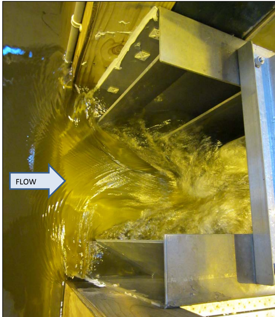
Figure 22: Water surface drawdown at the entrance to a steep pass fishway (low head, shallow slope).
