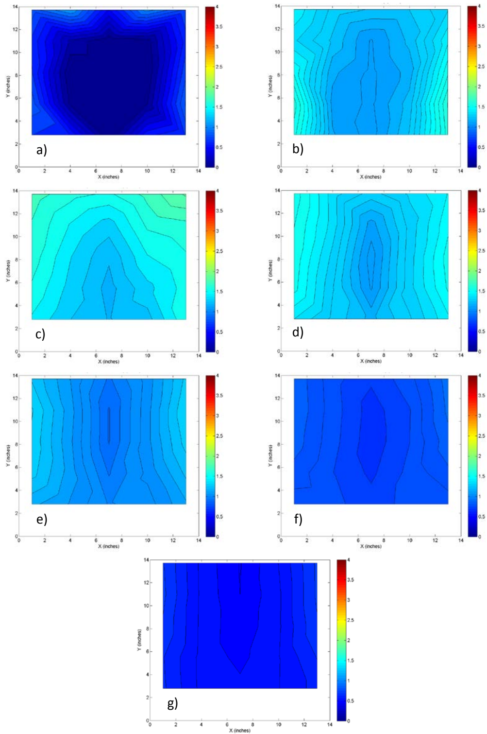
Figure 29: CFD model results for turbulent kinetic energy for low head and shallow slope at sections a) 23, b) 73, c) 123, d) 163, e) 203, f) 248, and g) 294 inches from the inlet, units are in foot pound-force.
