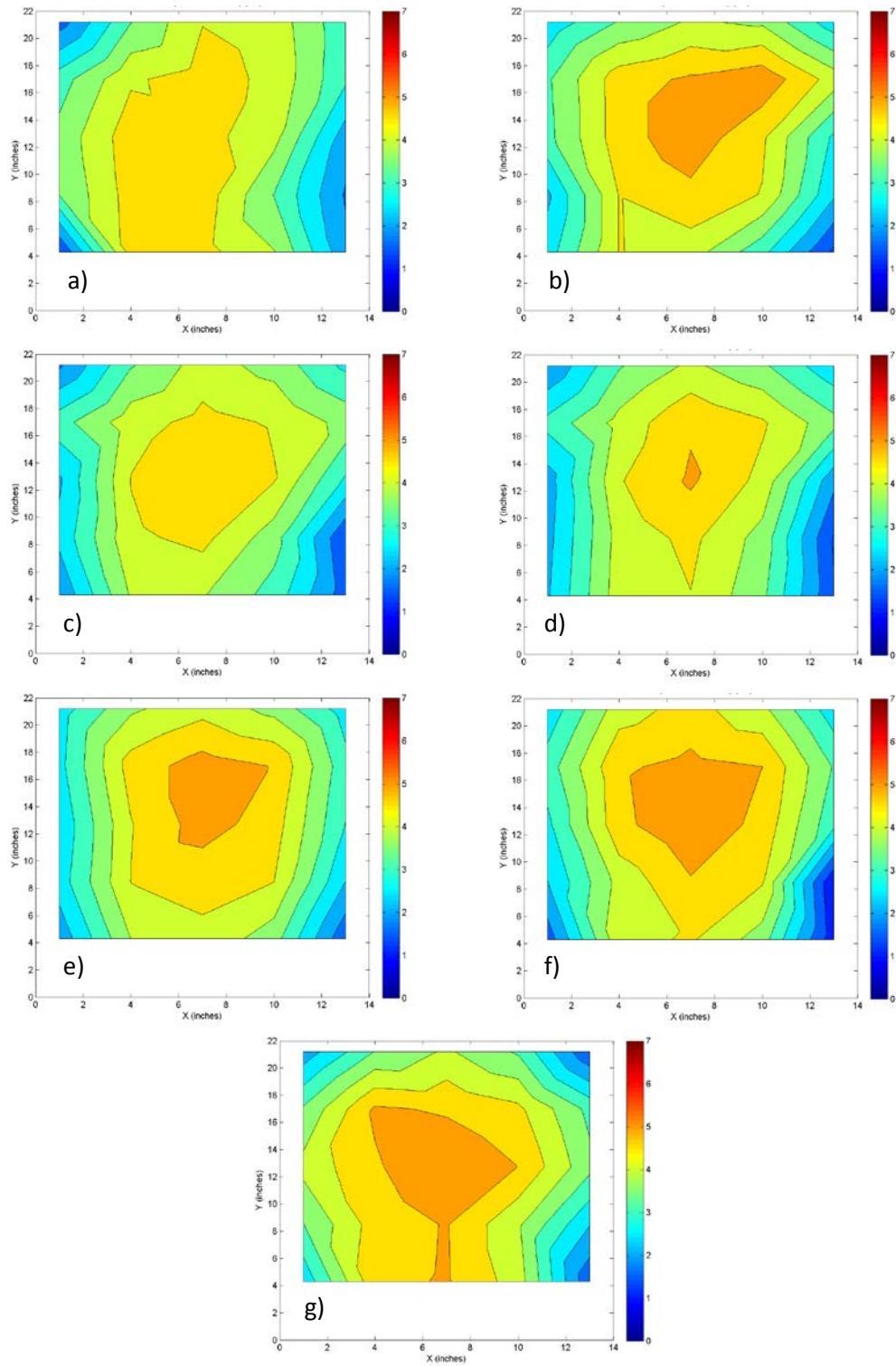
Figure 9: ECM velocity for high head and shallow slope at sections a) 23, b) 73, c) 123, d) 163, e) 203, f) 248, and g) 294 inches from the inlet, units are feet per second.
