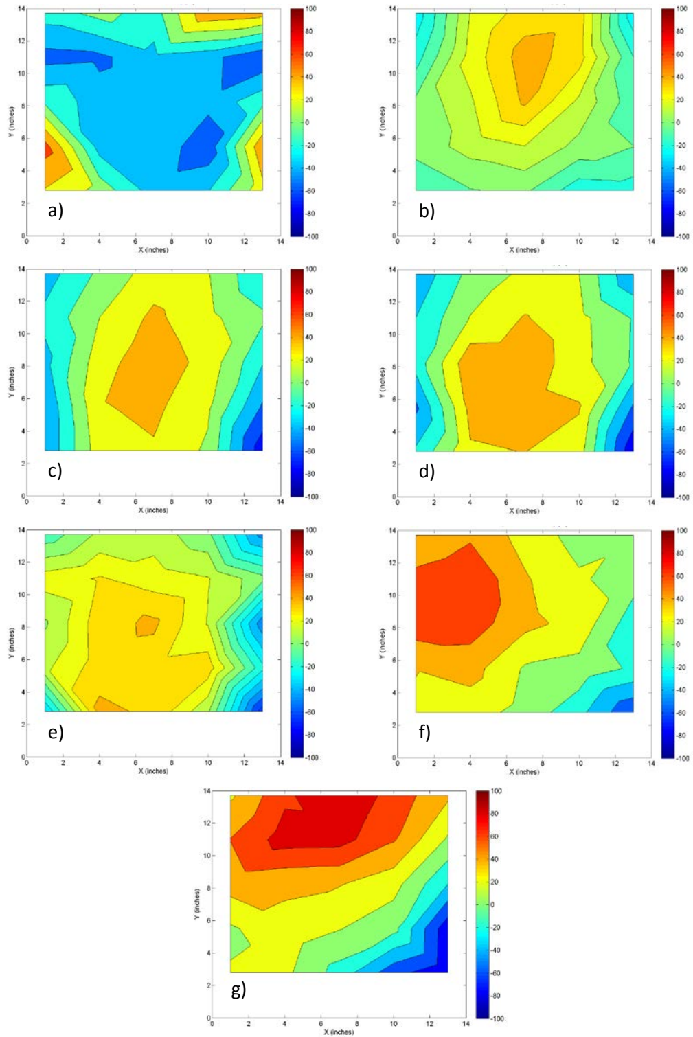
Figure 16: Percentage error between ECM and CFD velocities for low head and shallow slope at sections a) 23, b) 73, c) 123, d) 163, e) 203, f) 248, and g) 294 inches from the inlet, units are percent.
