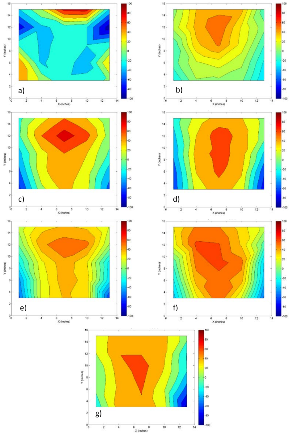
Figure 18: Percentage error between ECM and CFD velocities for low head and steep slope at sections a) 23, b) 73, c) 123, d) 163, e) 203, f) 248, and g) 294 inches from the inlet, units are percent.
