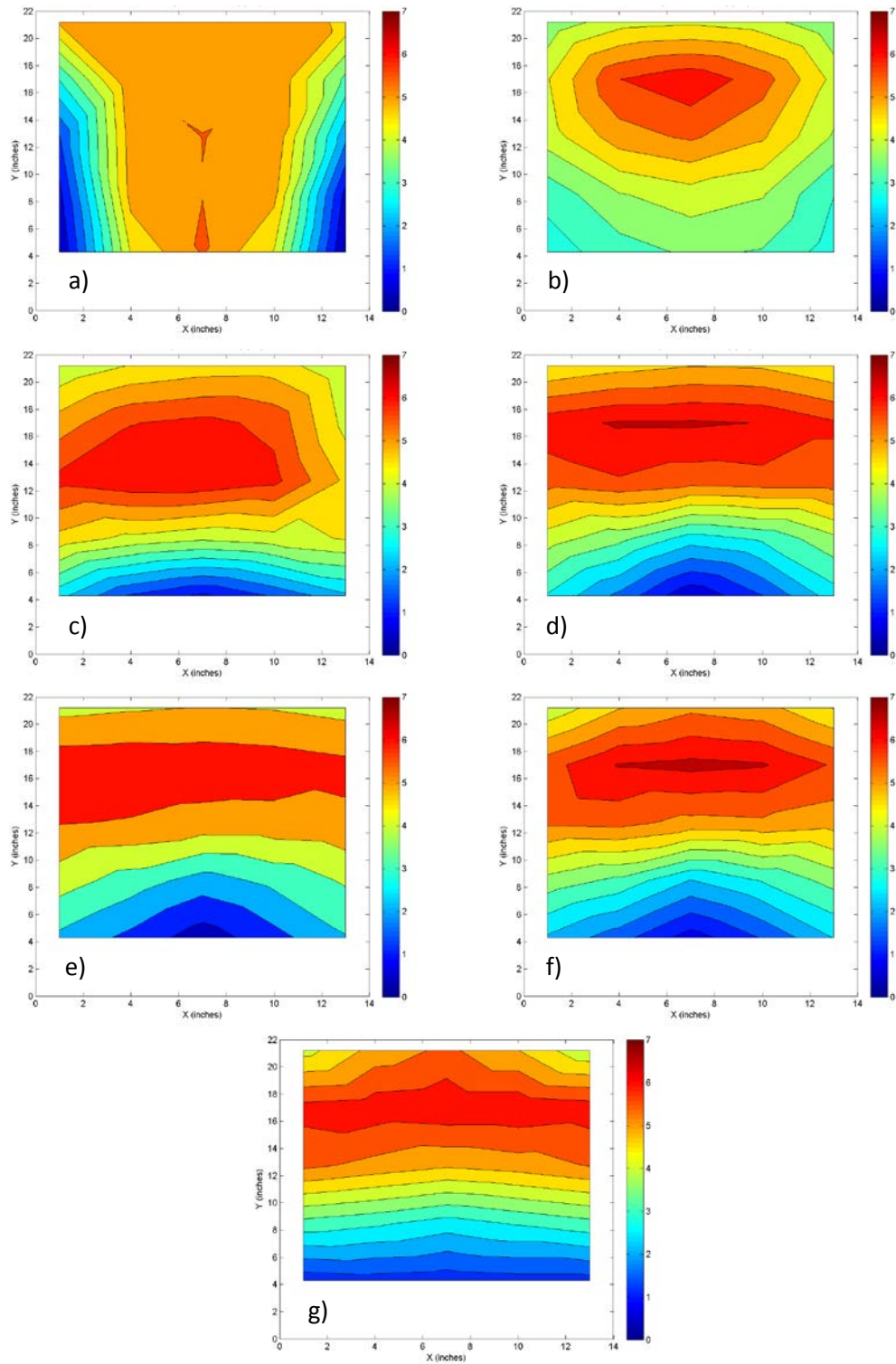
Figure 25: CFD model results for velocity for high head and shallow slope at sections a) 23, b) 73, c) 123, d) 163, e) 203, f) 248, and g) 294 inches from the inlet, units are in feet per second.
