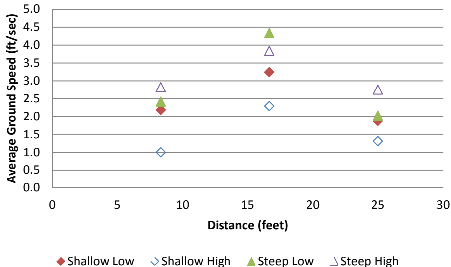
Figure 34: Variation in groundspeed for American shad in a steep pass fishway.
