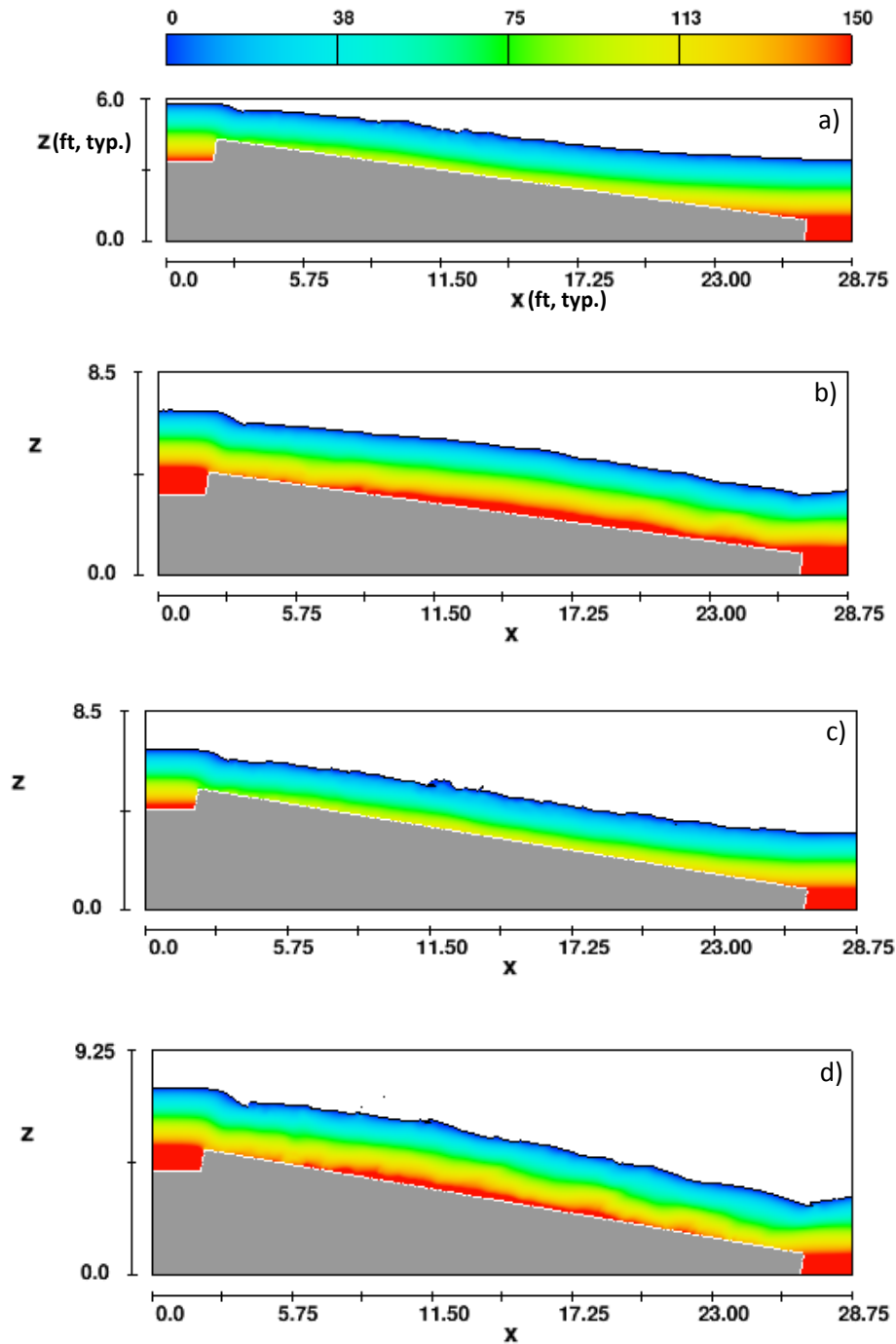
Figure 35: Pressure distribution at longitudinal centerline at 30 seconds of simulation time for a) low head, shallow slope, b) high head, shallow slope, c) low head steep slope, d) high head, steep slope, units are pound-force/square foot.
