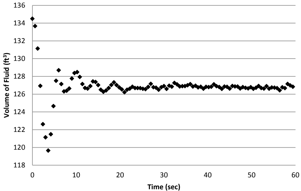
Figure 4: CFD model output for the low head shallow slope condition which illustrates stationarity in the volume of fluid being reached at about 20 seconds of simulation time.
