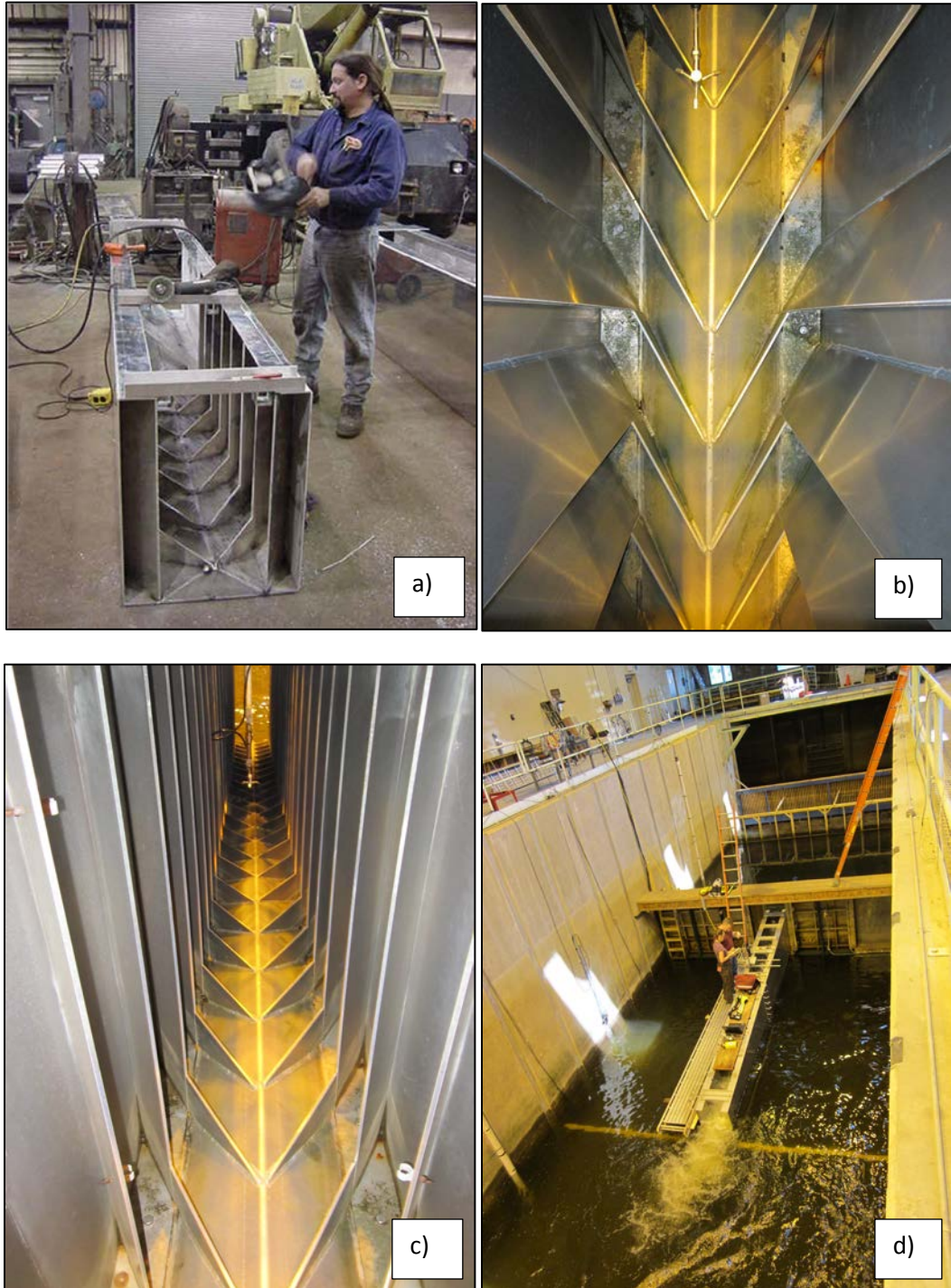
Figure 1: a) Fabrication of a steppass fishway. b) Interior of a steppass fishway looking down from overhead. c) Interior of steppass fishway looking downstream with ADV device in background. d) Installation of a steppass fishway at the Conte Lab. Photo Credit: USFWS
