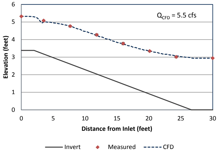
Figure 12: CFD model and observed water surface elevation for the time-averaged water surface profile at the centerline of the fishway for low head and shallow slope. Error bars represent the standard deviation.
