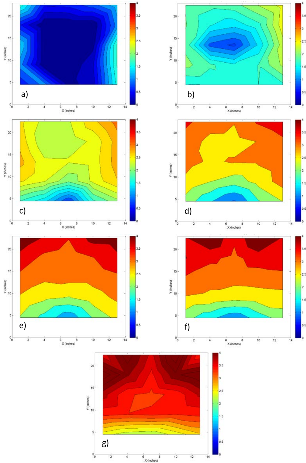
Figure 32: CFD model results for turbulent kinetic energy for high head and steep slope at sections a) 23, b) 73, c) 123, d) 163, e) 203, f) 248, and g) 294 inches from the inlet, units are in foot pound-force.
