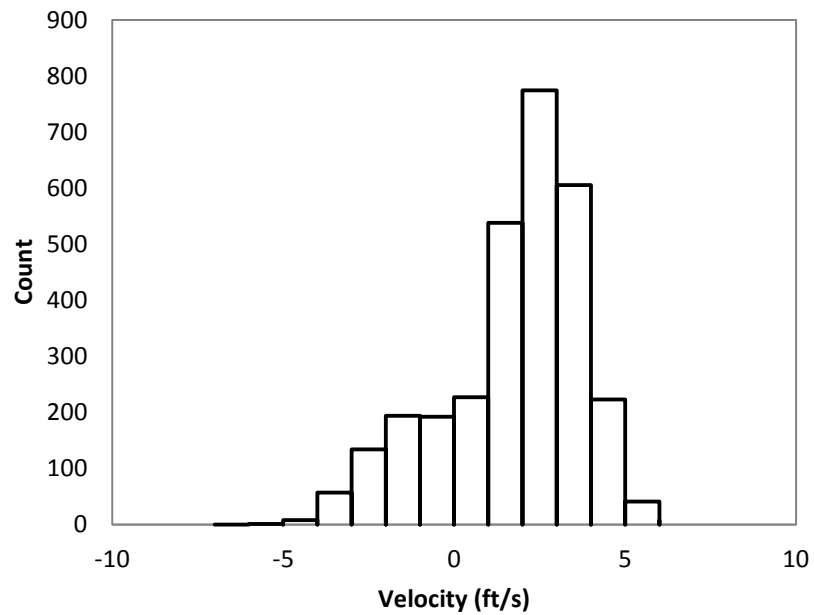
Figure 53: Unfiltered velocity data distribution at a point in section 73.
