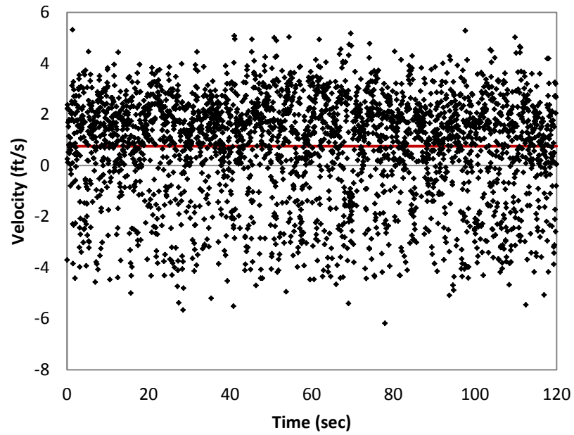
Figure 52: Unfiltered time series velocity data at a point in section 73. The red (bold) horizontal line indicates the mean value for the velocity.
