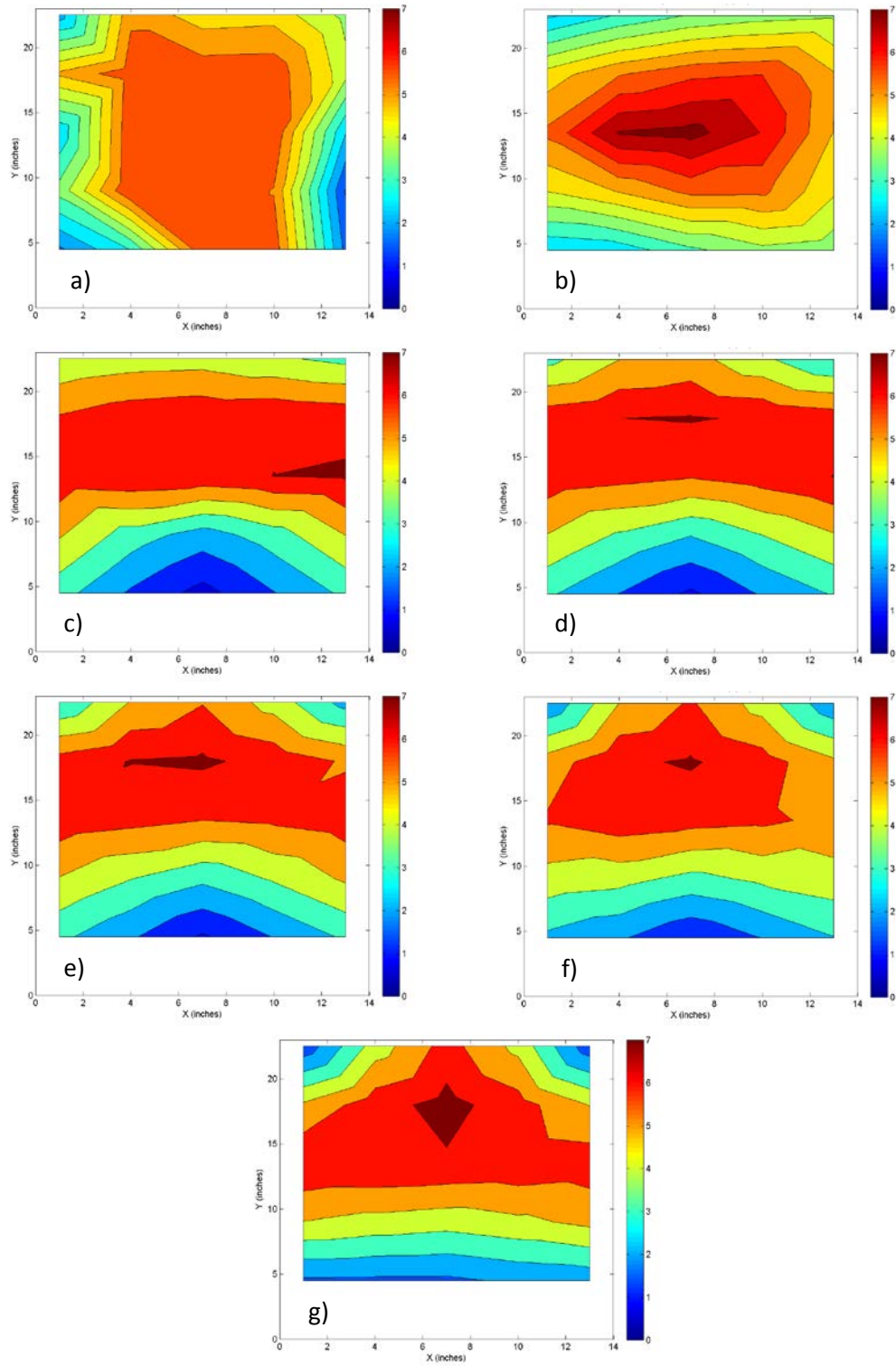
Figure 27: CFD model results for velocity for high head and steep slope at sections a) 23, b) 73, c) 123, d) 163, e) 203, f) 248, and g) 294 inches from the inlet, units are in feet per second.
