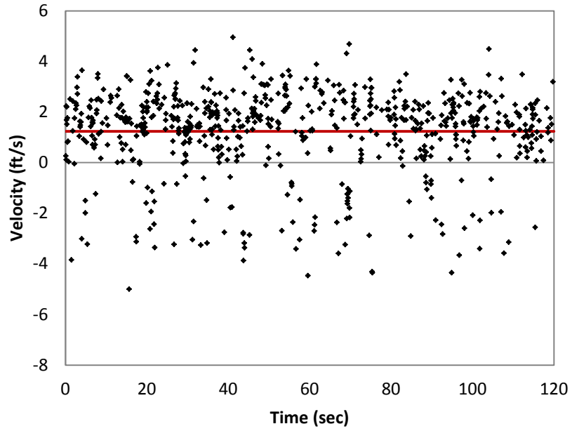
Figure 54: Filtered time series velocity distribution at a point in section 73. The red (bold) horizontal line indicates the mean value for the velocity.
