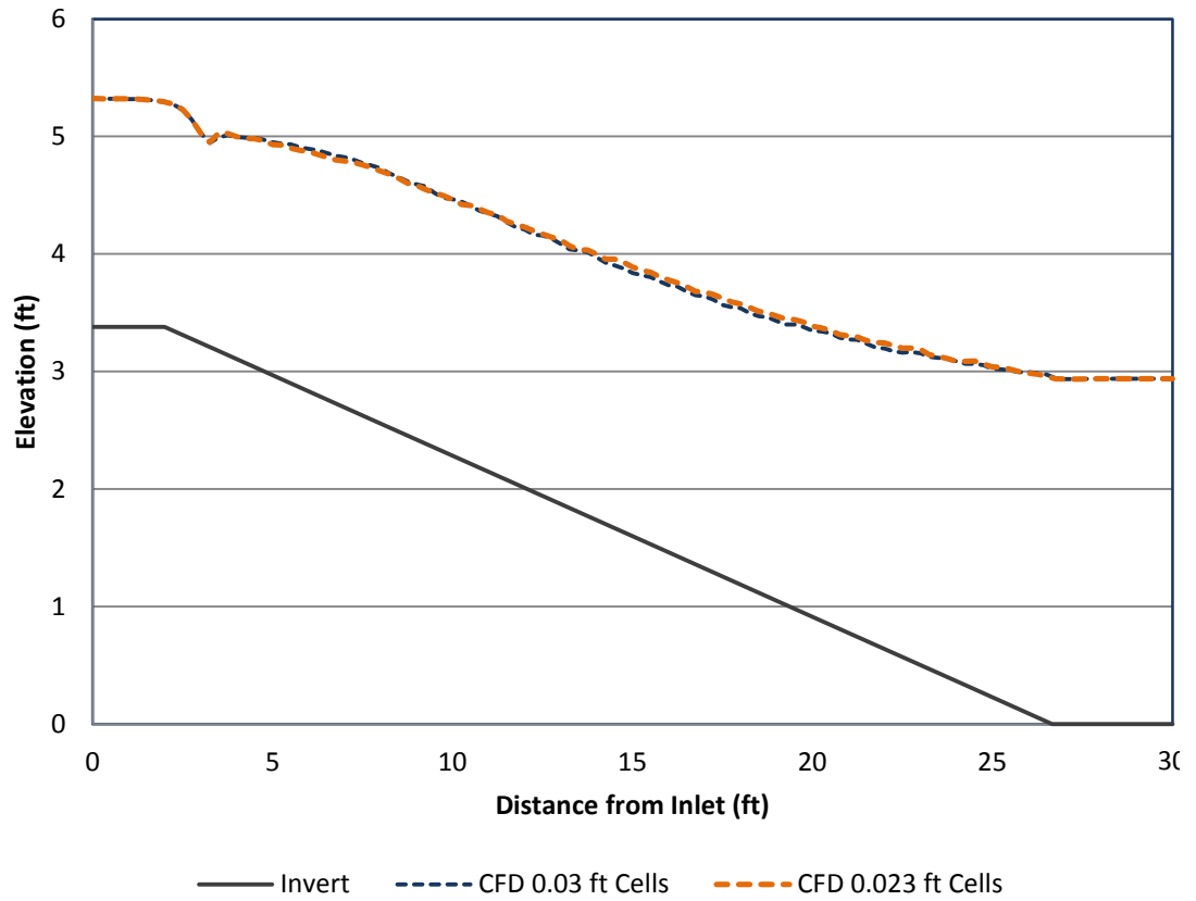
Figure 5: CFD model results for water surface profile at the centerline of the fishway for coarse and fine meshes, low head and shallow slope.
