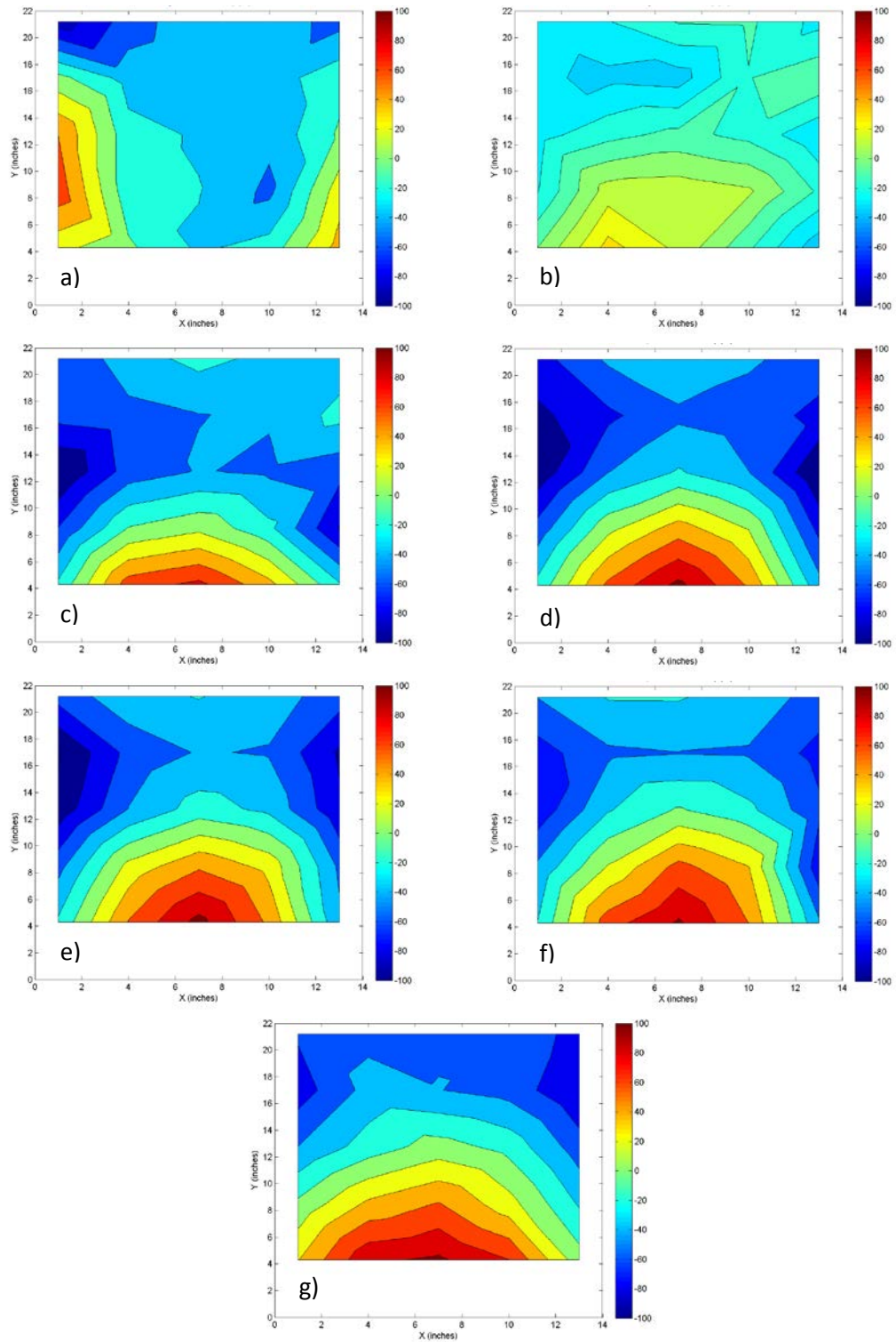
Figure 17: Percentage error between ECM and CFD velocities for high head and shallow slope at sections a) 23, b) 73, c) 123, d) 163, e) 203, f) 248, and g) 294 inches from the inlet, units are percent.
