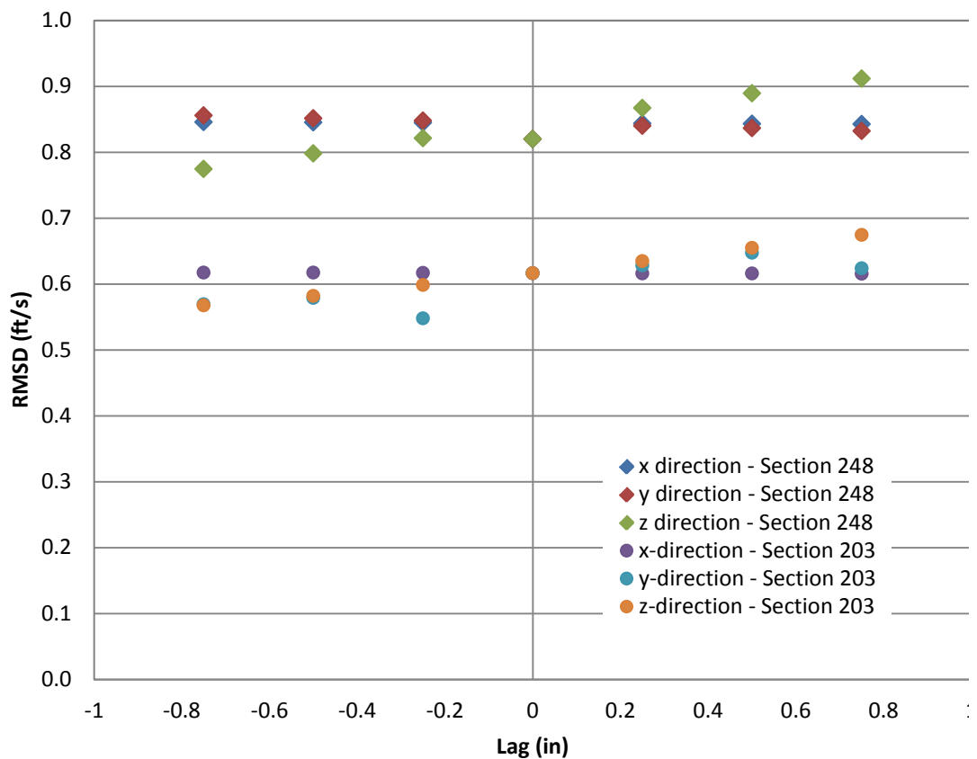
Figure 20: Lag analysis for sections 203 and 248 inches from the inlet for the low head, shallow slope simulation.
