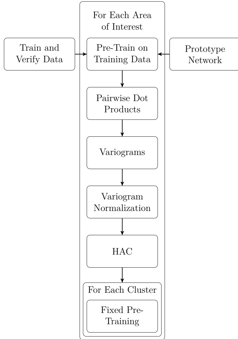
Figure 5.7: Pre-training
