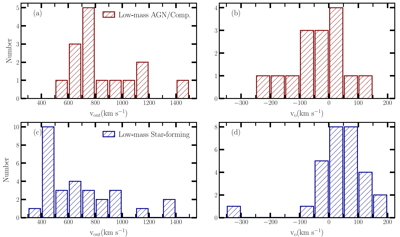
Figure 10. Same as Figure 8, but for the low-mass outflow galaxies with masses M_* < 10^{10}M_\odot . The medians of outflow and offset velocities for AGNs and composites are 777 and -46 km s ^{-1} , respectively, while SF galaxies have a lower median outflow velocity of 609 km s ^{-1} and a redshifted median offset velocity of 42 km s ^{-1} . See Section 4.5 for more details.
