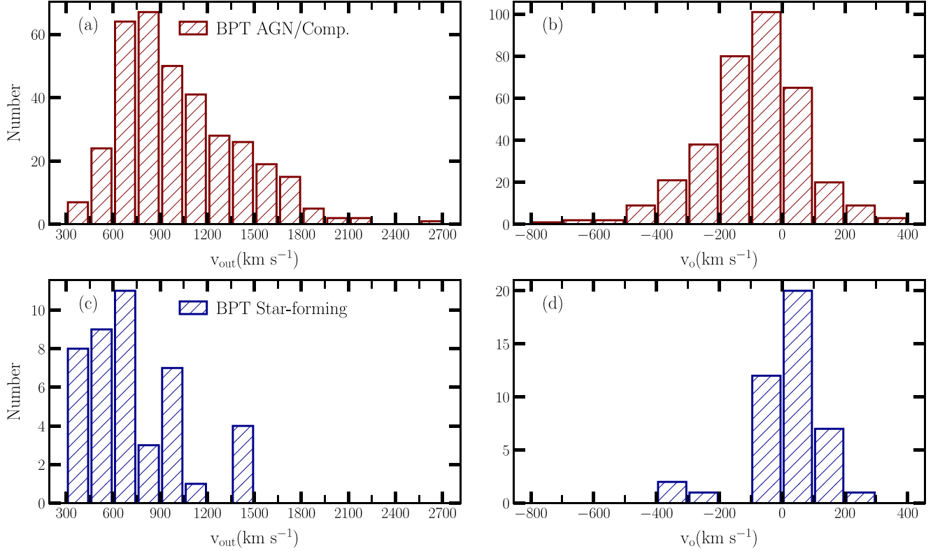
Figure 8. Outflow properties. (a)–(b): Distributions of outflow velocity ( v_{out} ) and offset velocity ( v_o ) for the BPT-AGNs and composites in our outflow sample shown in maroon histograms. The medians of outflow velocity and offset velocity are 936 km s ^{-1} and -84 km s ^{-1} , respectively. (c)–(d): Same as panels (a)–(b) except for the SF galaxies with outflow signatures plotted in blue histograms. Outflow and offset velocity median values are 655 km s ^{-1} and 28 km s ^{-1} , respectively. See Section 4.3 for more details.
