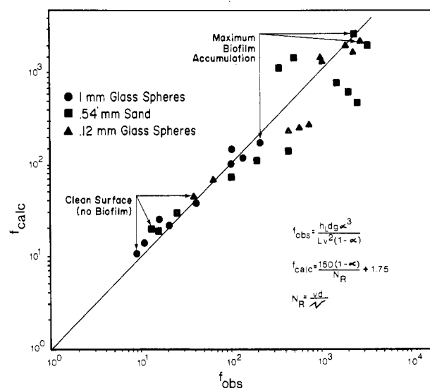
Figure 9. Comparison of measured porous media friction factors with values computed by using the Carman-Kozeny equation (eq 5).
