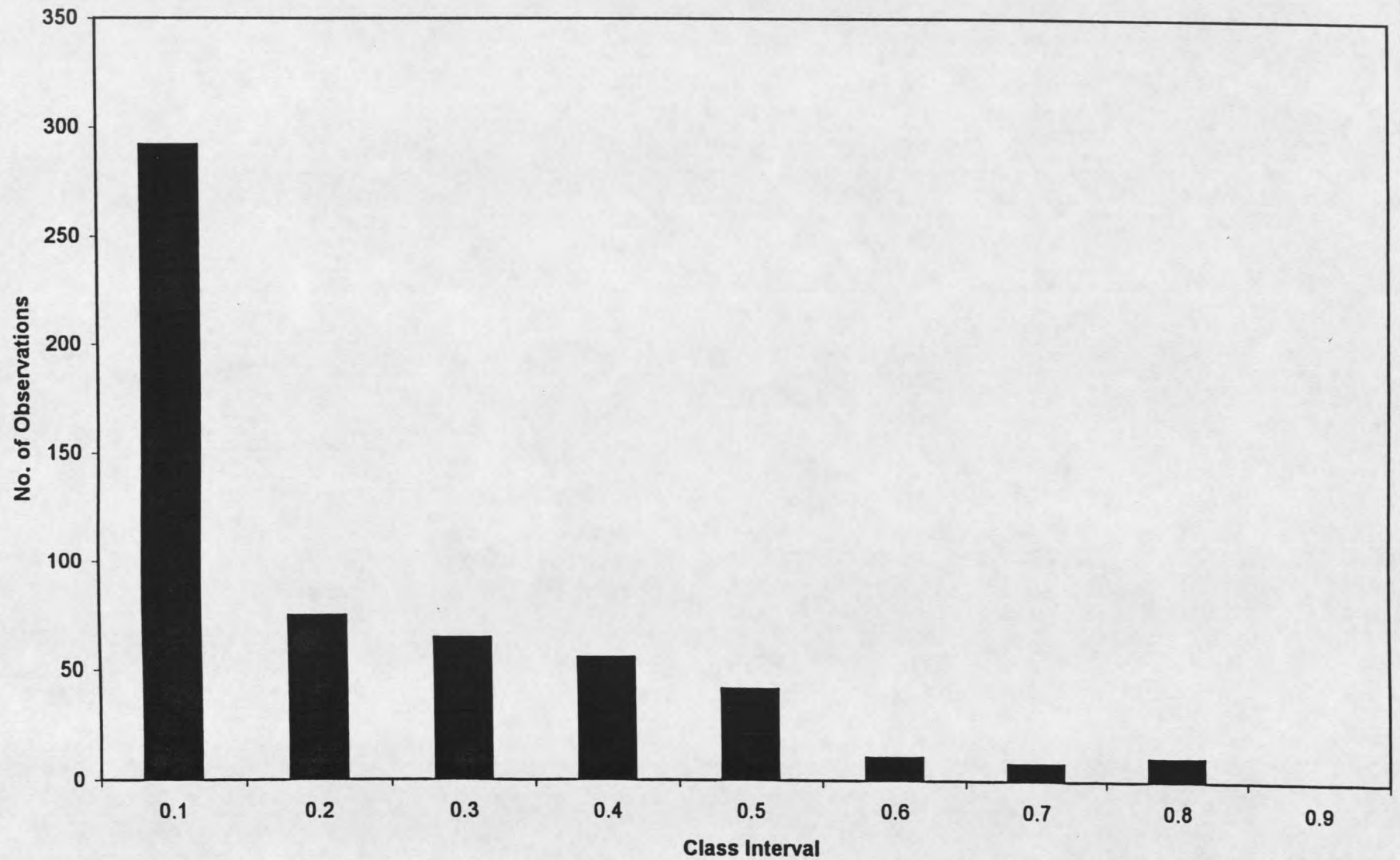
Fig. 3: Frequency distribution from AFLP data
