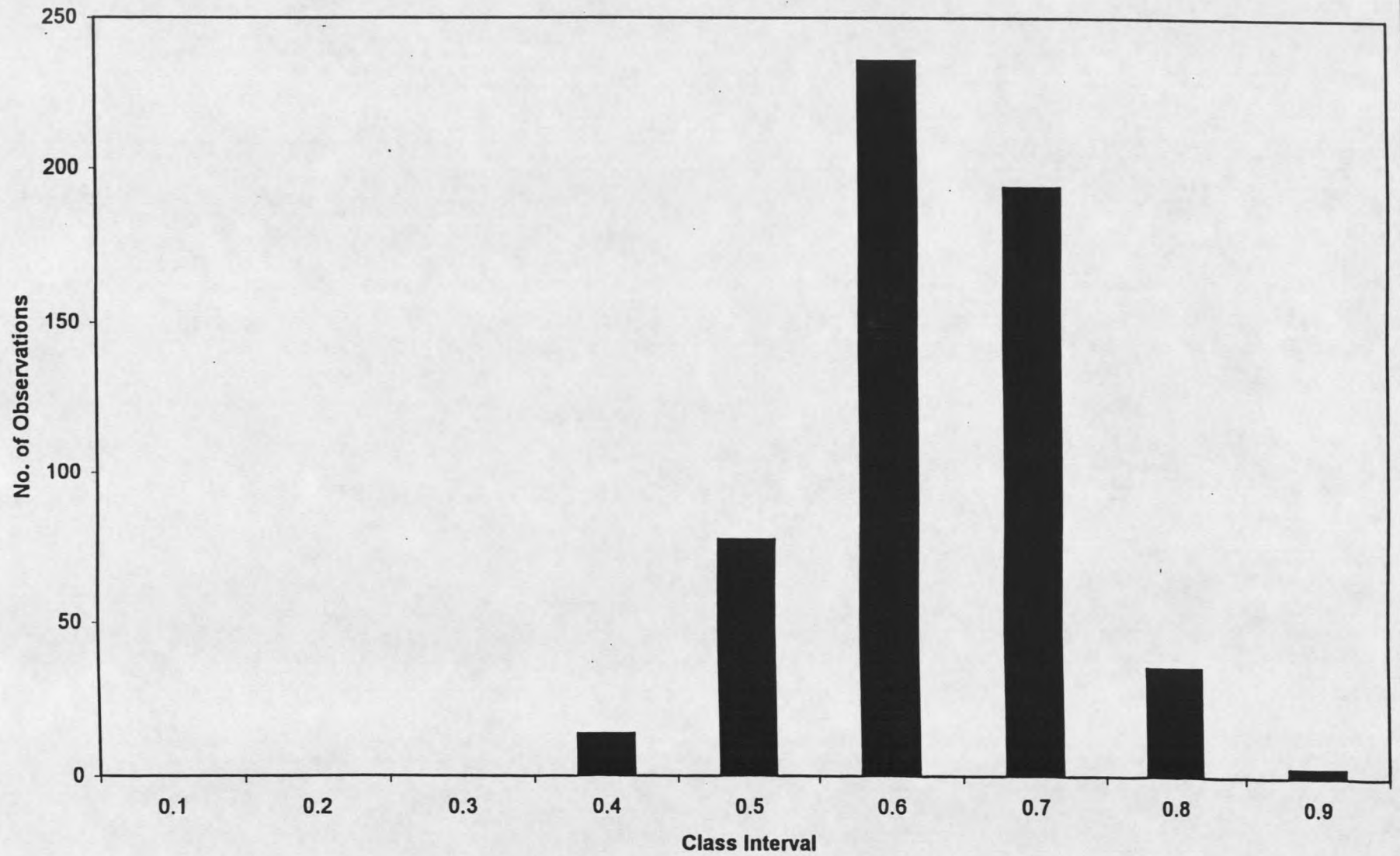
Fig. 2: Frequency distribution from AFLP data
