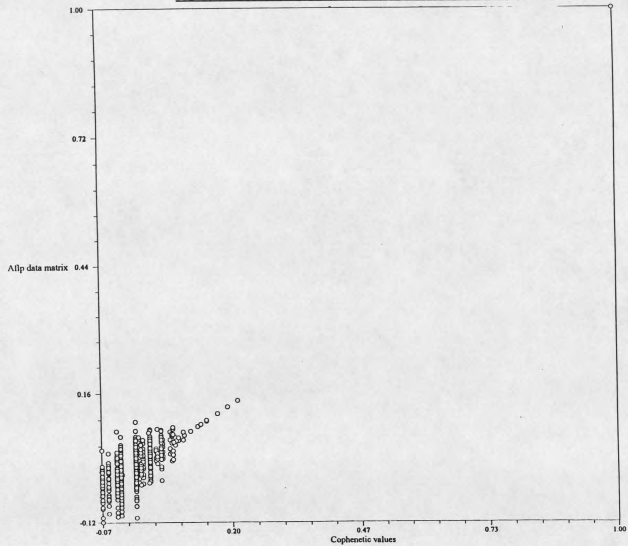
Fig 5: Comparison between cophenetic matrix with AFLP data matrix
