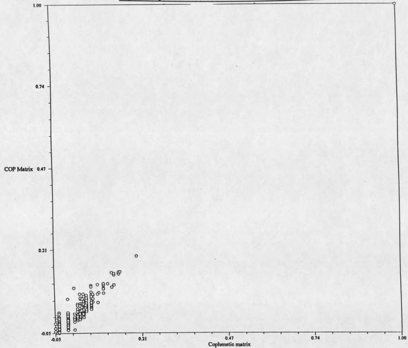
Fig 6: Comparison between COP matrix with cophenetic values
