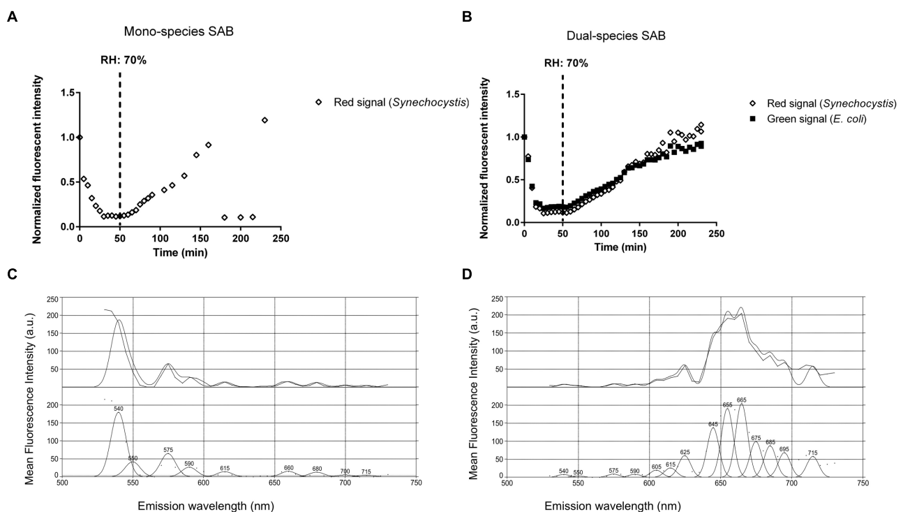
FIGURE 4 | Biofilm recovery after desiccation. Recovery of fluorescence of a mono (A) and dual-species SAB during rewetting (B). Emission spectra recorded in cyanobacterial cells before (C) and after (D) rewetting. Spectral profiles were analyzed by PICKFIT deconvolution software to show individual phycobiliproteins: Phycoerythrin, 575 nm; Phycocyanin, 645 nm; Allophycocyanin, 665 nm; Chlorophyll a, 685 nm (Wolf and Schübler, 2005).
