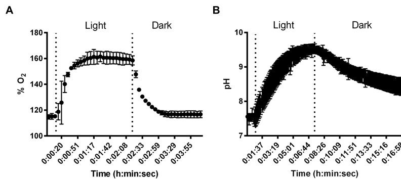
FIGURE 3 | Results of changes in O 2 % saturation (A) and pH (B) in dual-species SABs during shifts between light and dark conditions. Data points are average of triplicate experiments. Error bars represent standard deviation of triplicate experiments.
