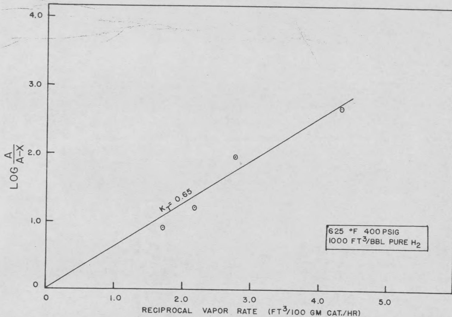
Fig. 3. Desulfurization vs. Reciprocal Vapor Rate (Run U.S.S.-22)
