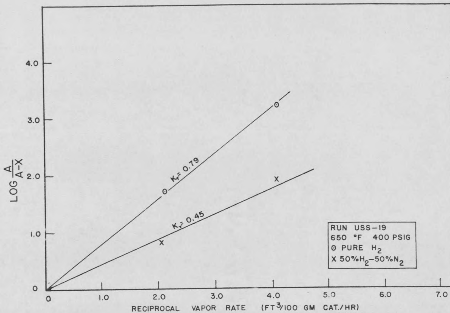
Fig. 10. Effect of Diluent Gas on K_T
