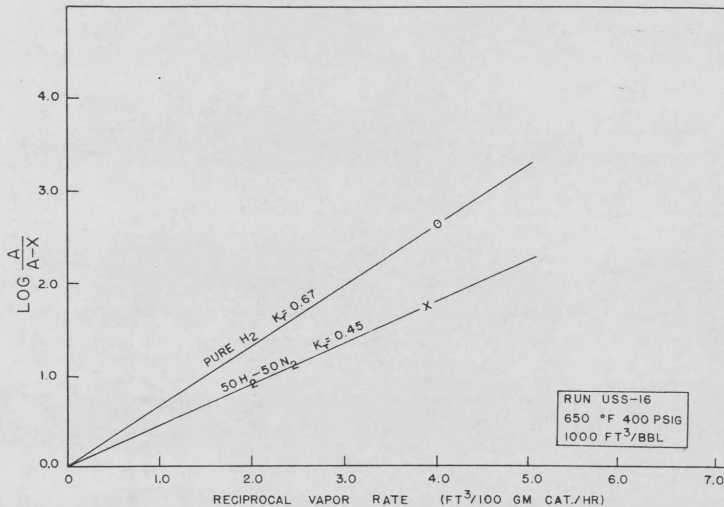
Fig. 9. Effect of Diluent Gas on K_T
