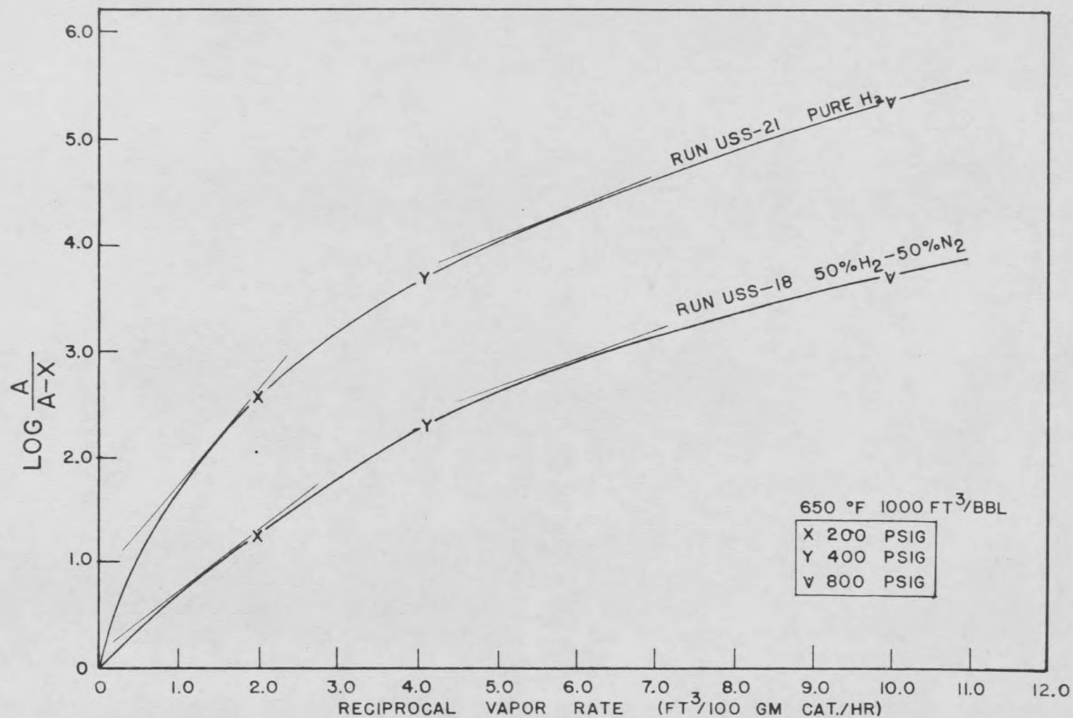
Fig. 3. Effect of Vapor Rate at Various Pressures on the Degree of Desulfurization at Constant Ratio of Feed to Catalyst
