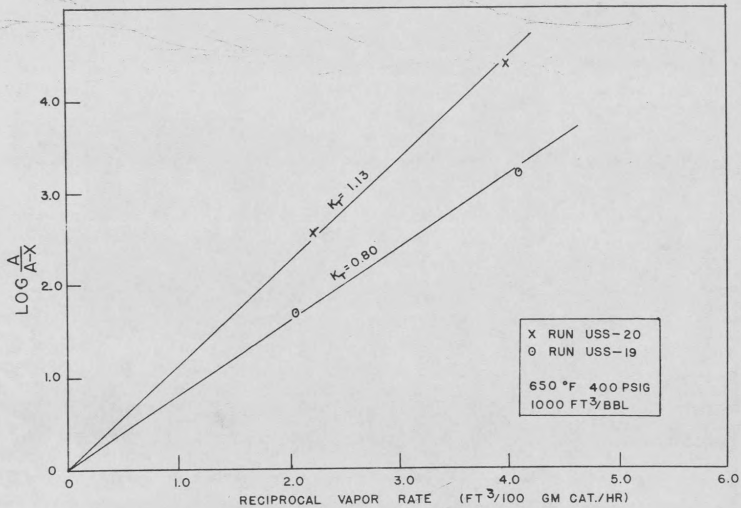
Fig. 4. Desulfurization vs. Reciprocal Vapor Rate (Runs U.S.S.-19 and-20)
