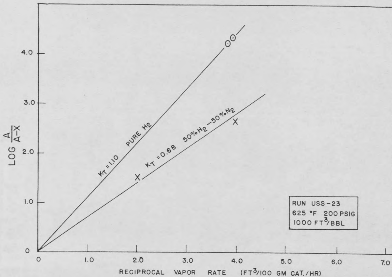
Fig. 11. Effect of Diluent Gas on K_T
