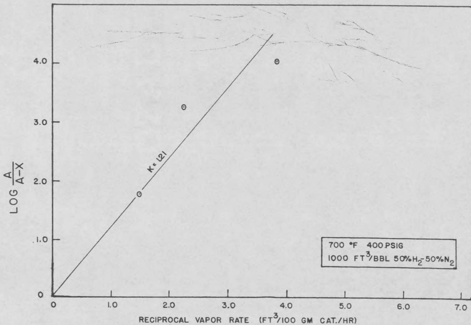
Fig. 2. Desulfurization vs. Reciprocal Vapor Rate (Run U.S.S.-17)
