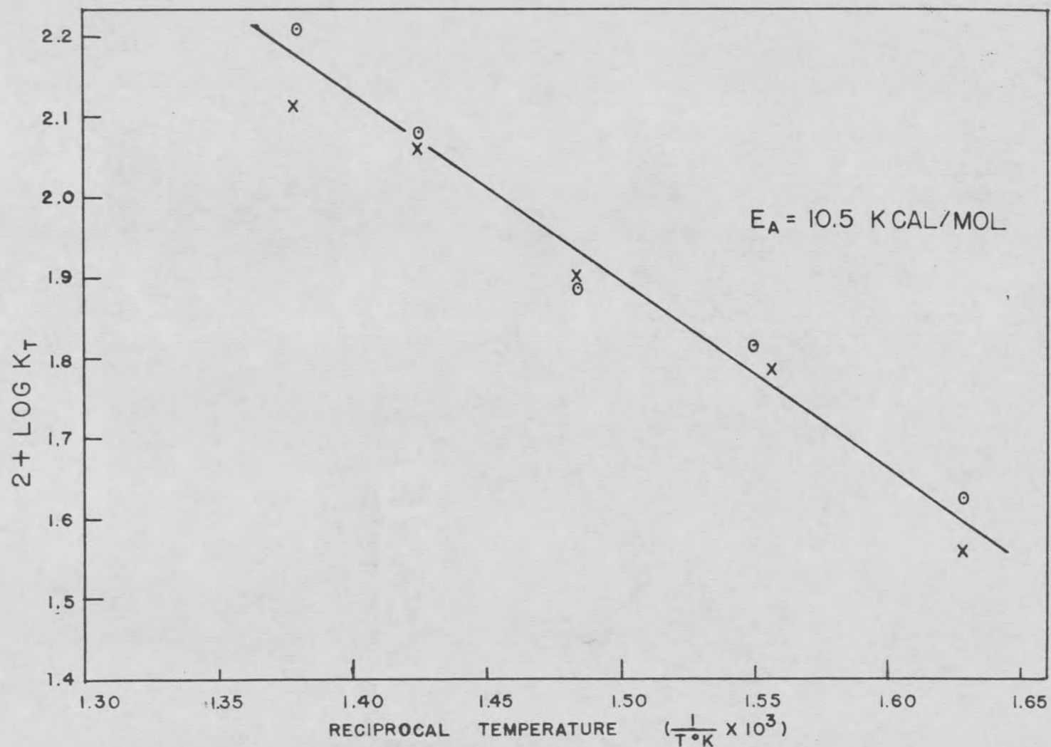
Fig. 5. Determination of the Effect of Temperature ( E_a ) on K_T (Runs U.S.S.-10 and-11)
