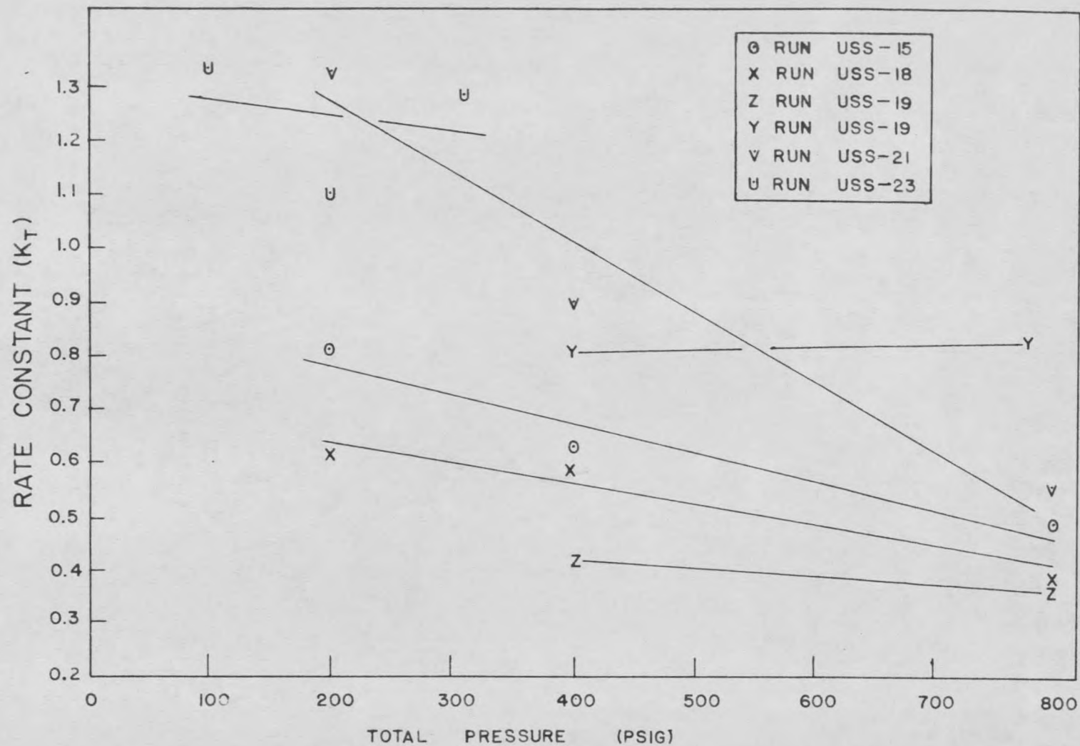
Fig. 7. Effect of Total Pressure on the Rate Constant ( K_T )
