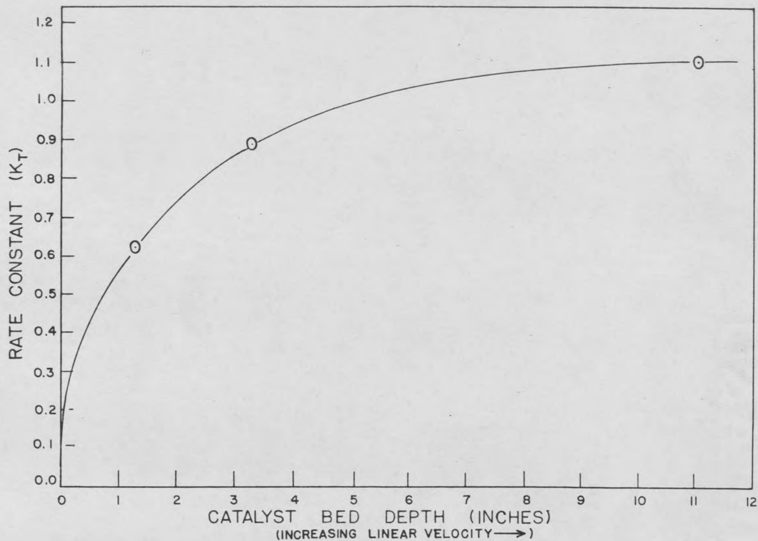
Fig. 13. Effect of Catalyst Bed Depth on K_T
