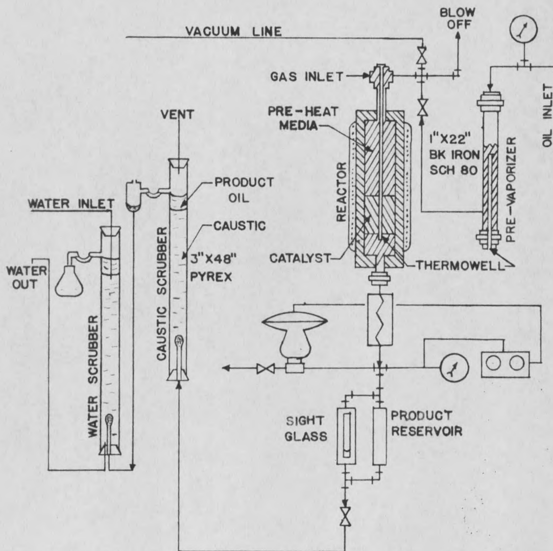
Figure 1 - Schematic Diagram of Desulfurization Unit for Processing Light Oil.
