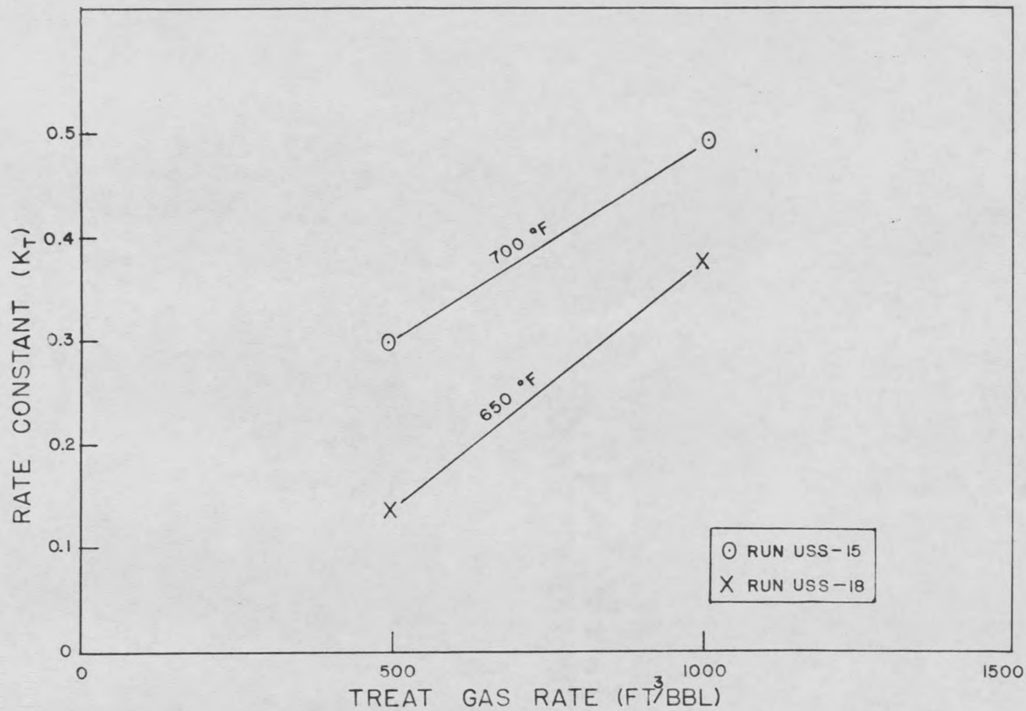
Fig. 12. Effect of Treat Gas Rate on K_T
