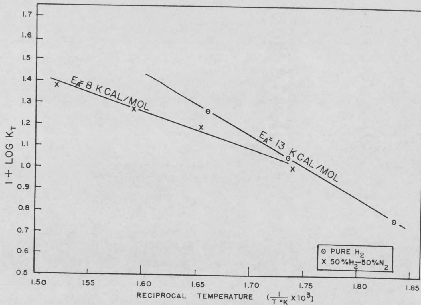
Fig. 6. Determination of the Effect of Temperature ( E_a ) on K_T (Run U.S.S.-24)
