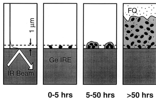
FIG. 2. ATR/FT-IR methodology (40). IR absorbance is measured in a region within the aqueous medium confined to a distance of approximately 1 \mu m from the Ge substratum. Cell attachment and lateral colonization of the substratum can be monitored with the bacterial IR signal (lateral growth curve). The unique IR spectrum of an FQ which appears in the region adjacent to the substratum (base of the biofilm) can be detected if the bacterial (background) spectrum does not change too drastically. Egg-shaped symbols, dots, and dark and light shaded areas represent cells, FQ, IRE, and EPS matrix, respectively.
