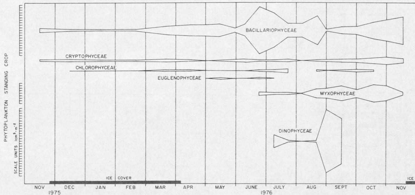
Figure 31. Seasonal variations in class composition of the phytoplankton standing crop at Station 2 in the Tongue River Reservoir. Data were collected from November 1975 through November 1976.
