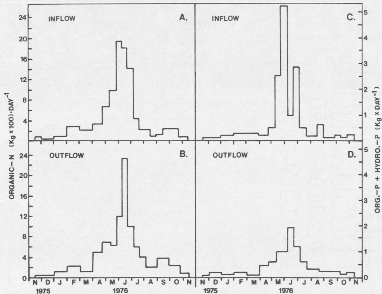
Figure 14. Seasonal loads of organic nitrogen and organic + hydrolyzable phosphorus carried by the inflow and outflow waters.
