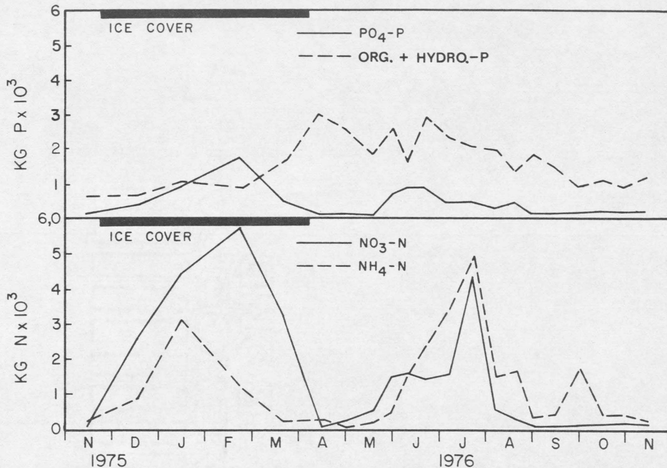
Figure 28. Seasonal storage of inorganic nitrogen, orthophosphorus and organic + hydrolyzable phosphorus in the Tongue River Reservoir.
