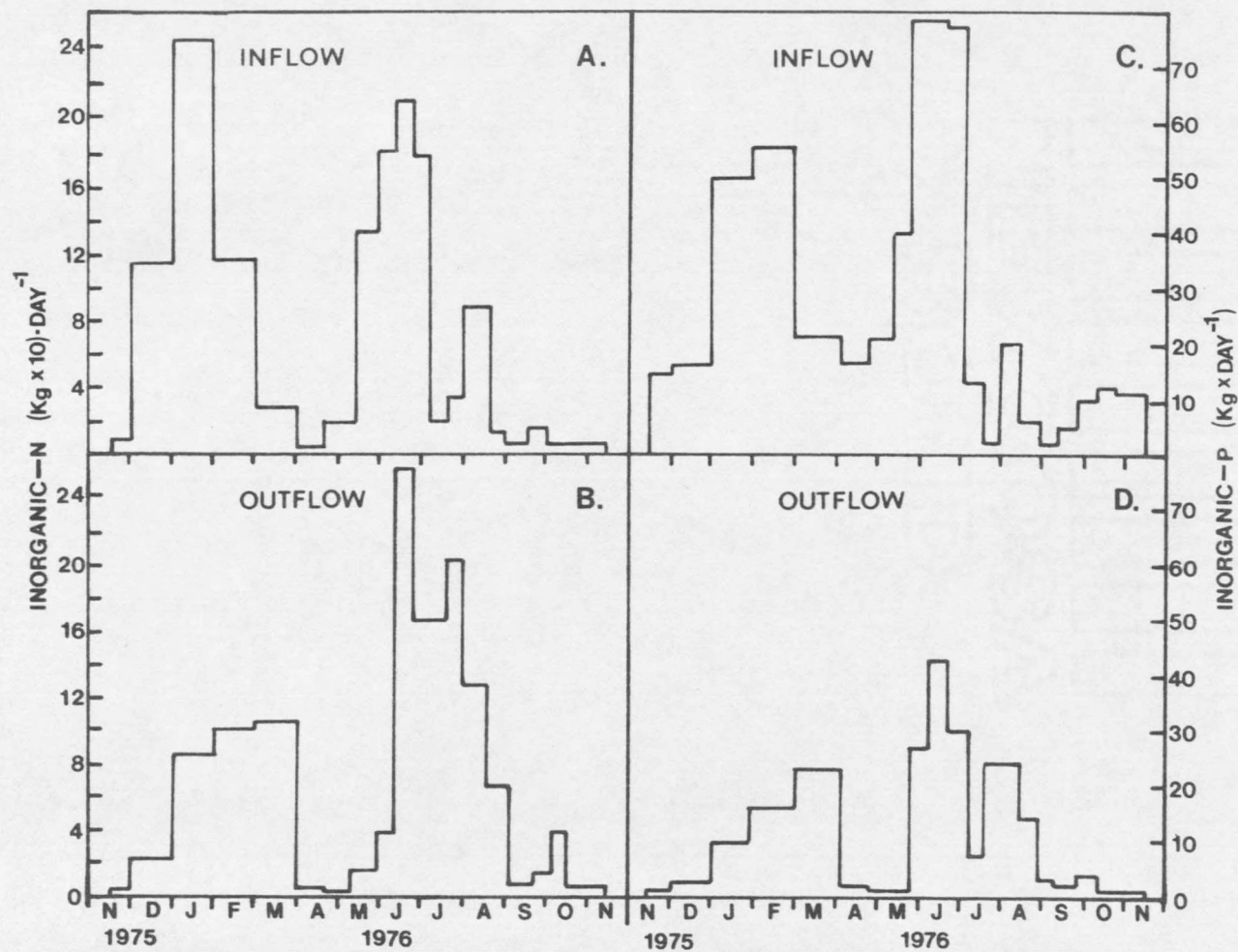
Figure 13. Seasonal loads of inorganic nitrogen ( \text{NO}_2 + \text{NO}_3 + \text{NH}_3\text{-N} ) and inorganic phosphorus ( \text{PO}_4\text{-P} ) carried by the inflow and outflow waters.
