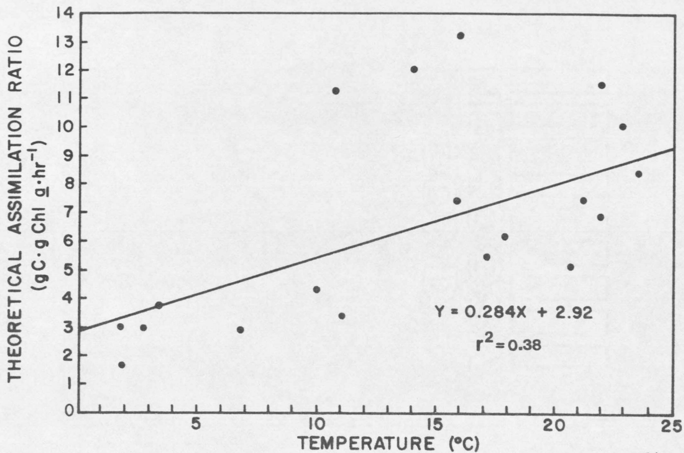
Figure 39. Regression line correlating theoretical assimilation ratios (based on 14 C estimates of diel photosynthesis) with euphotic zone temperatures at Station 2 in the Tongue River from November 1975 through November 1976.
