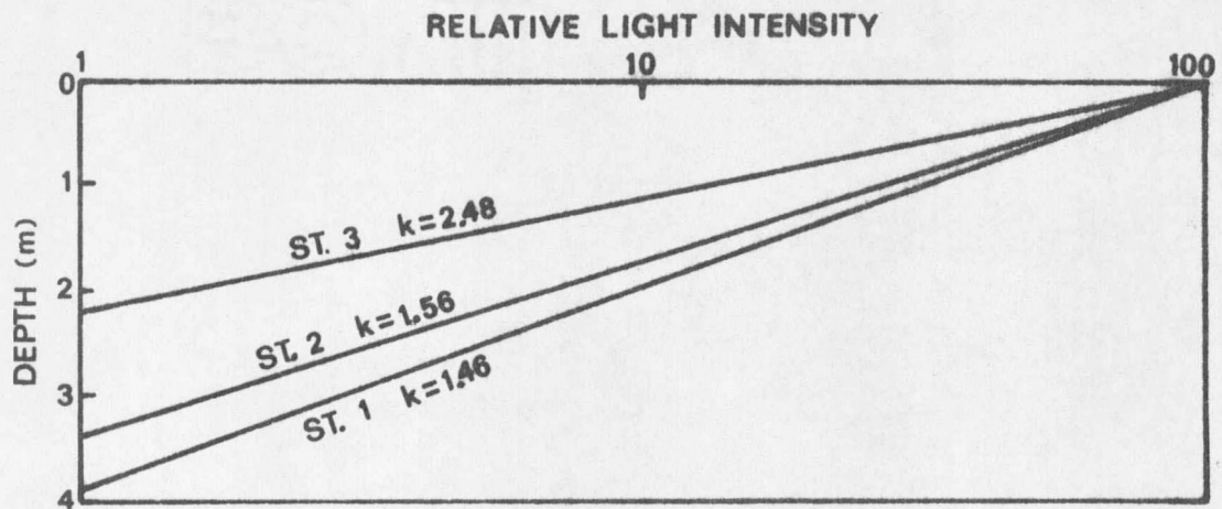
Figure 16. Penetration of total visible light, mean extinction coefficients ( k ) and euphotic zone depths in the Tongue River Reservoir from 6/75 - 11/76.
