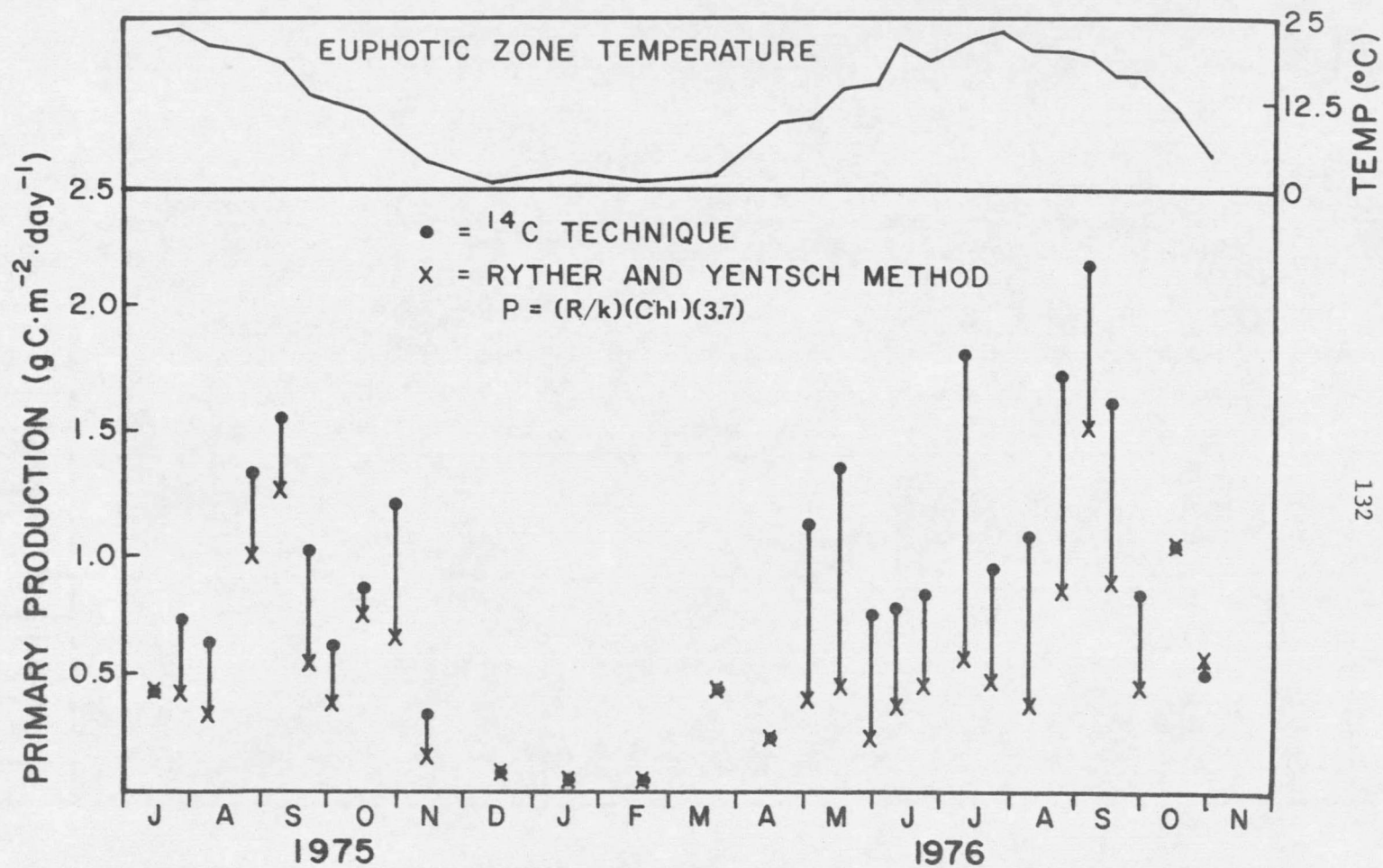
Figure 37. Differences in day rate estimates of photosynthesis at Station 2 in the Tongue River Reservoir as estimated by the ^{14}\text{C} technique and the method of Ryther and Yentsch (1957). Results are plotted against the euphotic zone temperature.
