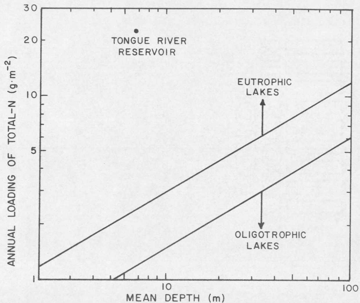
Figure 43. Vollenweider's (1970) model for the trophic classification of lakes based on annual surface loading of total nitrogen as a function of mean depth.
