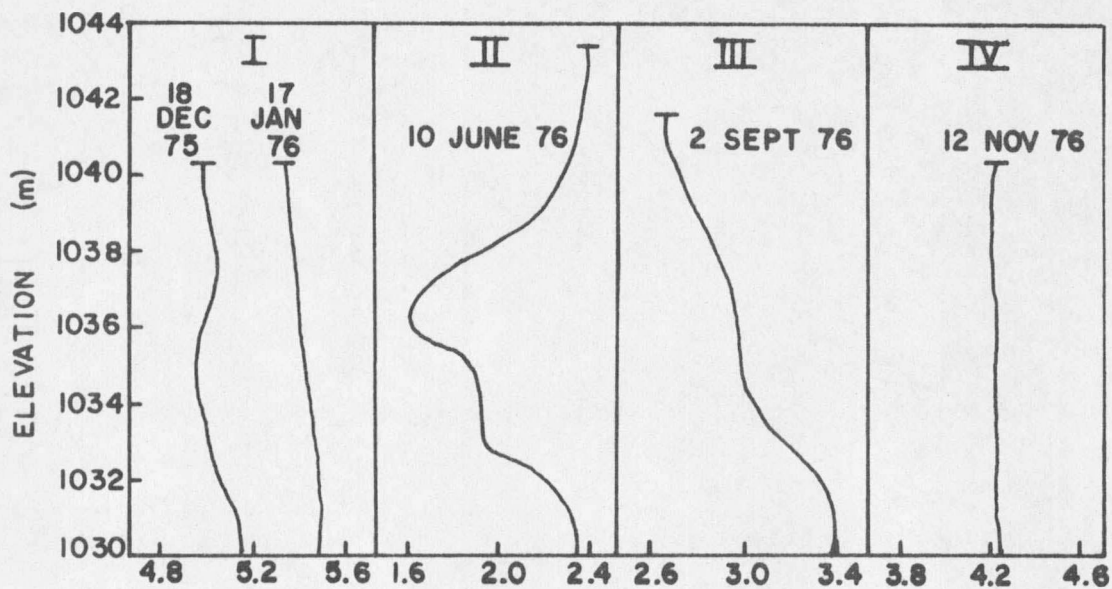
Figure 22. Total alkalinity (me·L -1 ) profiles in the Tongue River Reservoir on selected dates.
