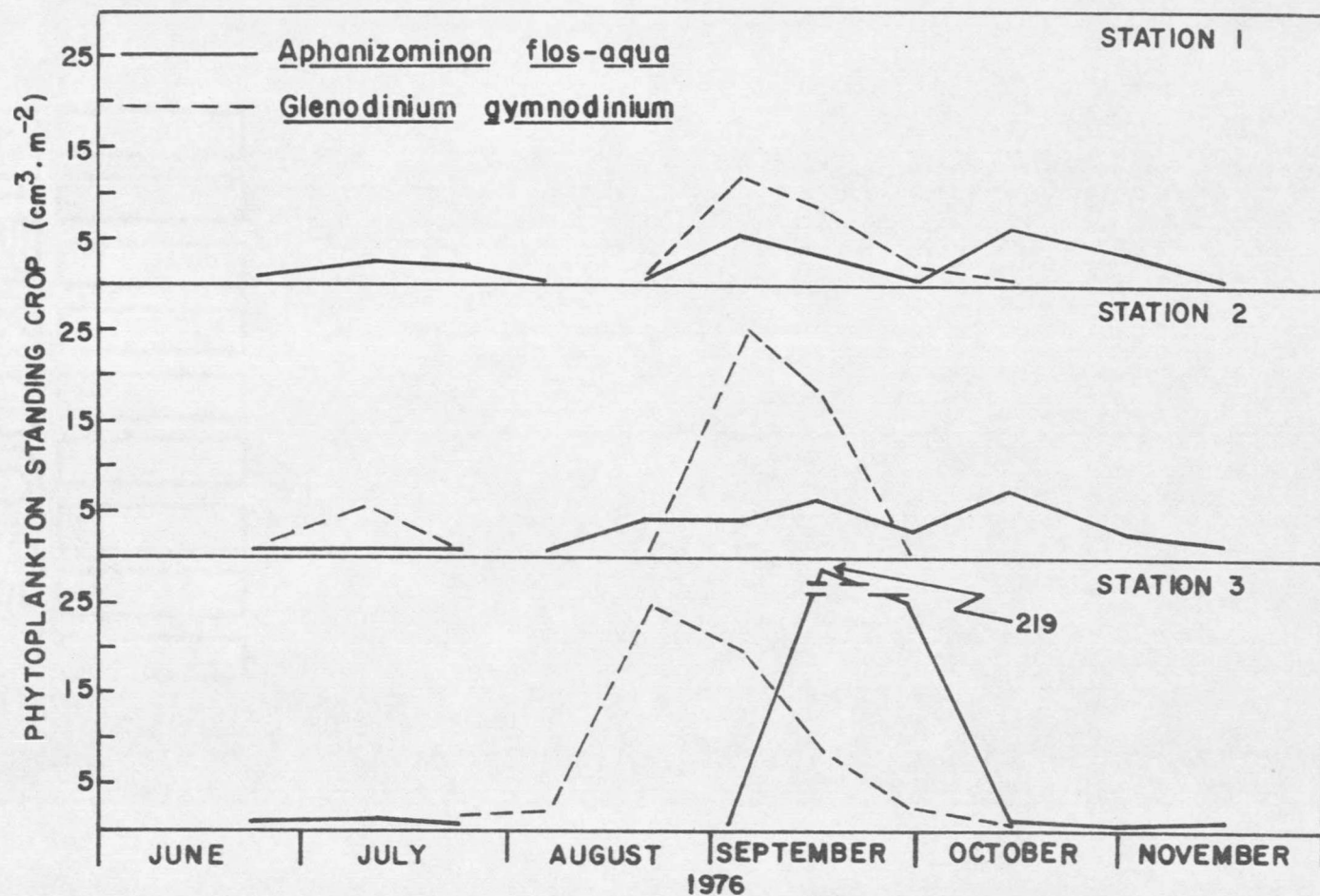
Figure 33. Seasonal succession of Aphanizomenon flos-aqua and Glenodinium gymnodinium in 1976 at three sampling sites in the Tongue River Reservoir.
