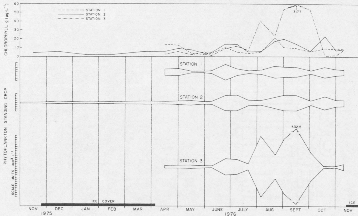
Figure 29. Seasonal variations in the volumetric phytoplankton standing crop and chlorophyll a concentration at three Tongue River Reservoir sampling sites. Data were collected from November 1975 through November 1976.
