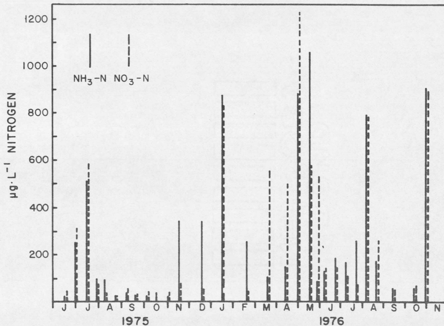
Figure 46. Ammonia and nitrate concentrations measured in the mine discharge water from June 1975 through November 1976.
