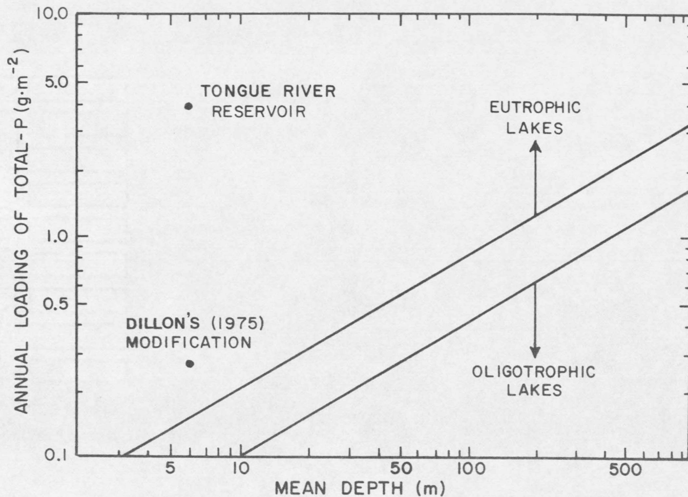
Figure 42. Vollenweider's (1970) model for the trophic classification of lakes based on annual surface loading of total phosphorus as a function of mean depth.
