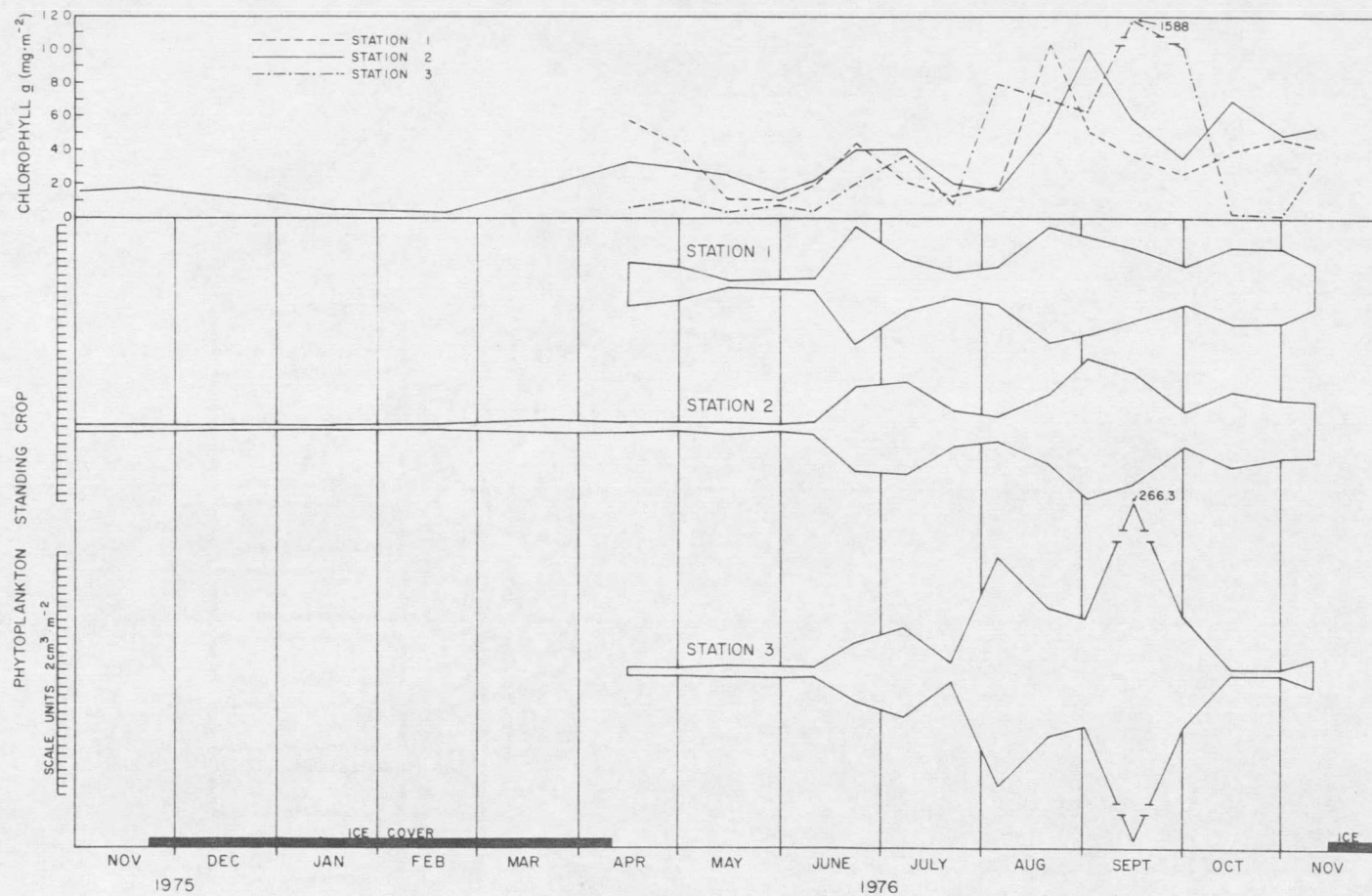
Figure 30. Seasonal variations in the areal phytoplankton standing crop and chlorophyll a concentration at three Tongue River Reservoir sampling sites. Data were collected from November 1975 through November 1976.
