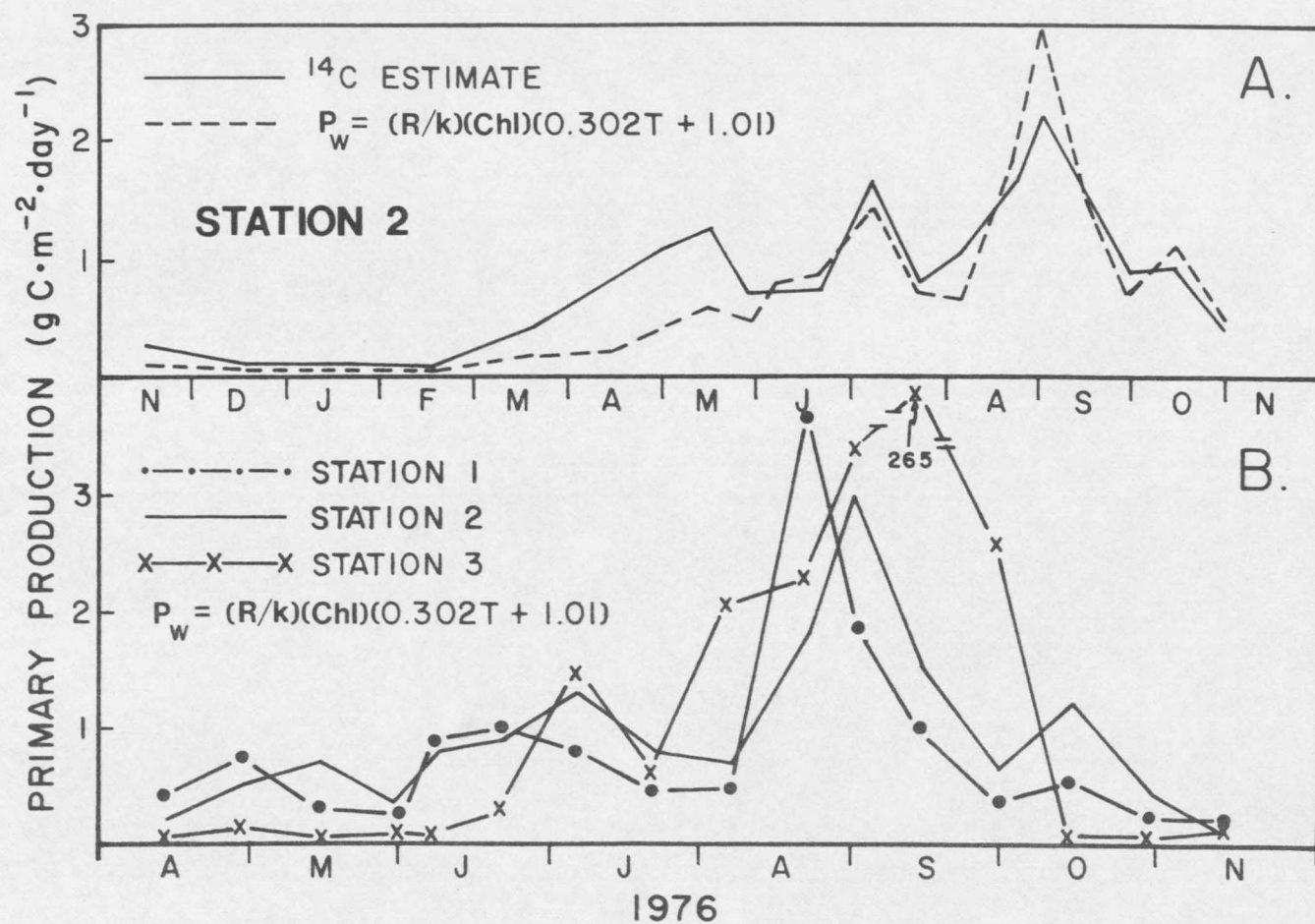
Figure 41. A. Comparison of estimates of diel photosynthesis at Station 2. Estimates were obtained by the 14 C method and by a modified Ryther and Yentsch (1957) formula. B. Diel photosynthesis at three Tongue River Reservoir sampling sites during the growing season of 1976 as estimated by Equation 2.
