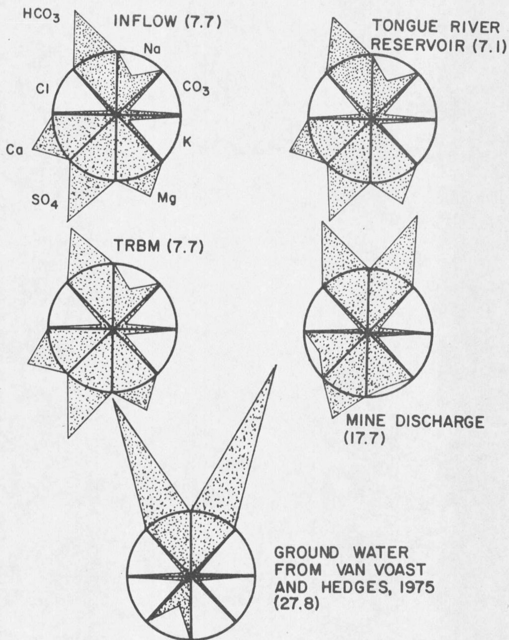
Figure 45. Ionic polygonic diagrams of the mean relative concentrations in equivalent percentages of the major cations and anions at several sampling sites. The number in parentheses represents the sum of the cations ( \text{me}\cdot\text{L}^{-1} ).
