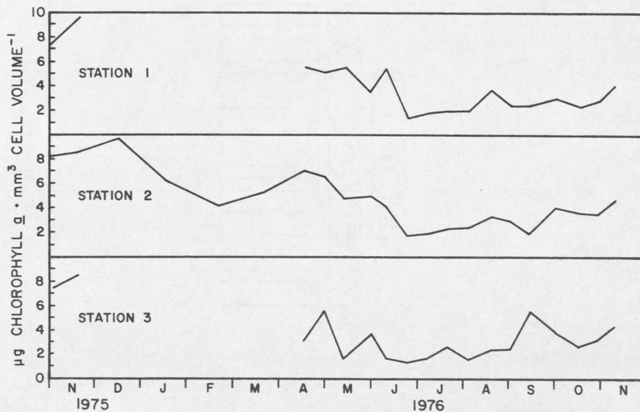
Figure 35. Seasonal euphotic zone phytoplankton chlorophyll a /cell volume ratios in the Tongue River Reservoir. Data were collected from November 1975 through November 1976.
