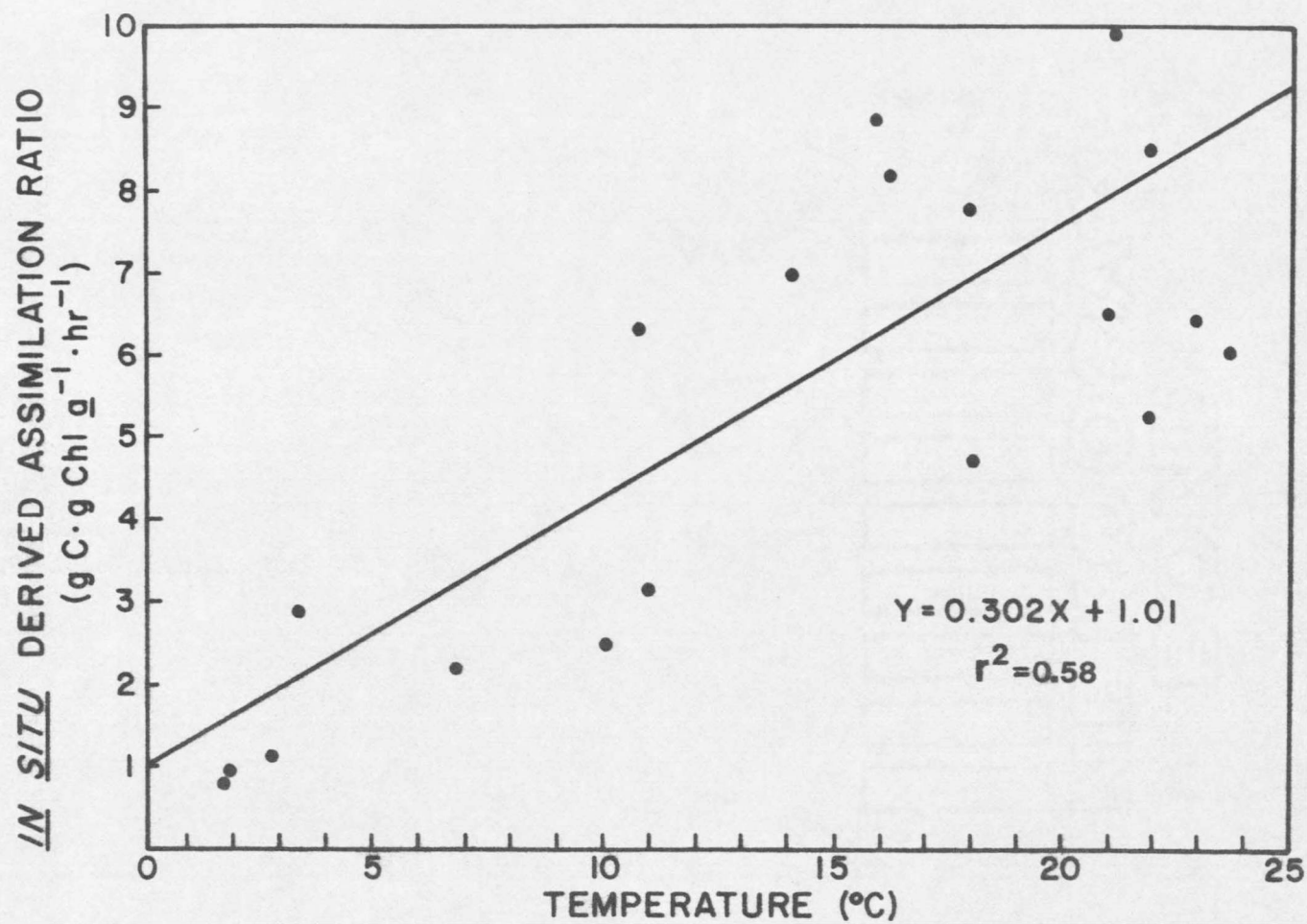
Figure 38. Regression line correlating in situ derived assimilation ratios and euphotic zone temperatures at Station 2 in the Tongue River Reservoir from November 1975 through November 1976.
