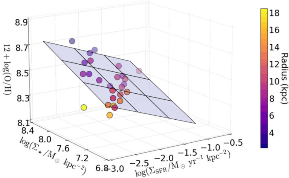
Figure 13. 3D visualization of the resolved Fundamental Metallicity Relation for the 26 H II regions in the galaxy NGC 99 color coded by galactocentric radius. The x-axis and y-axis are the stellar mass and star formation rate surface densities, respectively, for each region. Gas-phase metallicities from the N2 indicator are shown on the z-axis. The points are well fit by a linear plane described by Equation (11). An animated version of this figure is available online, where we rotate around the z-axis for one full rotation in an 18 s animation.
