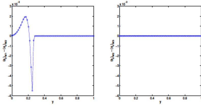
FIGURE 7. Biomass volume fraction difference between two pairs of models at t = 60 . Left: The difference between model 1 and model 2 at t = 60 . The largest difference is in the order of O(10^{-3}) . Right: The difference between model 2 and model 3 at t = 60 . The two models give virtually identical results. Parameter values are identical to those used in Figure 6.
