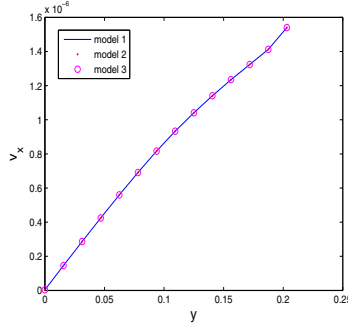
FIGURE 4. Blow-up of v_x in the bio lm region with respect to solutions of all three models at t = 200 . The results are essentially indistinguishable.
