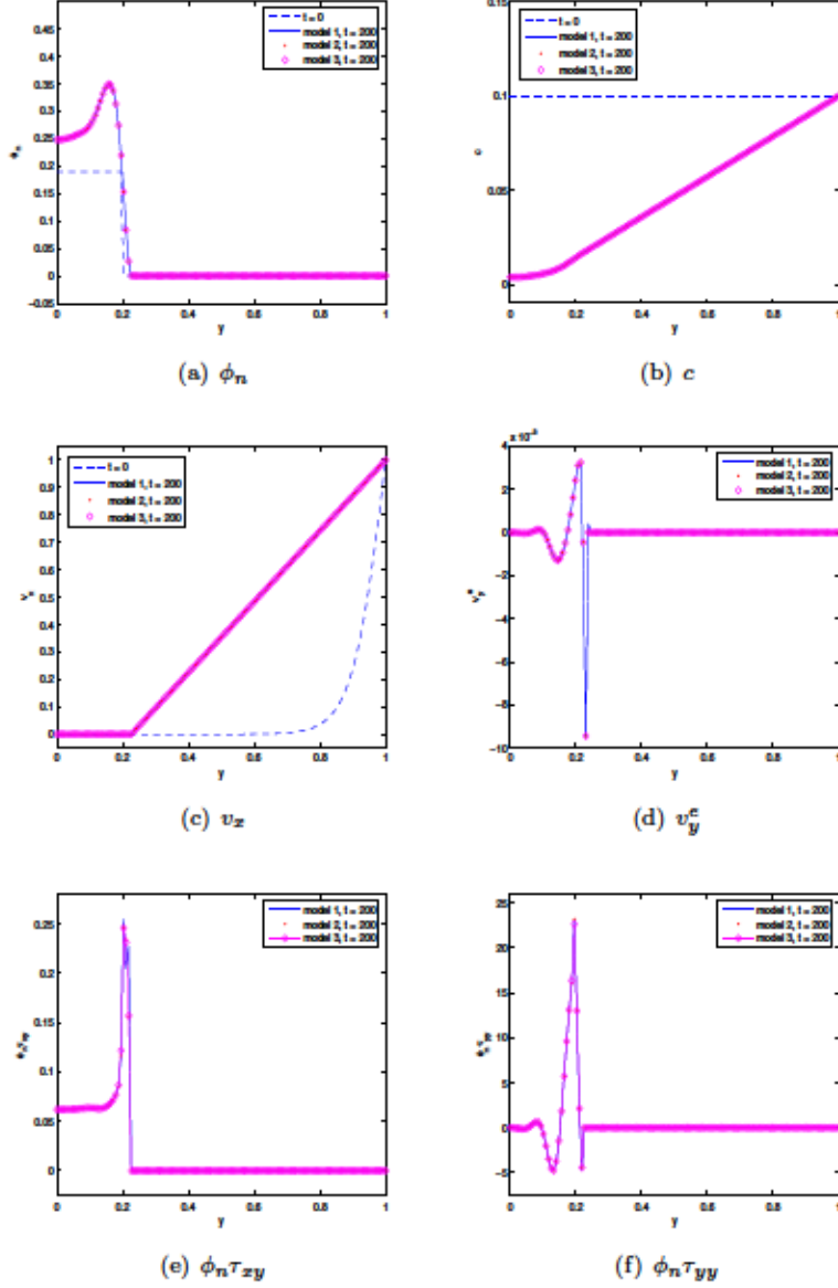
FIGURE 9. Solutions of the three models at t = 200 and mobility parameter \Lambda = 2.5 \times 10^{-9} , mixing parameter \chi = 0.65 , and relaxation time \Lambda_1 = 50 . The results from model 2 and 3 are essentially indistinguishable. The stress fluctuation from model 1 differs slightly from those from model 2 and model 3.
