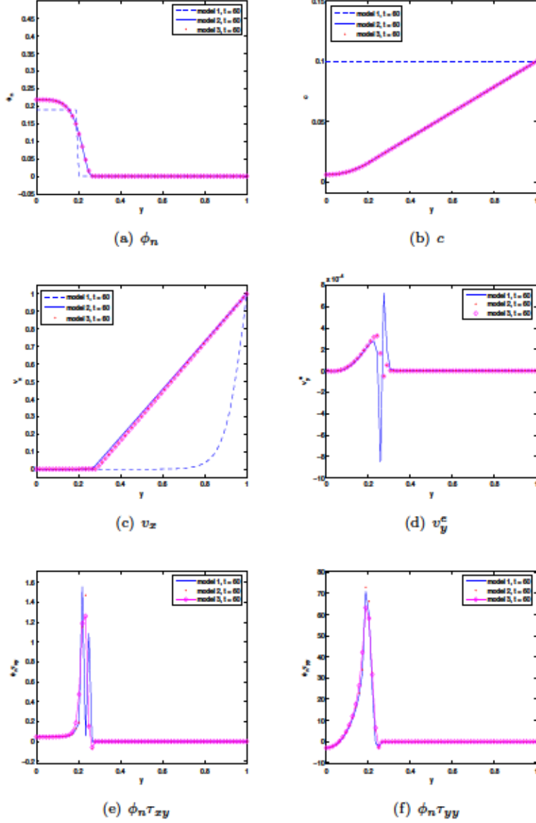
FIGURE 6. Solutions of all three models at t = 60 , mobility parameter \Lambda = 2.5 \times 10^{-7} , mixing parameter \chi = 0.55 , and relaxation time \Lambda_1 = 50 . Model 1 exhibits the largest fluctuation in velocity and elastic stress at the biofilm-solvent interface while the other two models show mild fluctuations.
