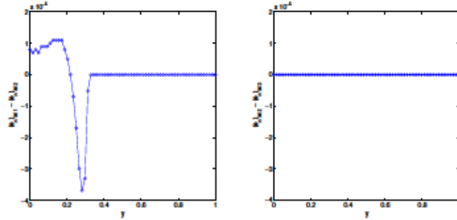
FIGURE 2. Difference of the biomass volume fraction between model 1 and 2 as well as model 2 and 3 at t = 200 . Left: The difference in the biomass volume fraction between model 1 and model 2. The largest difference is in the order of O(10^{-5}) . Right: The difference in the biomass volume fraction between model 2 and model 3. Model 2 and 3 give virtually identical results. Parameter values are identical to the ones used in Figure 1.
