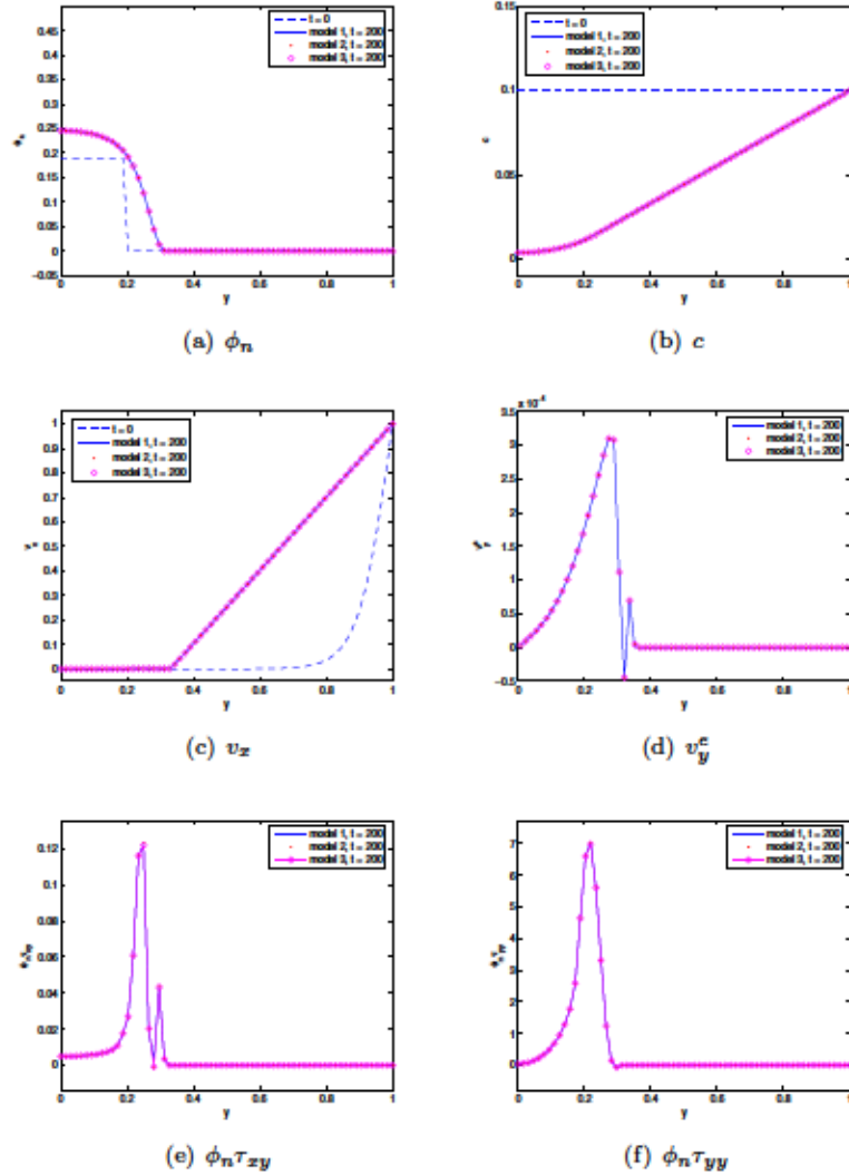
FIGURE 1. Solutions of the three models at t = 200 , mobility parameter \Lambda = 2.5 \times 10^{-7} , mixing parameter \chi = 0.55 , and relaxation time \Lambda_1 = 2.5 \times 10^3 . The separable model 1 and 2 are referred to as model 1 and 2 while the nonseparable model is referred to as model 3 in the text and the figures. (a). The biomass volume fraction \phi_n ; (b). the nutrient concentration c ; (c). the velocity component in the x-direction v_x ; (d). the velocity component in the y-direction v_y = v_y^c ; (e). the elastic shear stress \phi_n \tau_{xy} ; (f). the elastic normal stress \phi_n \tau_{yy} . The three models' predictions are essentially indistinguishable in this parameter regime.
