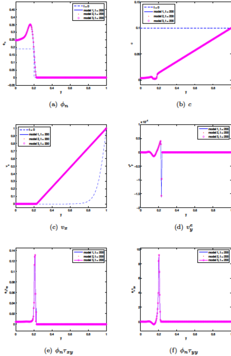
FIGURE 5. Solutions of the three models at t = 200 , mobility parameter \Lambda = 2.5 \times 10^{-9} , mixing parameter \chi = 0.65 , and relaxation time \Lambda_1 = 2.5 \times 10^3 . The results are essentially indistinguishable.
