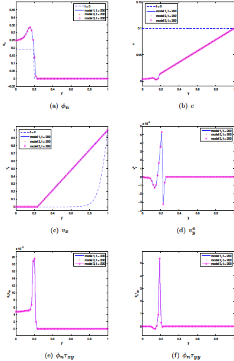
FIGURE 3. Solutions of the three models at t = 200 , mobility parameters \Lambda = 2.5 \times 10^{-9} , mixing parameter \chi = 0.55 , and relaxation time \Lambda_1 = 2.5 \times 10^3 . The nutrient is consumed the most at the front of the biofilm. The three models' predictions are essentially indistinguishable.
