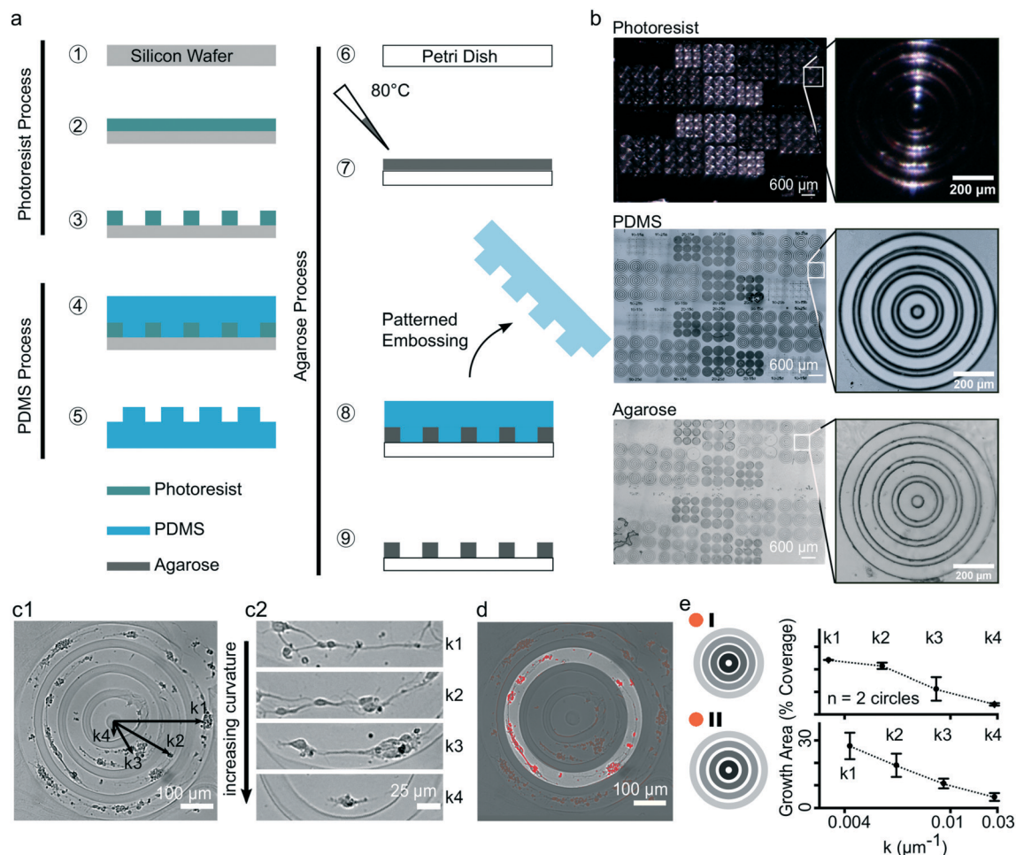
Fig. 2 Device design shows the robust fabrication of curvature features and embedded curved neurite outgrowth. (a) Schematic of micropatterning process flow. The photoresist process takes place in the cleanroom and yields a modeling master. The process of polydimethylsiloxane (PDMS) stamp formation is repeatable and done in a physical wet lab setting. The last process uses liquified agarose hydrogel as a base layer onto which the PDMS microstructures get imprinted. This step yields the multi-curvature hydrogel patterns where neuronal cells grow within the grooves. (b) Microscope images show the photoresist structure on the master, the microstructures after being cast into PDMS, and the imprinted hydrogel microstructures. (c1 and c2) DIC images of day 12 cortical neurons forming circular networks in the multi-layered curvatures. Distinct curved growth patterns depend on curvatures k_1 , k_2 , k_3 , and k_4 , where k_1 is always the smallest curvature. (d) Image processing mask used to extract curvature-dependent static and transient calcium activity within one circular network. (e) The diagram shows curvature-dependent coverage of total ring growth area in the micropatterns, extracted from two patterns ( n = 2 , each) at 12 DIV. The covered growth area decreases as curvature increases.
