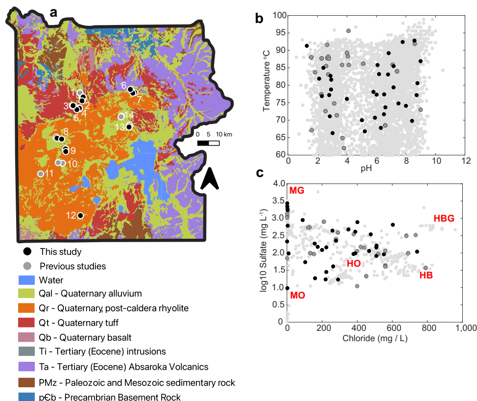
Fig. 1 | Locations of 69 Yellowstone National Park (YNP) hot spring samples analyzed in this study and major geochemical parameters measured in spring waters. a Map of sampling locations within YNP, modified from USGS I-711, as indicated in the Materials and Methods. Hydrothermal regions are labeled as follows: 1: Norris-Mammoth Corridor (NMC), 2: Norris Geyser Basin (NOR), 3: Sylvan Springs (SYL), 4: Geyser Creek (GCR), 5: Gibbon River (GRV), 6: Washburn (WB), 7: Seven Mile Hole (SMH), 8: Lower Geyser Basin (LGB), 9: Middle Geyser Basin (MGB), 10: Upper Geyser Basin (UGB), 11: Smokejumper (SJ), 12: Phantom Fumarole (PFU), 13: Greater Obsidian Pool Area (GOPA), 14: Crater Hills (CRH). The regions hosting the 34 springs newly analyzed here are indicated in black circles and those only hosting the springs from previous studies are shown in grey circles. b Spring pH and temperature of the 34 hot spring samples newly analyzed in this study (black
