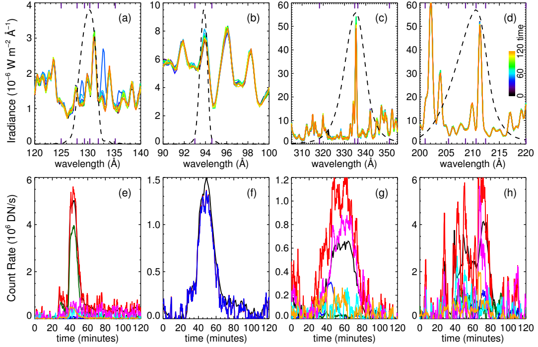
Figure 4.1: Upper: solar spectra observed by SDO /EVE for four SDO /AIA channels ((a) AIA/131 Å, (b) AIA/94 Å, (c) AIA/335 Å, and (d) AIA/211 Å) with colors indicating the time of observations. The arbitrarily scaled effective areas of these AIA EUV channels are overplotted in dashed lines. Lower: predicted light curves in four AIA channels (in units of DN/s) by convolving the EVE-observed irradiance spectrum in different wavelength ranges (different colors; the wavelength ranges are also indicated by tick marks in the upper panel) with AIA wavelength response functions in comparison with the total counts light curves observed by AIA (black). (e) AIA/131 Å, Red (EVE full spectra), blue ([125.0 Å, 128.0 Å]), dark green ([128.0 Å, 129.4 Å]), cyan([129.4 Å, 130.4 Å]), magenta([130.4 Å, 132.0 Å]), orange([132.0 Å, 135.2 Å]). (f) AIA/94 Å, Red (EVE full spectra), blue([93.0 Å, 94.6 Å]). (g) AIA/335 Å, Red (EVE full spectra), blue ([128.0 Å, 135.2 Å]), dark green ([135.2 Å, 318.0 Å]), cyan([318.0 Å, 334.8 Å]), magenta([334.8 Å, 336.2 Å]), orange([336.2 Å, 351.2 Å]). (h): AIA/211Å, Red (EVE full spectra), blue ([201.0 Å, 205.4 Å]), dark green ([205.4 Å, 208.6 Å]), cyan([208.6 Å, 210.6 Å]), magenta([210.6 Å, 212.4 Å]), orange([212.4 Å, 219.6 Å])
