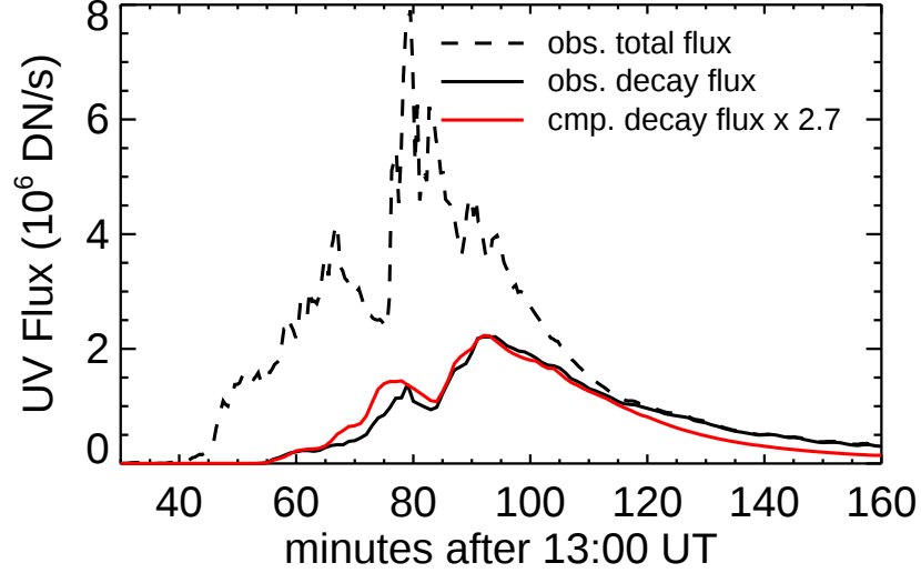
Figure 3.9: Comparison of the synthetic transition region C IV line emissions (red) in the decay phase with the UV flux observed by AIA/1600 Å channel (black) for all flare loops. The observed decay flux is derived by subtracting the full Gaussian profile that represents the rise of UV light curve from the observed light curve for each footpoint and summing over all footpoints.
