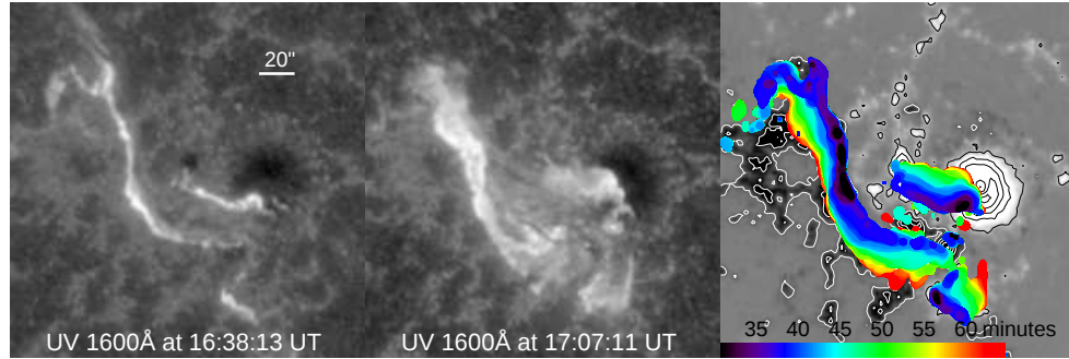
Figure 2.1: Light curves and images of the M8.0 flare observed on 2005 May 13. The upper panel shows background-subtracted and normalized light curves in HXR (25–50 keV) observed by RHESSI detector 4 (blue), SXR (1–8 Å) by GOES XRS (red), and UV (1600 Å band) by TRACE (dark green). Also plotted are the time derivatives of the 1–8 Å SXR flux (brown), and magnetic reconnection flux (black) measured by using UV 1600 Å observations and the longitudinal magnetogram from SOHO /MDI. The left and middle images in the lower panel are snapshots of UV images during the impulsive and decay phases of the flare observed by TRACE , while the lower right panel shows evolution of the UV brightening on top of the MDI longitudinal magnetogram taken at 16:03:02 UT with the color bar indicating the start times of UV brightening at different locations.
