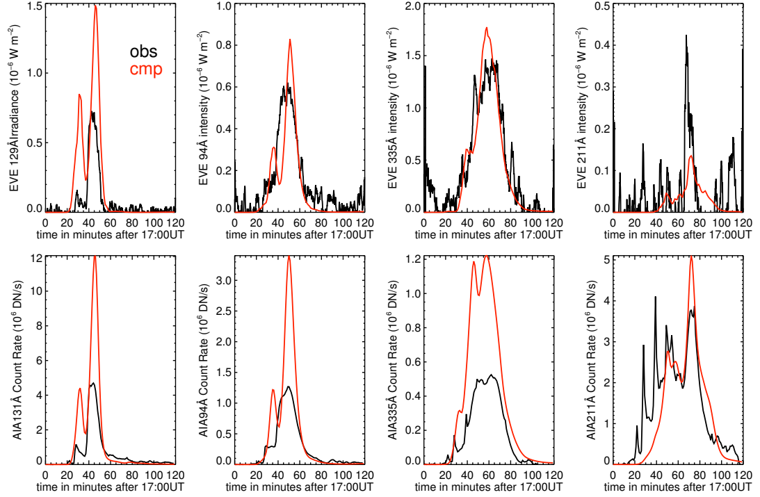
Figure 4.5: Top Panel: comparison of the synthetic line intensities in four iron lines Fe XXII line at 128.75 Å, Fe XVIII line at 93.93 Å, Fe XVI line at 335.41 Å, and Fe XIV line at 211.32 Å (red) with EVE-observed line emissions from the flare (black). Bottom panel: comparison of the synthetic light curves (red) with that observed (black) in four AIA EUV channels (131 Å, 94 Å, 335 Å, and 211 Å).
