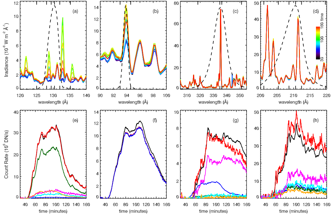
Figure 3.3: Upper: solar spectra observed by SDO /EVE for four SDO /AIA channels ((a) AIA/131 \text{\AA} , (b) AIA/94 \text{\AA} , (c) AIA/335 \text{\AA} , and (d) AIA/211 \text{\AA} ) with colors indicating the time of observations. The arbitrarily scaled effective areas of these AIA EUV channels are overplotted in dashed lines. Lower: predicted light curves in four AIA channels (in units of DN/s) by convolving the EVE-observed irradiance spectrum in different wavelength ranges (different colors; the wavelength ranges are also indicated by tick marks in the upper panel) with AIA wavelength response functions in comparison with the total counts light curves observed by AIA (black). (e) AIA/131 \text{\AA} , Red (EVE full spectra), blue ([125.0 \text{\AA} , 128.0 \text{\AA} ]), dark green ([128.0 \text{\AA} , 129.4 \text{\AA} ]), cyan([129.4 \text{\AA} , 130.4 \text{\AA} ]), magenta([130.4 \text{\AA} , 132.0 \text{\AA} ]), orange([132.0 \text{\AA} , 135.2 \text{\AA} ]). (f) AIA/94 \text{\AA} , Red (EVE full spectra), blue([93.0 \text{\AA} , 94.6 \text{\AA} ]). (g) AIA/335 \text{\AA} , Red (EVE full spectra), blue ([128.0 \text{\AA} , 135.2 \text{\AA} ]), dark green ([135.2 \text{\AA} , 318.0 \text{\AA} ]), cyan([318.0 \text{\AA} , 334.8 \text{\AA} ]), magenta([334.8 \text{\AA} , 336.2 \text{\AA} ]), orange([336.2 \text{\AA} , 351.2 \text{\AA} ]). (h): AIA/211 \text{\AA} , Red (EVE full spectra), blue ([201.0 \text{\AA} , 205.4 \text{\AA} ]), dark green ([205.4 \text{\AA} , 208.6 \text{\AA} ]), cyan([208.6 \text{\AA} , 210.6 \text{\AA} ]), magenta([210.6 \text{\AA} , 212.4 \text{\AA} ]), orange([212.4 \text{\AA} , 219.6 \text{\AA} ])
