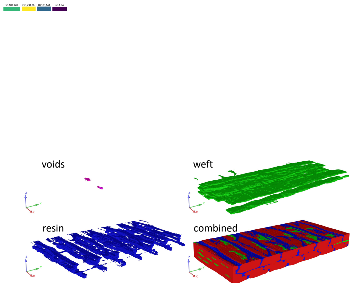
Figure 5. Finite element mesh generated showing the material regions of interest: voids, weft tows, resin, and combined with warp tows.
