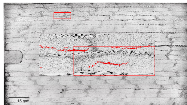
Figure 8. Optical image showing the resulting composite structure and cracks that have formed as a function of moisture uptake. Red regions indicate horizontal cracks that have formed.
