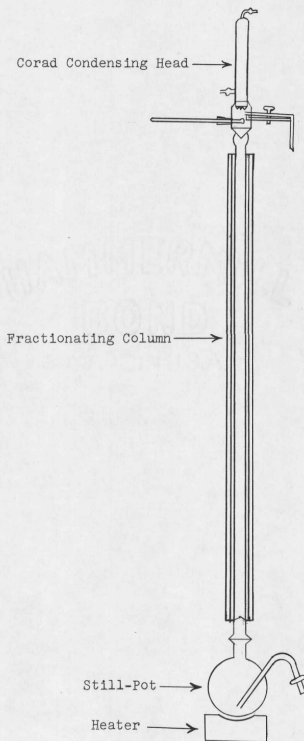
Figure 1. Diagram of Apparatus
