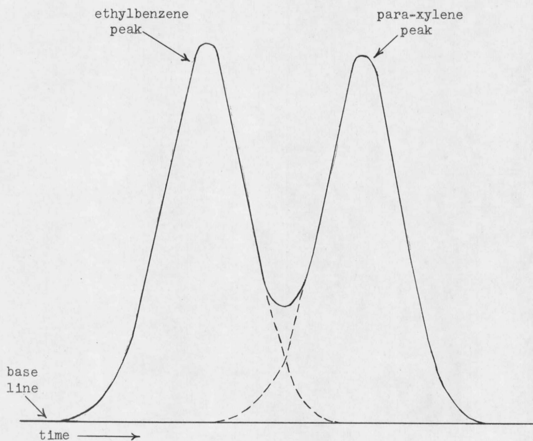
Figure 3. Chromatograph Separation Using 1-chloronaphthalene Column
