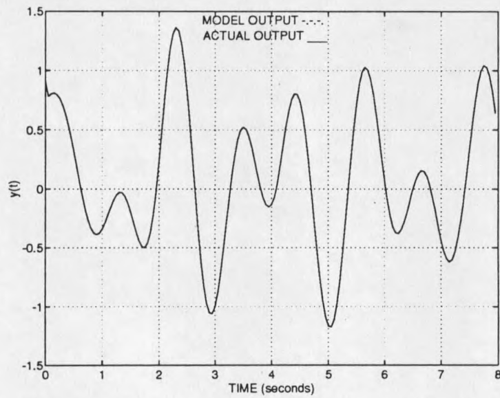
Figure 5. The output for both actual, y(t) and model, \hat{y}(t) for Example 1.
