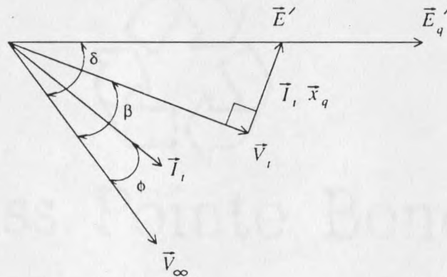
Figure 25. Steady-state vector diagram of bus voltages.
