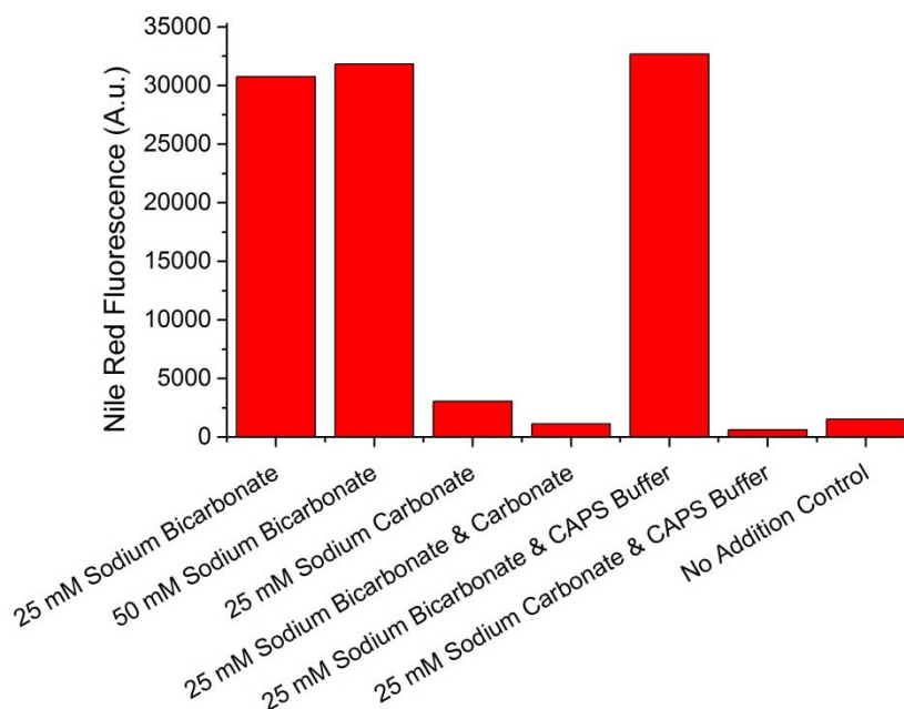
Figure 2. Nile Red fluorescence responses of Scenedesmus sp. WC-1 cultures that were amended with sodium bicarbonate, sodium carbonate, and combinations of the two with and without 50 mM CAPS buffer (pKa 10.3) (values are for the conclusion of the experiments). Growth was maintained in unbuffered Bold's basal medium illuminated with a 14:10 L/D cycle.
