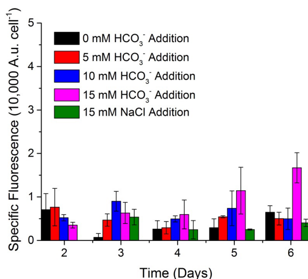
Figure 4. Mean and standard deviation of Scenedesmus sp. WC-1 specific Nile Red fluorescence in cultures which were sparged with 5% CO 2 (v/v) in air and switched to ambient air, at which time they were amended with 0, 5, 10, and 15 mM sodium bicarbonate, along with 15 mM sodium chloride as a control amendment. The gas sparge was changed and salt amendments were added at 3 days. Growth was maintained in unbuffered Bold's basal medium illuminated with a 14:10 L/D cycle ( n = 3 ).
