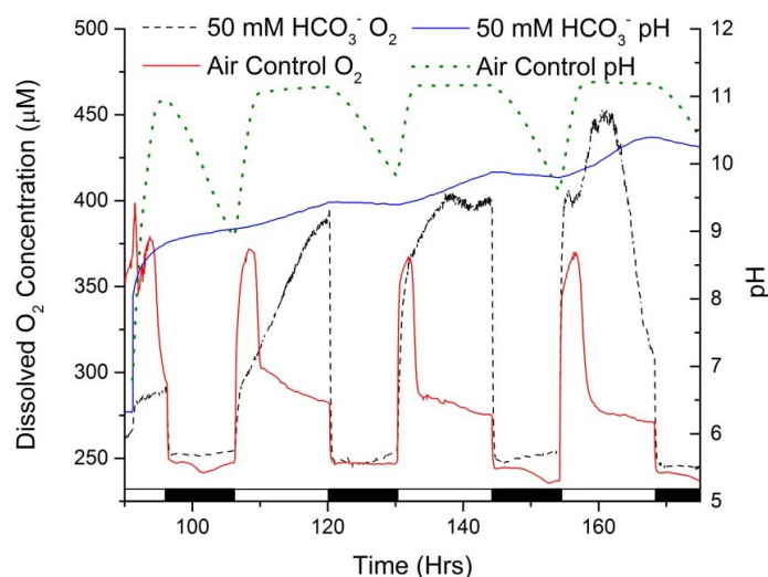
Figure 7. Dissolved oxygen (DO) concentration and medium pH of Scenedesmus WC-1 cultures which were sparged with 5% CO 2 (v/v) in air until near nitrate depletion, at which time (92 h) they were switched to ambient air and amended with 50 mM sodium bicarbonate. Comparison is made to cultures that did not receive the bicarbonate amendment. Growth was maintained in unbuffered Bold's basal medium illuminated with a 14:10 L/D cycle (bottom bar) (representative individual pH and DO profiles for triplicate culturing, n = 3 ).
