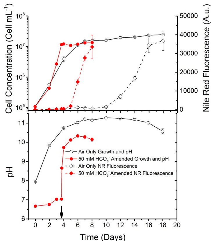
Figure 1. Scenedesmus sp. WC-1 mean and standard deviation of cellular concentration, total Nile Red fluorescence, and pH of cultures aerated with ambient air and cultures which were sparged with 5% CO 2 (v/v, in air) until near nitrate depletion, at which time they were amended with 50 mM sodium bicarbonate and switched to ambient air. Arrow indicates time of the gas sparge change and bicarbonate addition. Growth was maintained in unbuffered Bold's basal medium illuminated with a 14:10 L/D cycle ( n = 3 ). Figure adapted from [15].
