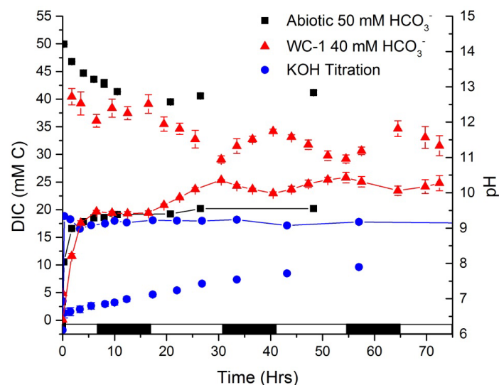
Figure 6. Bold's basal medium DIC (symbol only) and pH (symbol with line) when 50 mM NaHCO 3 was added, when 50 mM CHES buffer (pKa 9.3) and KOH was added to titrate the pH to 9.3 (abiotic experiments, n = 1 ), or mean and standard deviation when 40 mM NaHCO 3 was added to cultures of Scenedesmus WC-1 to induce TAG accumulation (biotic experiments, n = 3 ). Time axis begins at onset of abiotic experimentation or time of the gas sparge change and bicarbonate addition for the biotic experiment that was illuminated with a 14:10 L/D cycle (bottom bar).
