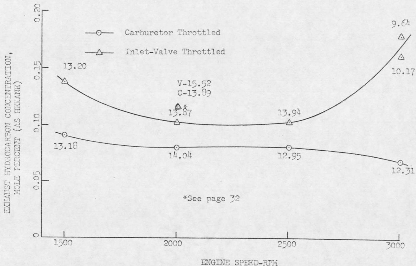
Figure 15. Exhaust Hydrocarbon Concentration as a Function of Engine Speed at Dynamometer Torque-Meter-Reading of 2.5 and Inlet-Valve Timing: Open 10° btdc, Close 51° abdc.
