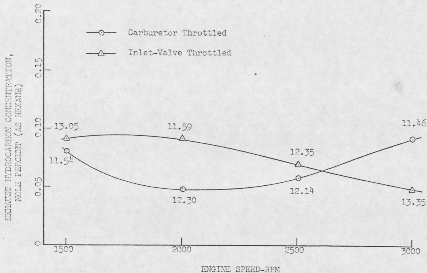
Figure 13. Exhaust Hydrocarbon Concentration as a Function of Engine Speed at Dynamometer Torque-Meter-Reading of 0.0 and Inlet-Valve Timing: Open 10° btdc, Close 51° abdc.
