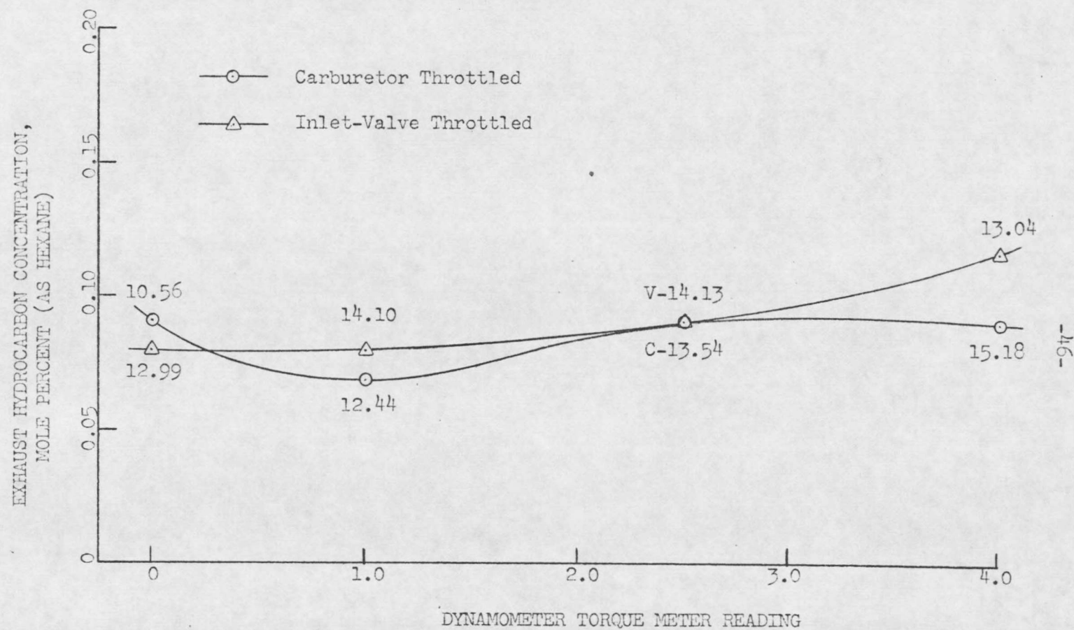
Figure 12. Exhaust Hydrocarbon Concentration as a Function of Engine Load at 2000 rpm and Inlet-Valve Timing: Open 0^{\circ} btdc, Close 35^{\circ} abdc.
