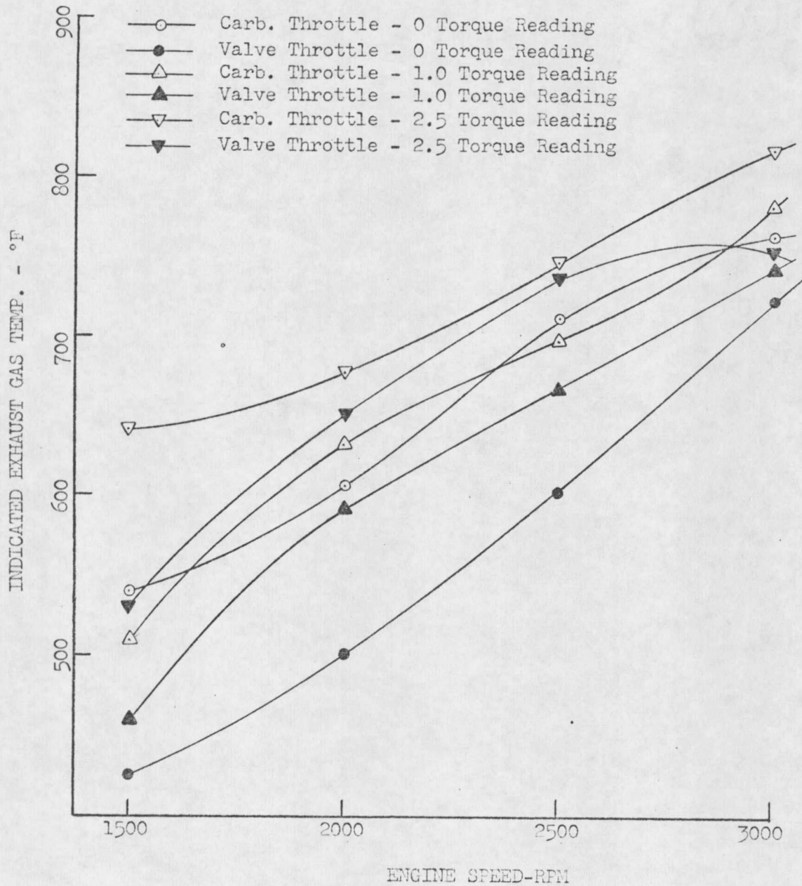
Figure 17. Comparison of Indicated Exhaust Temperatures Between Throttling Methods with Inlet-Valve Timing: Open 10° btdc, Close 51° abdc.
