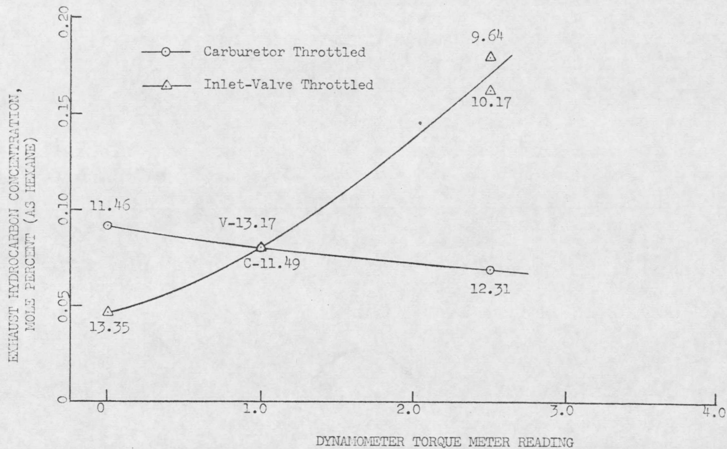
Figure 10. Exhaust Hydrocarbon Concentration as a Function of Engine Load at 3000 rpm and Inlet-Valve Timing: Open 10° btdc, Close 51° abdc.
