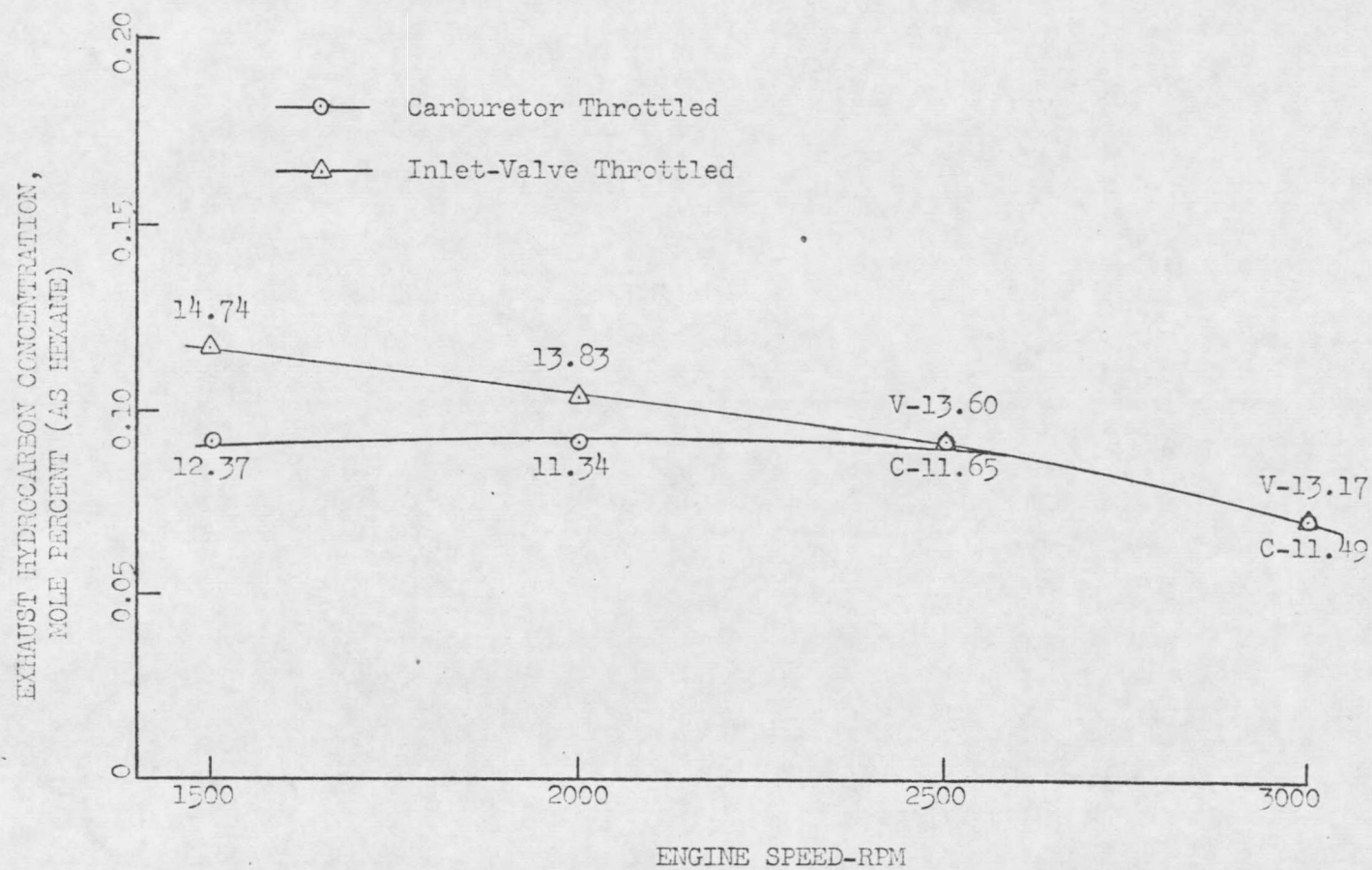
Figure 14. Exhaust Hydrocarbon Concentration as a Function of Engine Speed at Dynamometer Torque-Meter-Reading of 1.0 and Inlet-Valve Timing: Open 10° btdc, Close 51° abdc.
