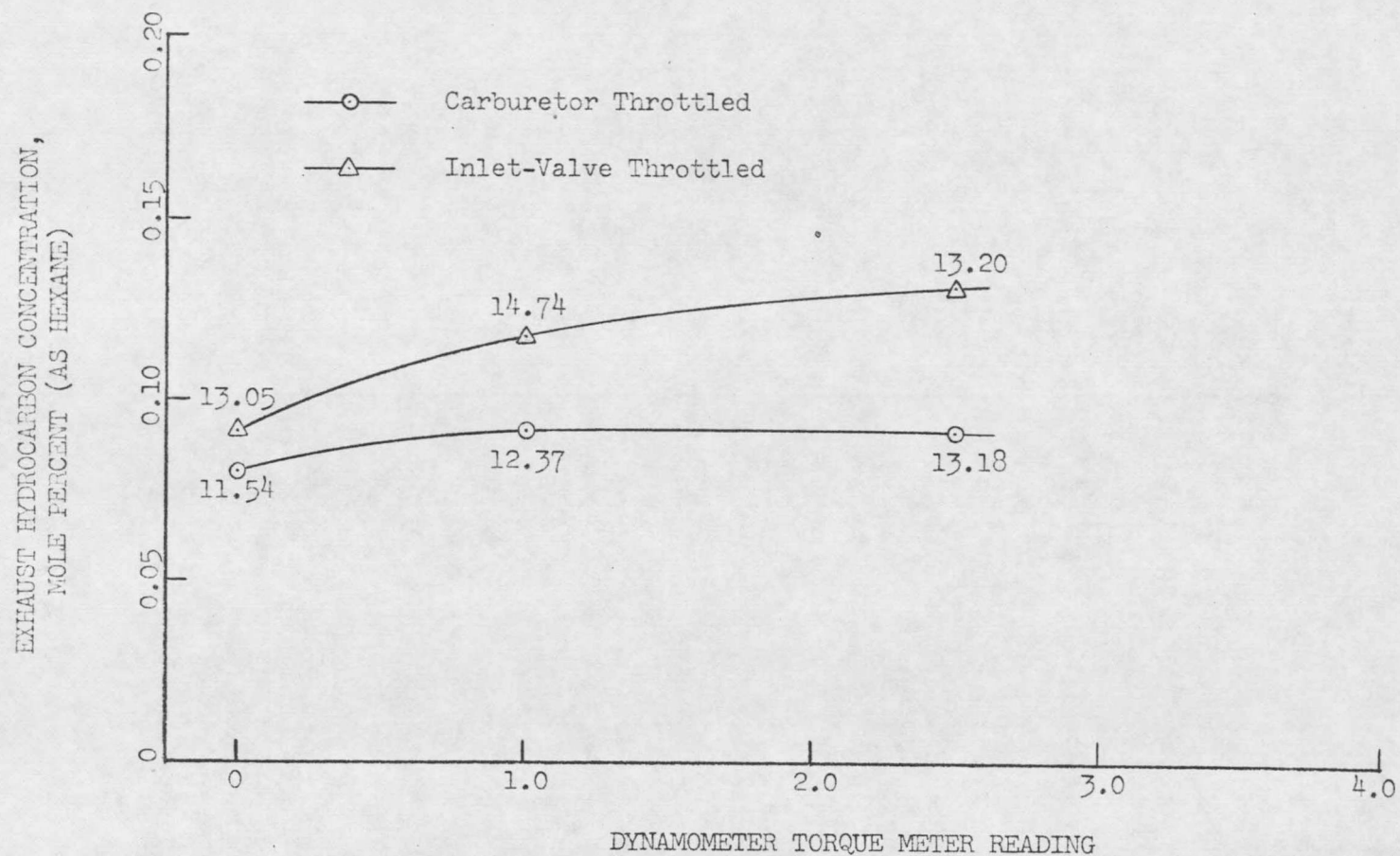
Figure 7. Exhaust Hydrocarbon Concentration as a Function of Engine Load at 1500 rpm and Inlet-Valve Timing: Open 10° btdc, Close 51° abdc.
