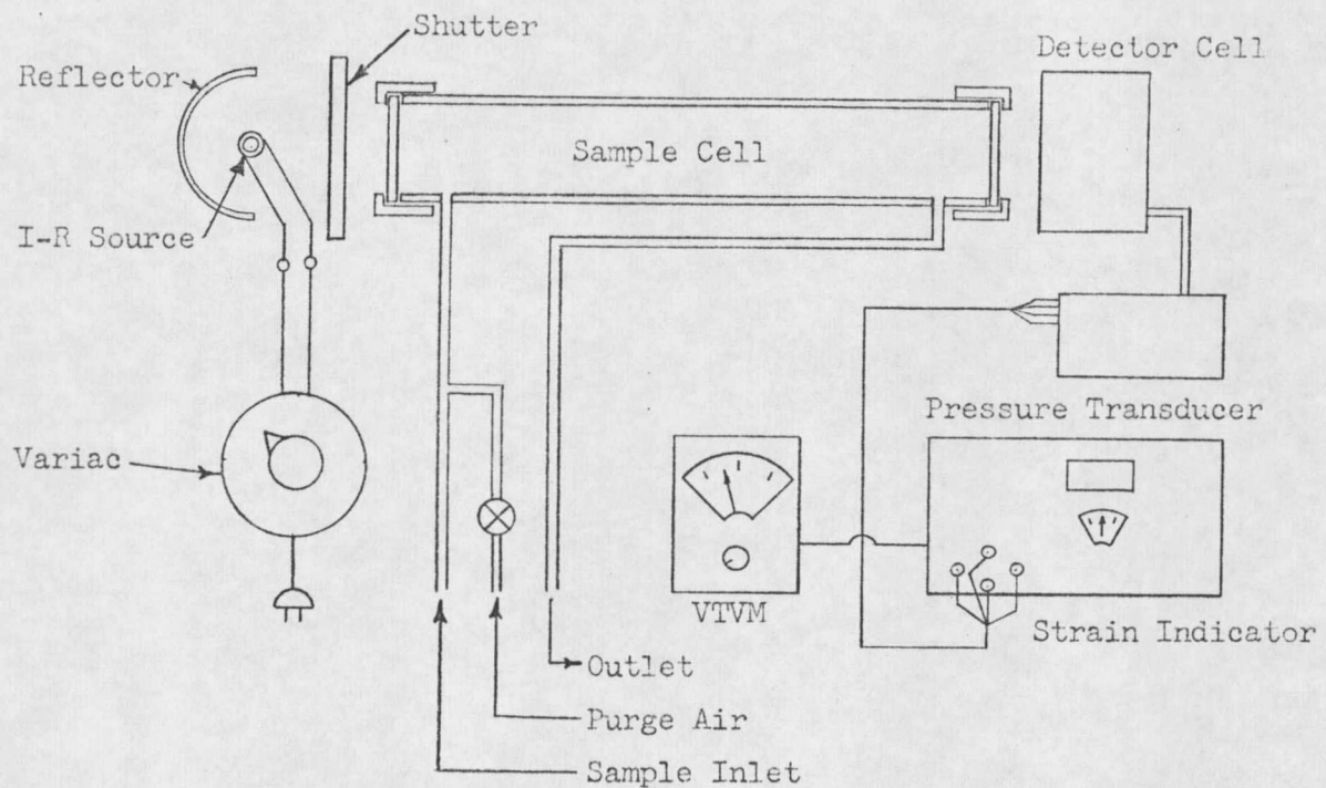
Figure 2. Schematic Diagram of Exhaust Gas Hydrocarbon Analyzer
