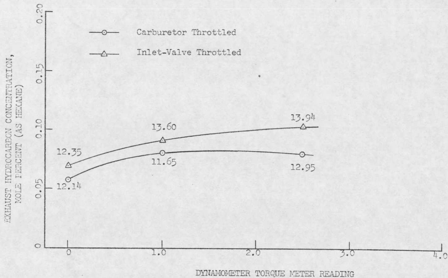
Figure 9. Exhaust Hydrocarbon Concentration as a Function of Engine Load at 2500 rpm and Inlet-Valve Timing: Open 10° btdc, Close 51° abdc.
