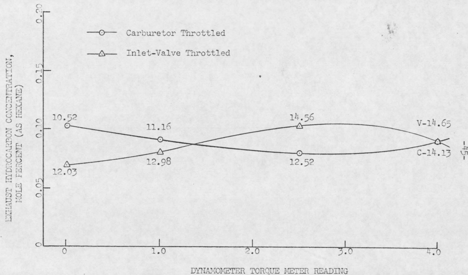
Figure 11. Exhaust Hydrocarbon Concentration as a Function of Engine Load at 2000 rpm and Inlet-Valve Timing: Open 10° btdc, Close 35° abdc.
