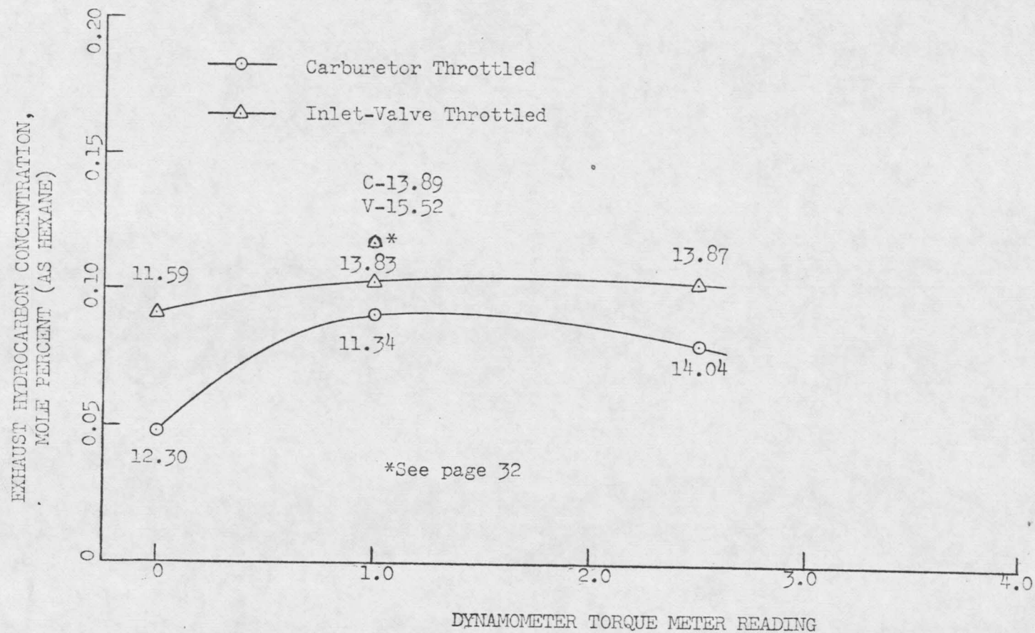
Figure 8. Exhaust Hydrocarbon Concentration as a Function of Engine Load at 2000 rpm and Inlet-Valve Timing: Open 10° btdc, Close 51° abdc.
