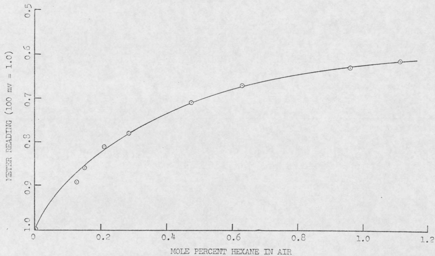
Figure 5. Response of Hydrocarbon Analyzer to N-Hexane in Air
