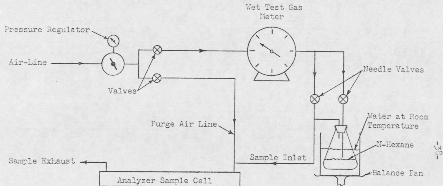
Figure 4. Schematic Diagram of Hydrocarbon Analyzer Calibration Equipment
