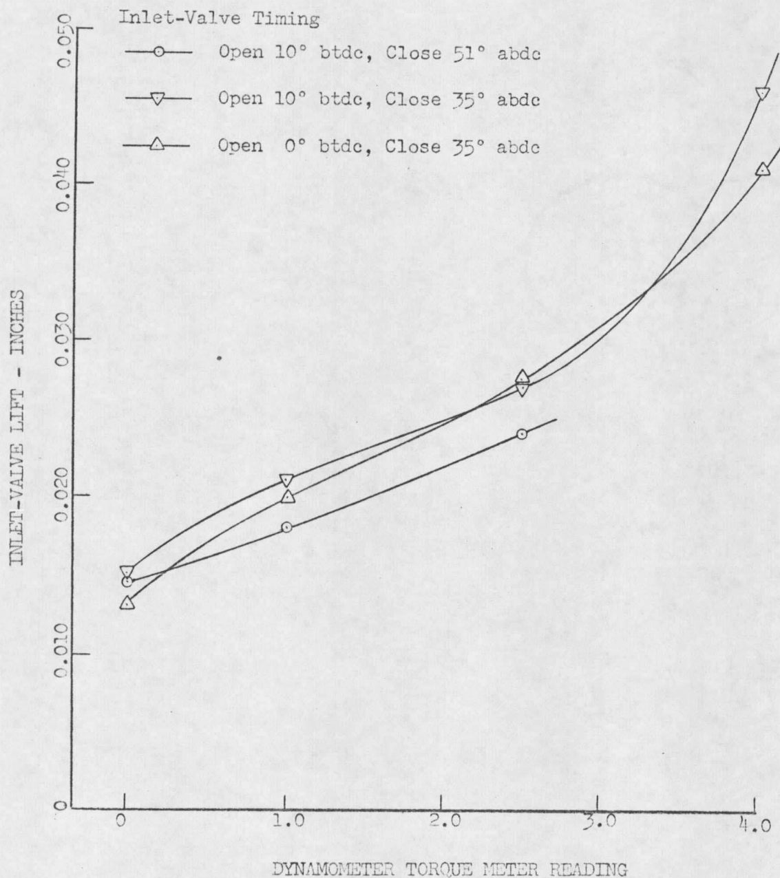
Figure 16. Required Inlet Valve Lifts for Various Engine Loads at Three Inlet-Valve Timing Specifications
