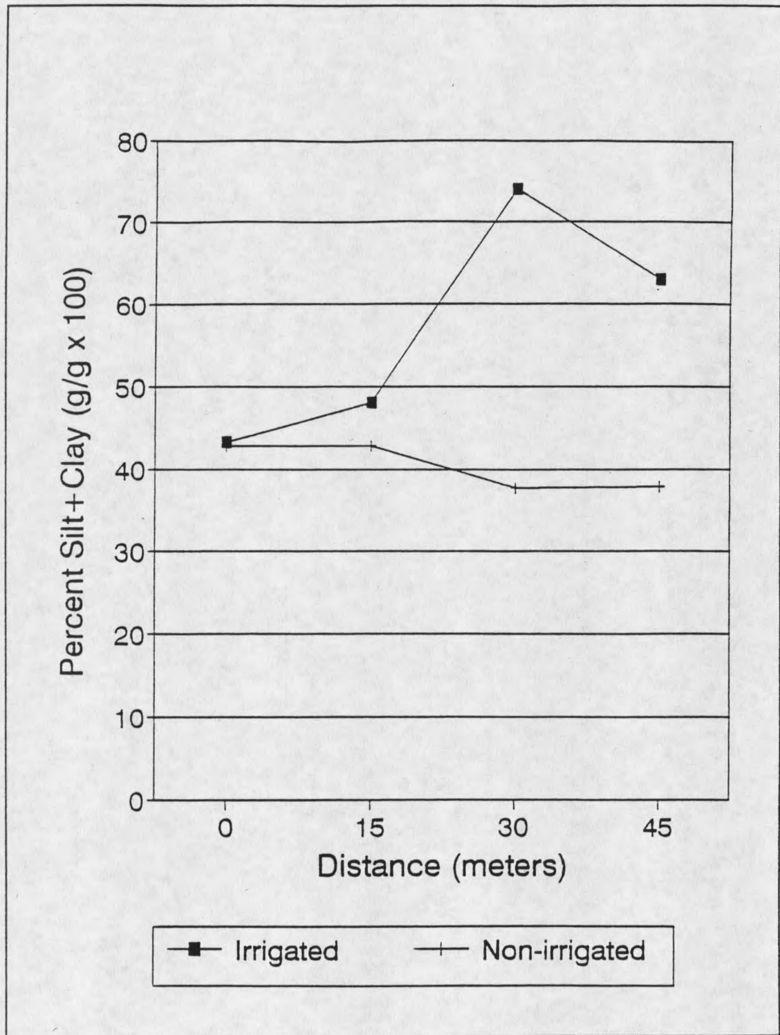
Figure 19. Comparison of percent silt + clay in soil samples obtained from various positions on irrigated and non-irrigated sites.
