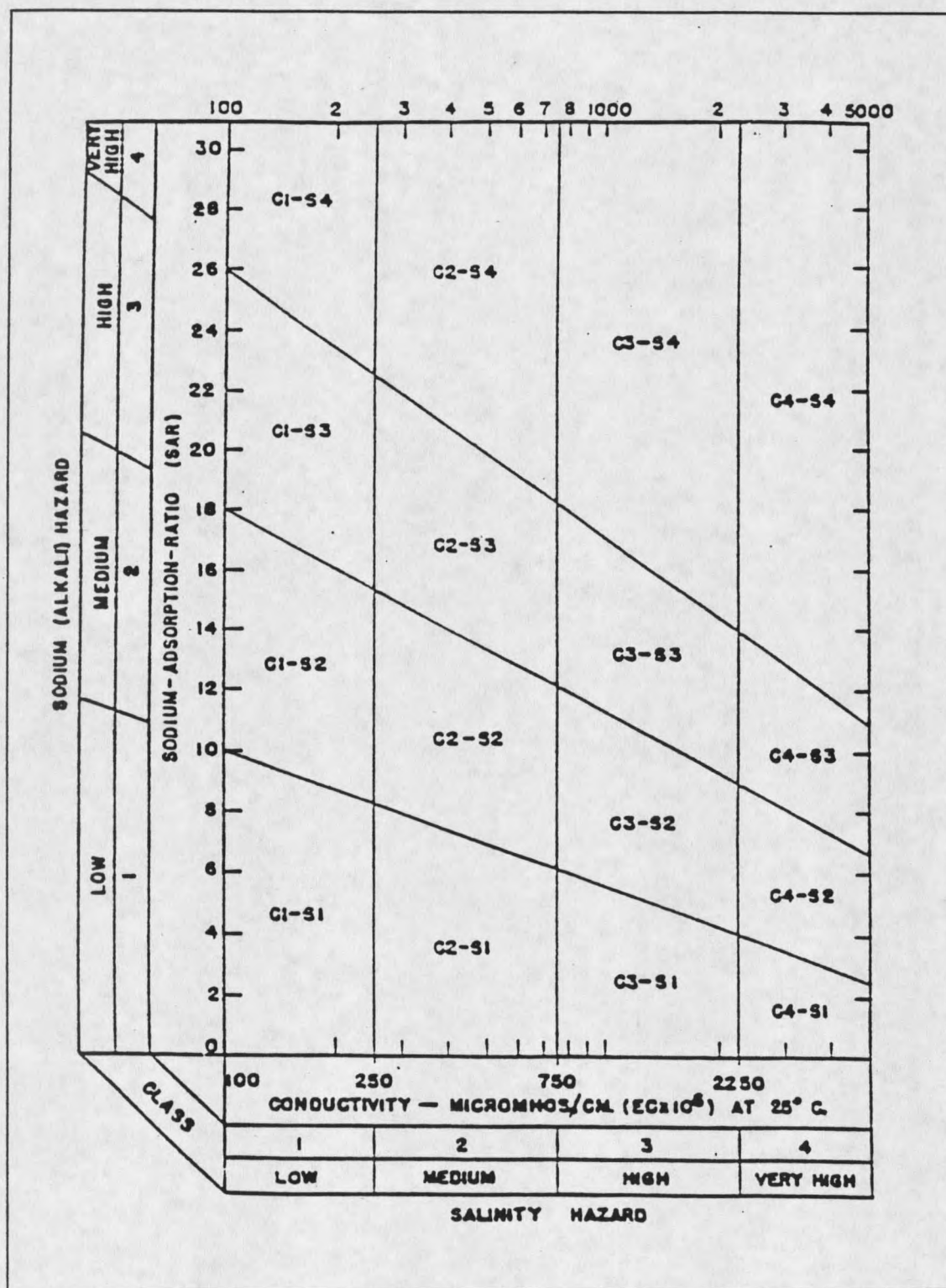
Figure 7. Suggested classification of irrigation waters (from U.S. Salinity Laboratory Staff, 1969).
