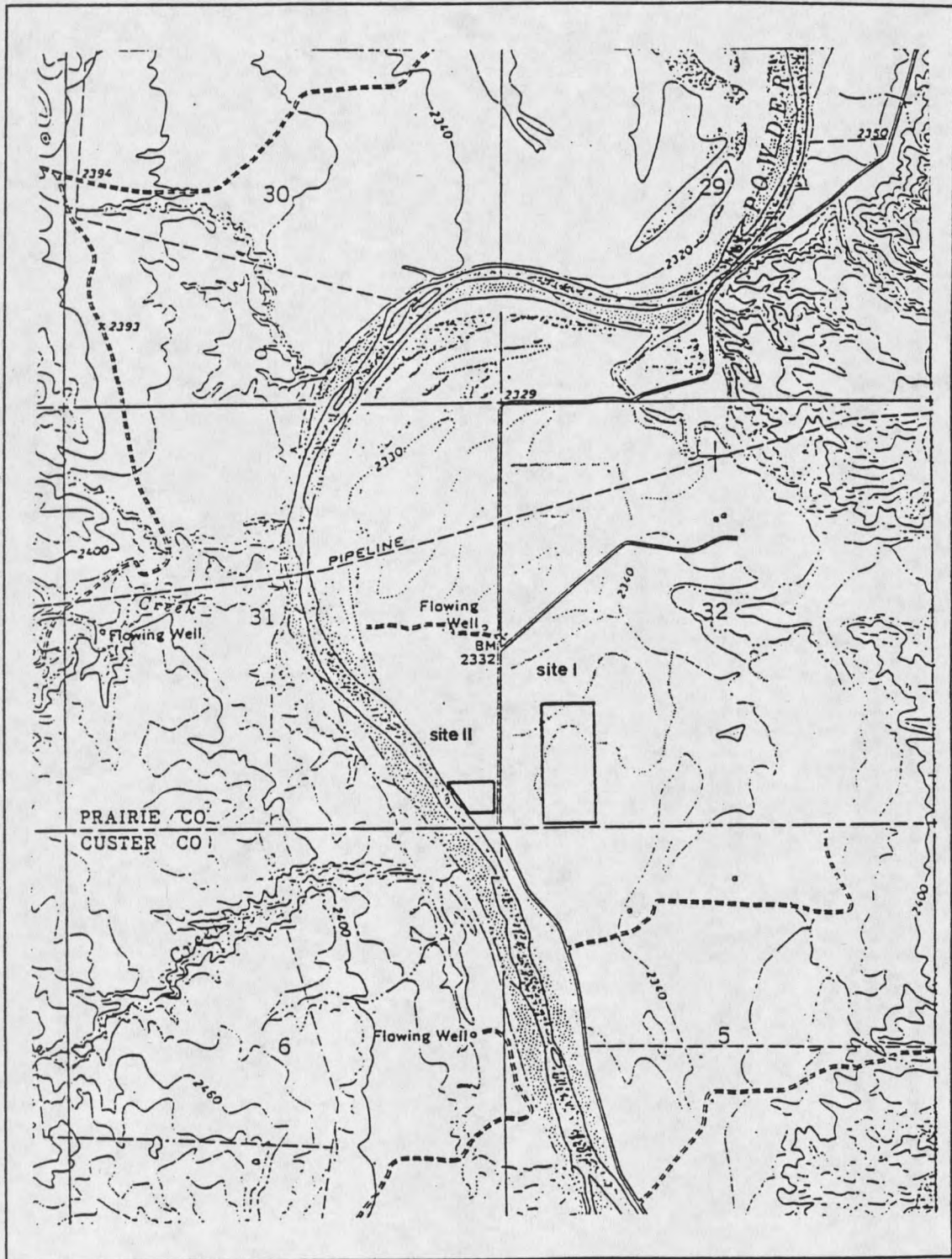
Figure 8. Map of the Powder River study area (U.S.G.S. 1964. Spring Creek Quad, 7.5 minute series topographic map).
