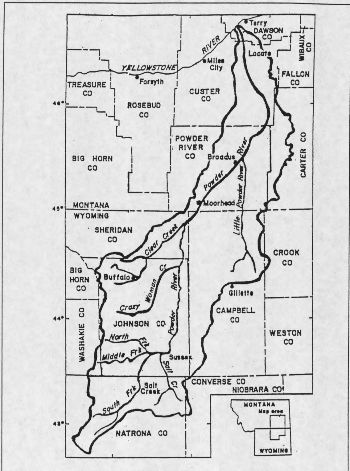
Figure 1. Map of the Powder River drainage area (from Carey, 1989).
