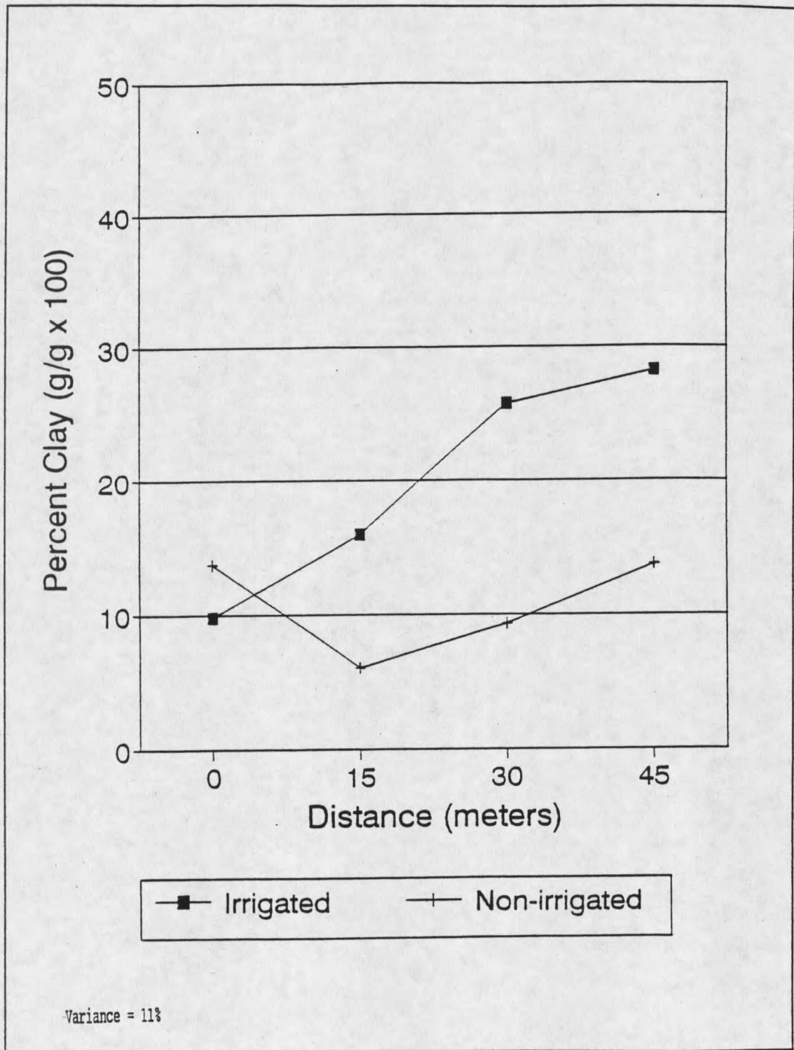
Figure 18. Comparison of percent clay in soil samples obtained from various positions on irrigated and non-irrigated sites.
