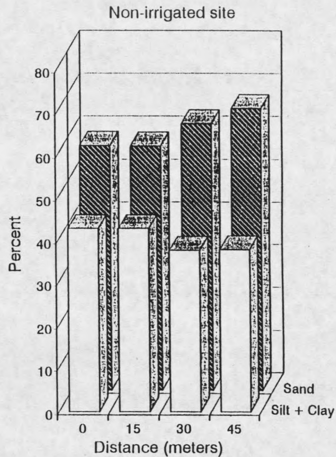
Figure 20. Ratio of percent sand to percent silt + clay of soil samples obtained from various positions on irrigated and non-irrigated sites.
