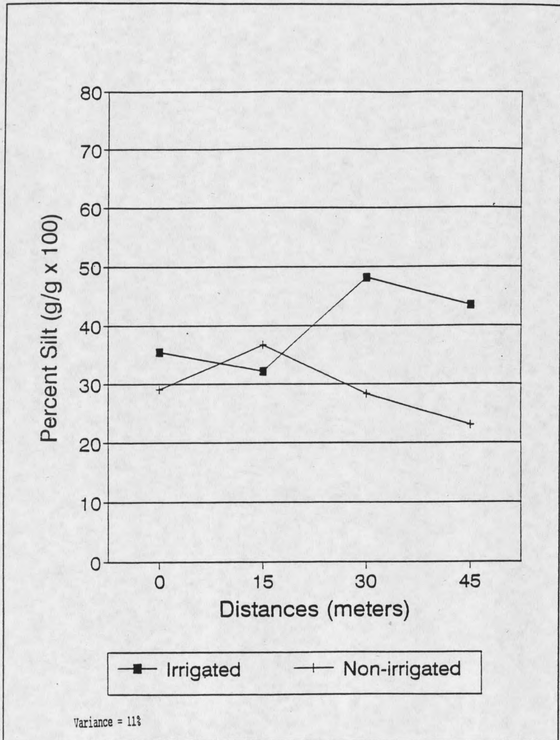
Figure 17. Comparison of percent silt in soil samples obtained from various positions on irrigated and non-irrigated sites.
