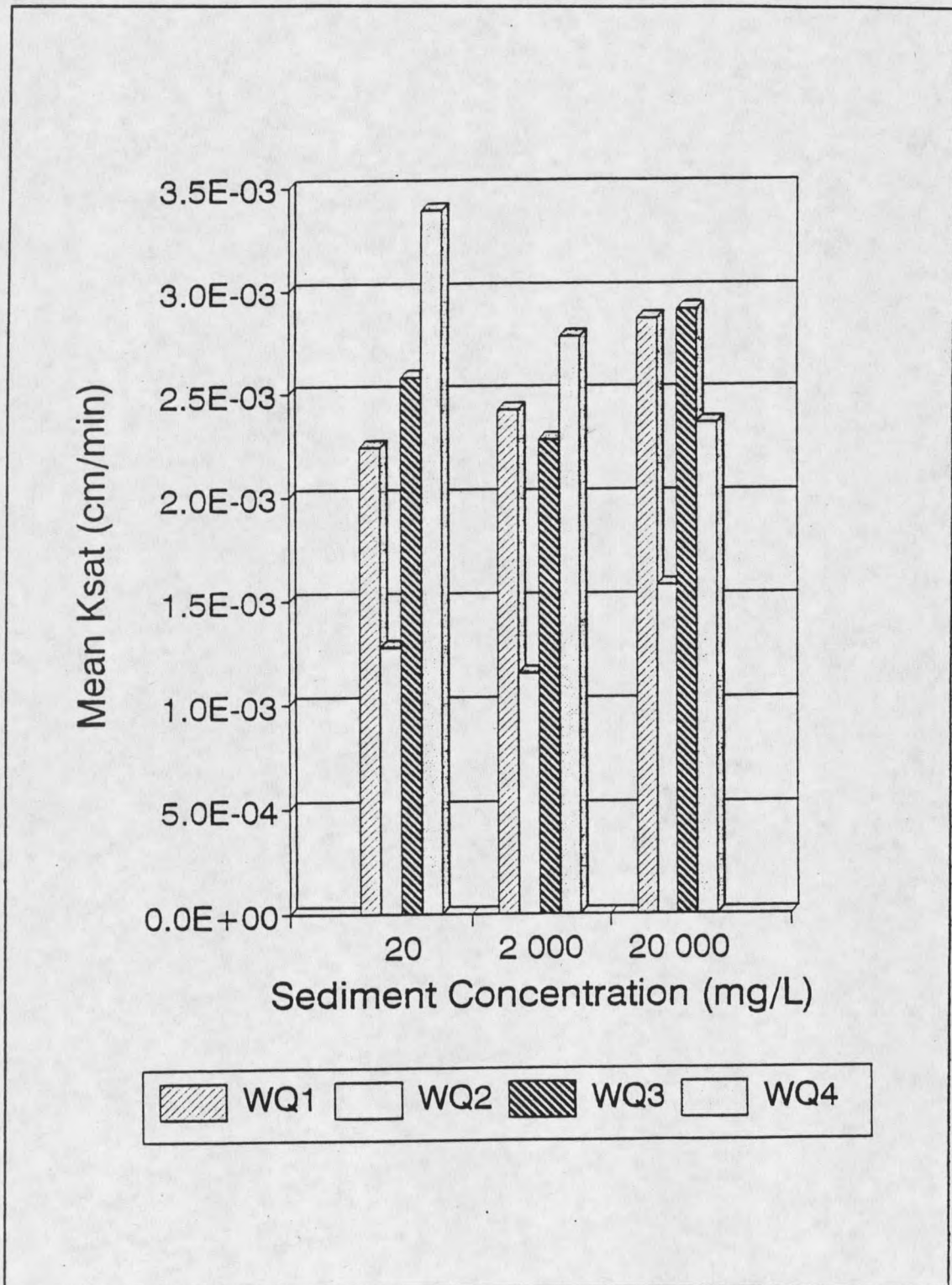
Figure 13. Mean K_{sat} as a function of water quality and sediment concentration.
