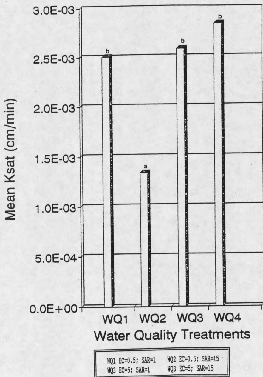
Figure 12. Mean K_{sat} as a function of water quality
