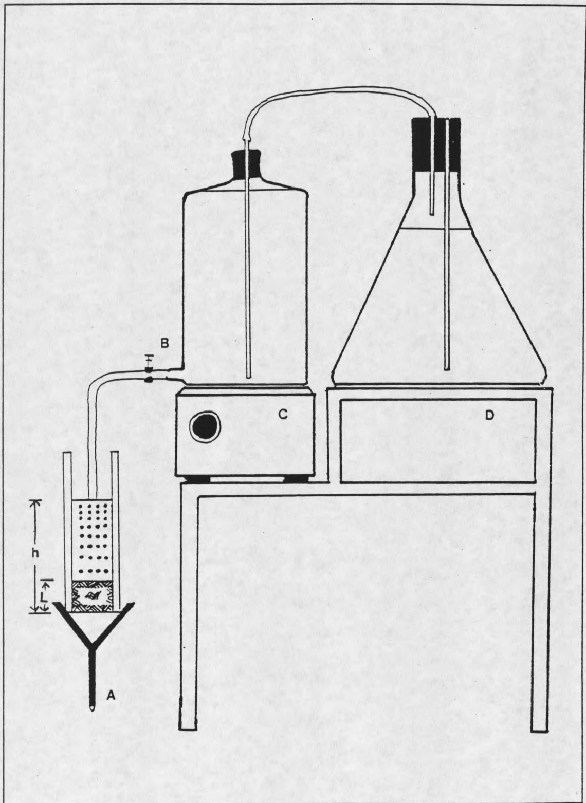
Figure 9. Experimental set-up for K_{sat} study.
