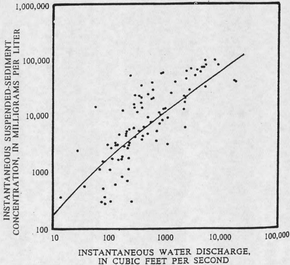
Figure 2. Relationship between streamflow and suspended sediment concentration for the Powder River (from U.S.G.S., 1986).
