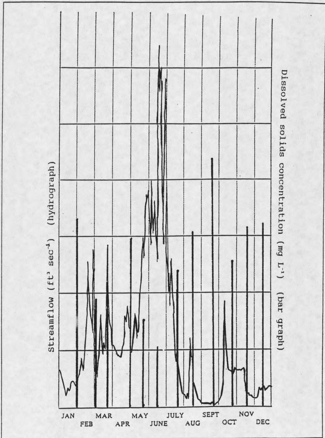
Figure 3. Relationship between Powder River streamflow and TDS near Arvada, Wyoming (from U.S.G.S., 1986).
