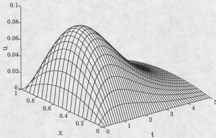
Figure 4: True solution of (4.13)
