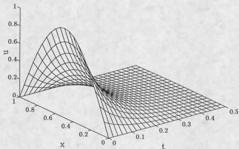
Figure 5: True solution of (4.15)
