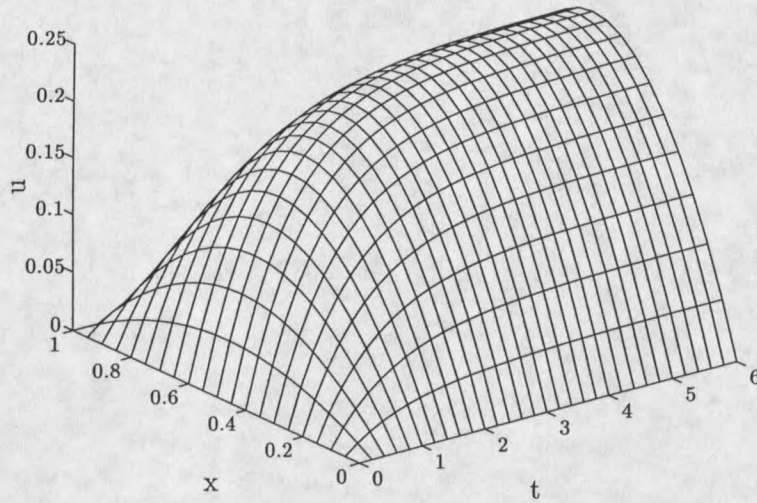
Figure 6: True solution of (4.19)
