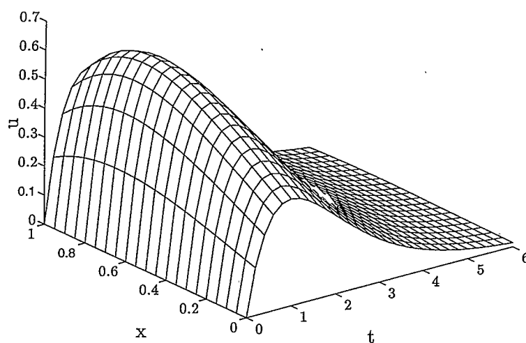
Figure 7: True solution of (4.25)
