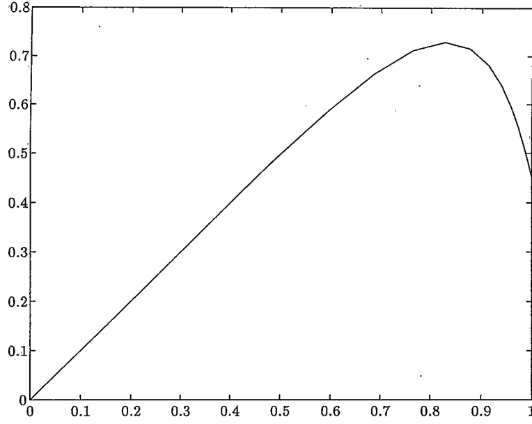
Figure 3: True solution of (3.36) with \rho = 10 , \kappa = 10
