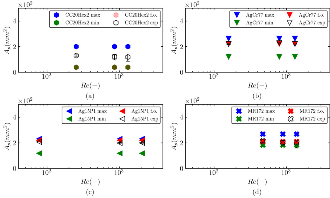
Fig. 11. Comparison between the projected areas of experiments (exp), final orientation model (f.o.), maximum (max) and minimum (min) eigenvalues projected area approach for particles (a) CC20Hex2, (b) AgCr77, (c) Ag15P1, and (d) MR172. For the capped-column CC20Hex2, the final orientation and the minimum eigenvalue projected areas coincide.
