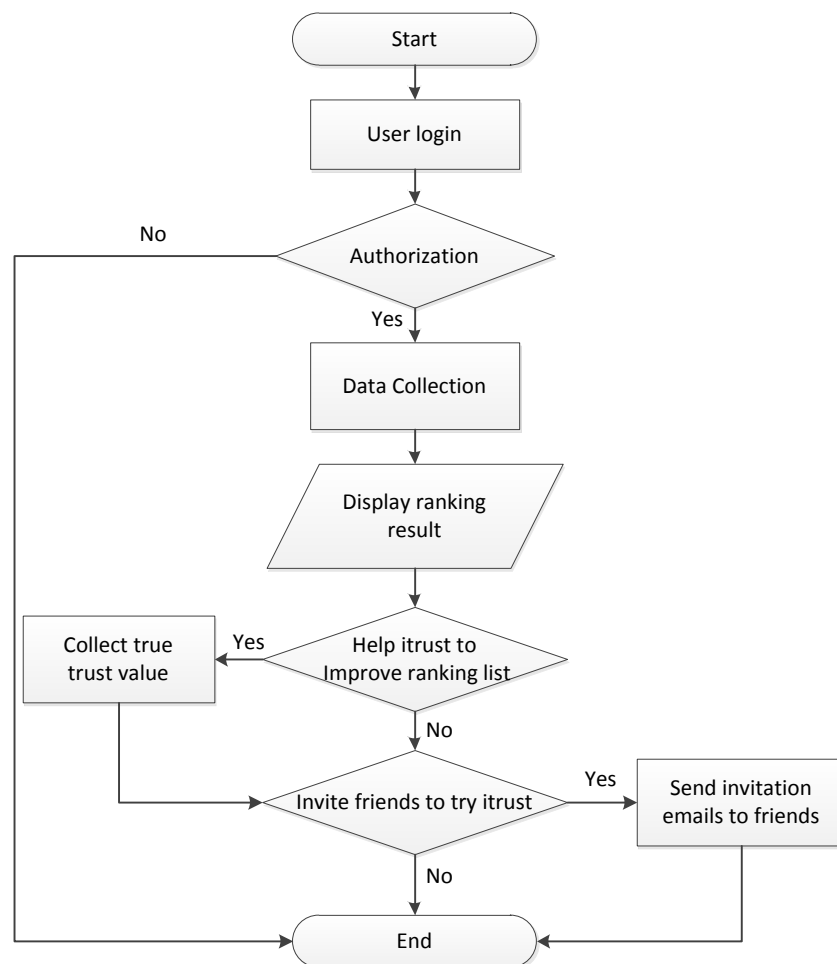
Figure 3. Flowchart of itrust
