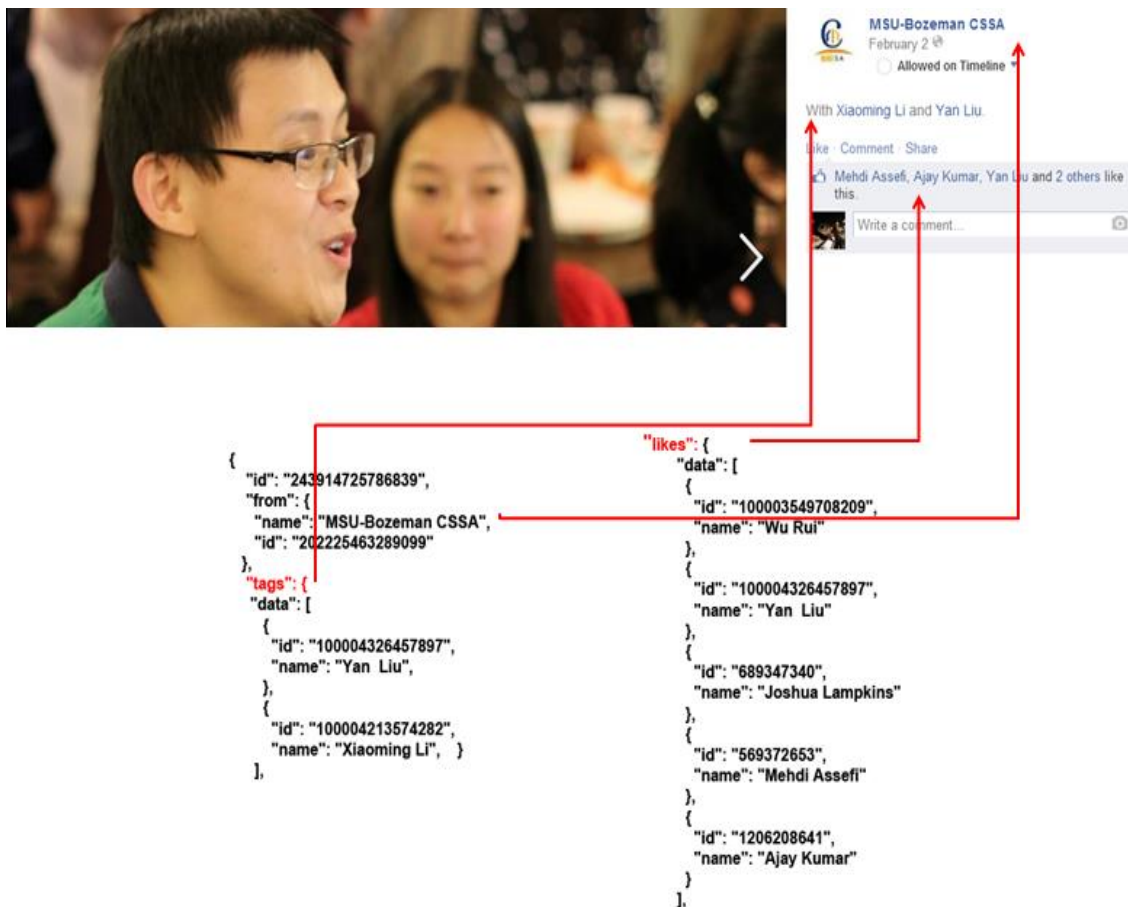
Figure 6. JSON format of fetched data
