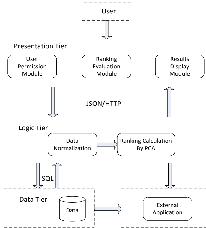
Figure 2. System architecture of itrust
