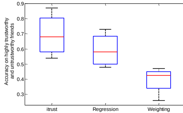
Figure 32. itrust accurately discovers highly trustworthy and highly untrustworthy friends
