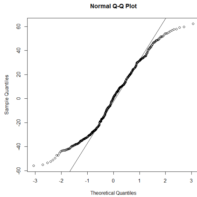
Figure 19. Normal Q-Q plot of the residuals
