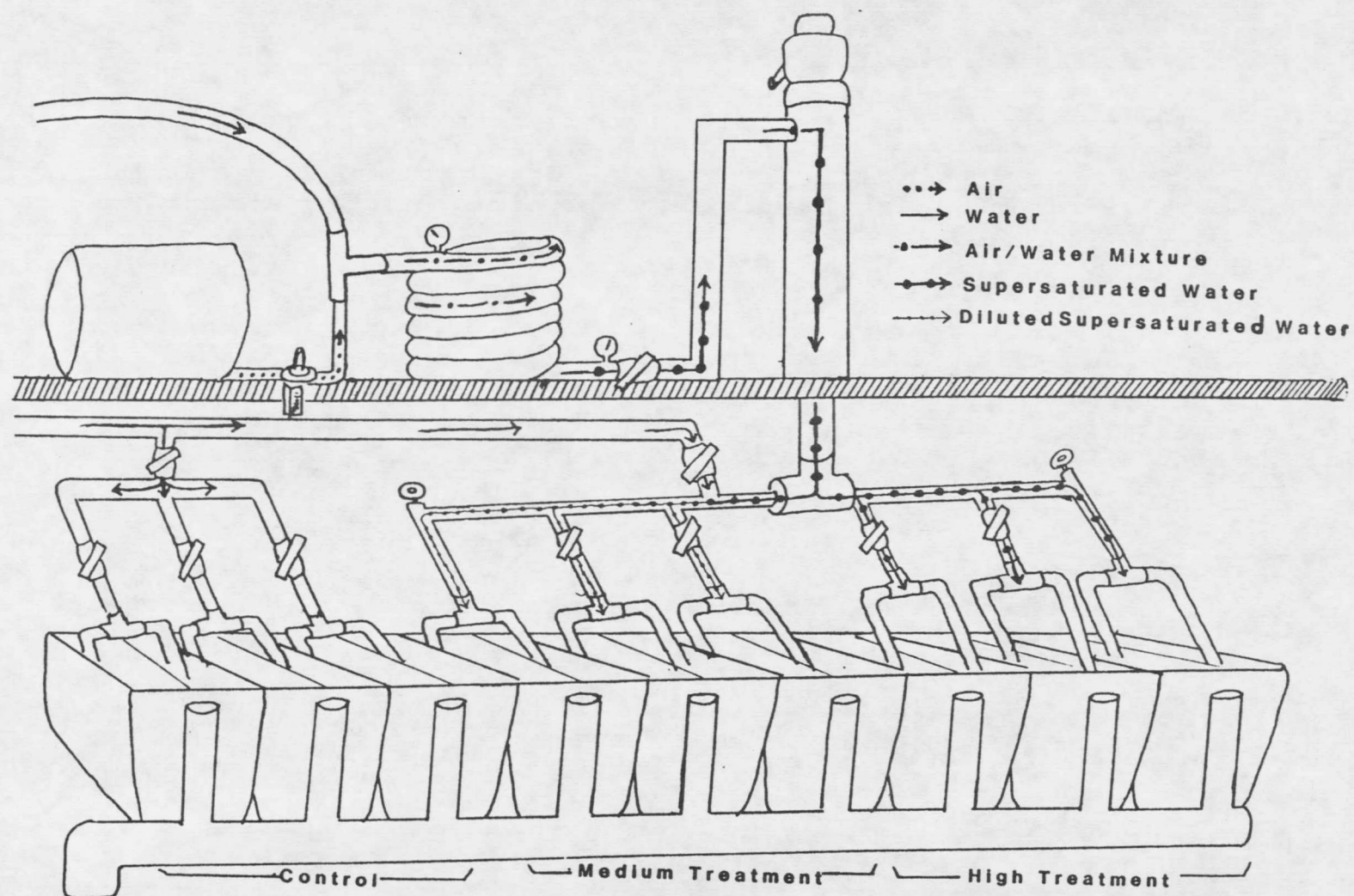
Figure 1. Laboratory apparatus used to test effects of three levels of gas supersaturation on juvenile brown and rainbow trout.
