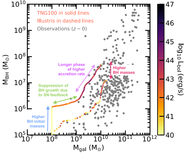
Figure 9. Illustration of one set of matched galaxies in TNG (solid line) and Illustris (dashed line) with total stellar mass of M_\star = 10^{10} M_\odot at z = 0 . Not all BHs in the same galaxy mass range follow the same track, but at least a large fraction does so. The BHs in TNG start with a higher initial mass, are stunted by an efficient SN feedback, experience longer phases of higher accretion rate than the BHs in Illustris. Consequently, the BHs in TNG reach larger masses by z = 0 in galaxies with M_{\star, z=0} = 10^{10} M_\odot . A few examples for galaxies of M_{\star, z=0} = 10^{10} M_\odot and M_{\star, z=0} = 10^{11} M_\odot are given in Appendix D.
