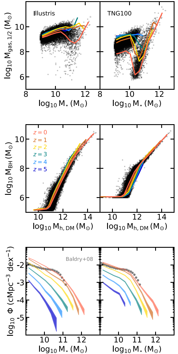
Figure 10. Different diagnostics to understand the evolution of the overall normalization of the M_{\text{BH}} - M_\star mean relation with time. Top panels: Mean mass of the gas contained in the half-mass radius of the galaxies; the entire population at z = 0 is shown in black. The gas content in the inner region of the galaxies diminishes with time. Middle panels: Mean BH mass as a function of the dark matter mass of their host haloes. We show in black all the haloes with BHs at z = 0 . At fixed dark matter halo mass, we find a larger evolution in TNG100, and almost no evolution in Illustris. Bottom panels: Galaxy stellar mass functions. Grey symbols show the observational constraints of Baldry, Glazebrook & Driver (2008) ( z \sim 0 ). The low-mass end of the galaxy mass function is overestimated in Illustris ( M_\star \leq 10^{10.5} M_\odot ); a better agreement is found for TNG100.
