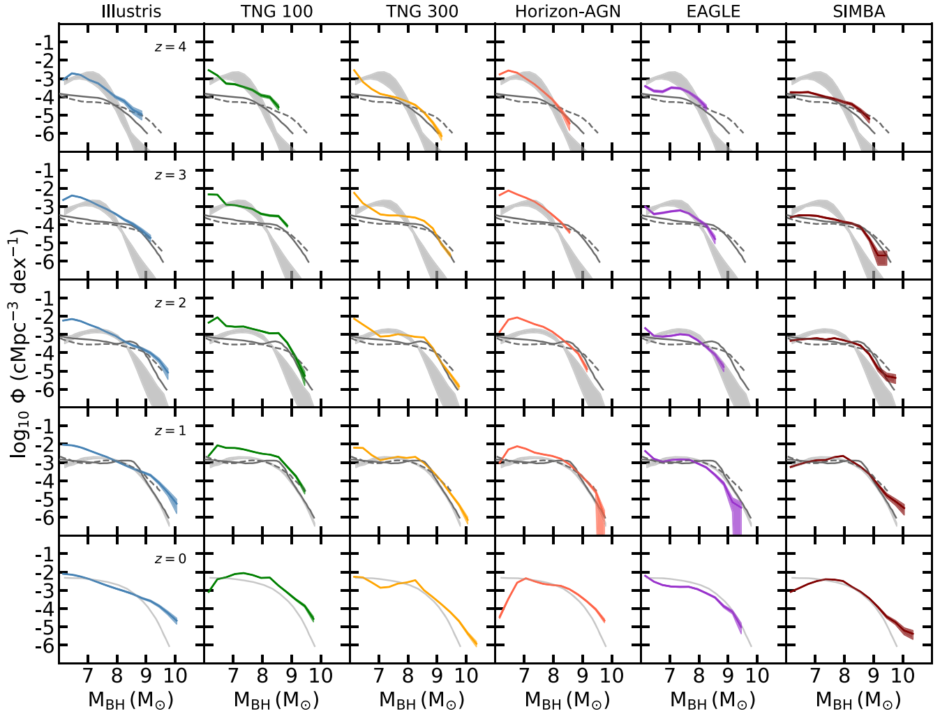
Figure 13. Redshift evolution of the BH mass function. Grey shaded areas represent the observational constraints of Merloni & Heinz (2008) for the same redshifts as for the simulations, with the exception of z = 0 for which we show the observations at z = 0.1 . We also show the observational constraints of Cao (2010) (solid grey lines) and Shankar et al. (2009) (dashed grey lines). The global trend seen in the observational constraints is reproduced, but some discrepancies are noticeable. At the low-mass end, some simulations produce too many M_{\text{BH}} \sim 10^7 M_{\odot} BHs at some redshift (Illustris, TNG, Horizon-AGN), or not enough (EAGLE), compared to the constraints of Merloni & Heinz (2008). All the simulations (except EAGLE) overproduce BHs of M_{\text{BH}} \sim 10^{10} M_{\odot} at z = 0 .
